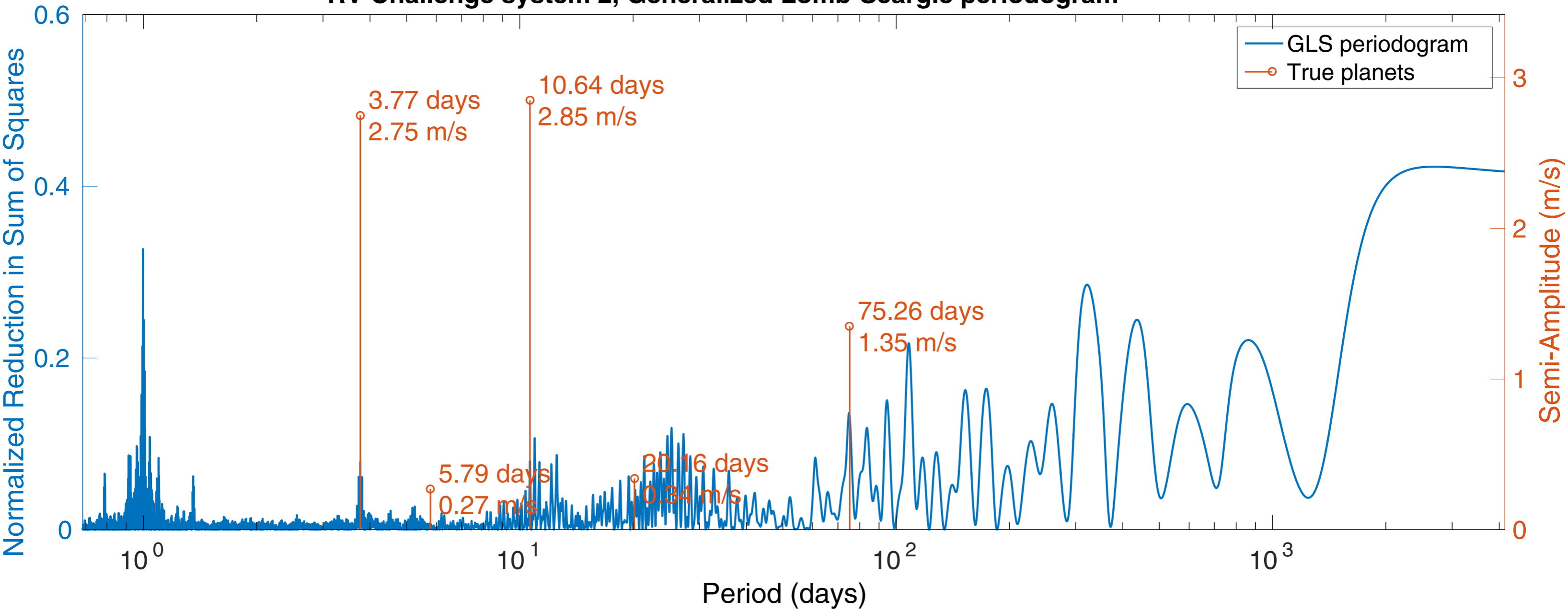
RV Challenge system 2, Generalized Lomb-Scargle periodogram
