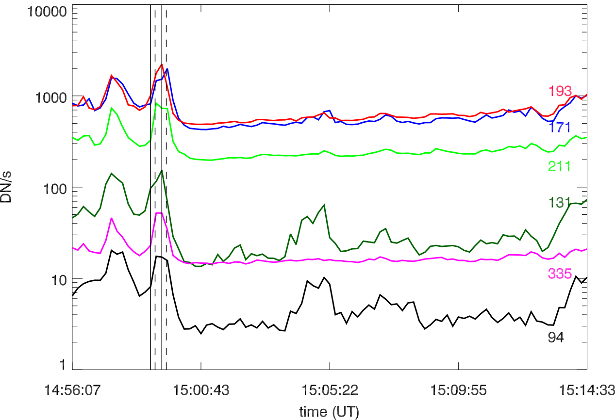
AIA light curve for the spire
