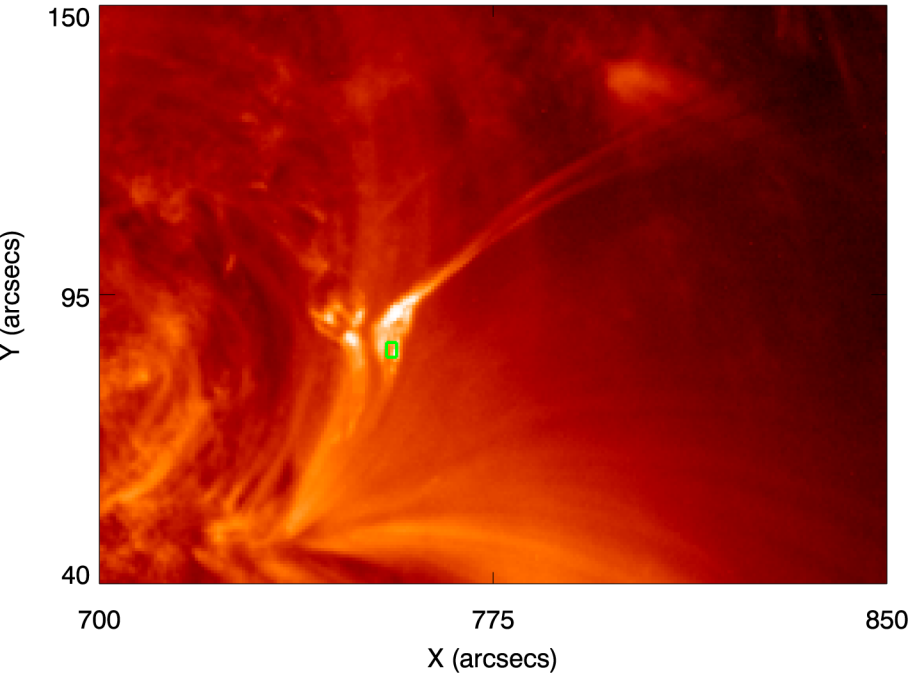
AIA 171 Å 16:35:12 UT (footpoint)
