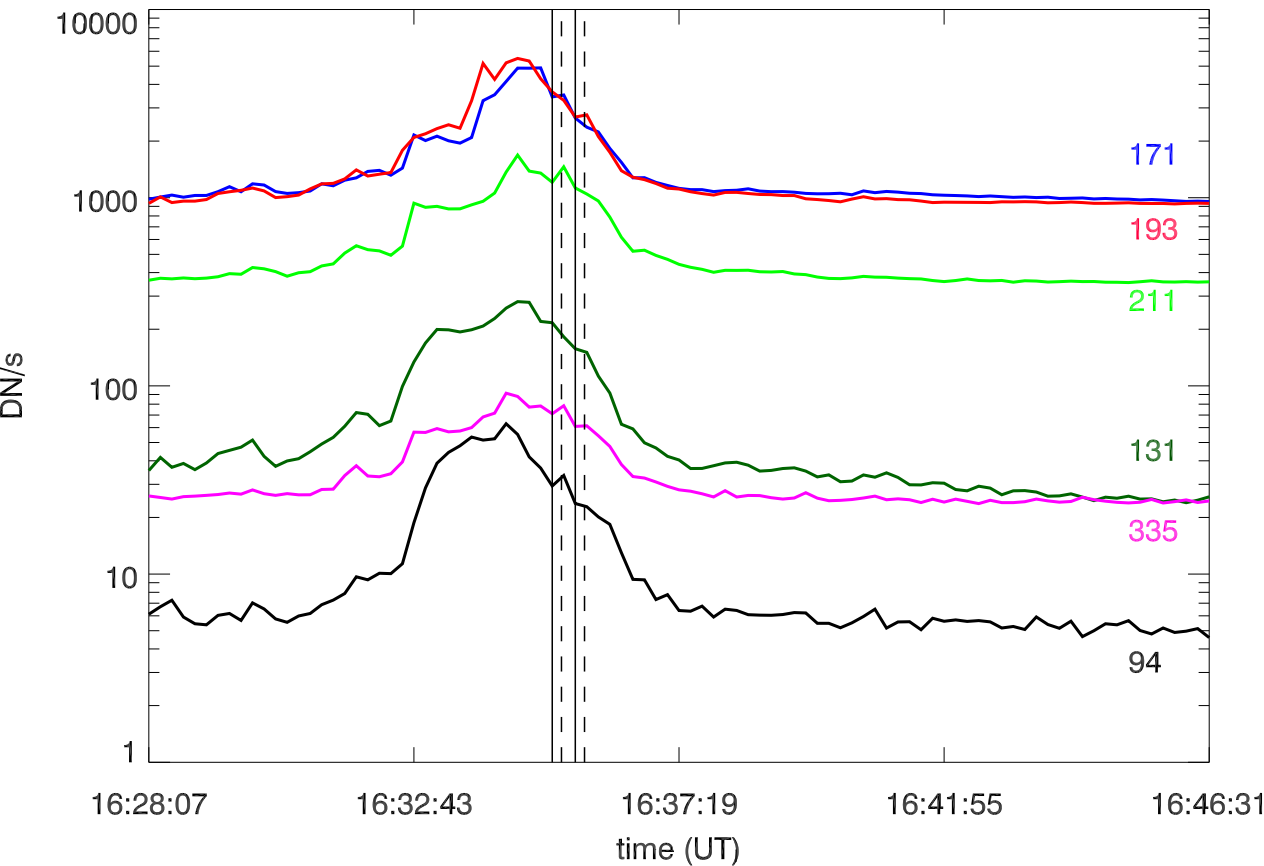
AIA light curve for the footpoint
