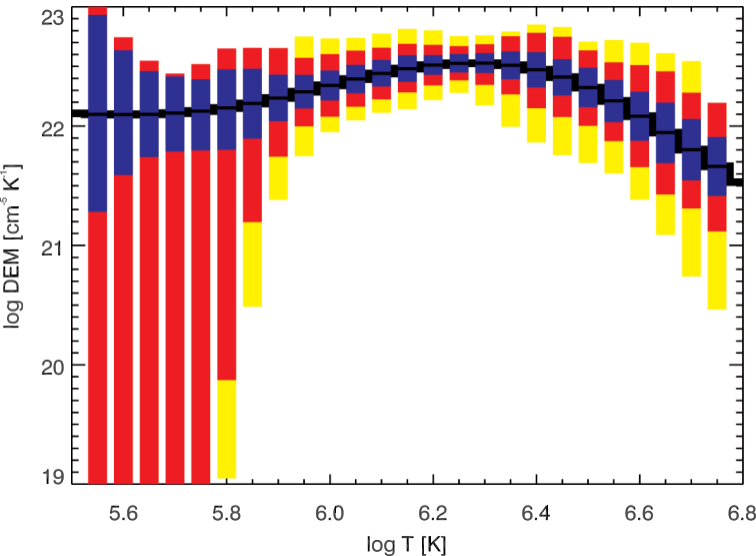
DEM of the jet-footpoint (AIA-XRT)
