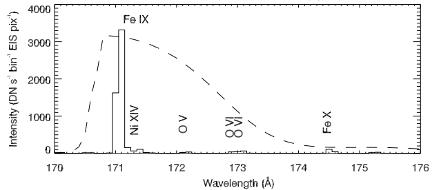
AIA 171 Å from AIA-XRT DEM (spire)
