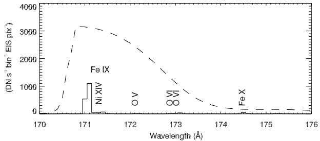
AIA 171 Å from EIS DEM (spire)
