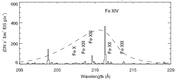
AIA 335 Å from EIS DEM (spire)
