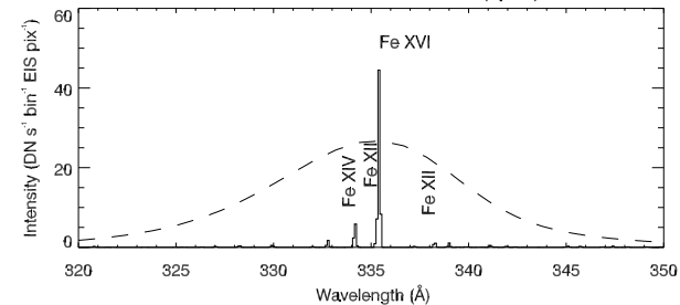
AIA 335 Å from AIA-XRT DEM (spire)
