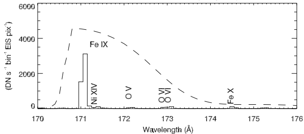
AIA 171 Å from EIS DEM (footpoint)
