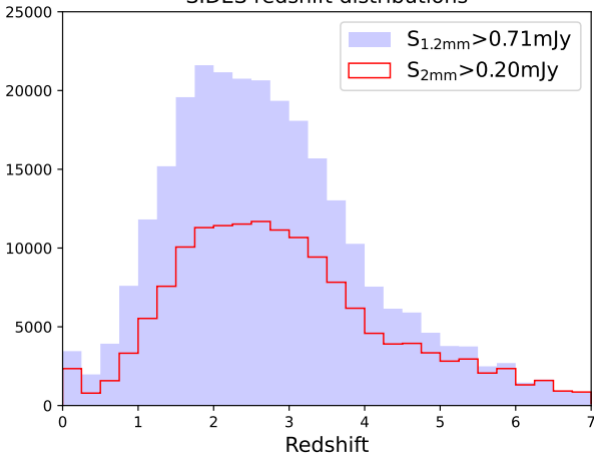
SIDES redshift distributions
