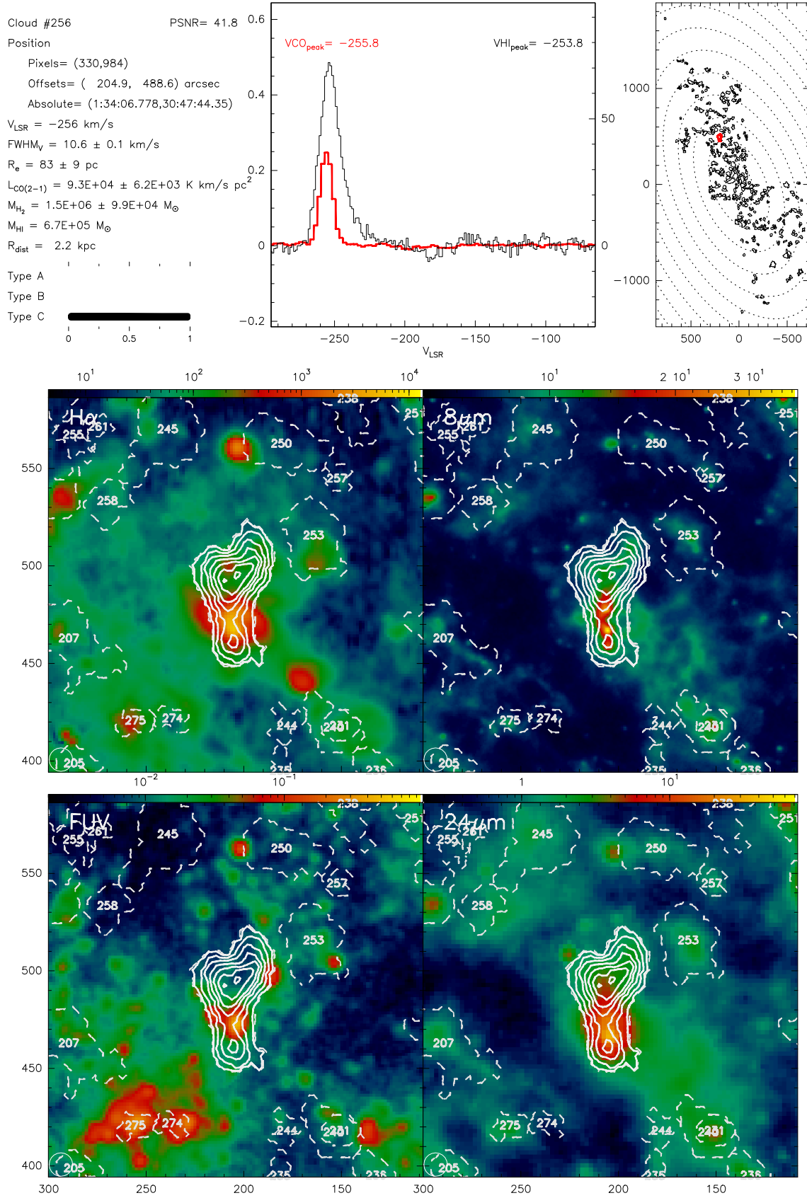
Fig. B.256. Catalogue entry for cloud 256. See description at the beginning of this appendix.
