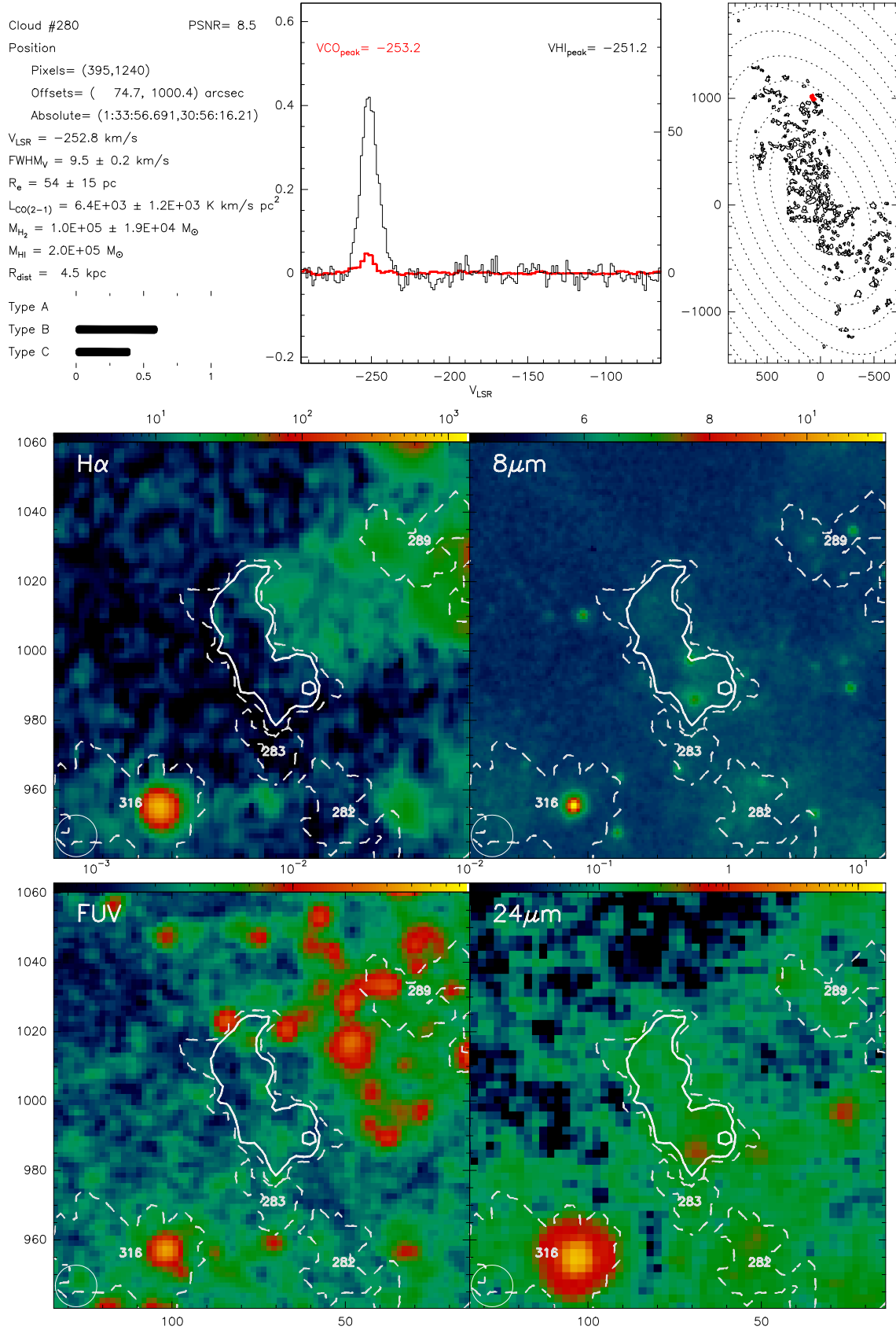
Fig. B.280. Catalogue entry for cloud 280. See description at the beginning of this appendix.
