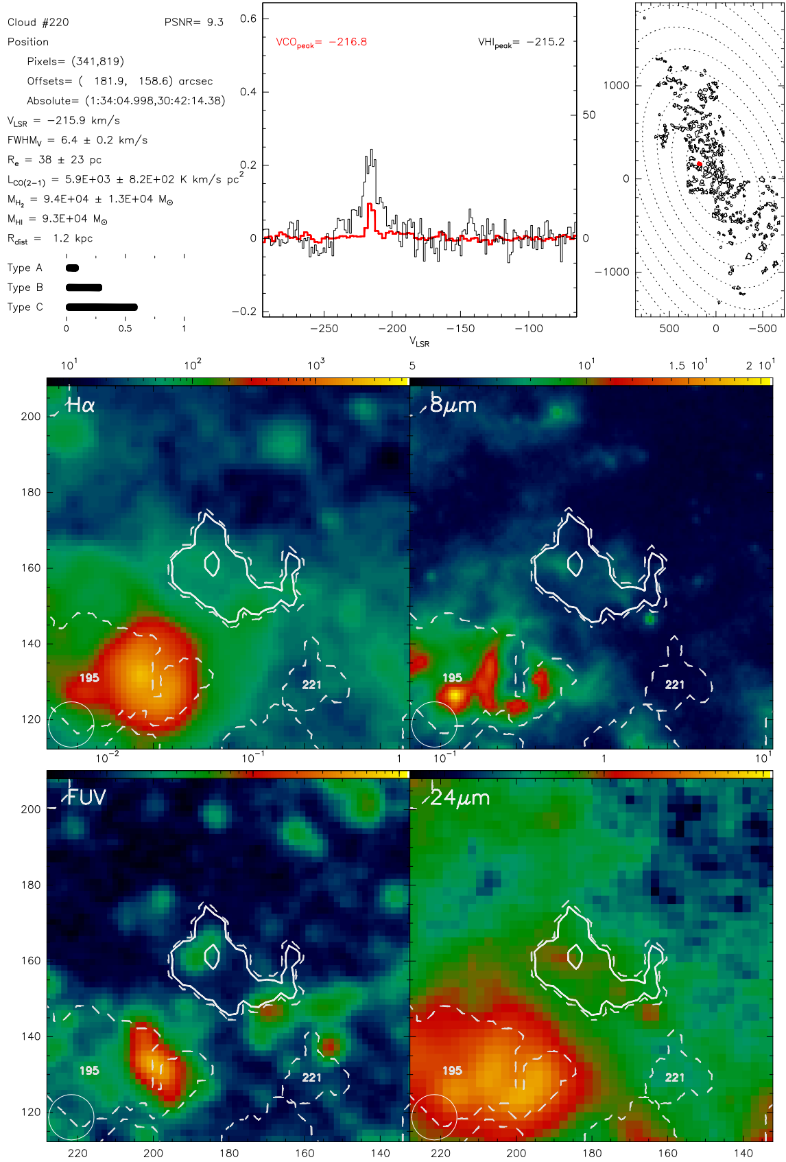
Fig. B.220. Catalogue entry for cloud 220. See description at the beginning of this appendix.
