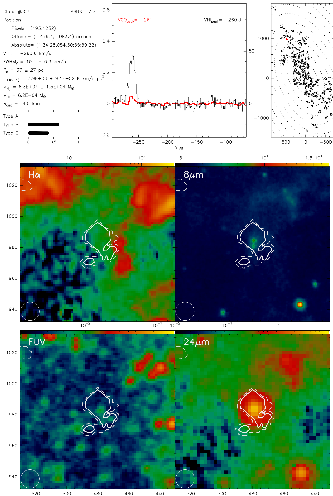
Fig. B.307. Catalogue entry for cloud 307. See description at the beginning of this appendix.
