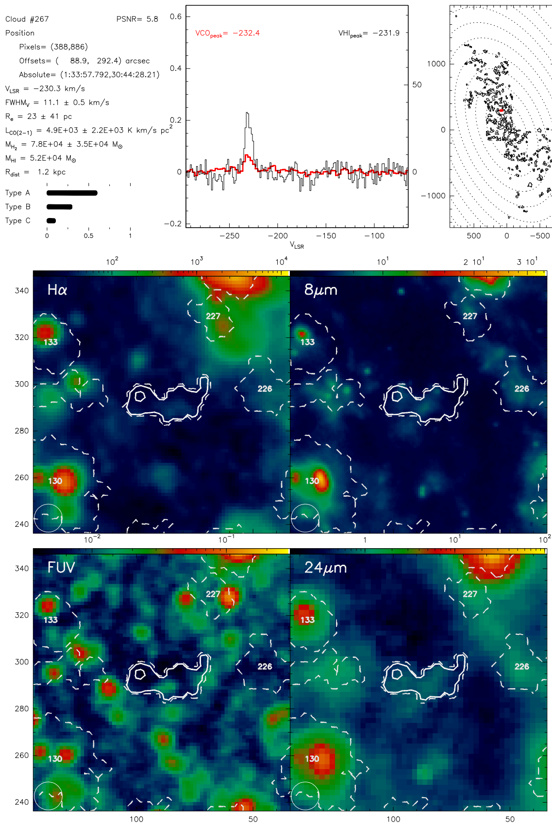
Fig. B.267. Catalogue entry for cloud 267. See description at the beginning of this appendix.
