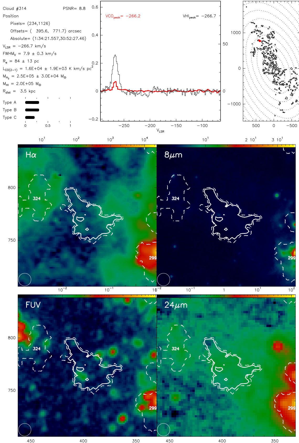
Fig. B.314. Catalogue entry for cloud 314. See description at the beginning of this appendix.
