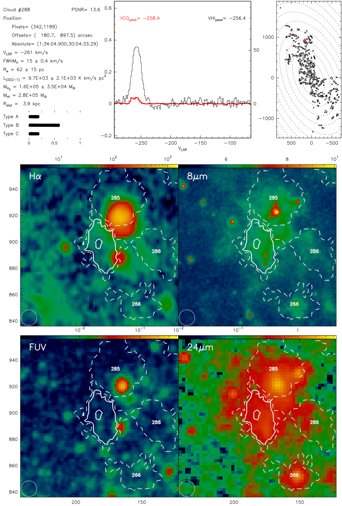
Fig. B.288. Catalogue entry for cloud 288. See description at the beginning of this appendix.
