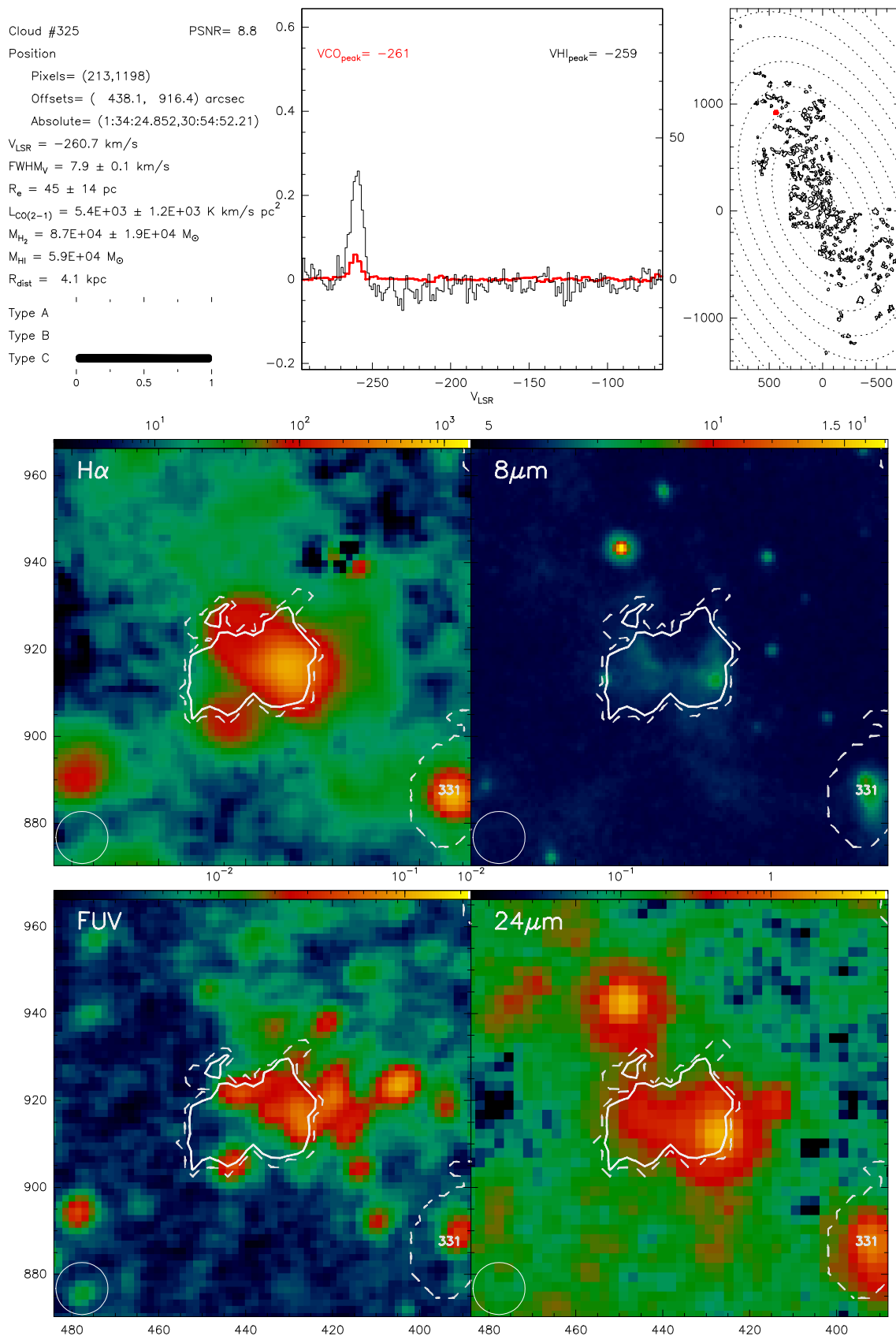
Fig. B.325. Catalogue entry for cloud 325. See description at the beginning of this appendix.
