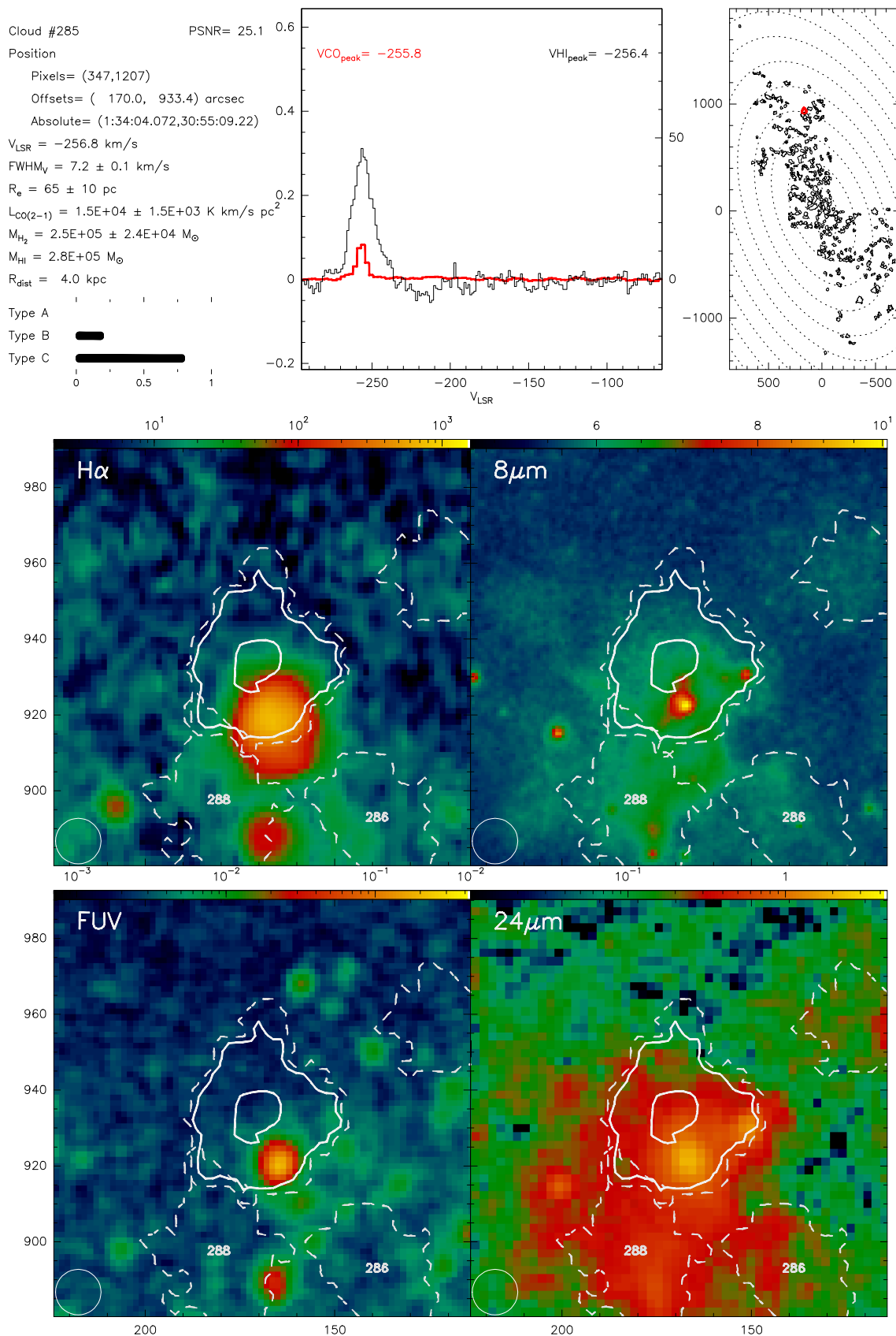
Fig. B.285. Catalogue entry for cloud 285. See description at the beginning of this appendix.
