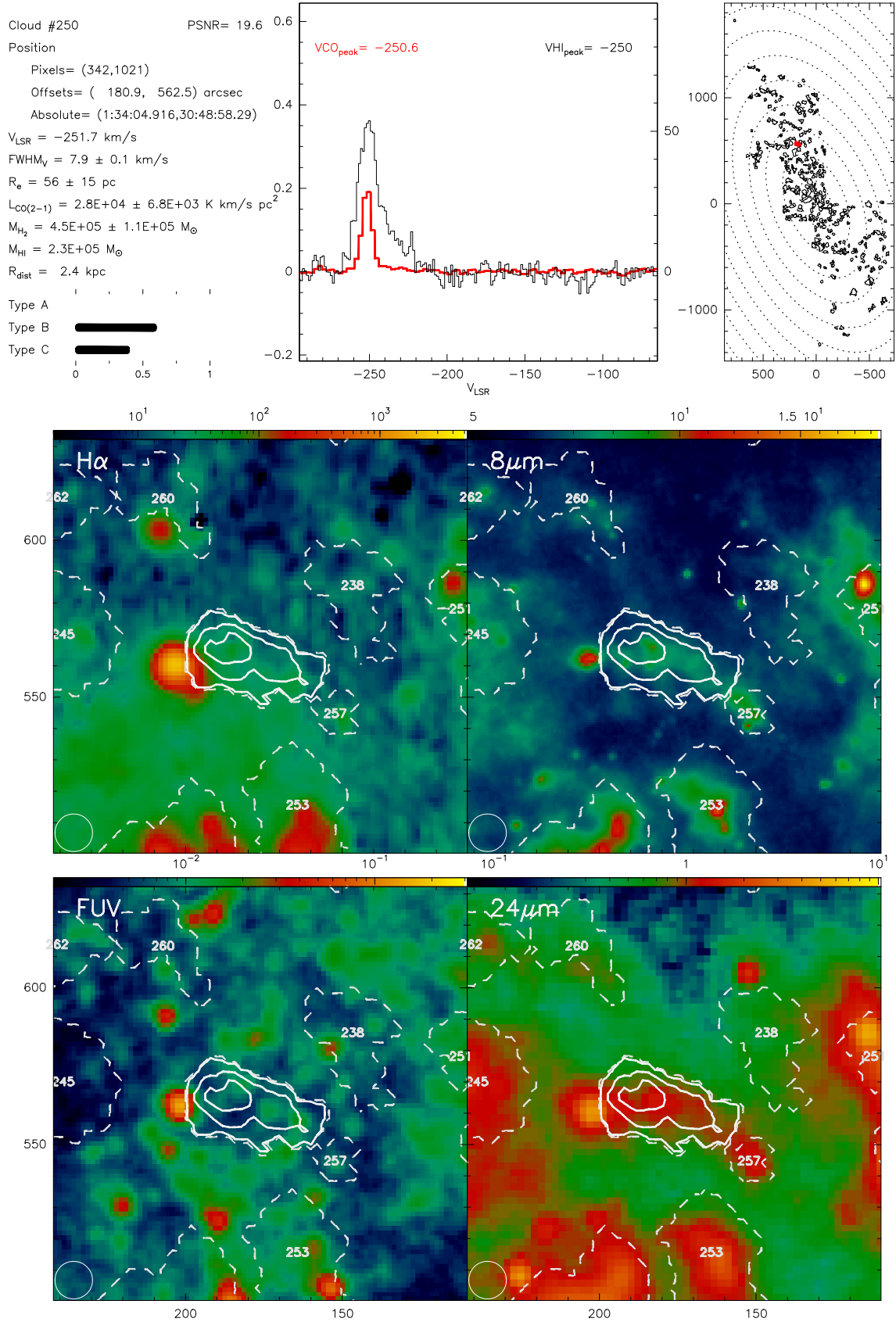
Fig. B.250. Catalogue entry for cloud 250. See description at the beginning of this appendix.
