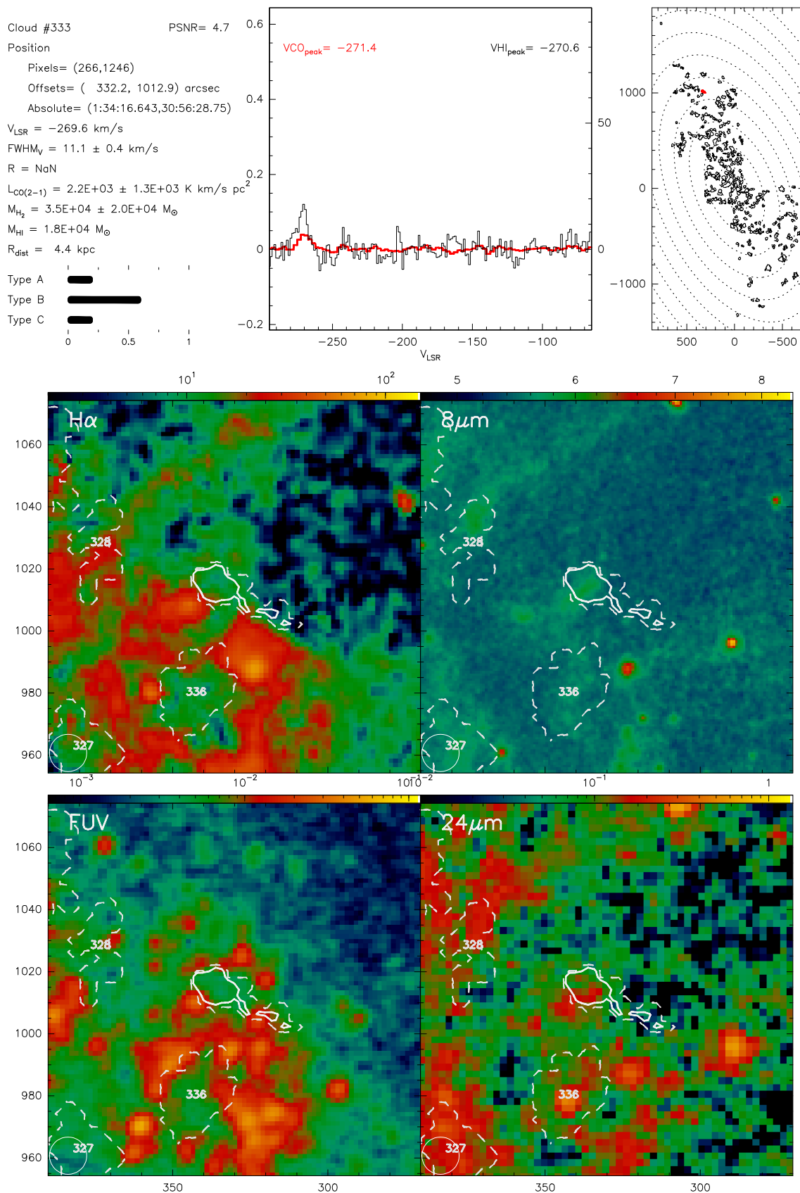
Fig. B.333. Catalogue entry for cloud 333. See description at the beginning of this appendix.
