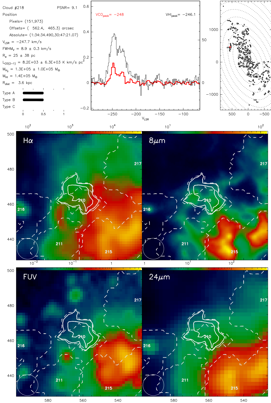
Fig. B.218. Catalogue entry for cloud 218. See description at the beginning of this appendix.
