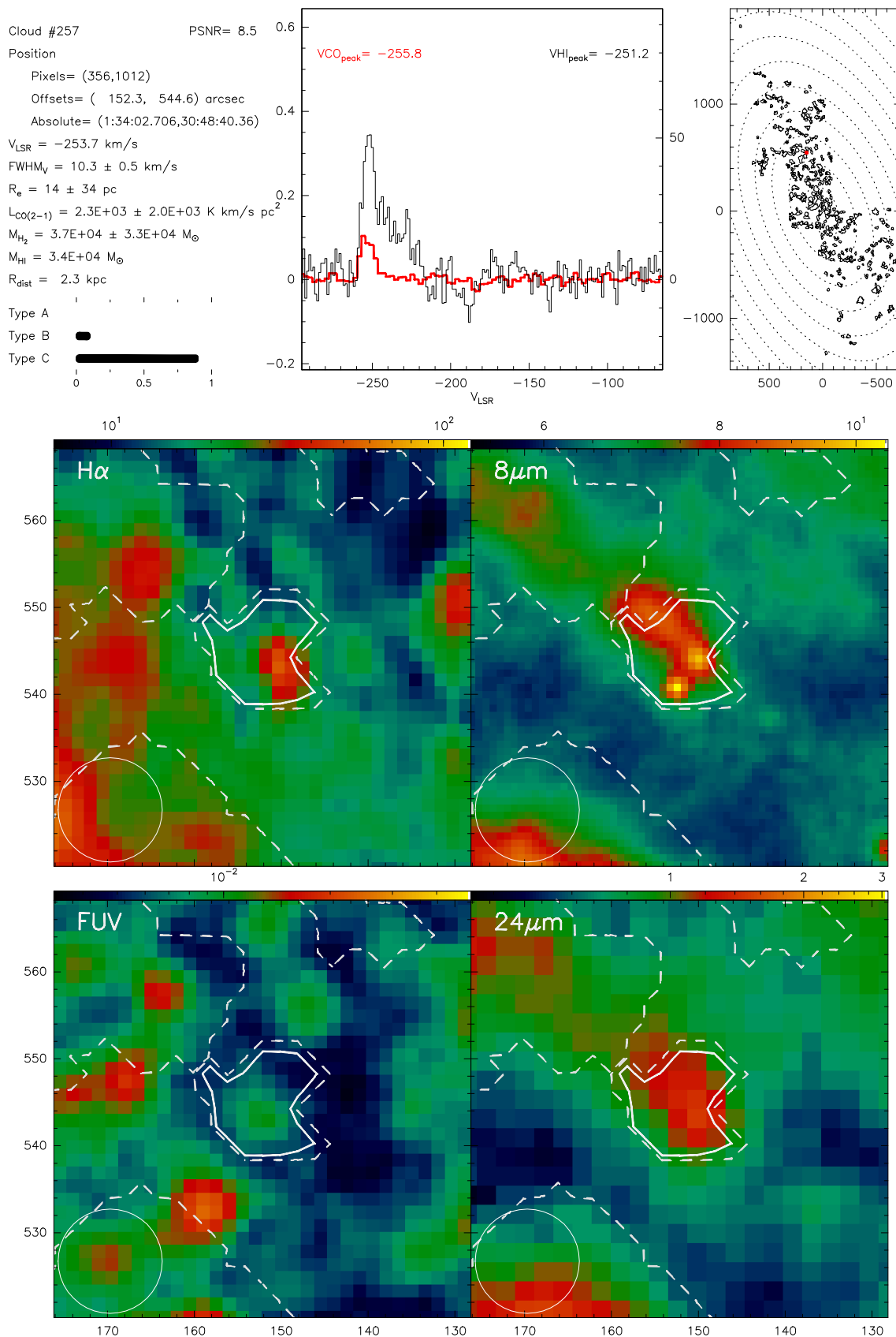
Fig. B.257. Catalogue entry for cloud 257. See description at the beginning of this appendix.
