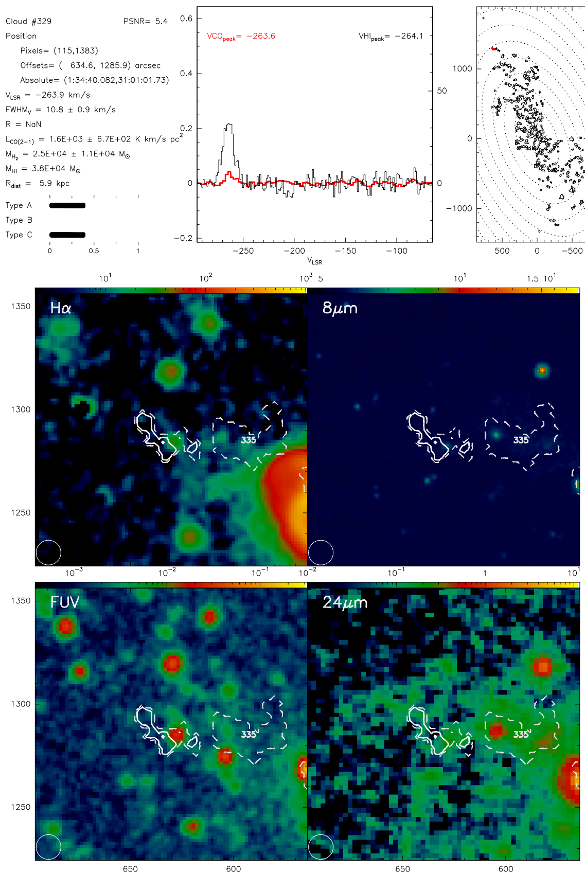
Fig. B.329. Catalogue entry for cloud 329. See description at the beginning of this appendix.
