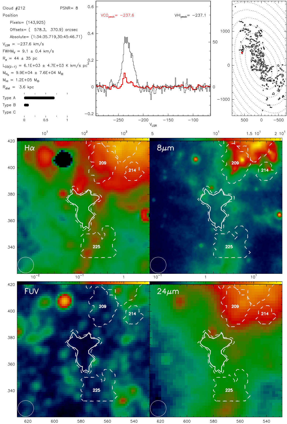
Fig. B.212. Catalogue entry for cloud 212. See description at the beginning of this appendix.
