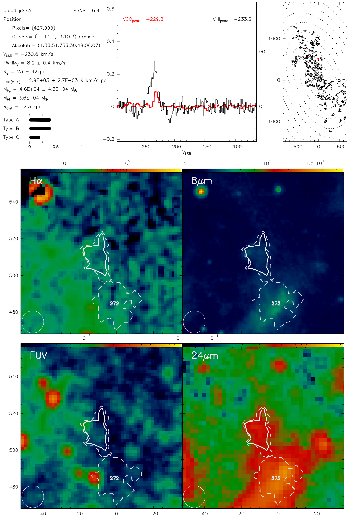
Fig. B.273. Catalogue entry for cloud 273. See description at the beginning of this appendix.
