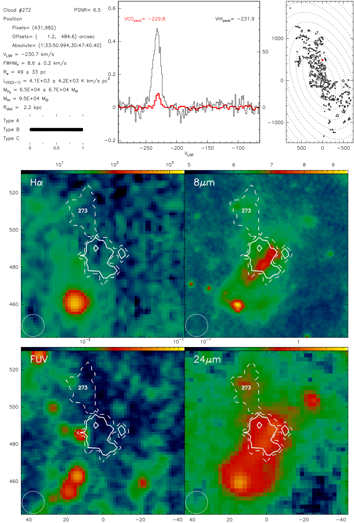
Fig. B.272. Catalogue entry for cloud 272. See description at the beginning of this appendix.
