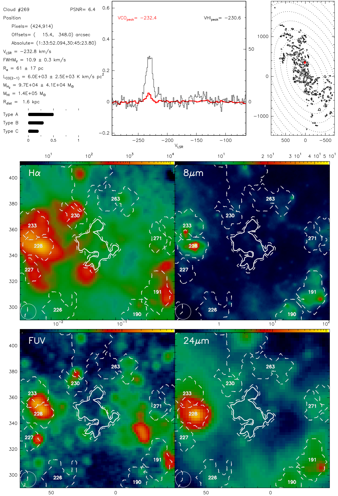
Fig. B.269. Catalogue entry for cloud 269. See description at the beginning of this appendix.
