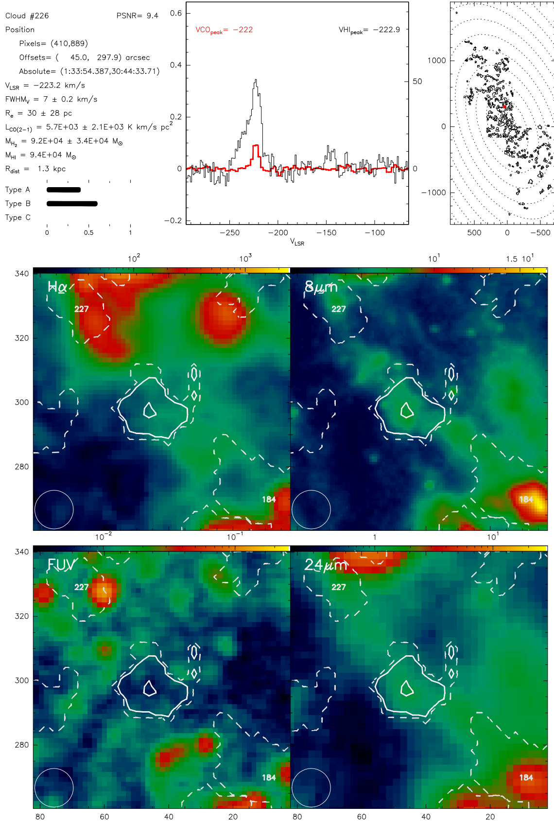
Fig. B.226. Catalogue entry for cloud 226. See description at the beginning of this appendix.
