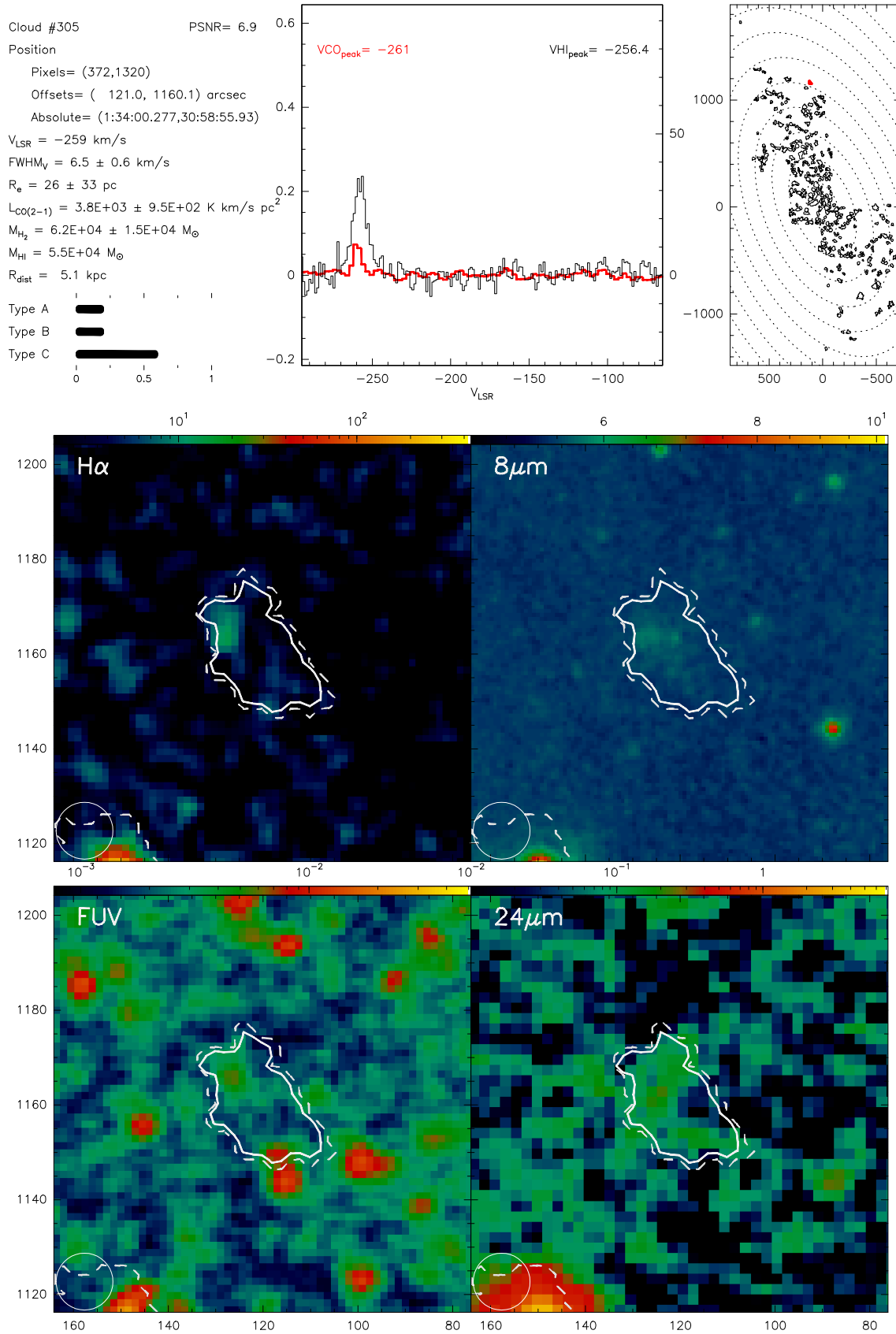
Fig. B.305. Catalogue entry for cloud 305. See description at the beginning of this appendix.
