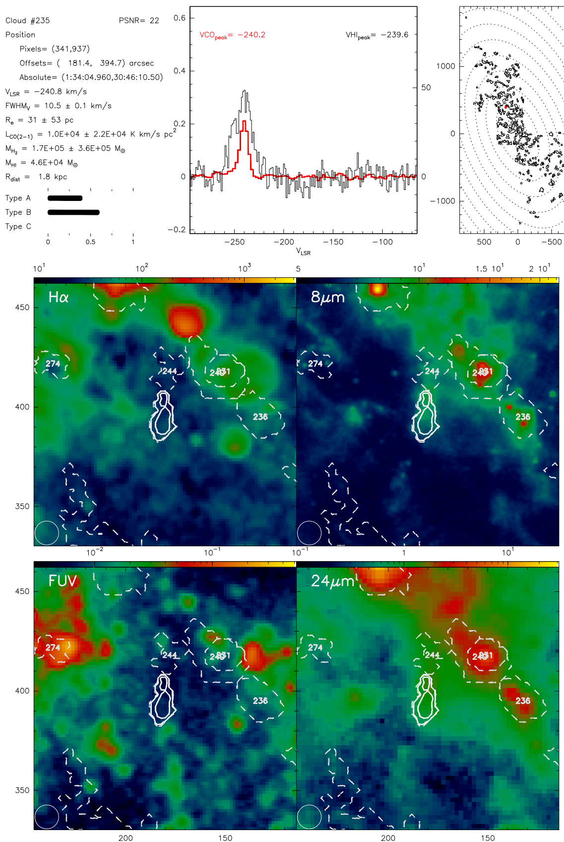
Fig. B.235. Catalogue entry for cloud 235. See description at the beginning of this appendix.
