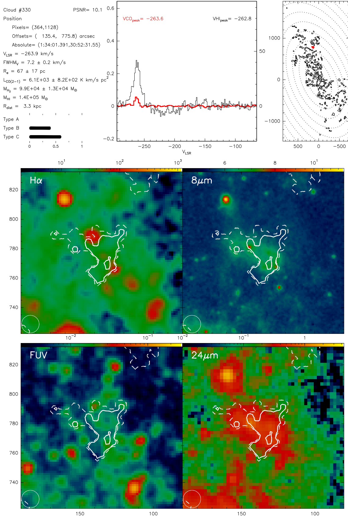
Fig. B.330. Catalogue entry for cloud 330. See description at the beginning of this appendix.
