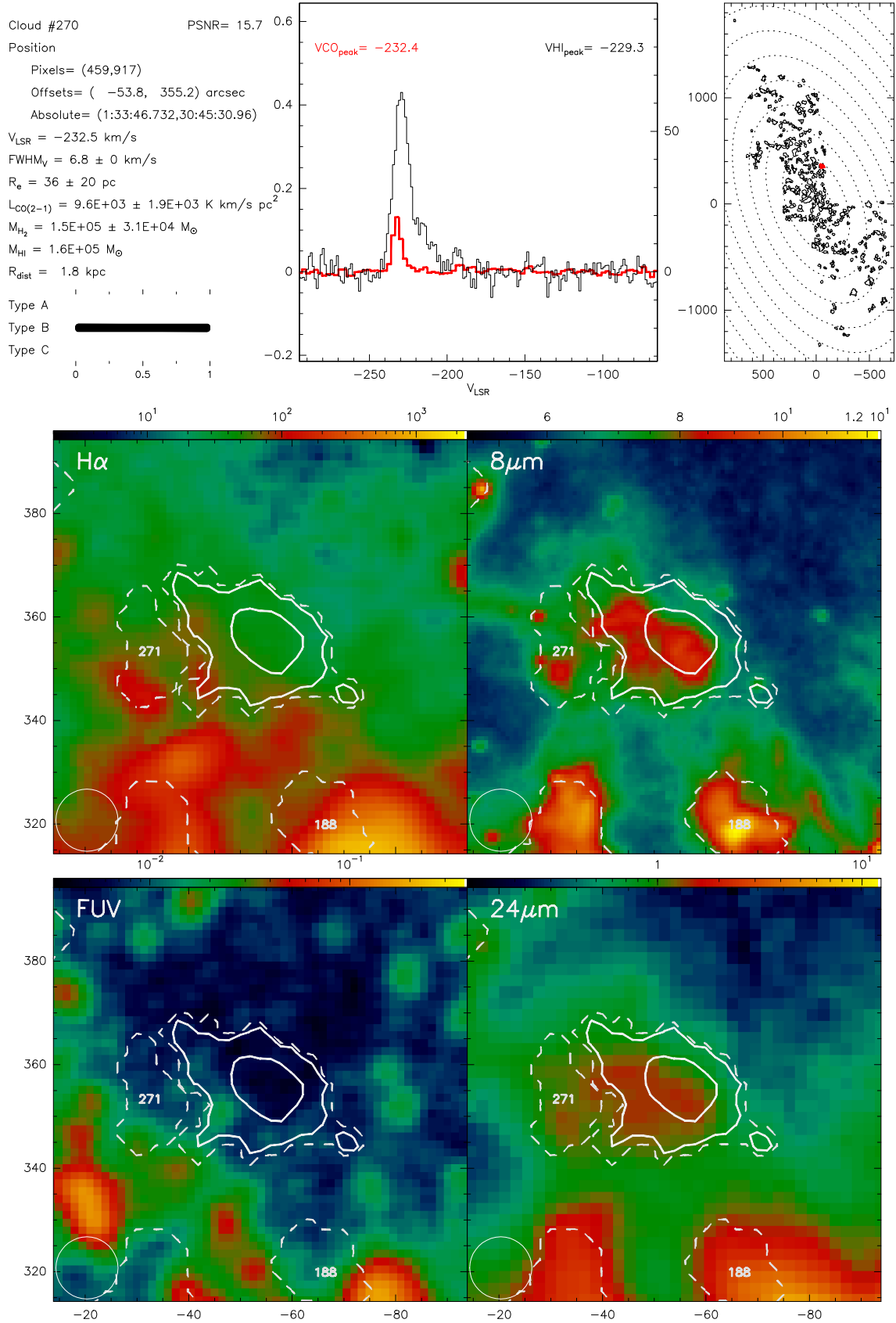
Fig. B.270. Catalogue entry for cloud 270. See description at the beginning of this appendix.
