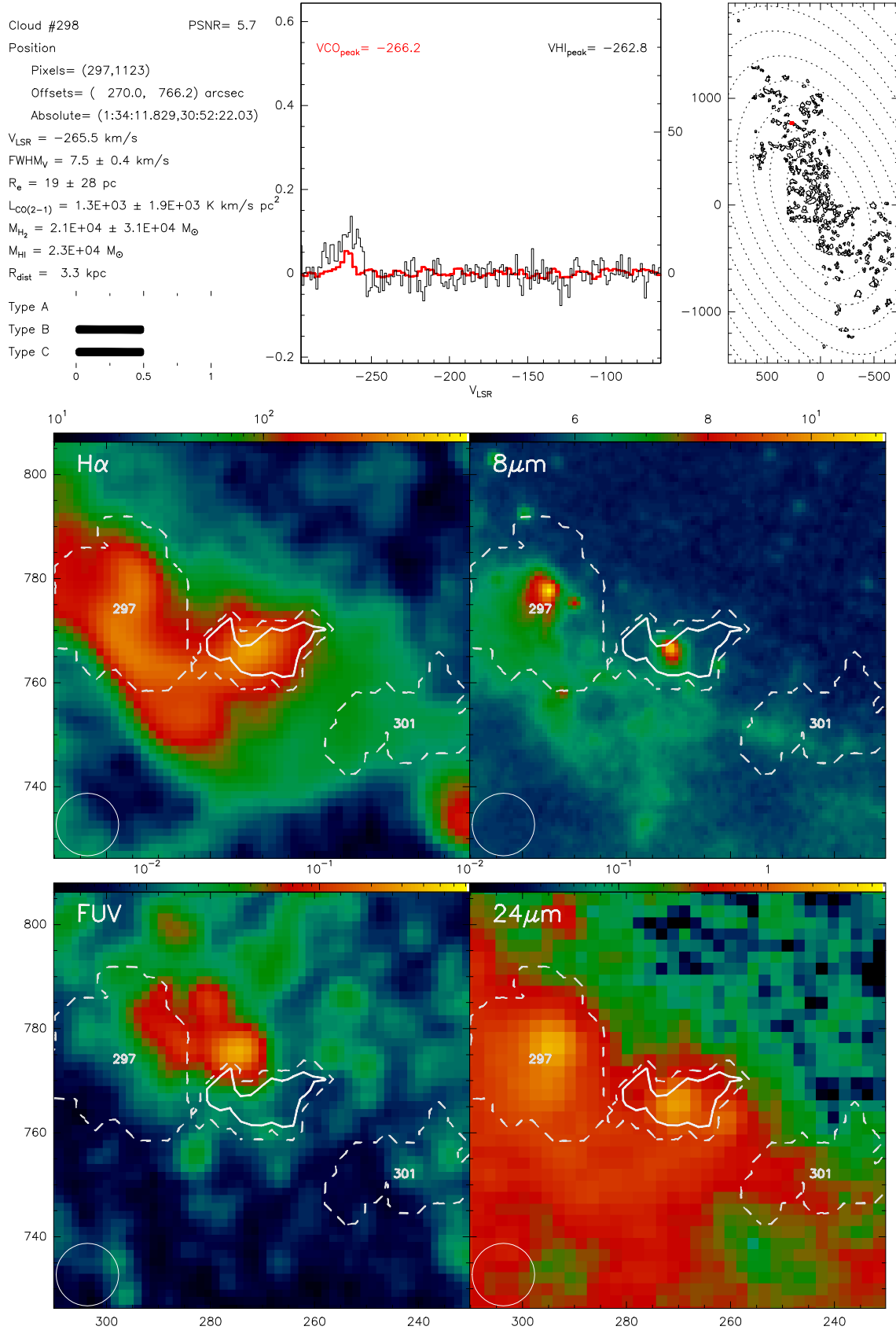
Fig. B.298. Catalogue entry for cloud 298. See description at the beginning of this appendix.
