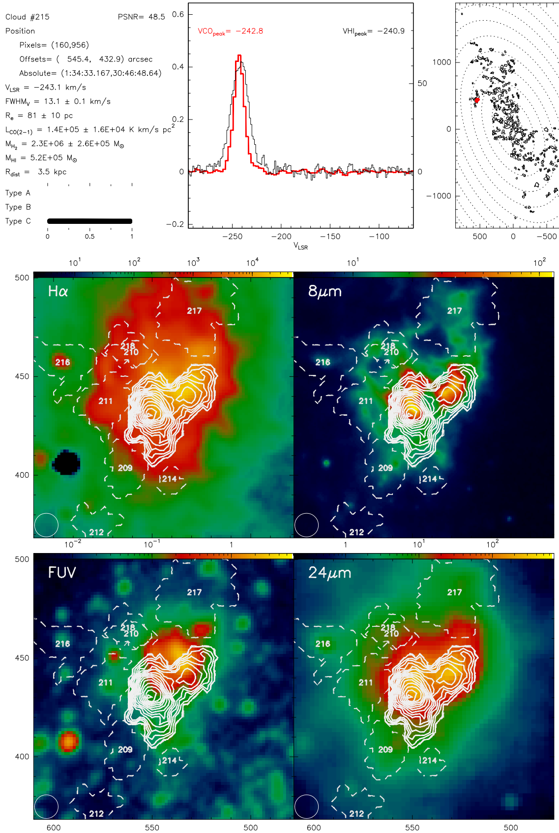
Fig. B.215. Catalogue entry for cloud 215. See description at the beginning of this appendix.
