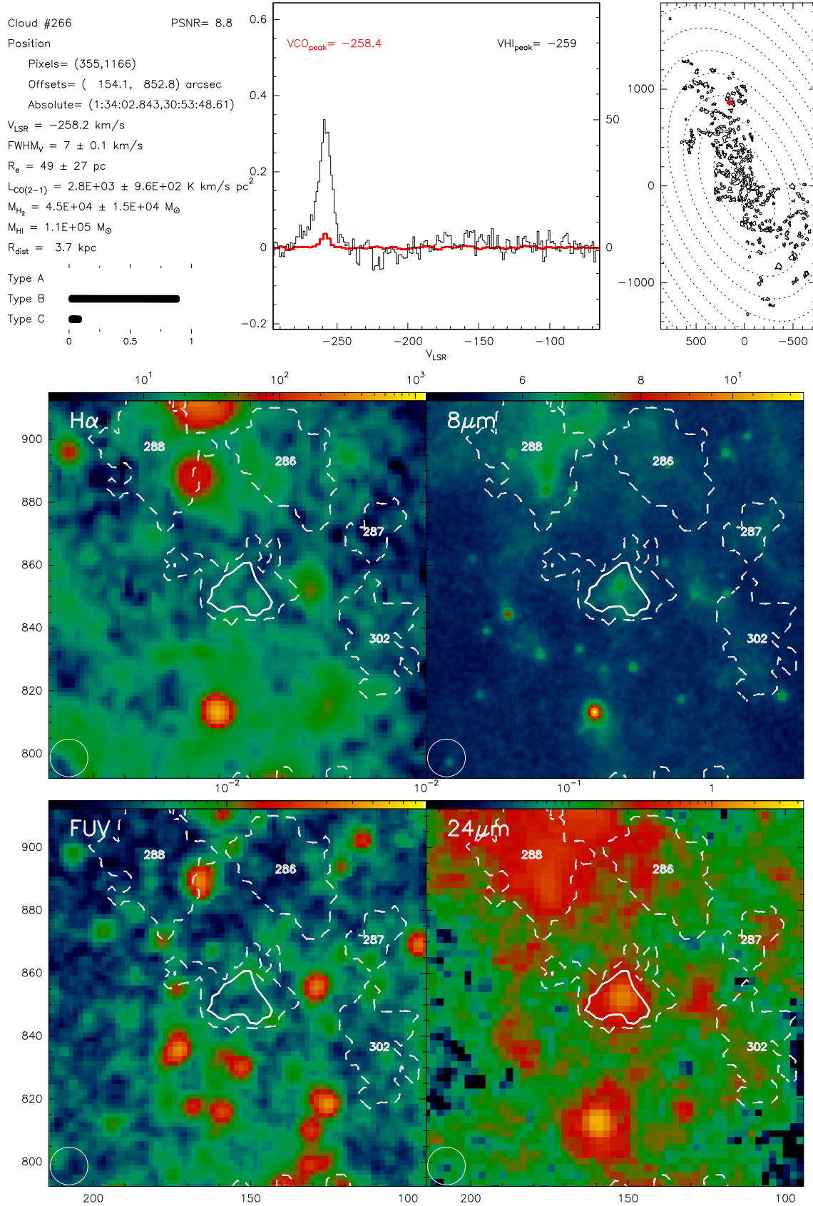
Fig. B.266. Catalogue entry for cloud 266. See description at the beginning of this appendix.
