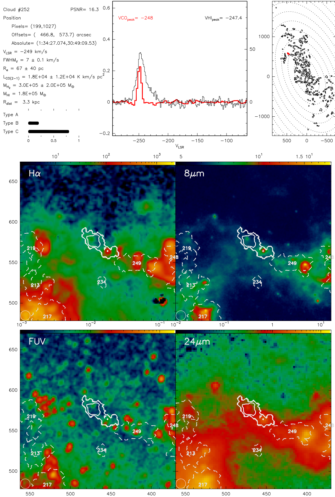
Fig. B.252. Catalogue entry for cloud 252. See description at the beginning of this appendix.
