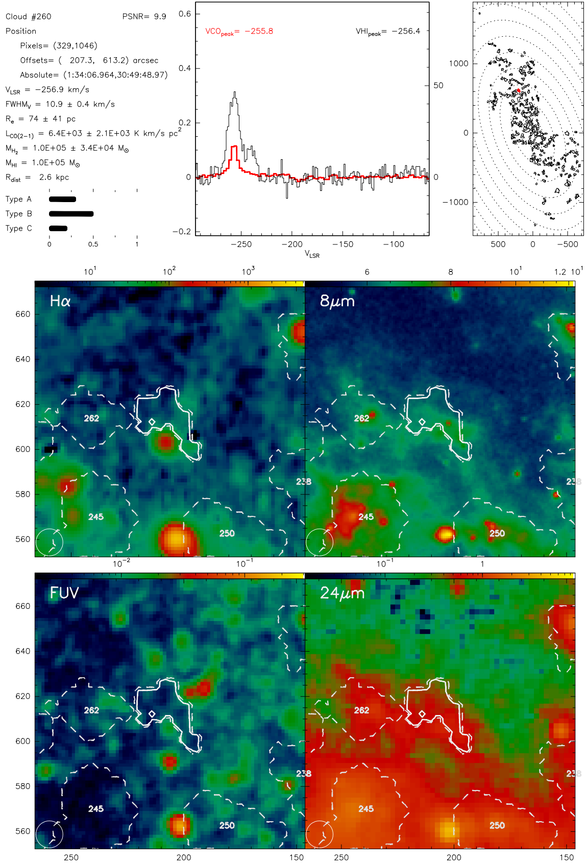
Fig. B.260. Catalogue entry for cloud 260. See description at the beginning of this appendix.
