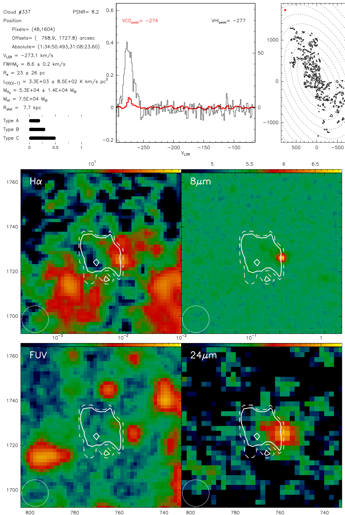
Fig. B.337. Catalogue entry for cloud 337. See description at the beginning of this appendix.
