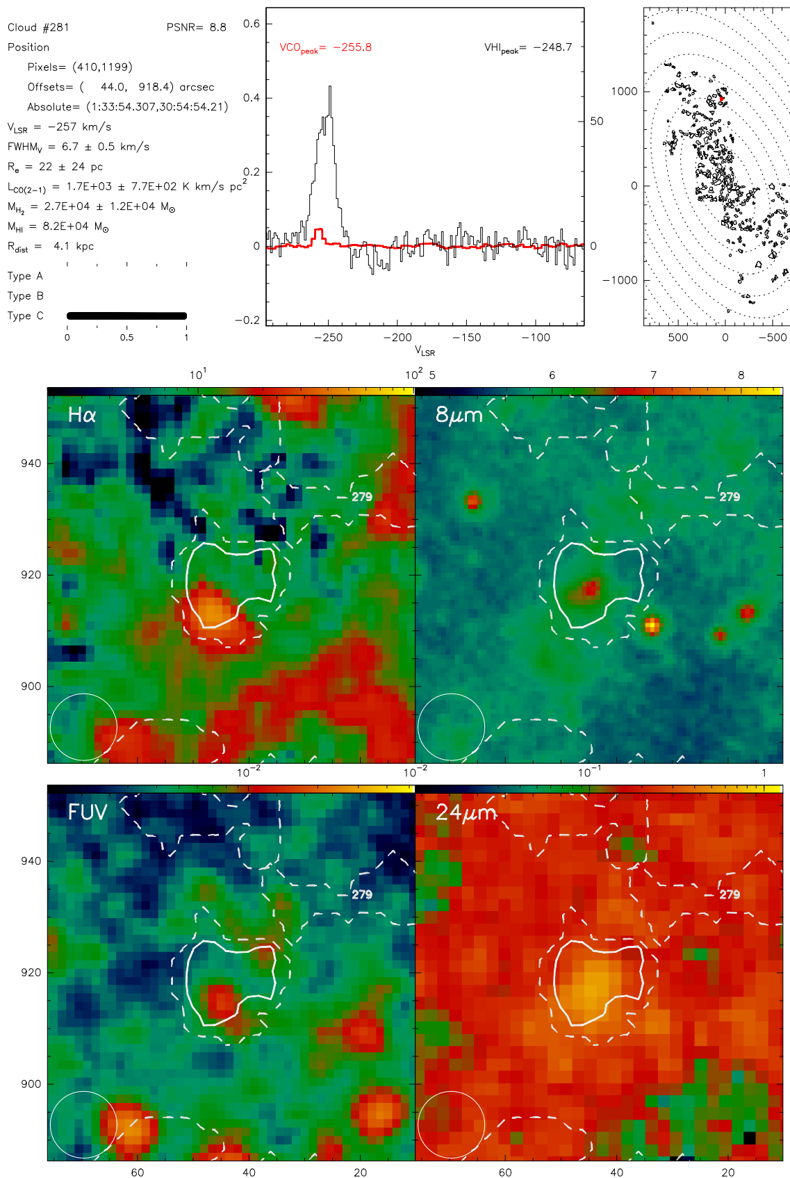
Fig. B.281. Catalogue entry for cloud 281. See description at the beginning of this appendix.
