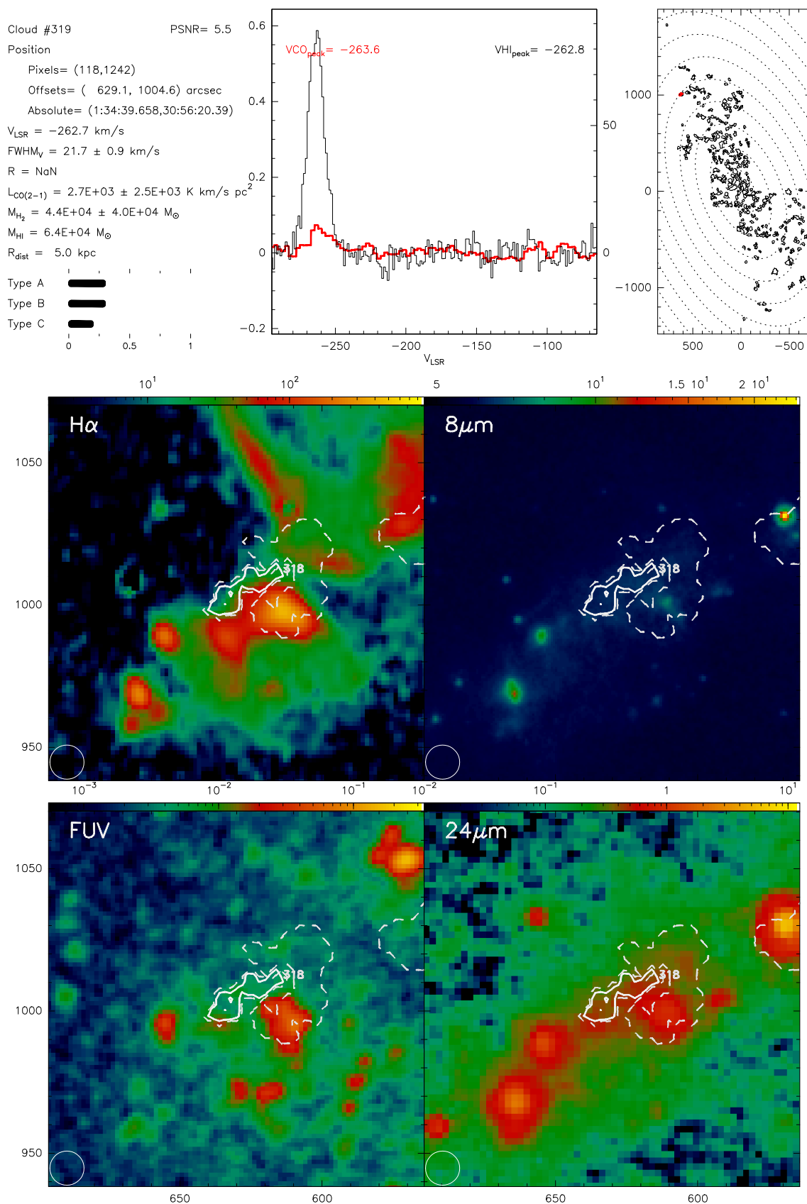
Fig. B.319. Catalogue entry for cloud 319. See description at the beginning of this appendix.
