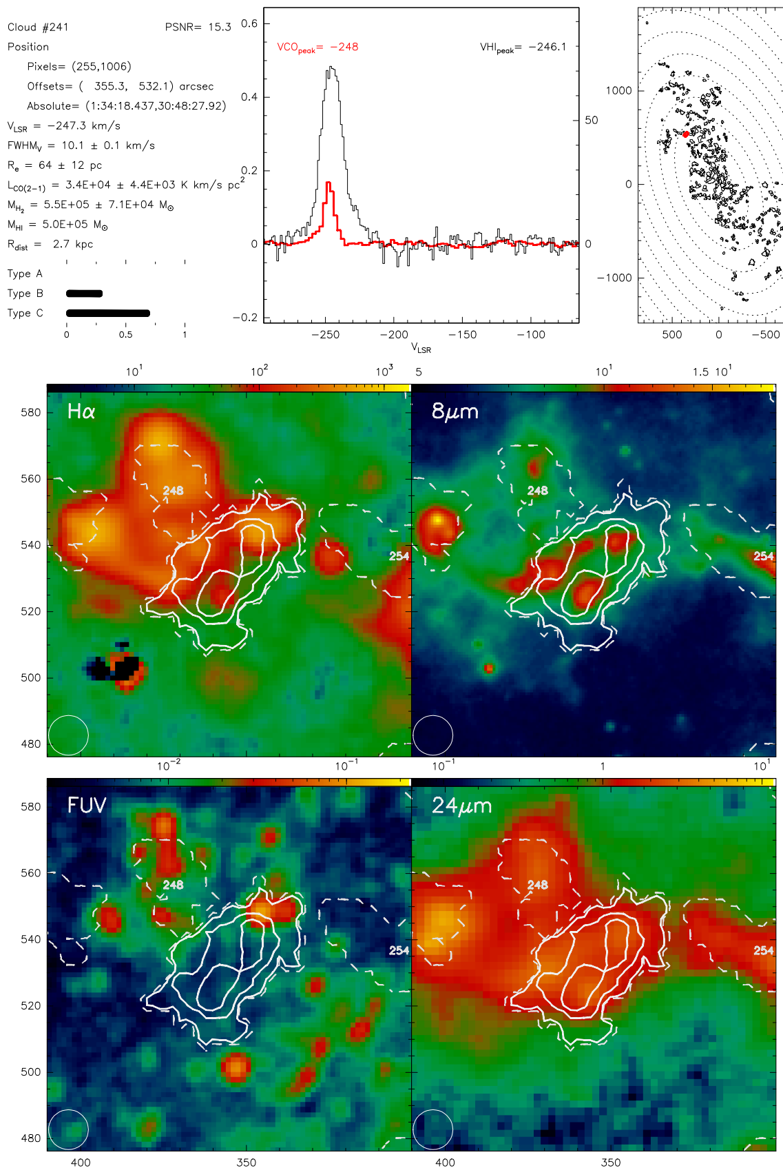
Fig. B.241. Catalogue entry for cloud 241. See description at the beginning of this appendix.
