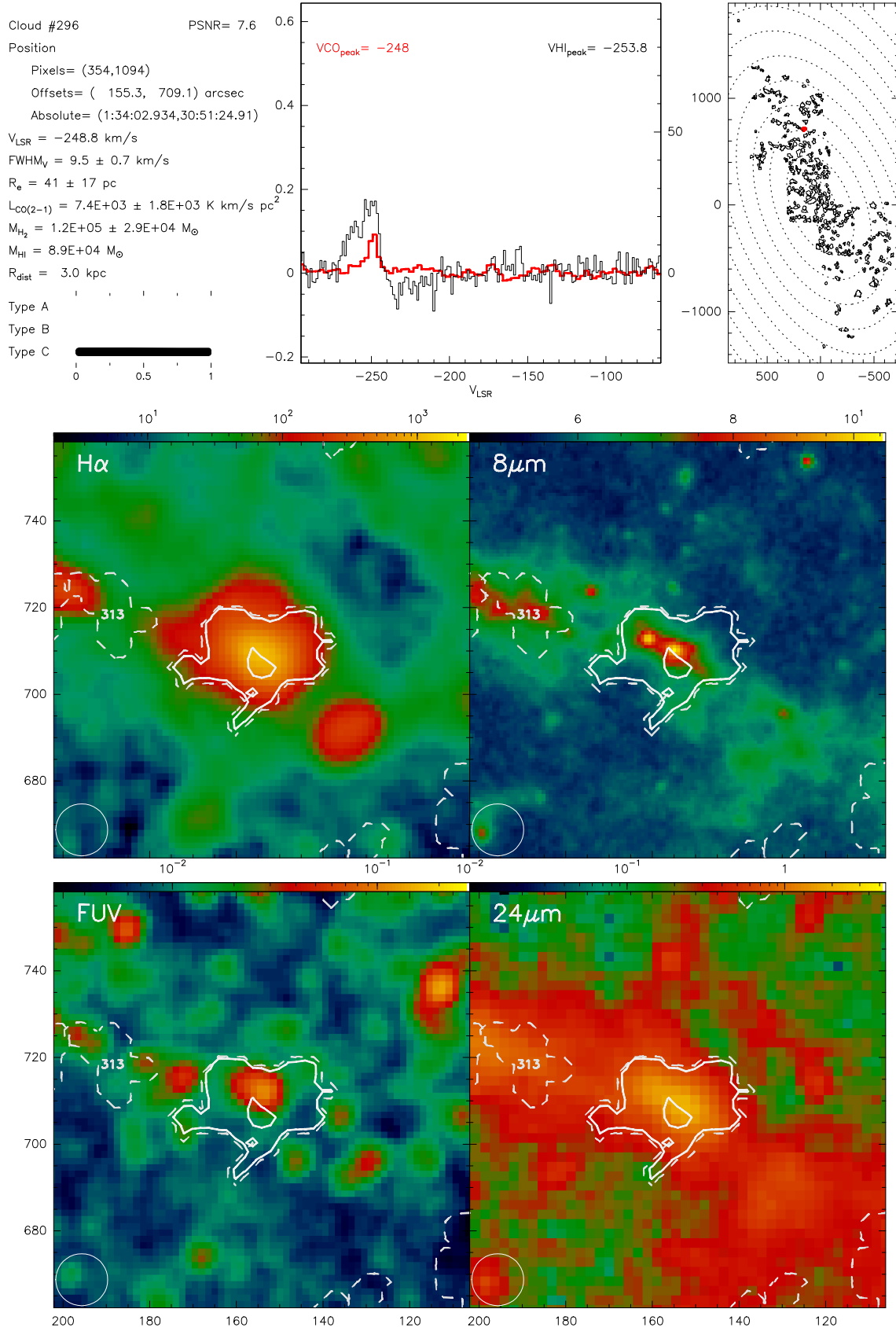
Fig. B.296. Catalogue entry for cloud 296. See description at the beginning of this appendix.
