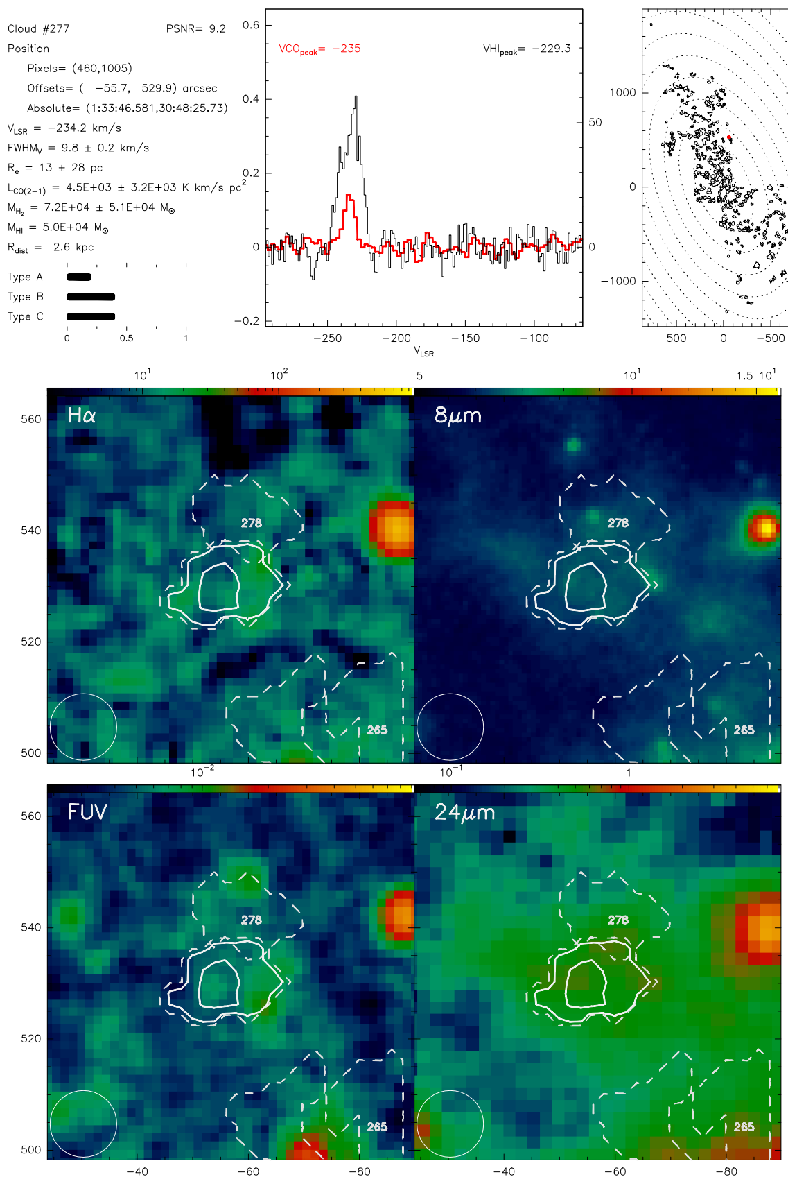
Fig. B.277. Catalogue entry for cloud 277. See description at the beginning of this appendix.
