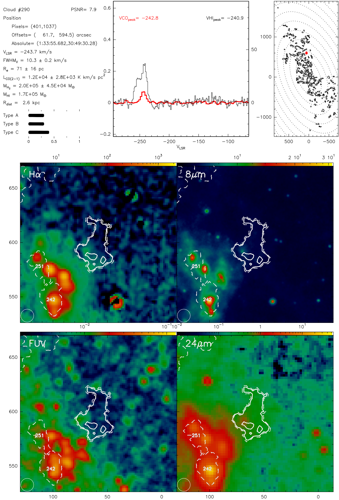
Fig. B.290. Catalogue entry for cloud 290. See description at the beginning of this appendix.
