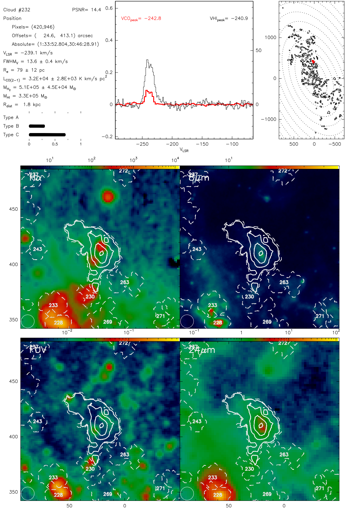
Fig. B.232. Catalogue entry for cloud 232. See description at the beginning of this appendix.
