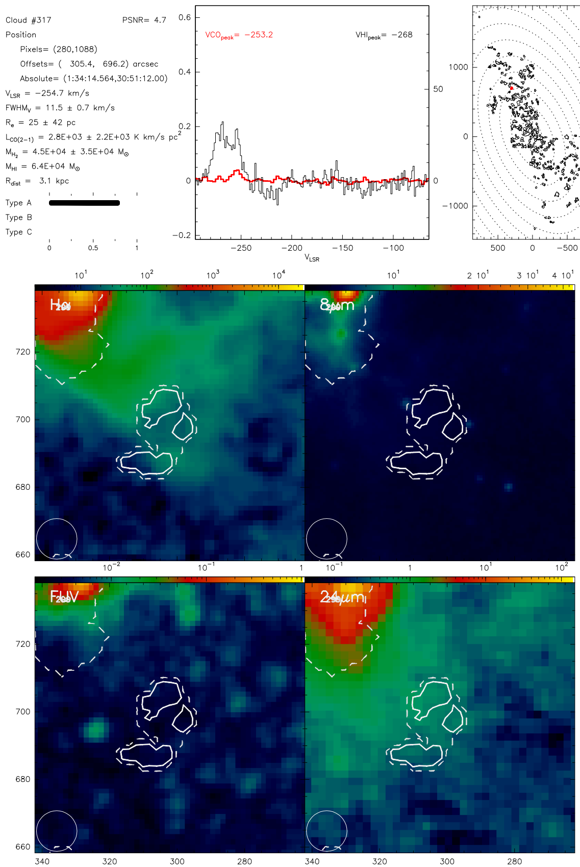
Fig. B.317. Catalogue entry for cloud 317. See description at the beginning of this appendix.
