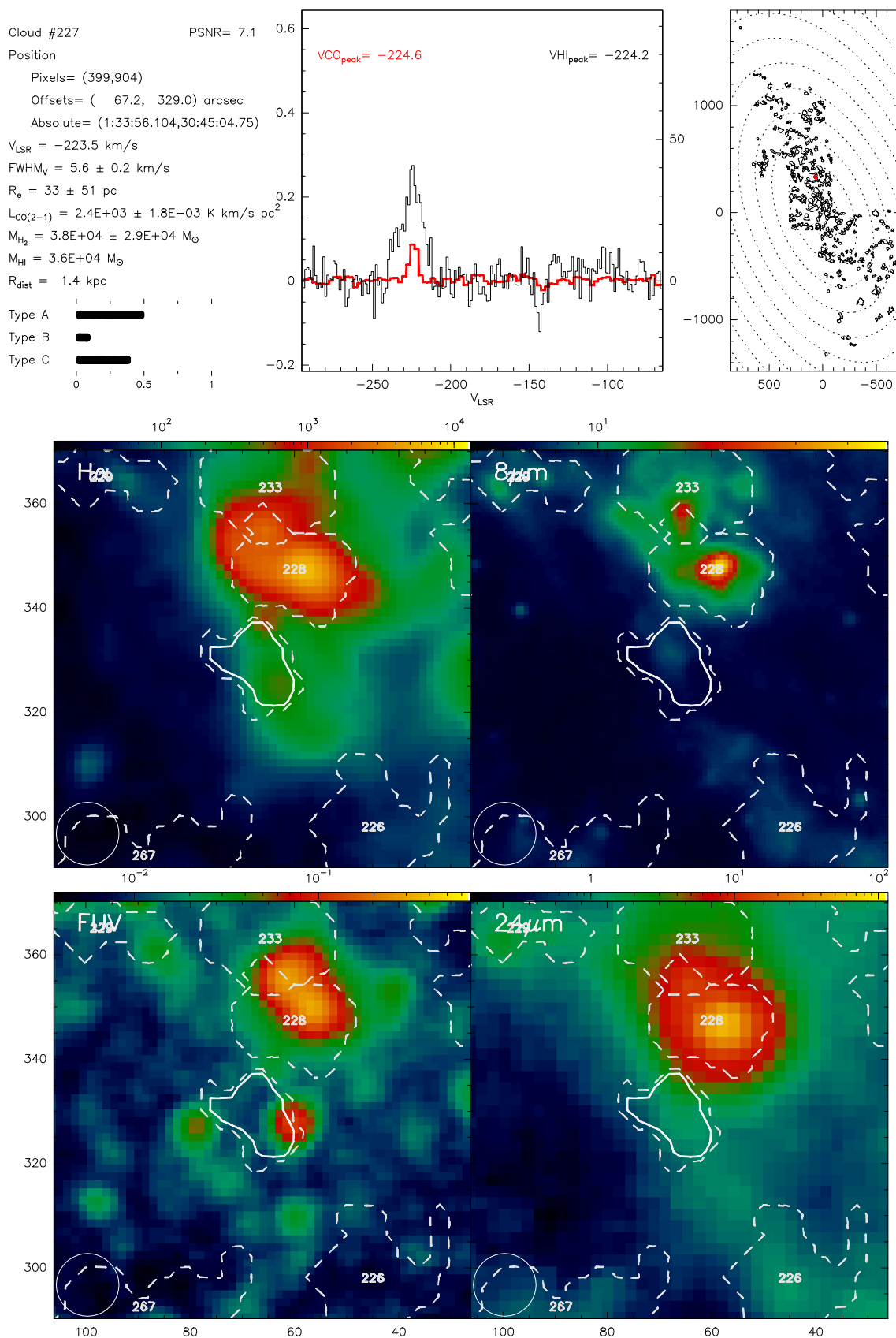
Fig. B.227. Catalogue entry for cloud 227. See description at the beginning of this appendix.
