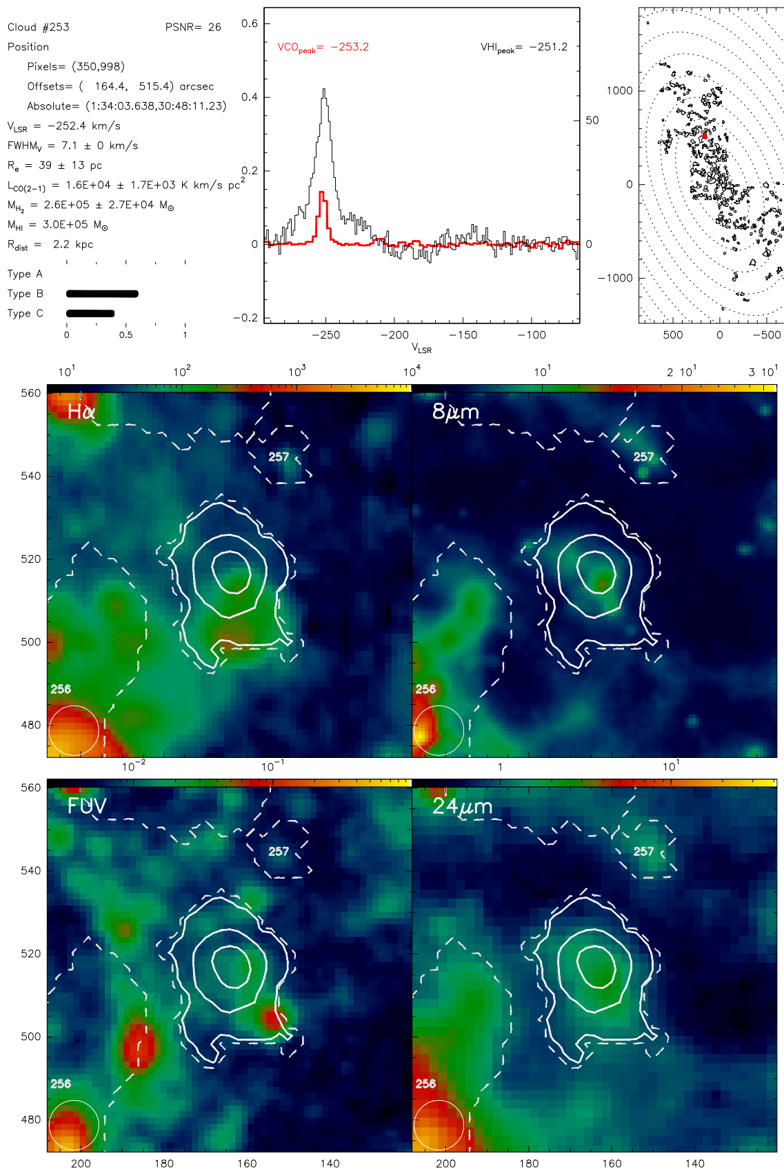
Fig. B.253. Catalogue entry for cloud 253. See description at the beginning of this appendix.
