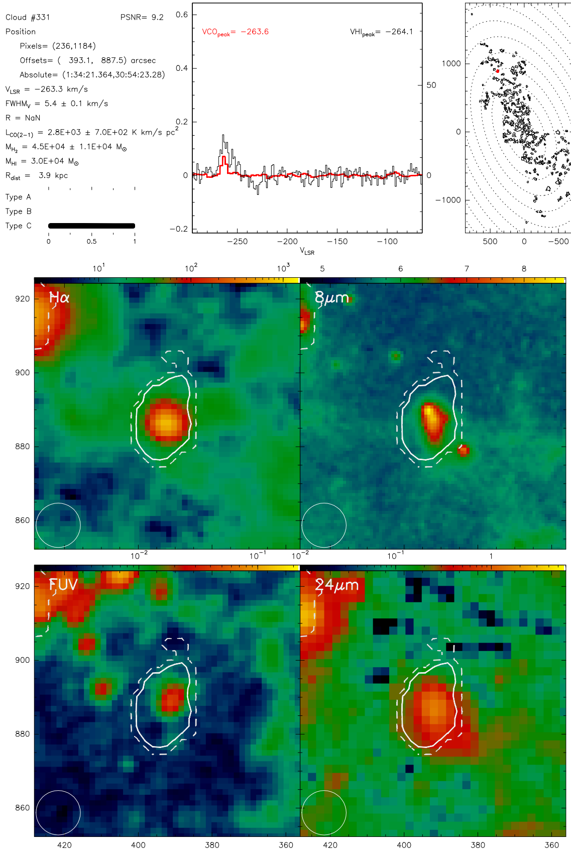
Fig. B.331. Catalogue entry for cloud 331. See description at the beginning of this appendix.
