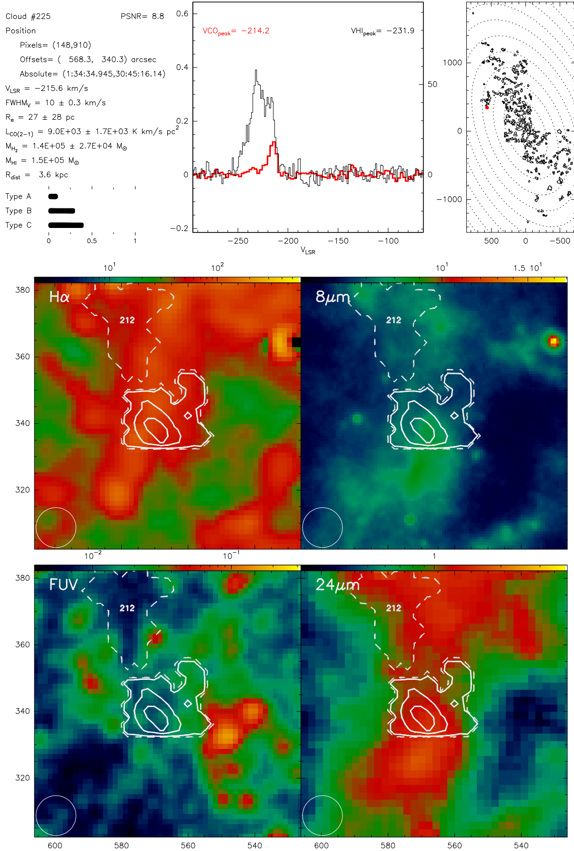
Fig. B.225. Catalogue entry for cloud 225. See description at the beginning of this appendix.
