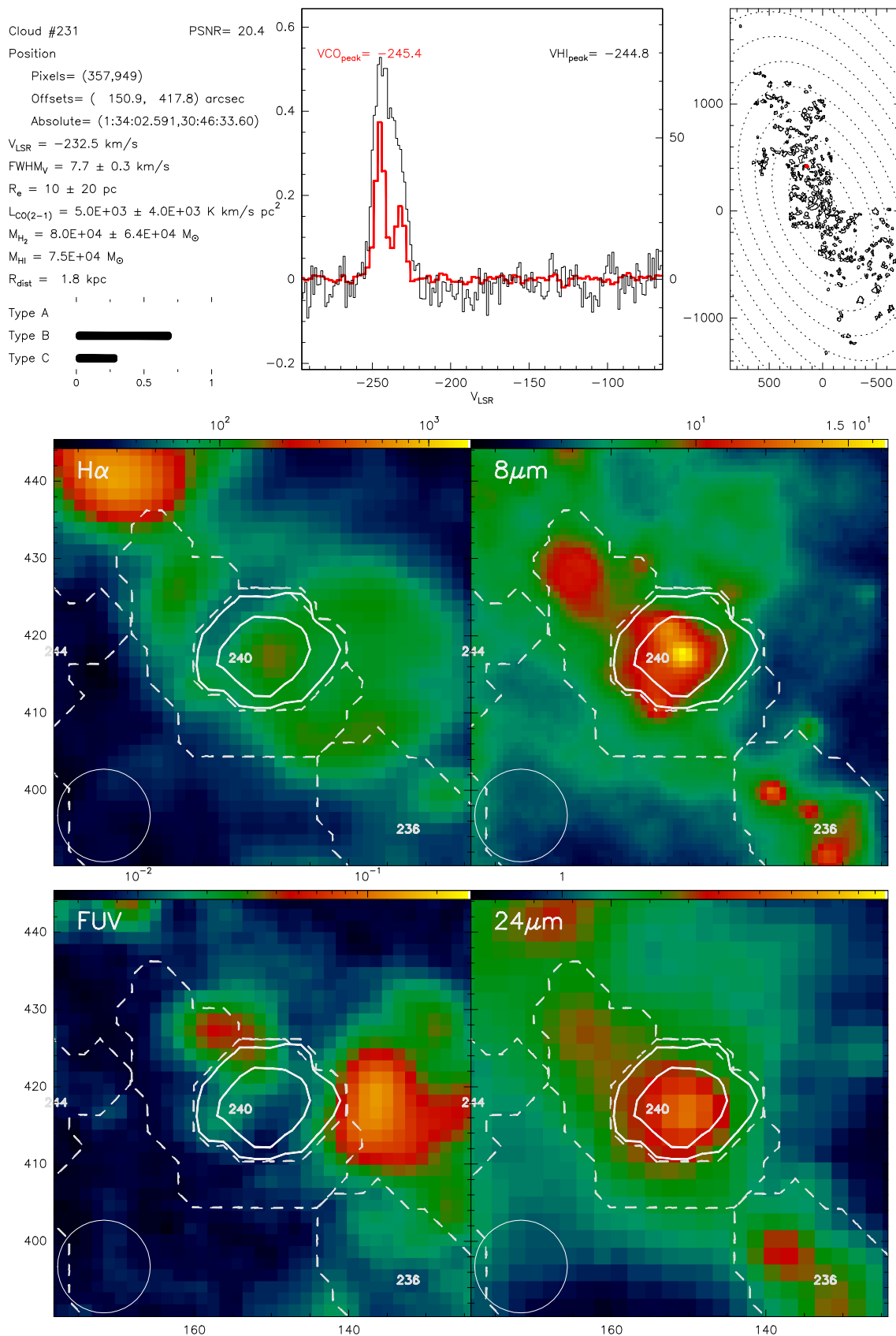
Fig. B.231. Catalogue entry for cloud 231. See description at the beginning of this appendix.
