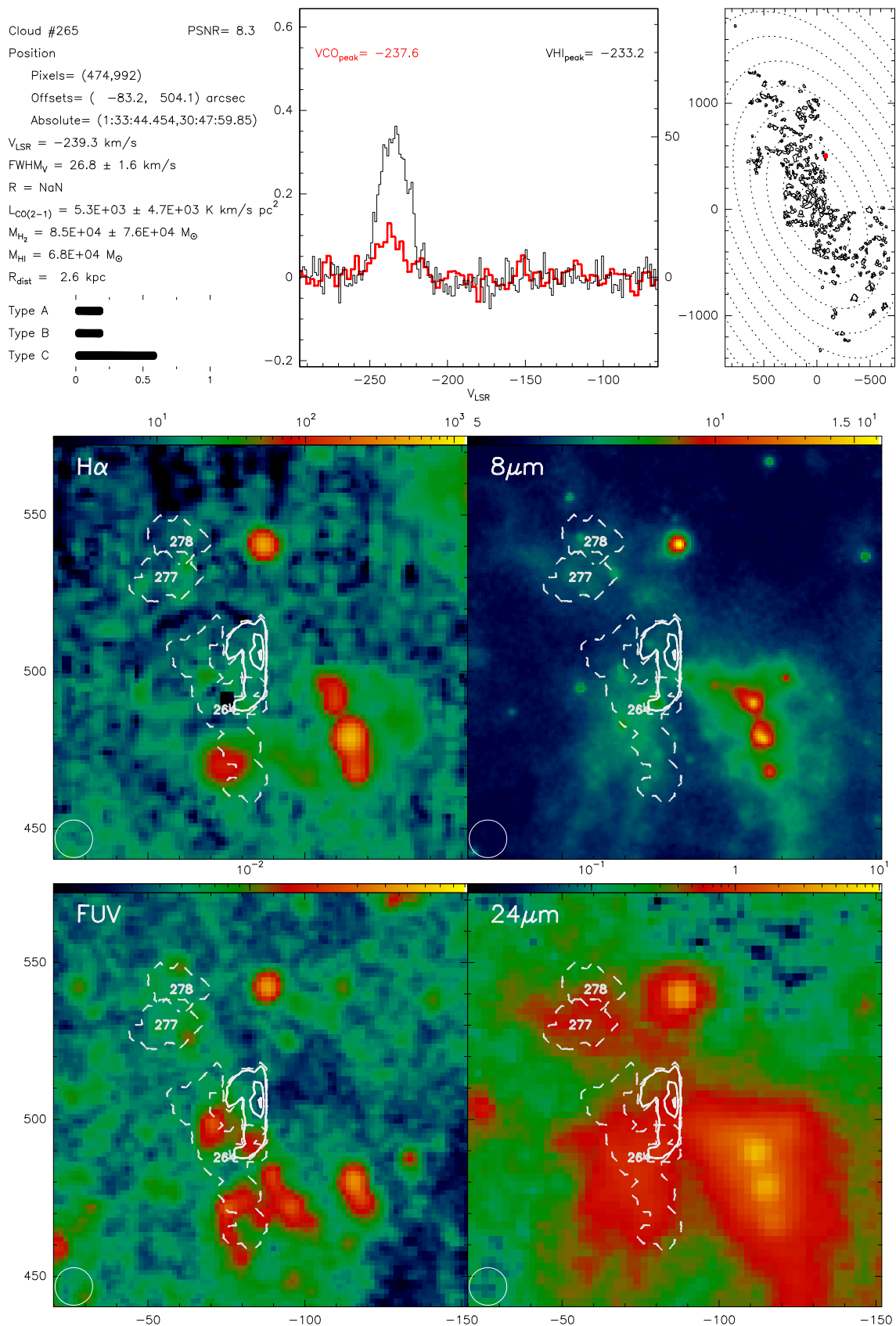
Fig. B.265. Catalogue entry for cloud 265. See description at the beginning of this appendix.
