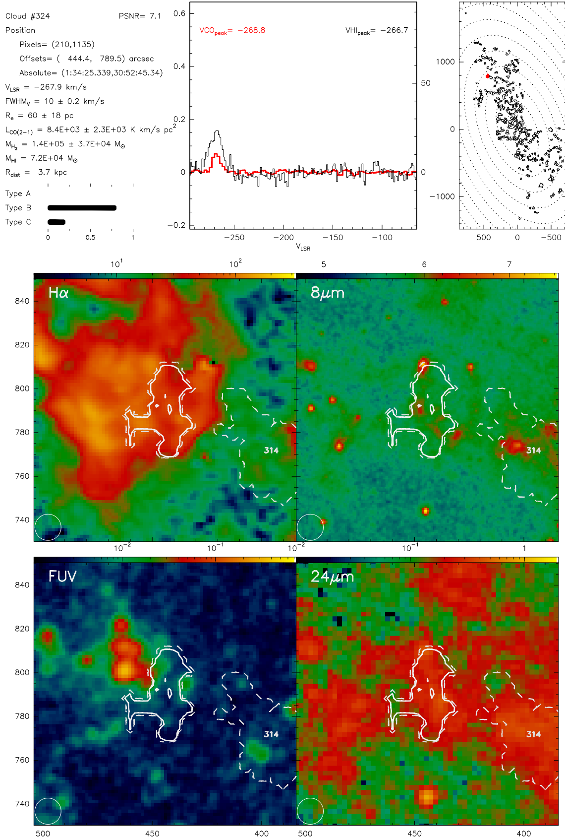
Fig. B.324. Catalogue entry for cloud 324. See description at the beginning of this appendix.
