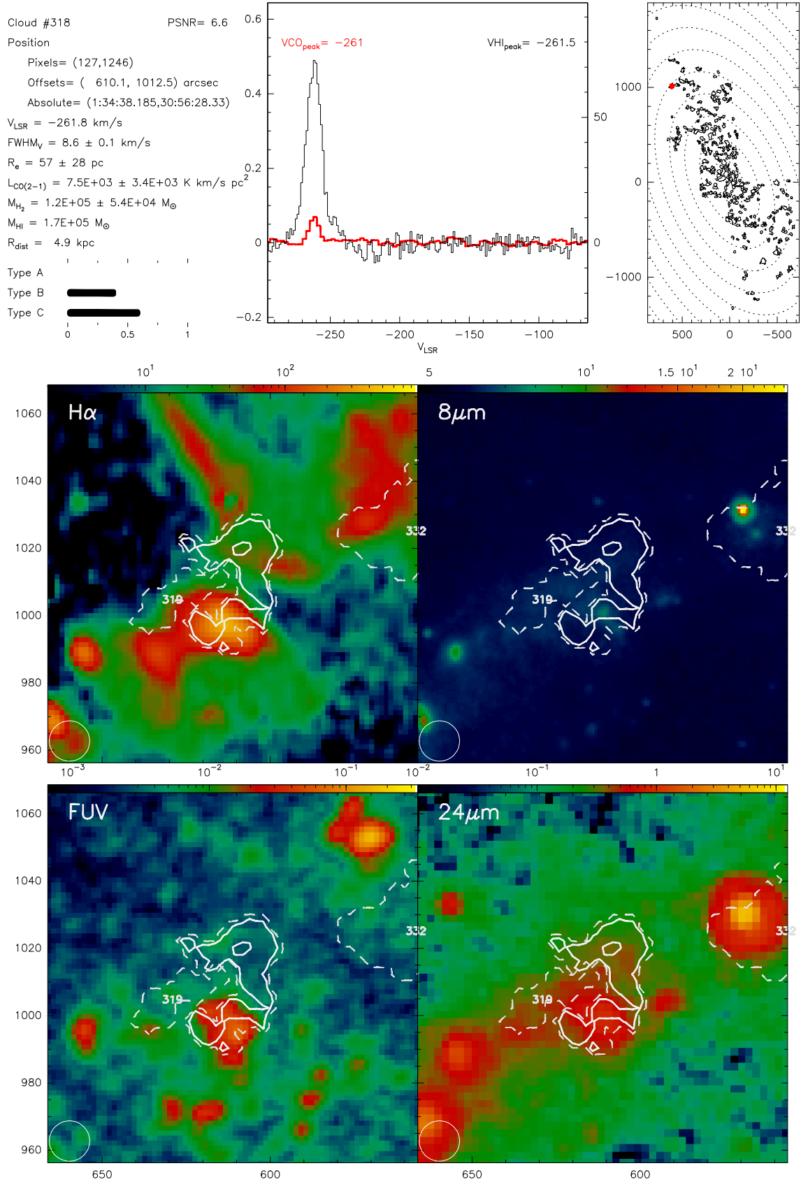
Fig. B.318. Catalogue entry for cloud 318. See description at the beginning of this appendix.
