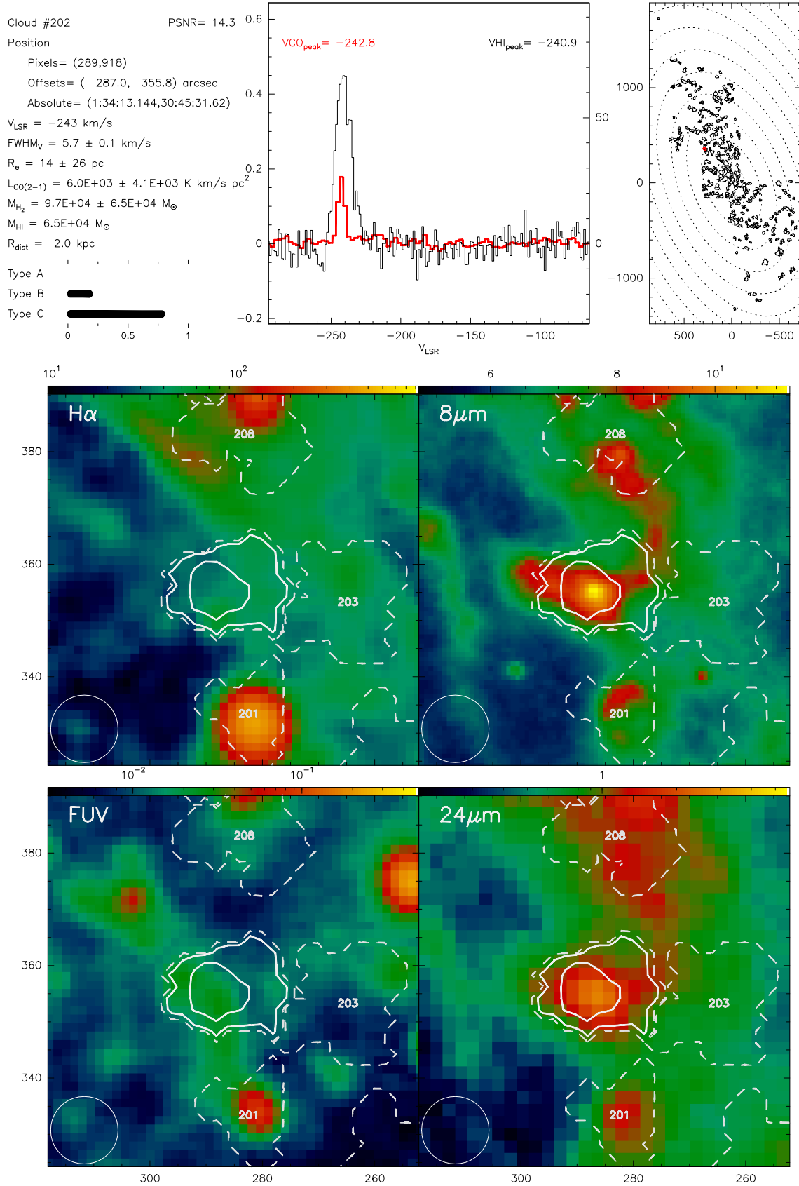
Fig. B.202. Catalogue entry for cloud 202. See description at the beginning of this appendix.
