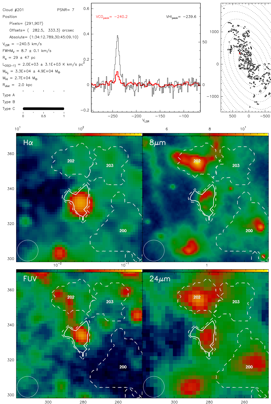
Fig. B.201. Catalogue entry for cloud 201. See description at the beginning of this appendix.
