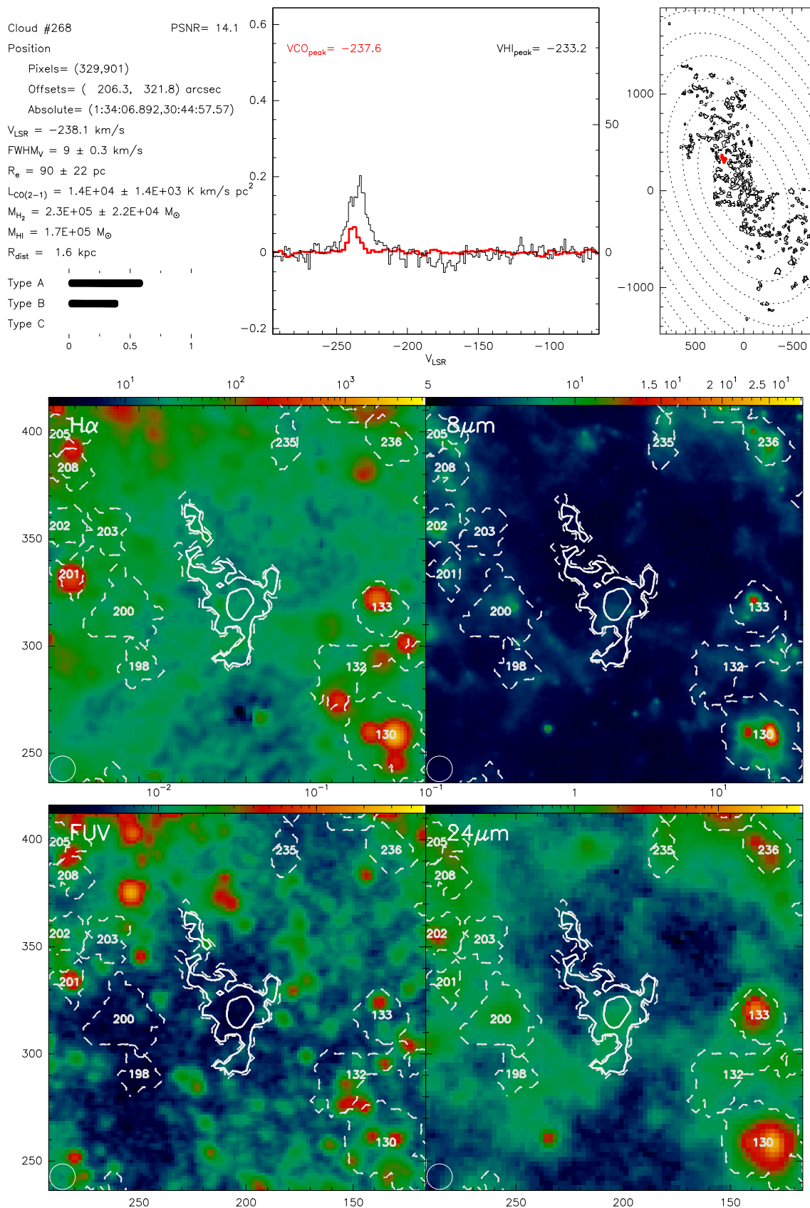
Fig. B.268. Catalogue entry for cloud 268. See description at the beginning of this appendix.
