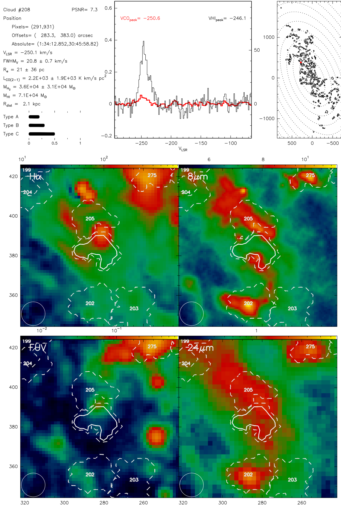
Fig. B.208. Catalogue entry for cloud 208. See description at the beginning of this appendix.
