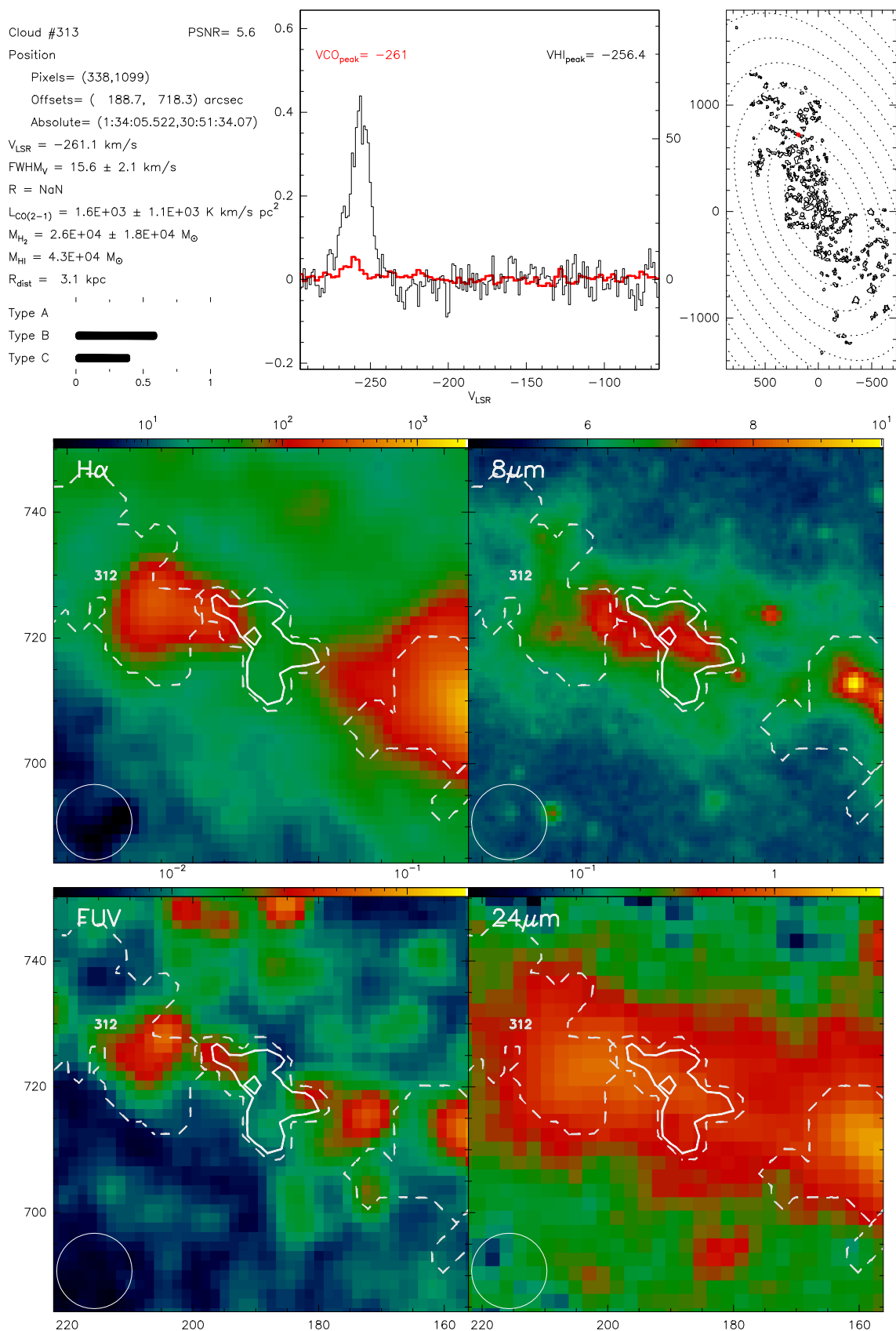
Fig. B.313. Catalogue entry for cloud 313. See description at the beginning of this appendix.
