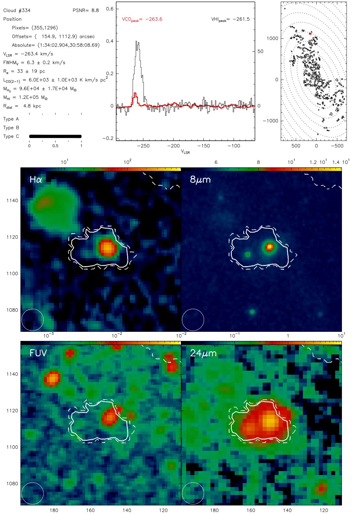
Fig. B.334. Catalogue entry for cloud 334. See description at the beginning of this appendix.
