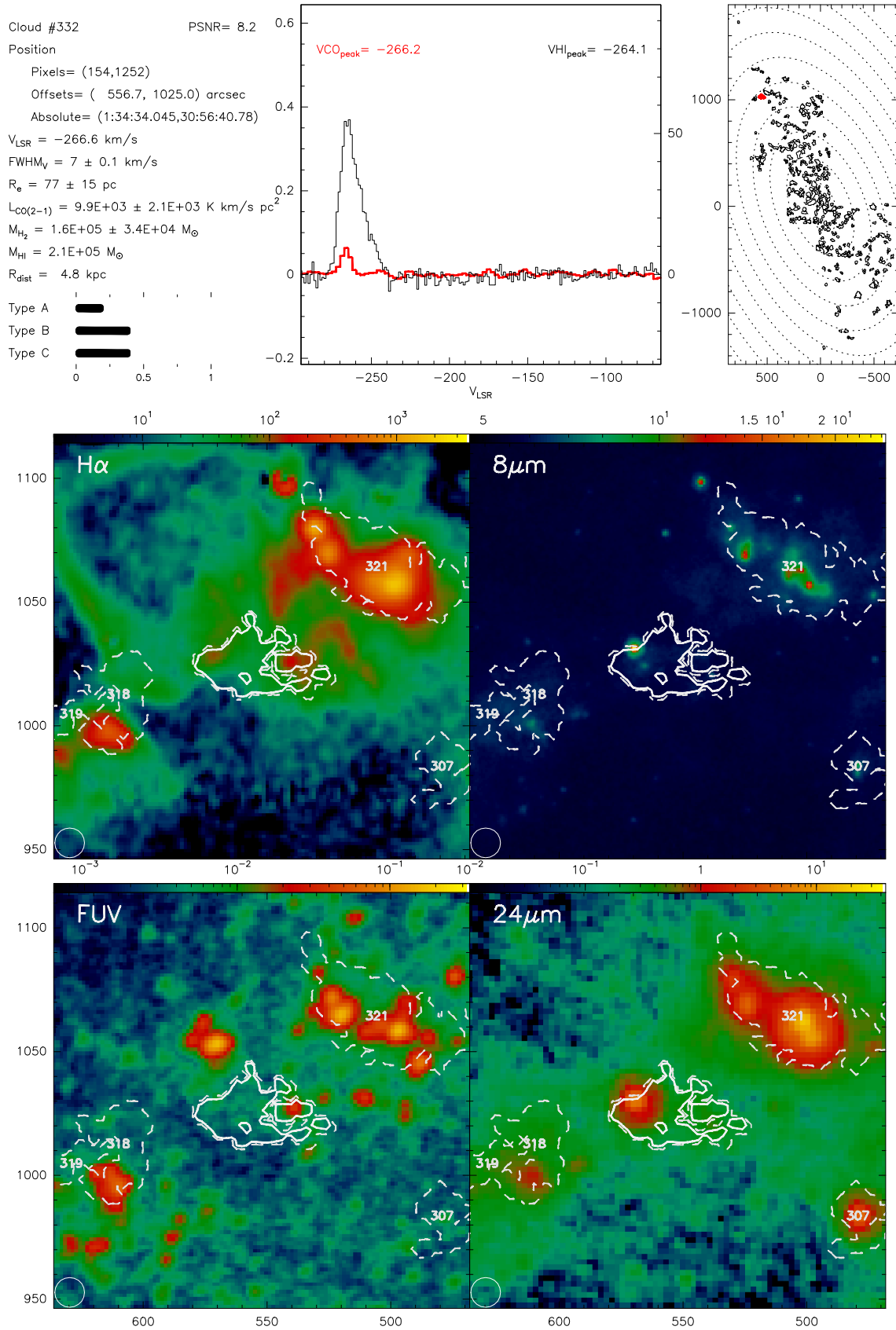
Fig. B.332. Catalogue entry for cloud 332. See description at the beginning of this appendix.
