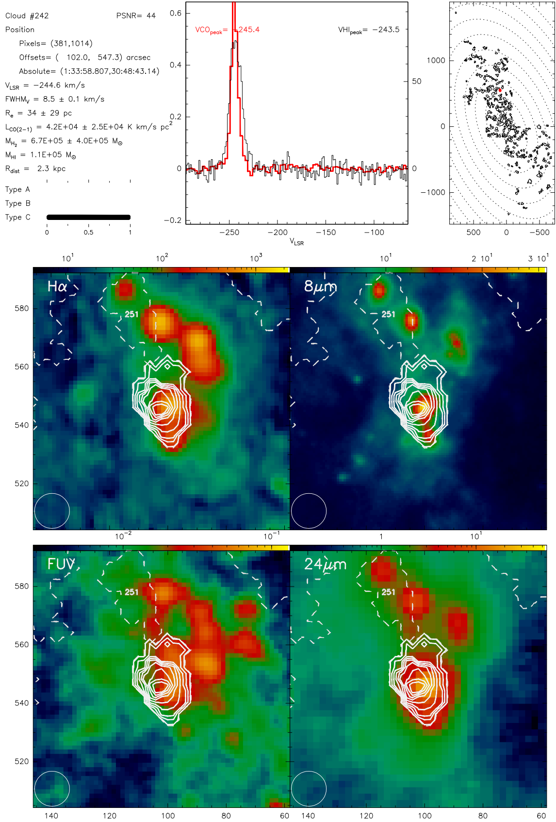
Fig. B.242. Catalogue entry for cloud 242. See description at the beginning of this appendix.
