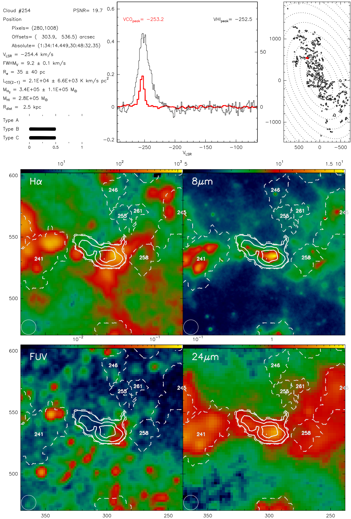
Fig. B.254. Catalogue entry for cloud 254. See description at the beginning of this appendix.
