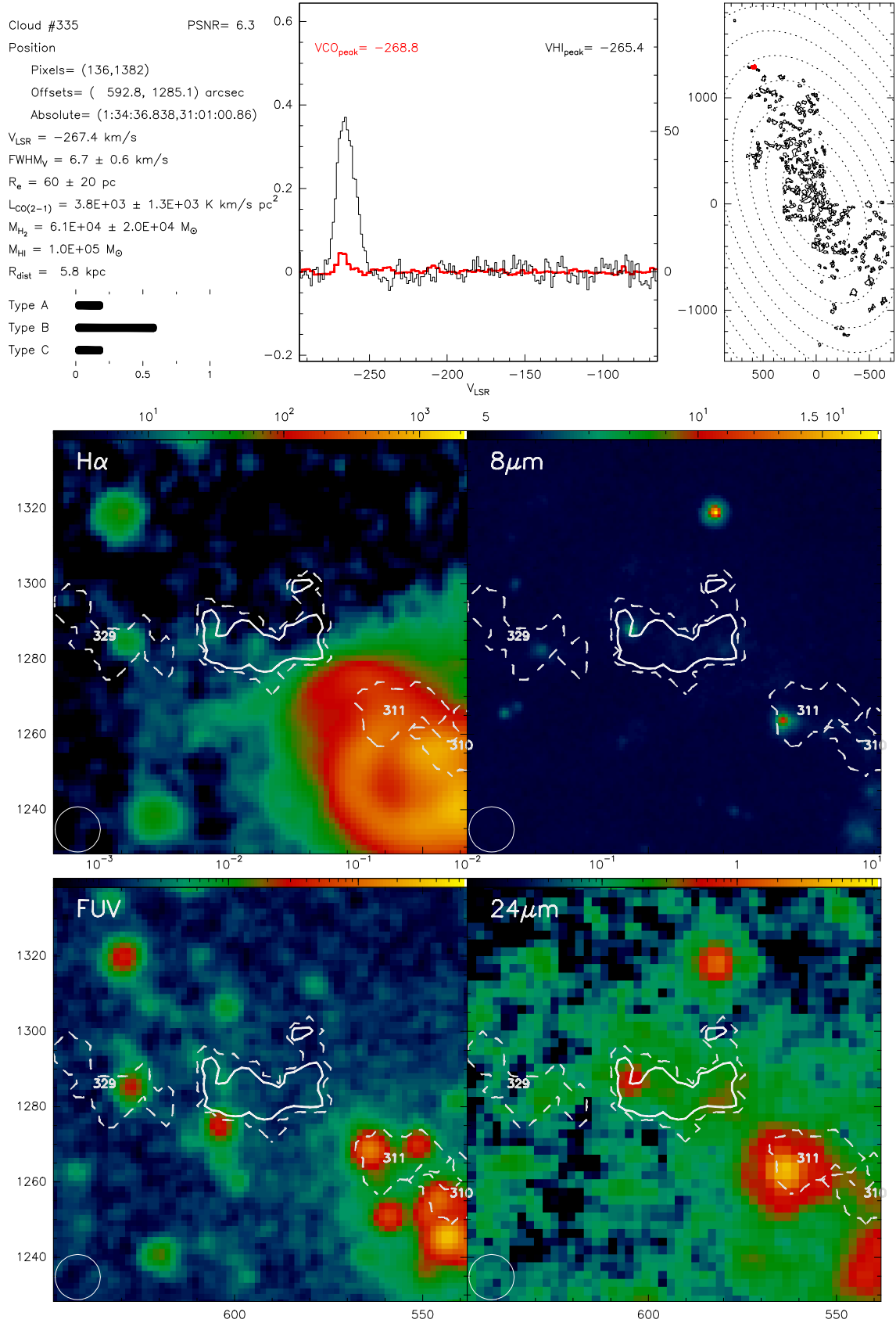
Fig. B.335. Catalogue entry for cloud 335. See description at the beginning of this appendix.
