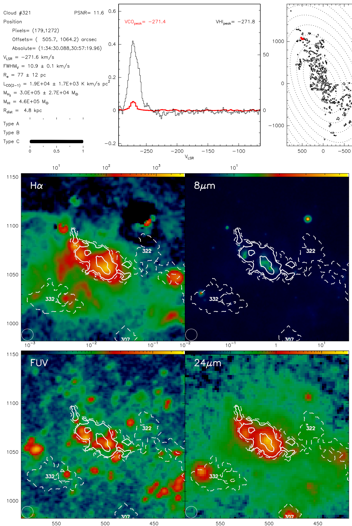
Fig. B.321. Catalogue entry for cloud 321. See description at the beginning of this appendix.
