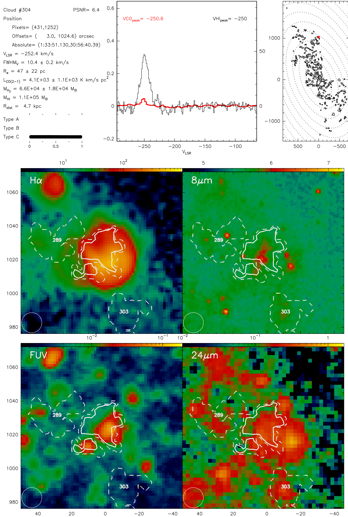
Fig. B.304. Catalogue entry for cloud 304. See description at the beginning of this appendix.
