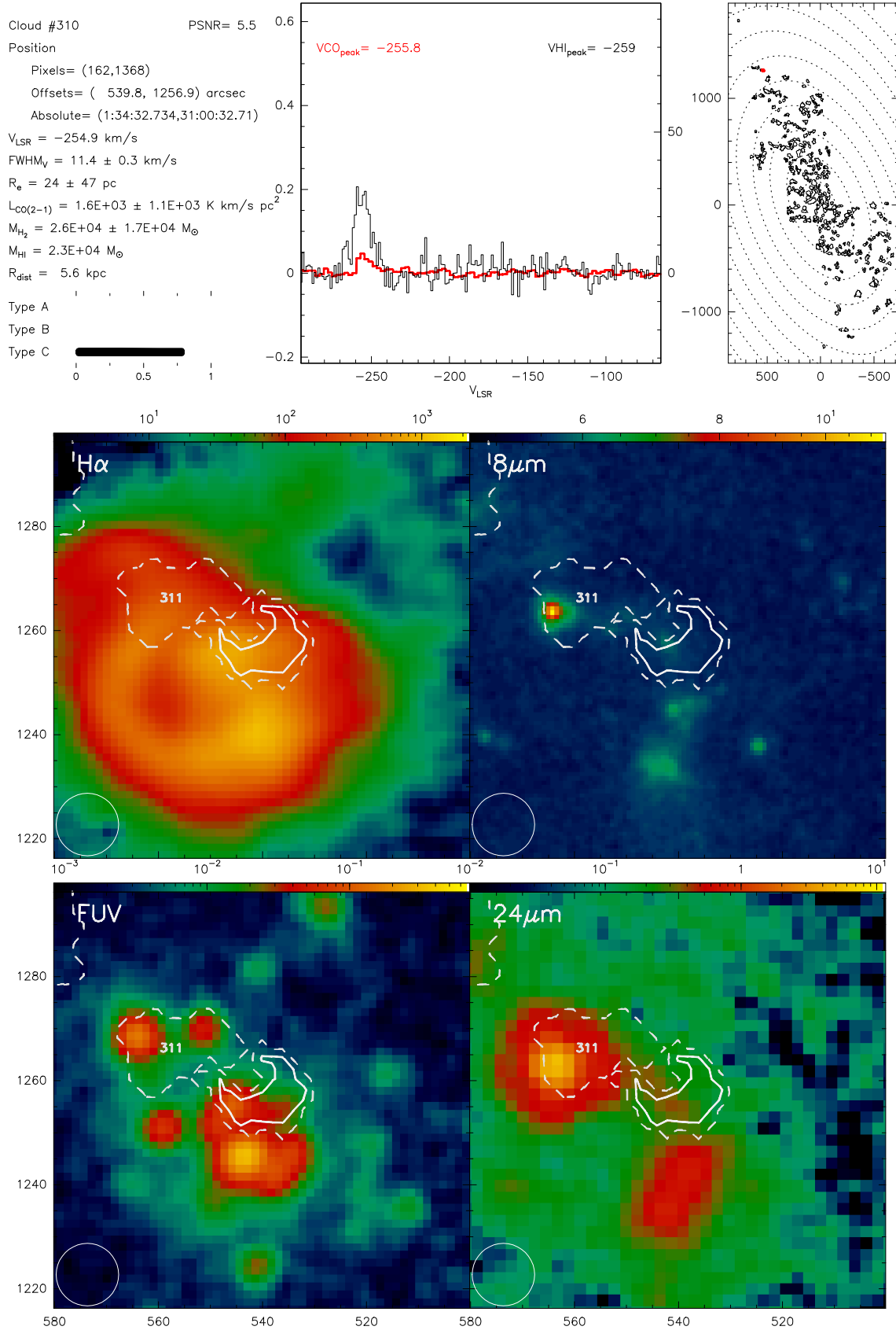
Fig. B.310. Catalogue entry for cloud 310. See description at the beginning of this appendix.
