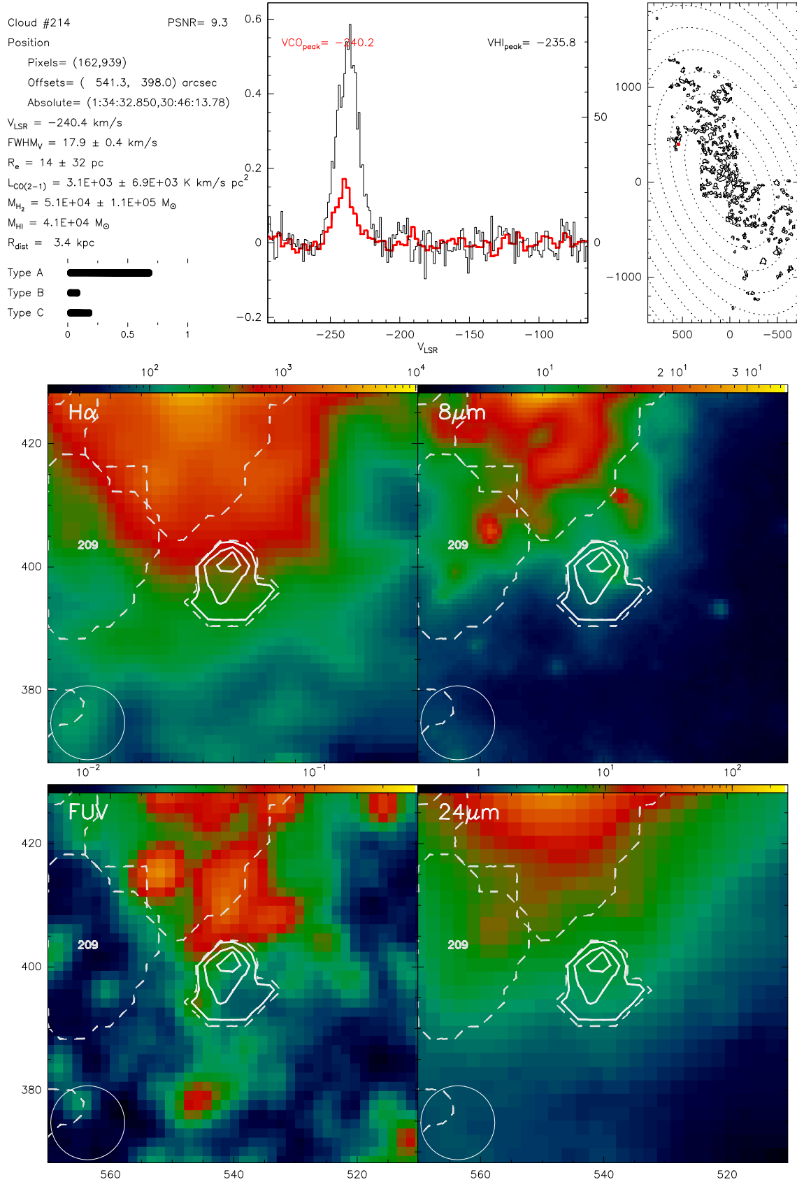
Fig. B.214. Catalogue entry for cloud 214. See description at the beginning of this appendix.
