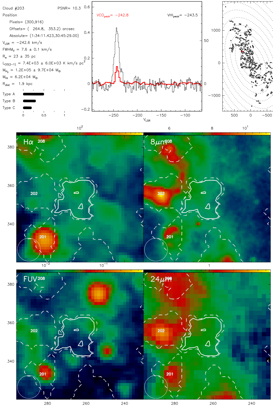
Fig. B.203. Catalogue entry for cloud 203. See description at the beginning of this appendix.
