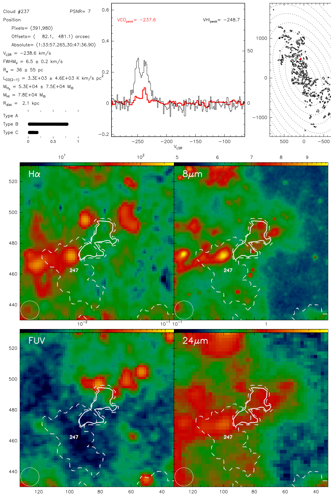
Fig. B.237. Catalogue entry for cloud 237. See description at the beginning of this appendix.
