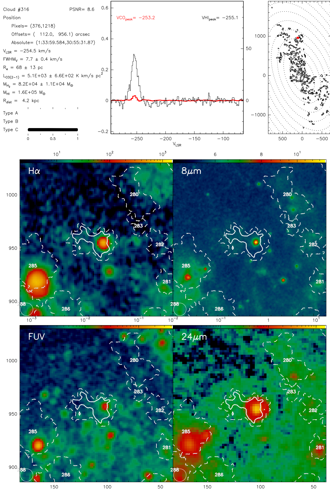
Fig. B.316. Catalogue entry for cloud 316. See description at the beginning of this appendix.
