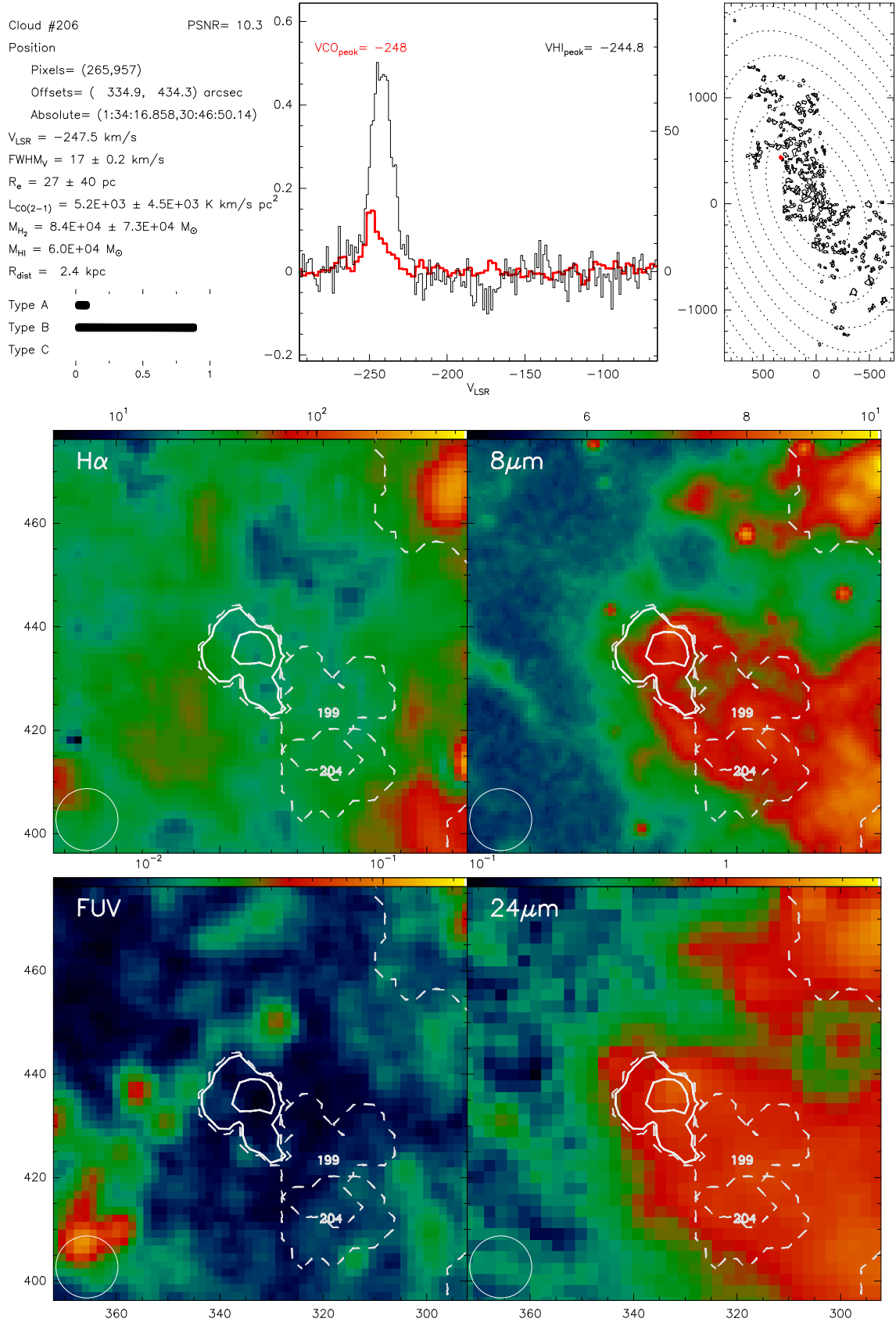
Fig. B.206. Catalogue entry for cloud 206. See description at the beginning of this appendix.
