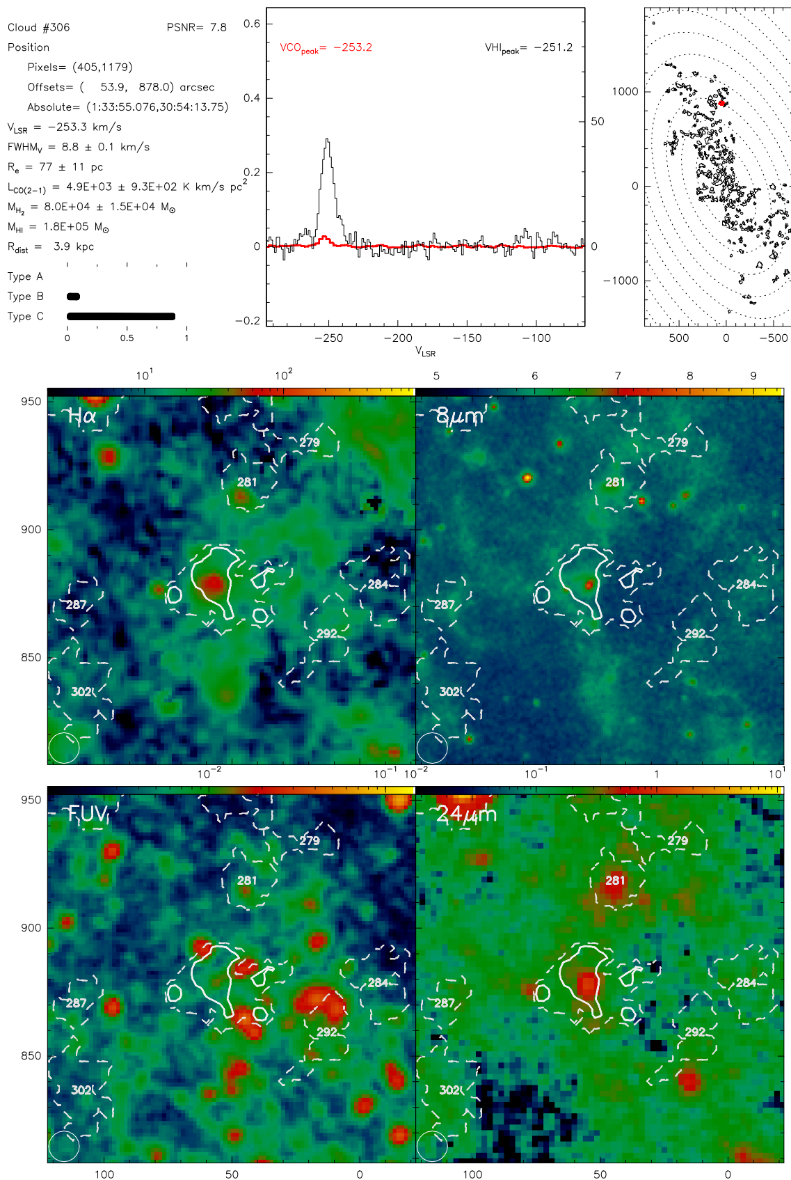
Fig. B.306. Catalogue entry for cloud 306. See description at the beginning of this appendix.
