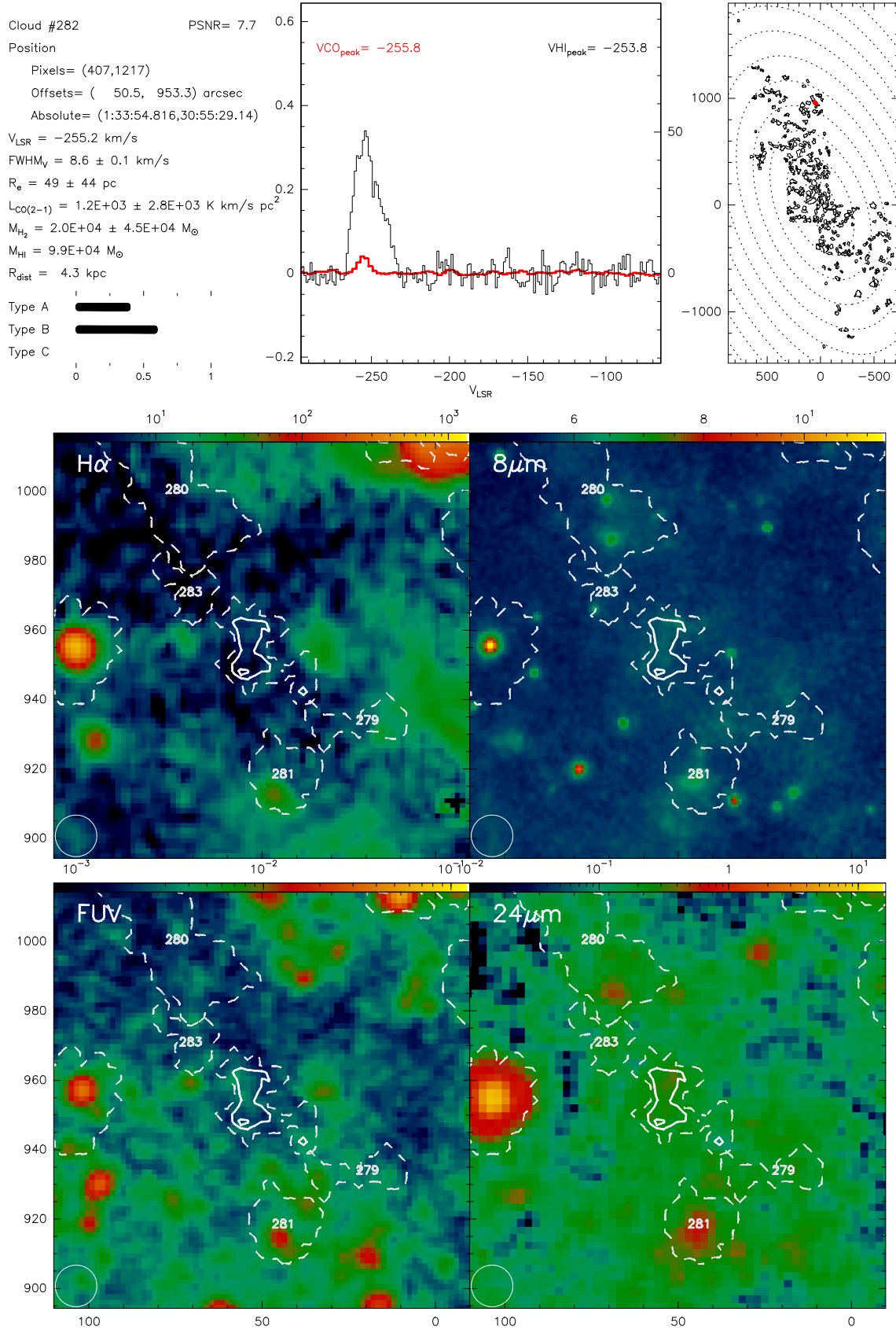
Fig. B.282. Catalogue entry for cloud 282. See description at the beginning of this appendix.
