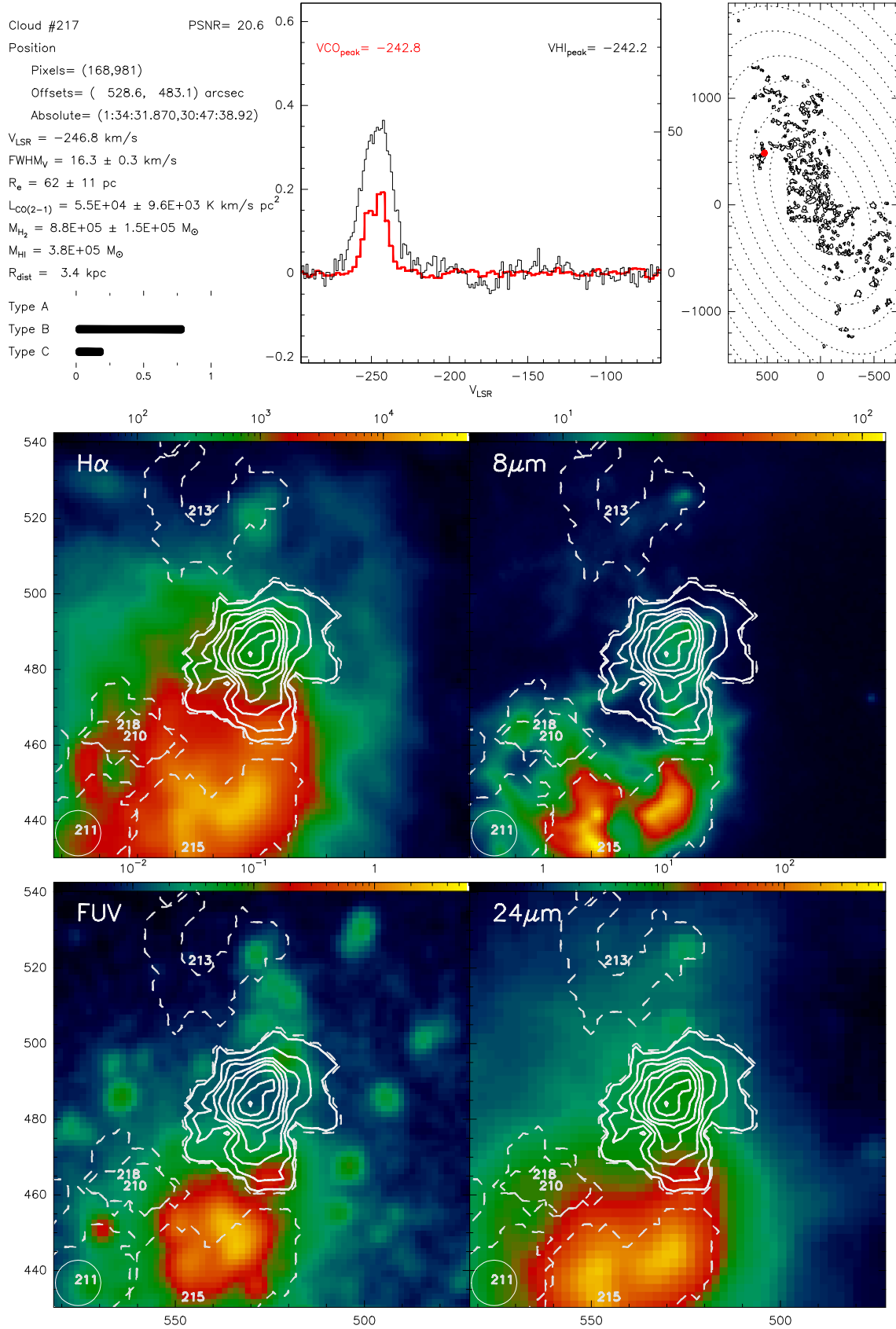
Fig. B.217. Catalogue entry for cloud 217. See description at the beginning of this appendix.
