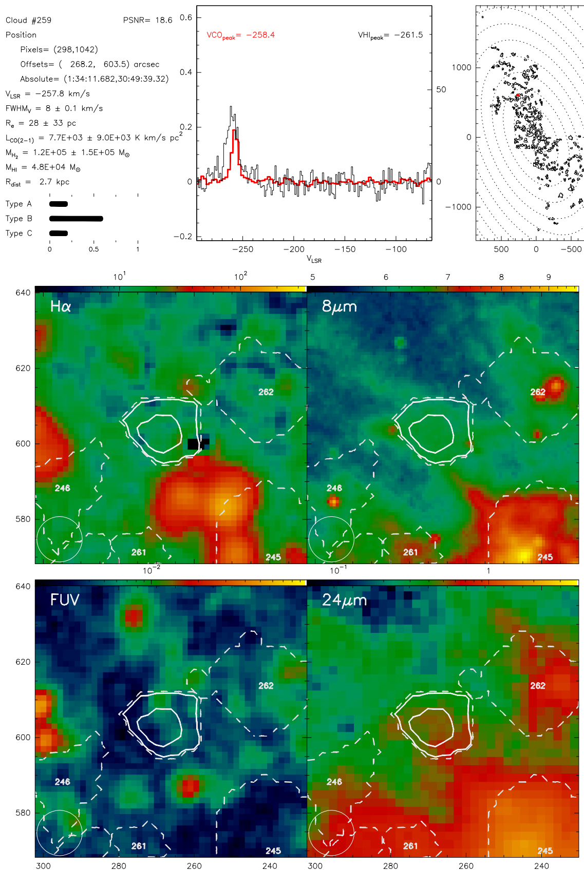
Fig. B.259. Catalogue entry for cloud 259. See description at the beginning of this appendix.
