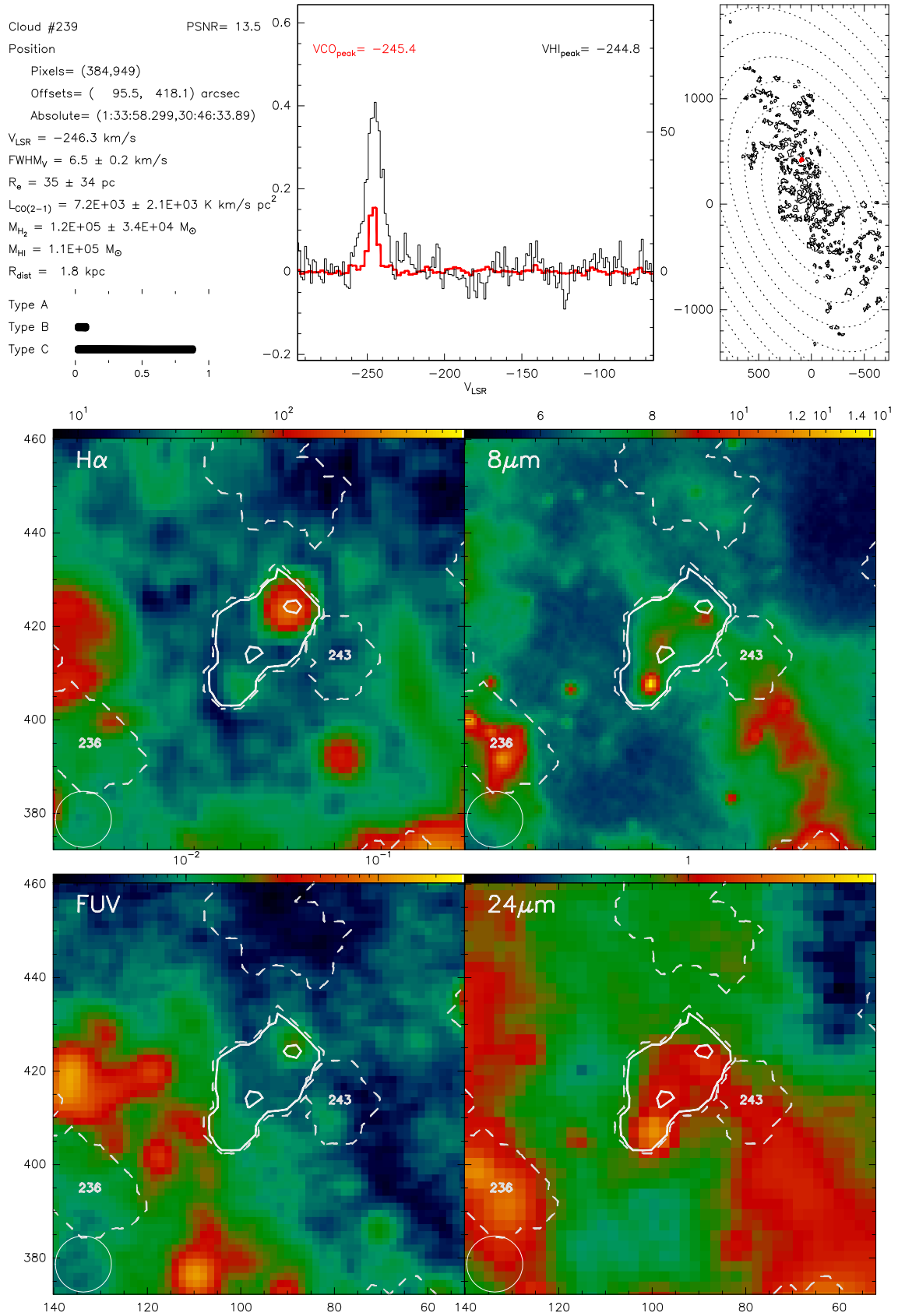
Fig. B.239. Catalogue entry for cloud 239. See description at the beginning of this appendix.
