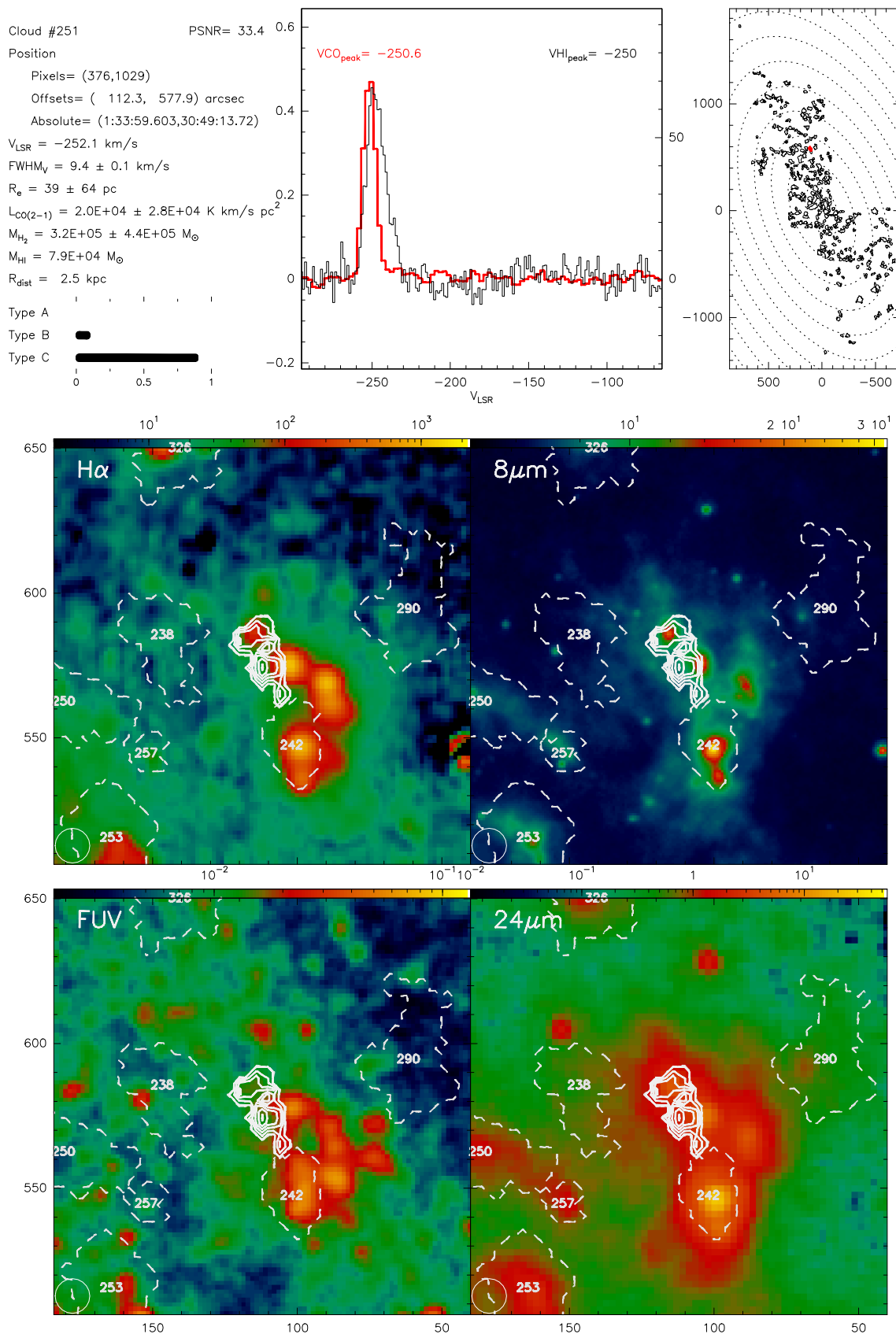
Fig. B.251. Catalogue entry for cloud 251. See description at the beginning of this appendix.
