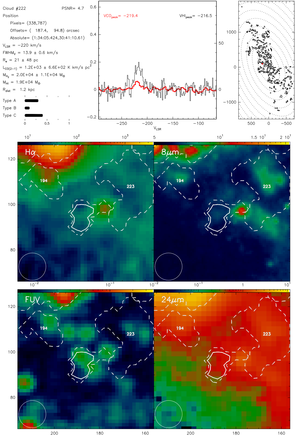
Fig. B.222. Catalogue entry for cloud 222. See description at the beginning of this appendix.
