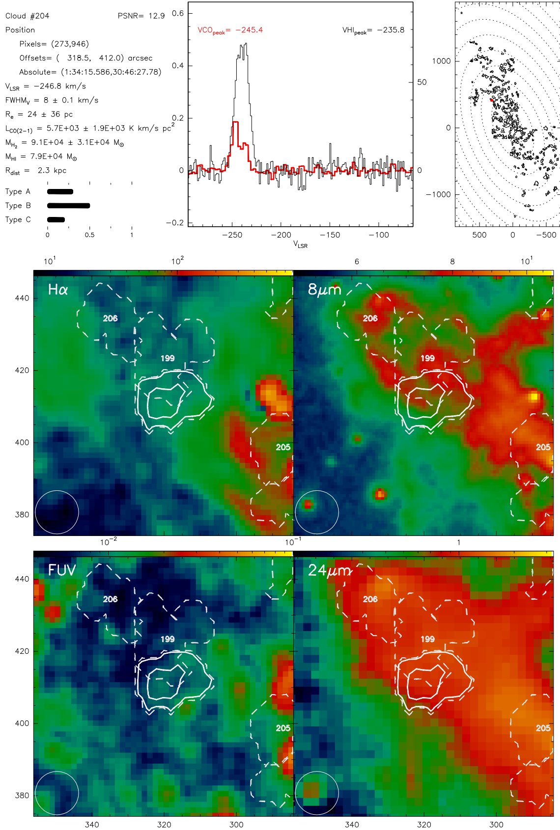
Fig. B.204. Catalogue entry for cloud 204. See description at the beginning of this appendix.
