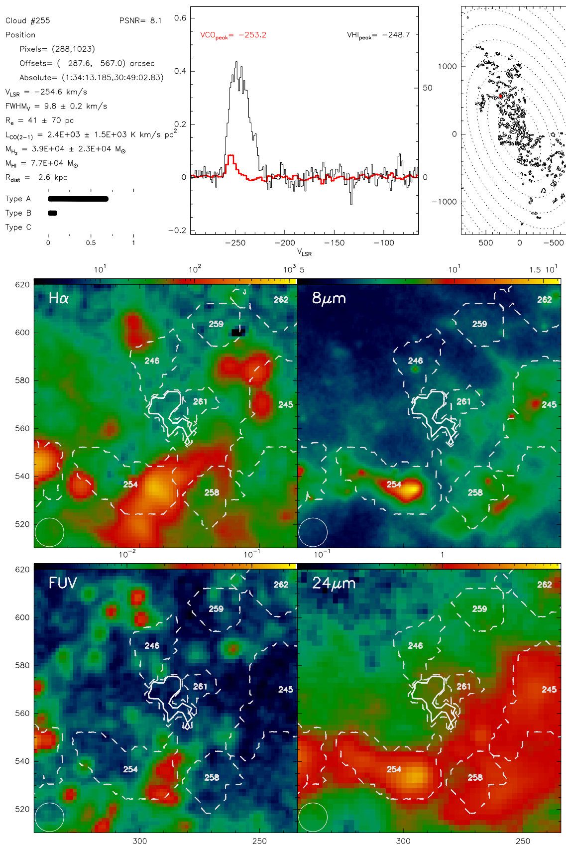
Fig. B.255. Catalogue entry for cloud 255. See description at the beginning of this appendix.
