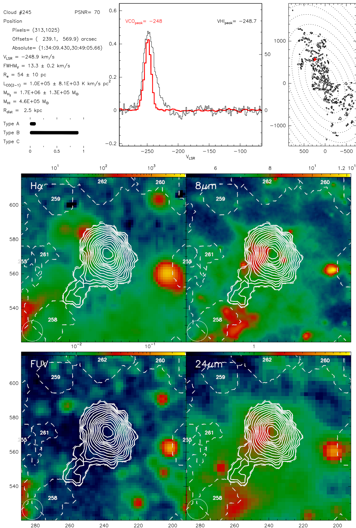
Fig. B.245. Catalogue entry for cloud 245. See description at the beginning of this appendix.
