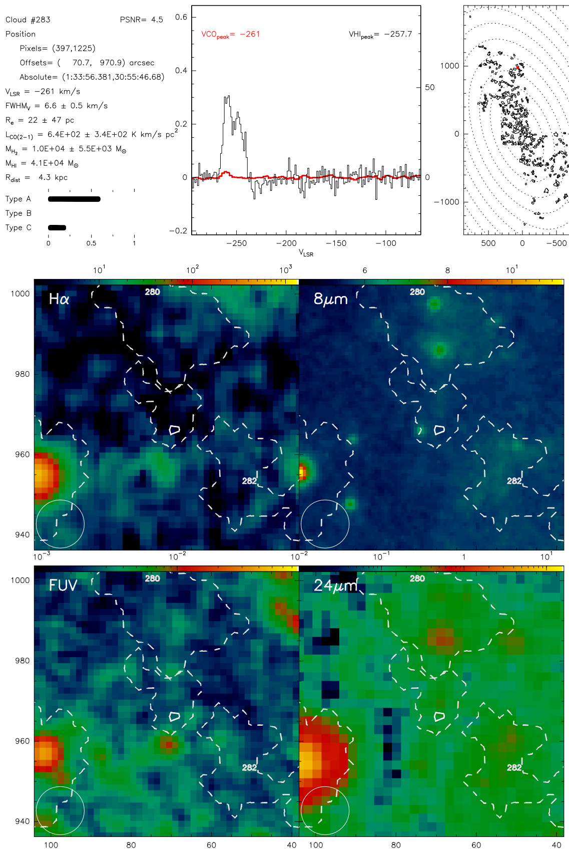
Fig. B.283. Catalogue entry for cloud 283. See description at the beginning of this appendix.
