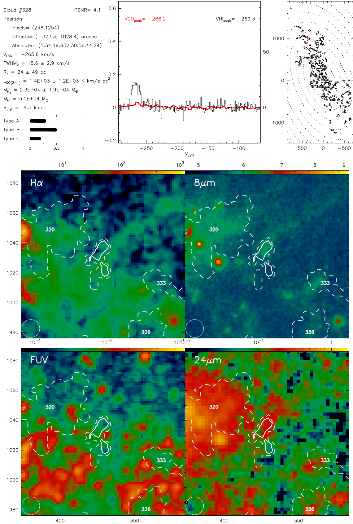
Fig. B.328. Catalogue entry for cloud 328. See description at the beginning of this appendix.
