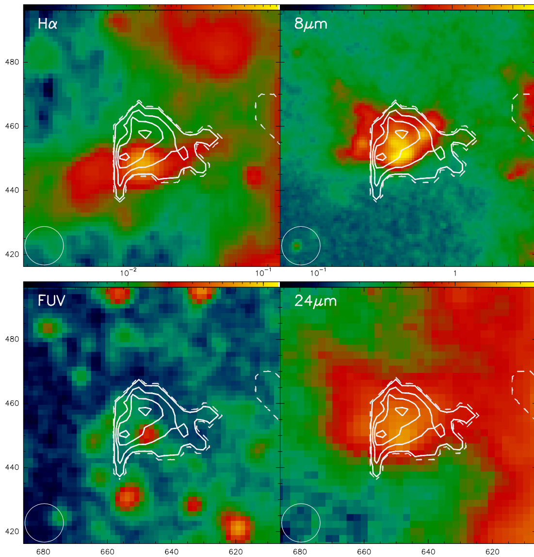
Fig. B.276. Catalogue entry for cloud 276. See description at the beginning of this appendix.
