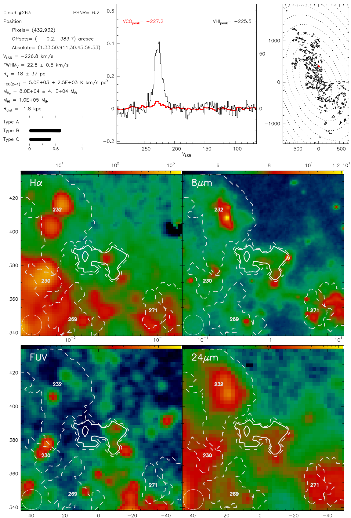
Fig. B.263. Catalogue entry for cloud 263. See description at the beginning of this appendix.
