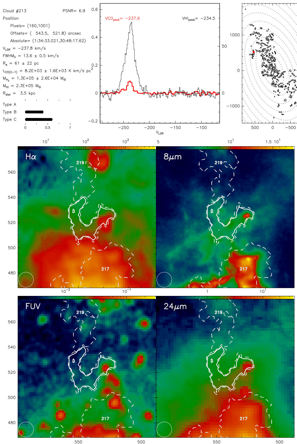
Fig. B.213. Catalogue entry for cloud 213. See description at the beginning of this appendix.
