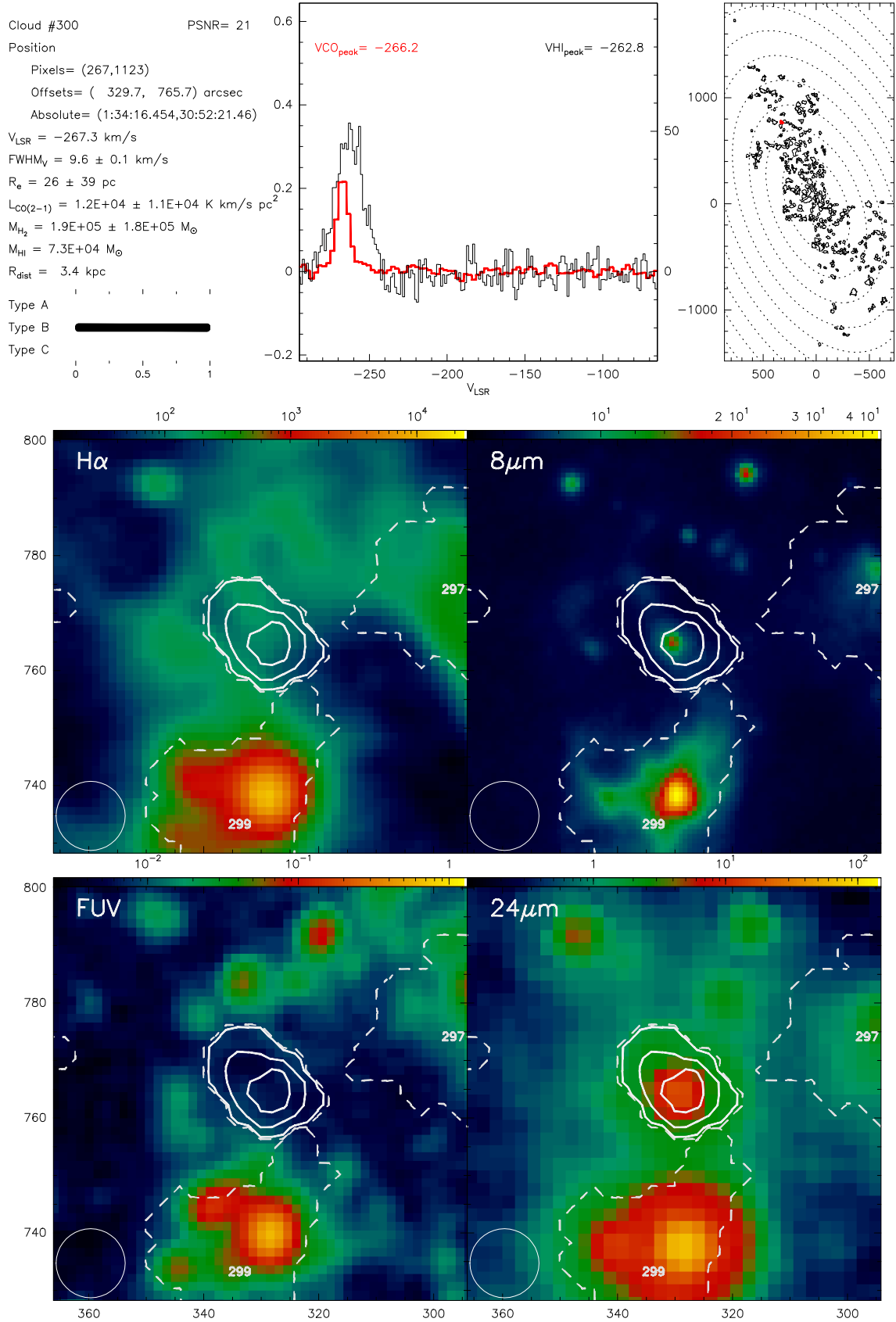
Fig. B.300. Catalogue entry for cloud 300. See description at the beginning of this appendix.
