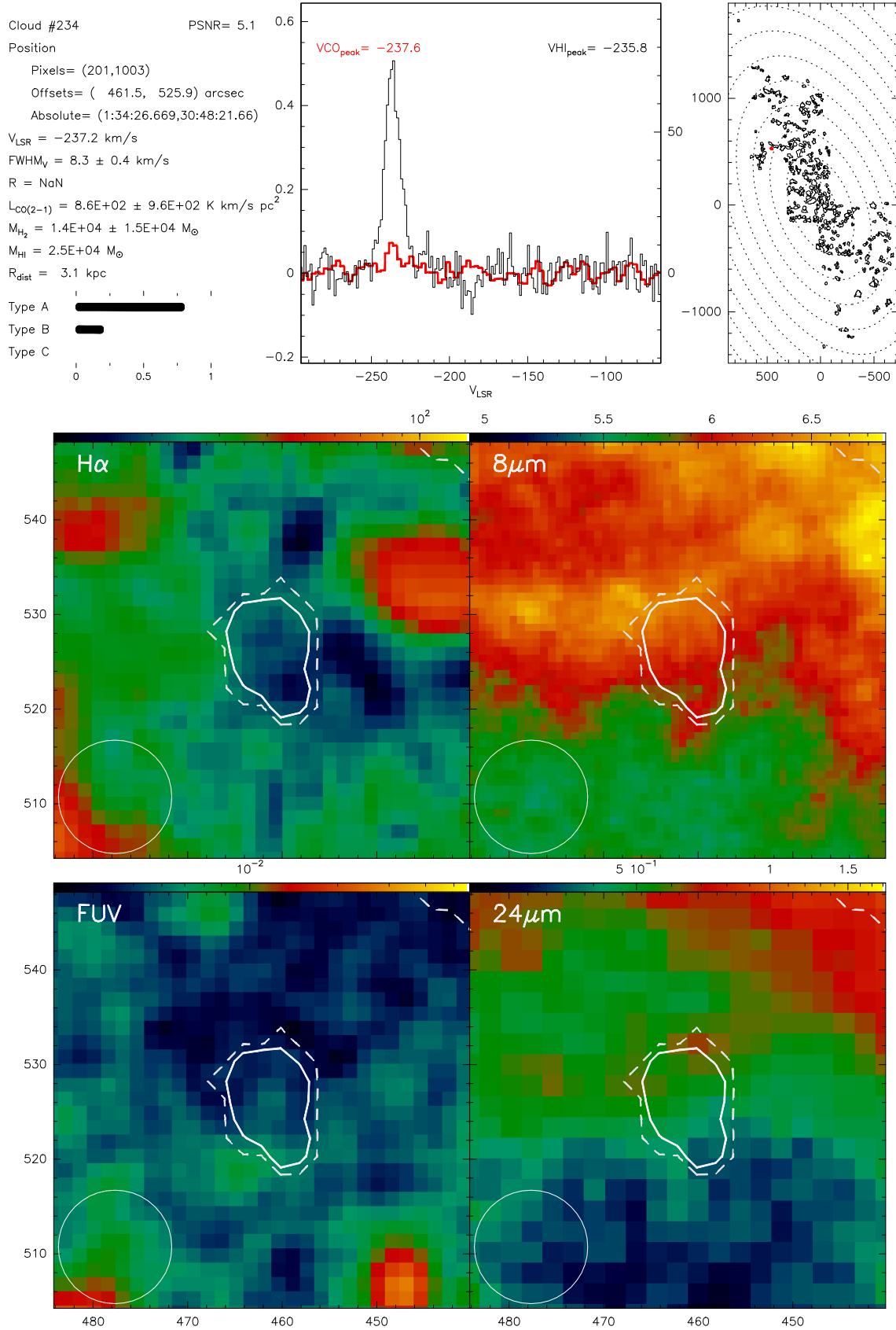
Fig. B.234. Catalogue entry for cloud 234. See description at the beginning of this appendix.
