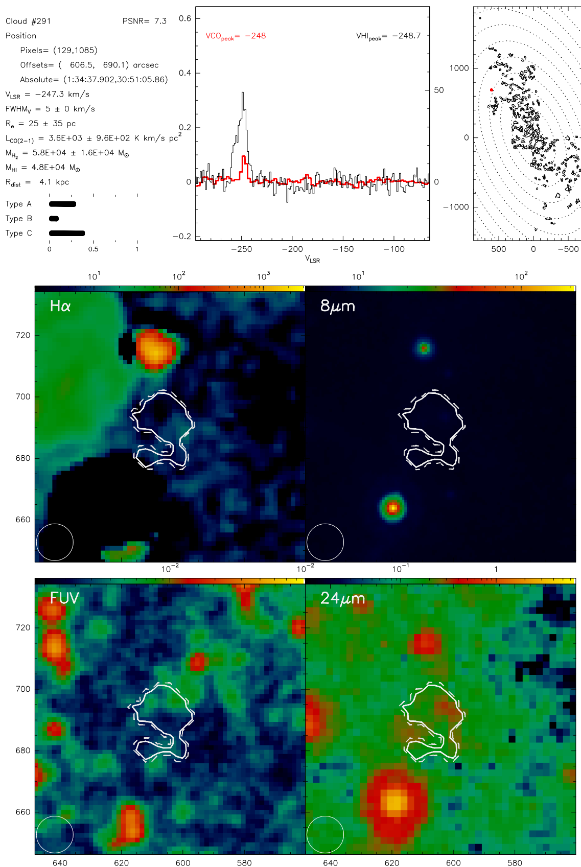
Fig. B.291. Catalogue entry for cloud 291. See description at the beginning of this appendix.
