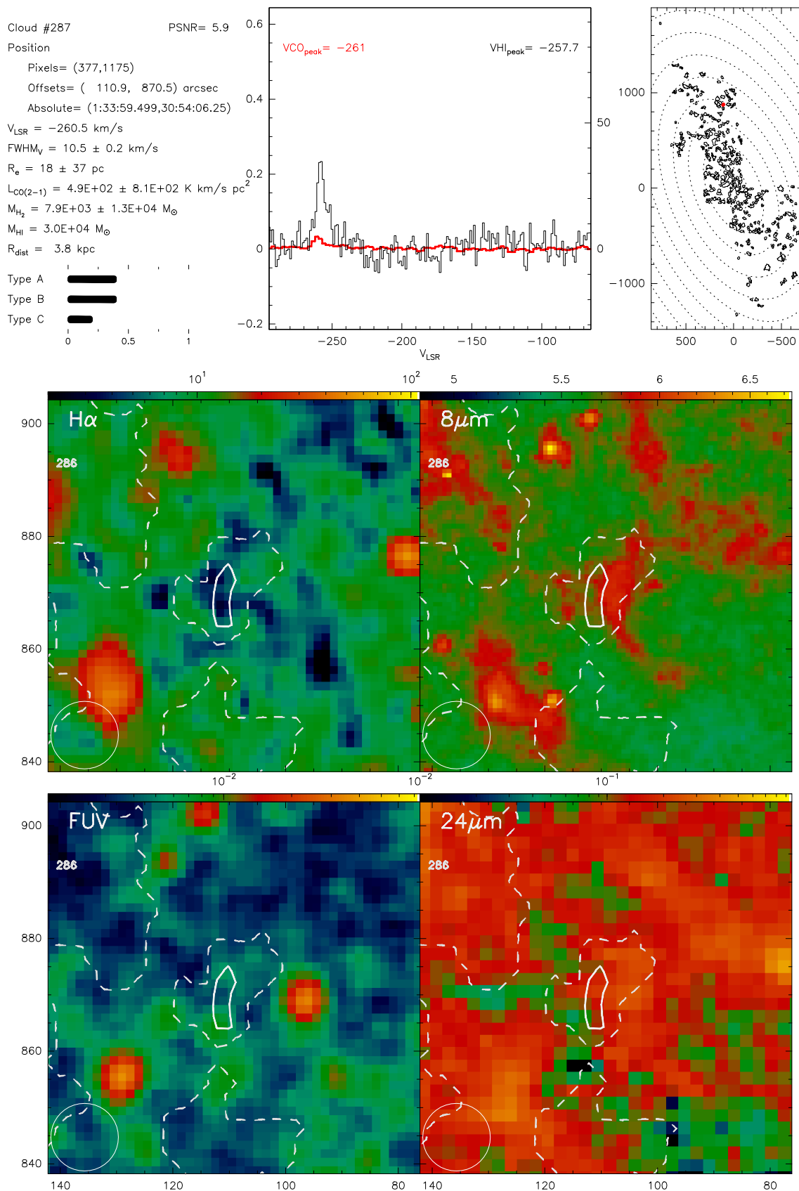
Fig. B.287. Catalogue entry for cloud 287. See description at the beginning of this appendix.
