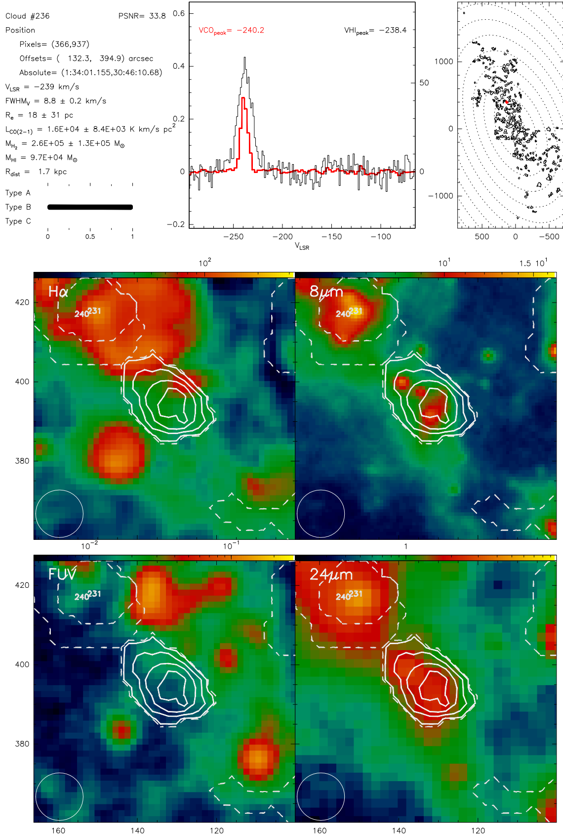
Fig. B.236. Catalogue entry for cloud 236. See description at the beginning of this appendix.
