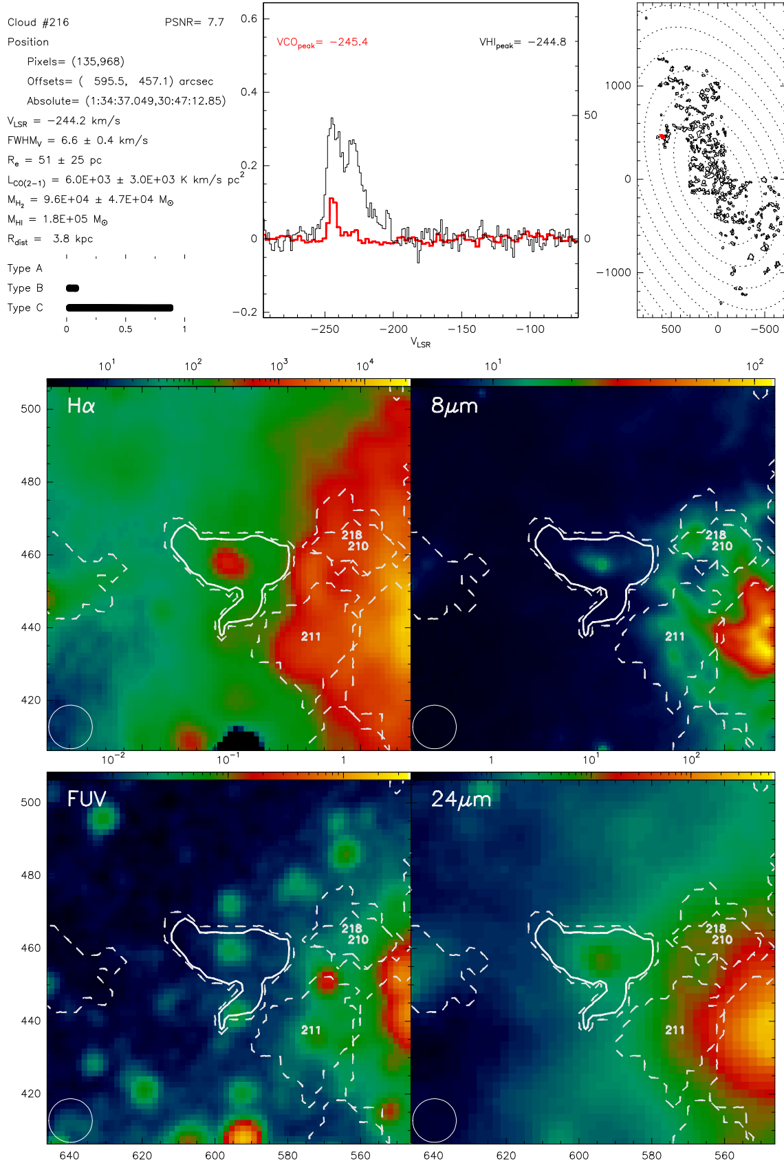
Fig. B.216. Catalogue entry for cloud 216. See description at the beginning of this appendix.
