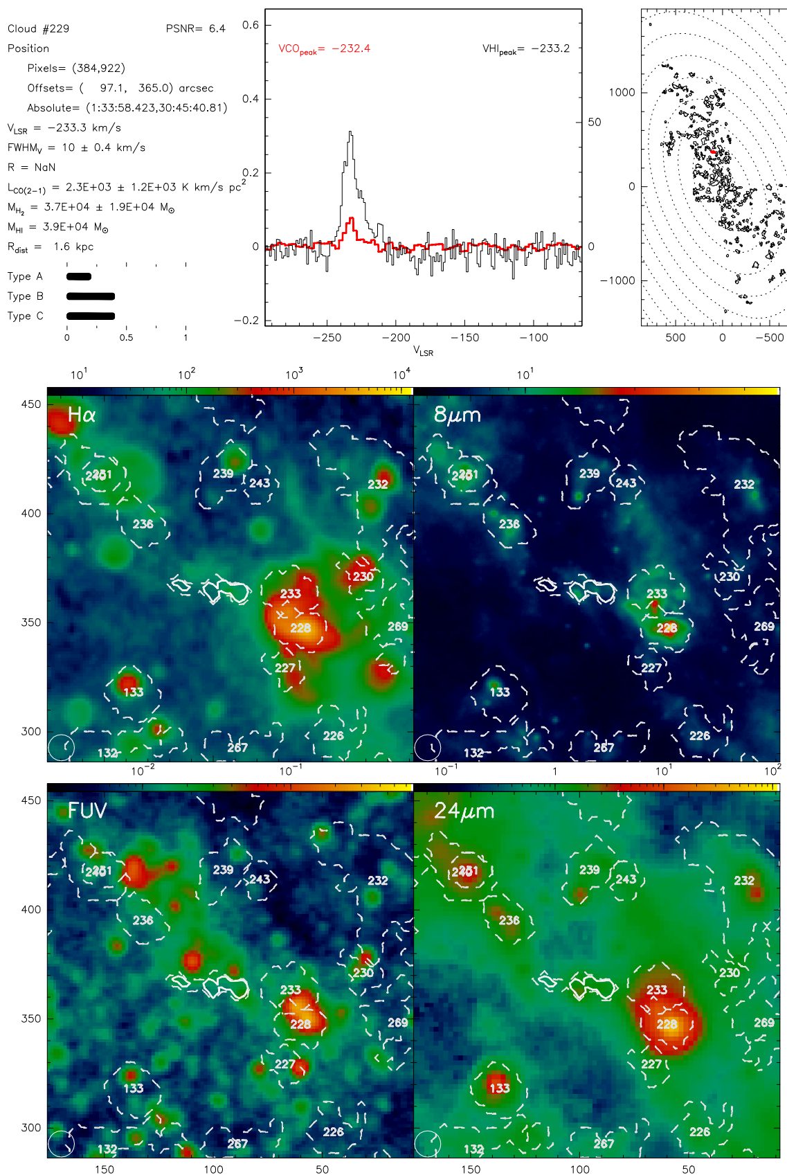
Fig. B.229. Catalogue entry for cloud 229. See description at the beginning of this appendix.
