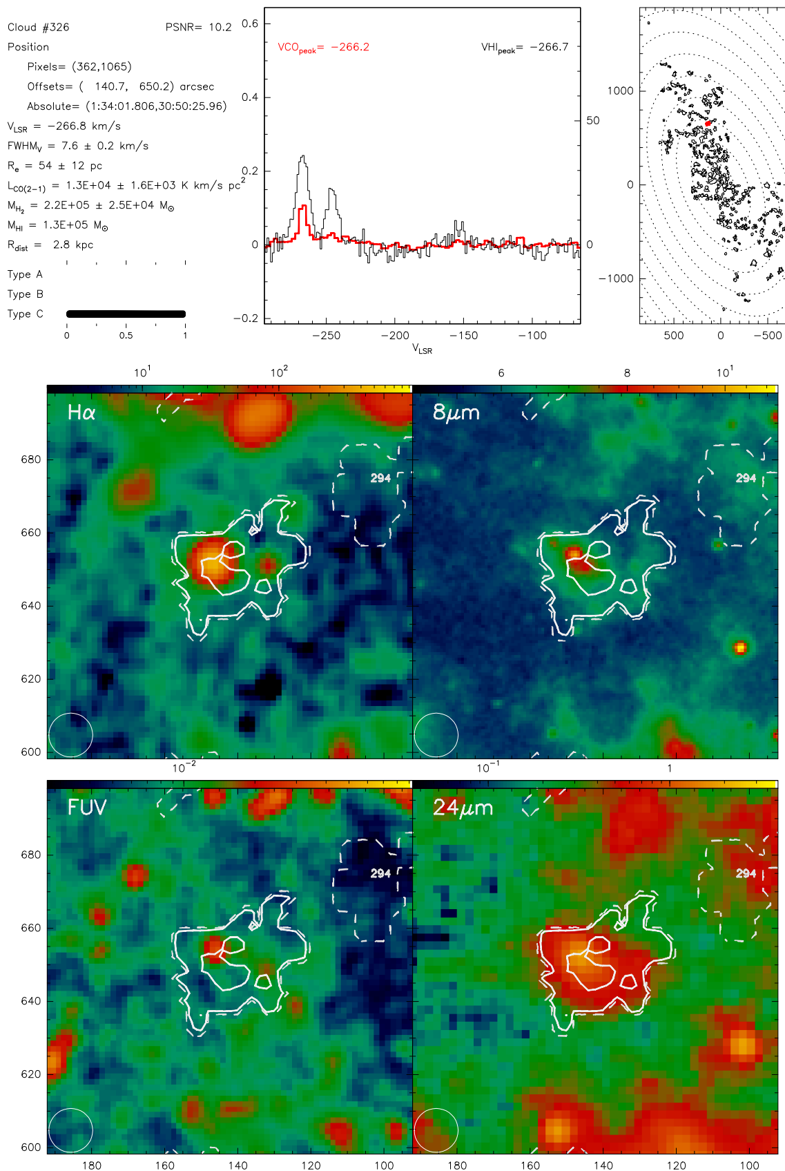
Fig. B.326. Catalogue entry for cloud 326. See description at the beginning of this appendix.
