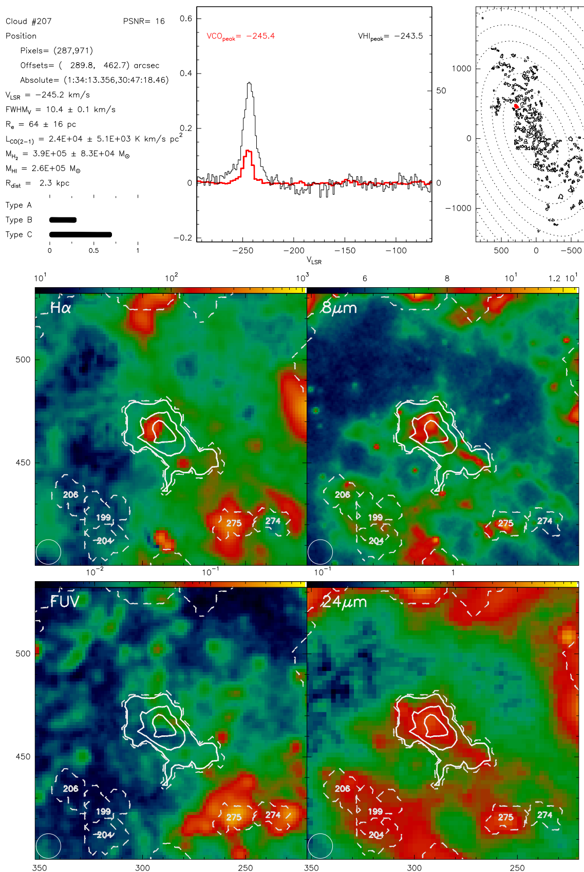
Fig. B.207. Catalogue entry for cloud 207. See description at the beginning of this appendix.
