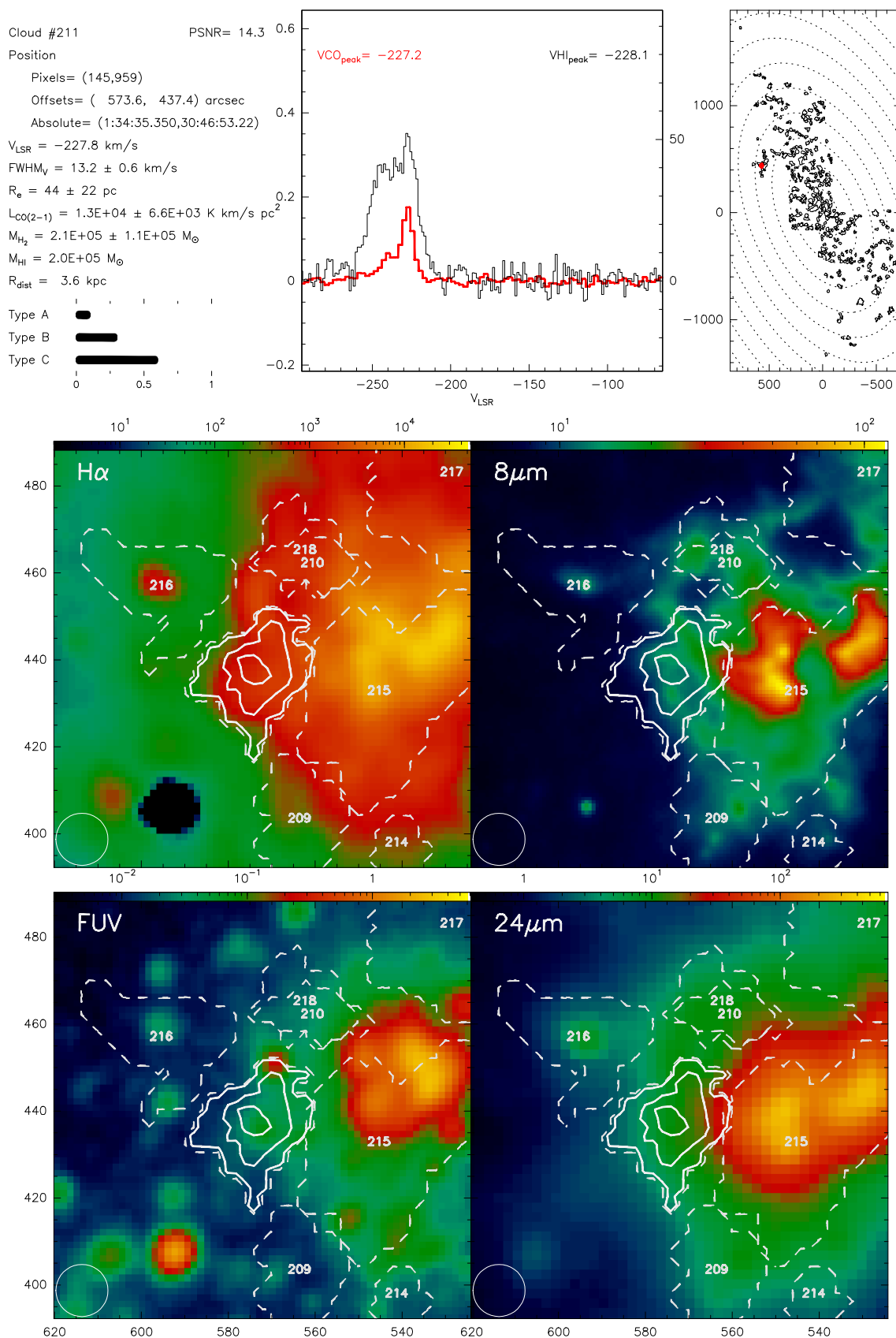
Fig. B.211. Catalogue entry for cloud 211. See description at the beginning of this appendix.
