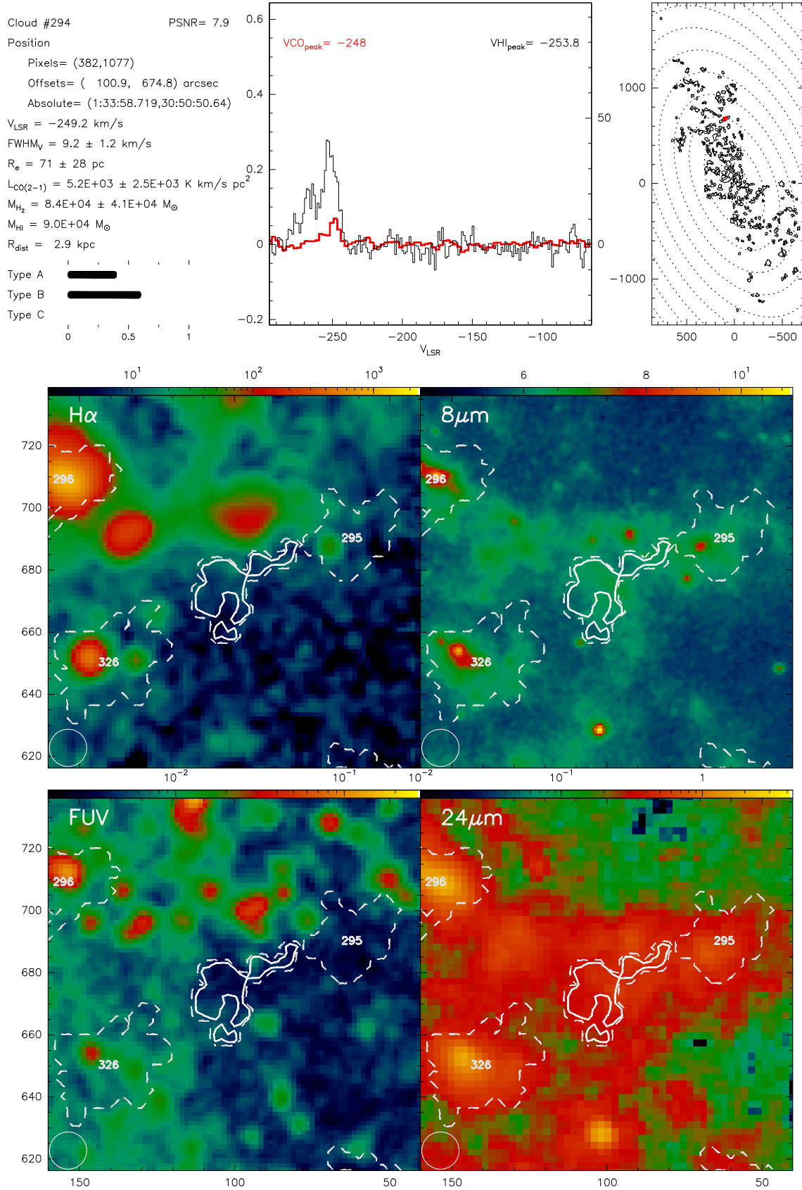
Fig. B.294. Catalogue entry for cloud 294. See description at the beginning of this appendix.
