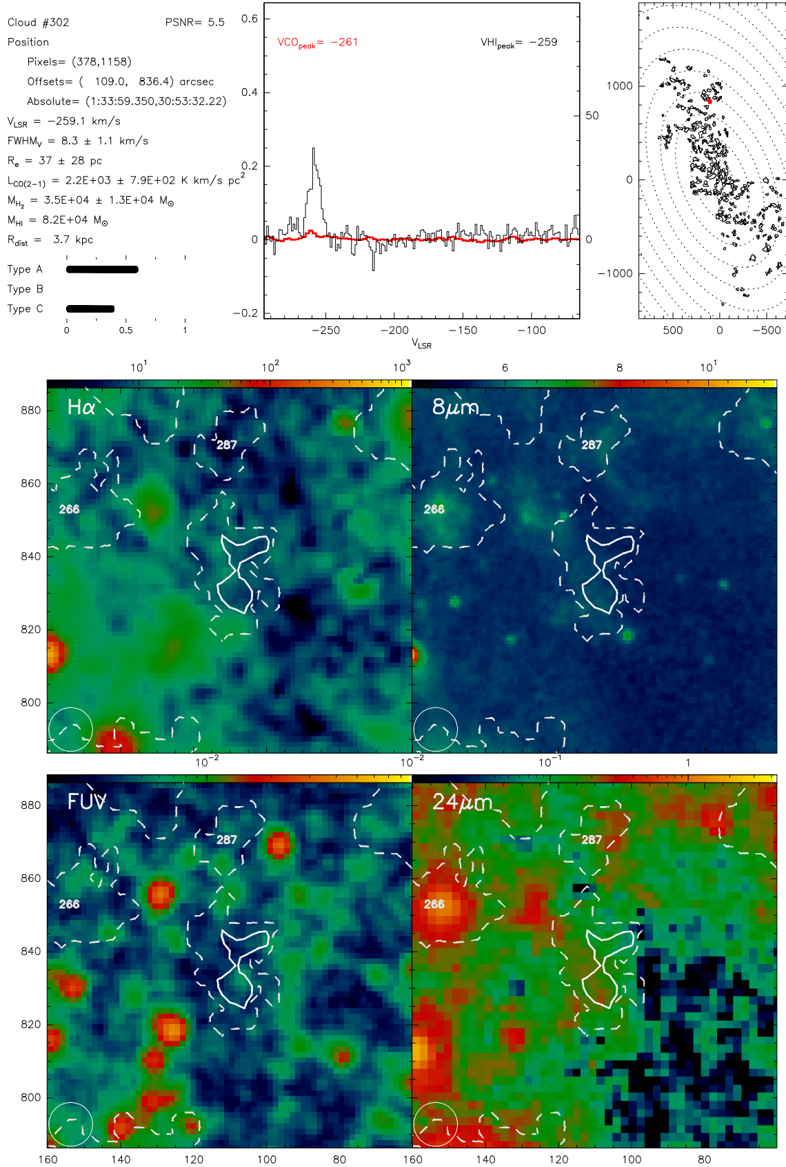
Fig. B.302. Catalogue entry for cloud 302. See description at the beginning of this appendix.
