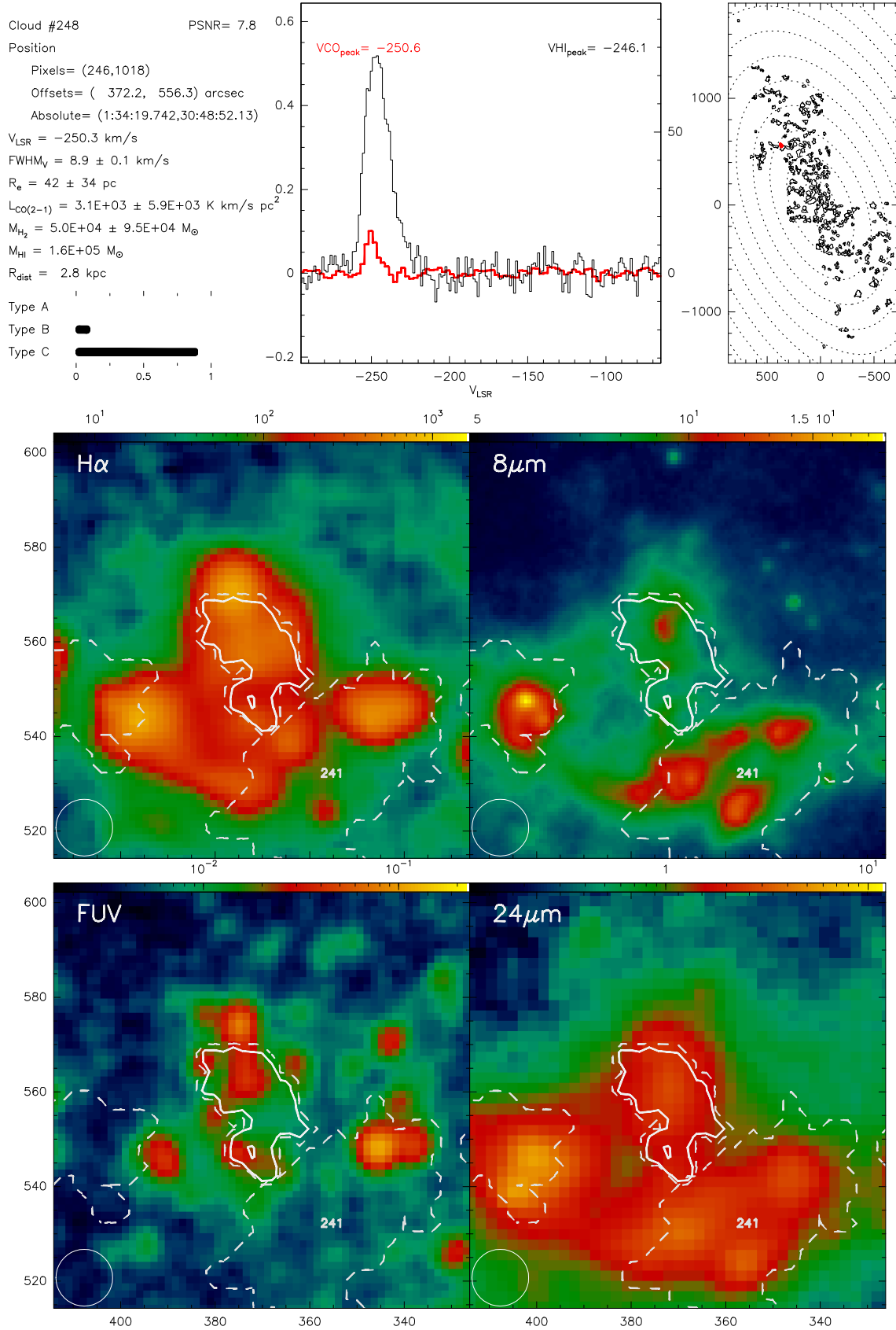
Fig. B.248. Catalogue entry for cloud 248. See description at the beginning of this appendix.
