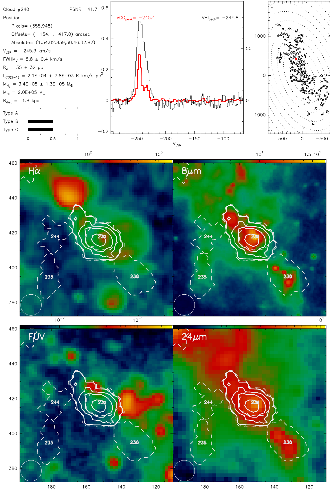
Fig. B.240. Catalogue entry for cloud 240. See description at the beginning of this appendix.
