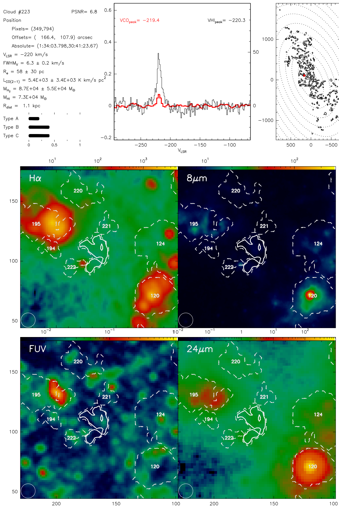
Fig. B.223. Catalogue entry for cloud 223. See description at the beginning of this appendix.
