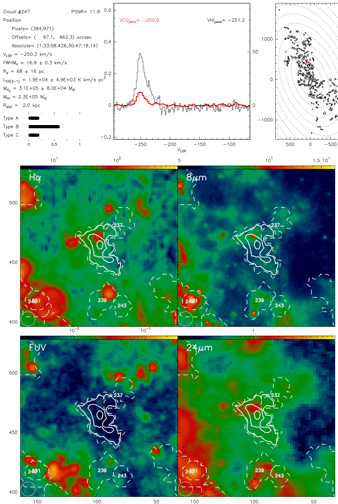
Fig. B.247. Catalogue entry for cloud 247. See description at the beginning of this appendix.
