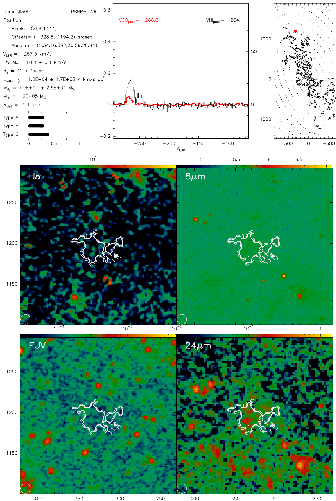
Fig. B.309. Catalogue entry for cloud 309. See description at the beginning of this appendix.
