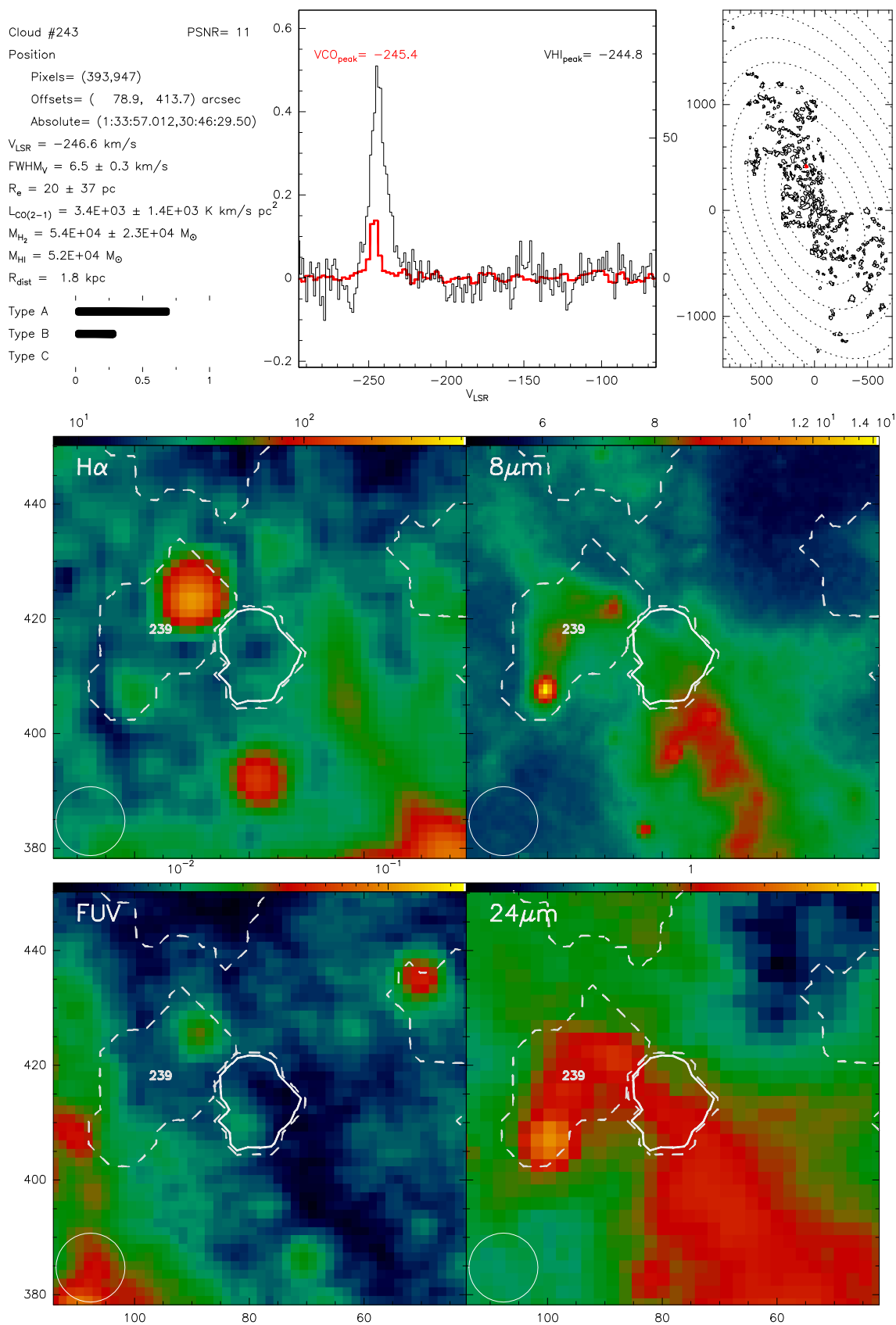
Fig. B.243. Catalogue entry for cloud 243. See description at the beginning of this appendix.
