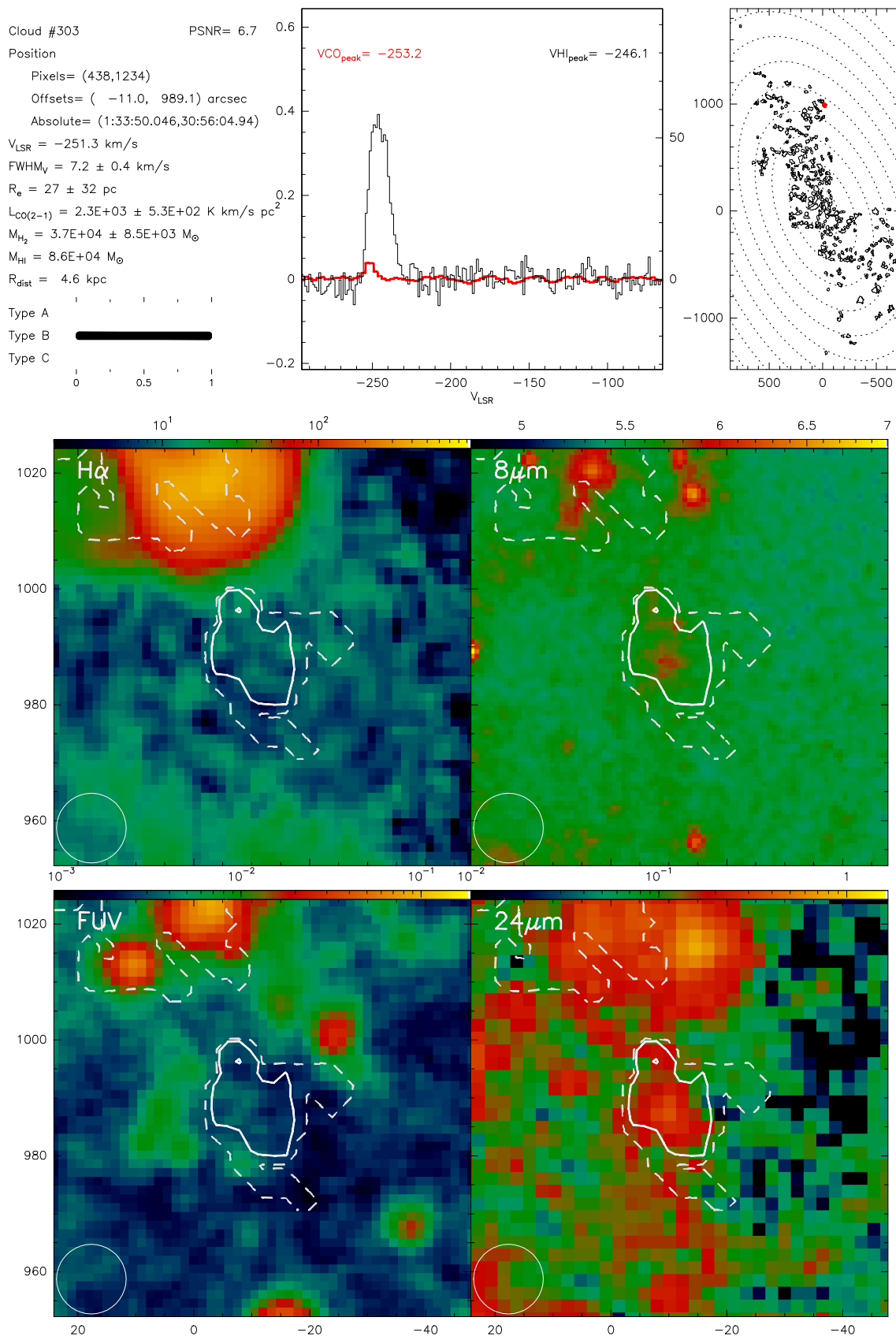
Fig. B.303. Catalogue entry for cloud 303. See description at the beginning of this appendix.
