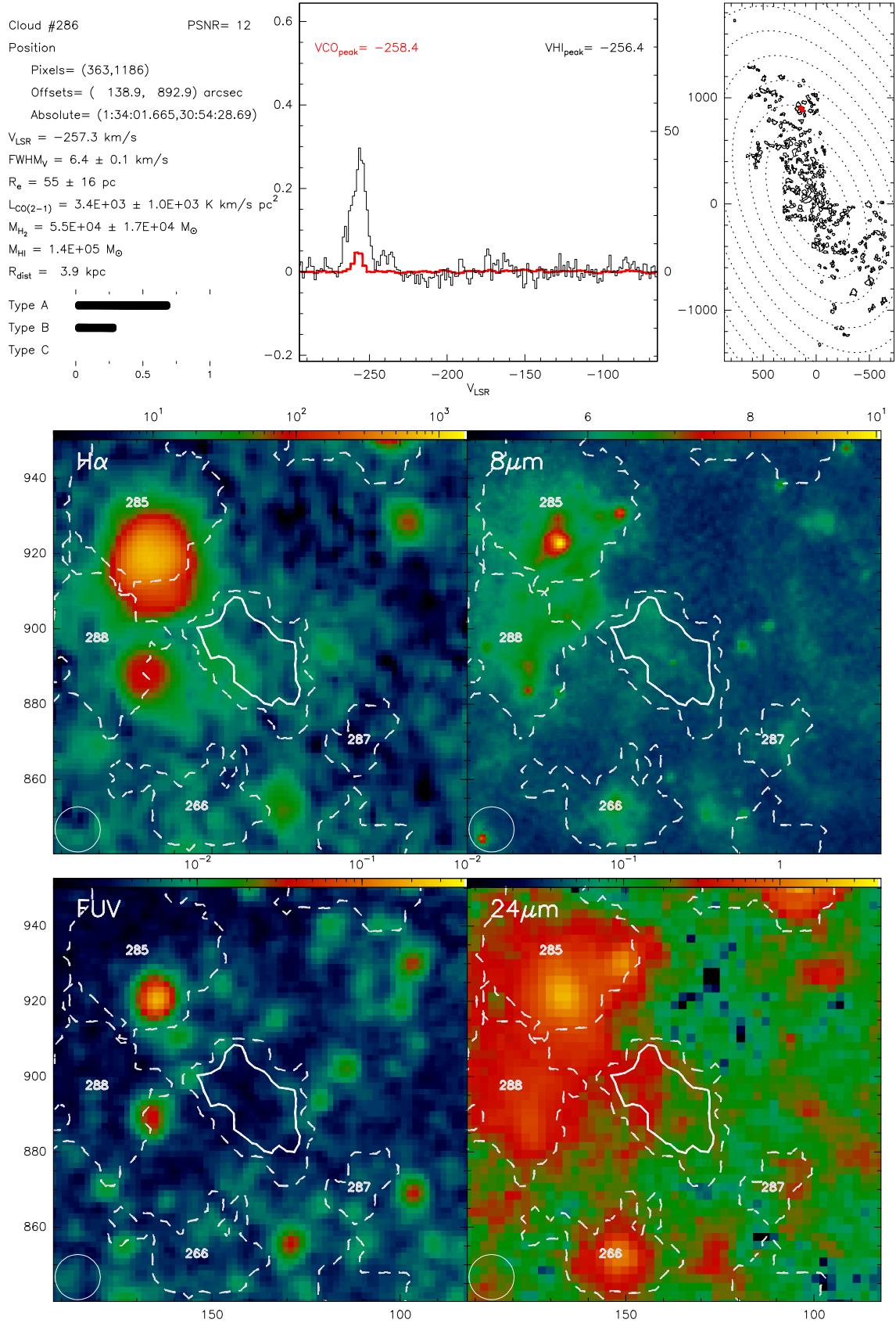
Fig. B.286. Catalogue entry for cloud 286. See description at the beginning of this appendix.
