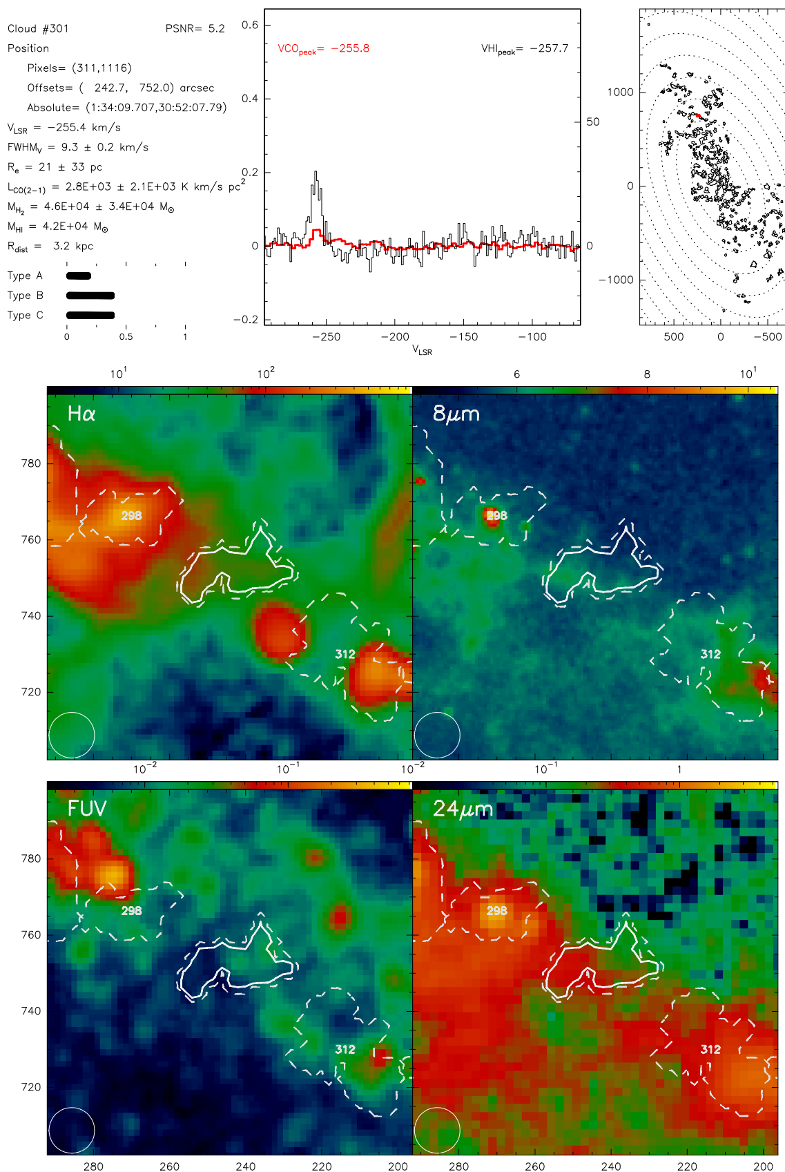
Fig. B.301. Catalogue entry for cloud 301. See description at the beginning of this appendix.
