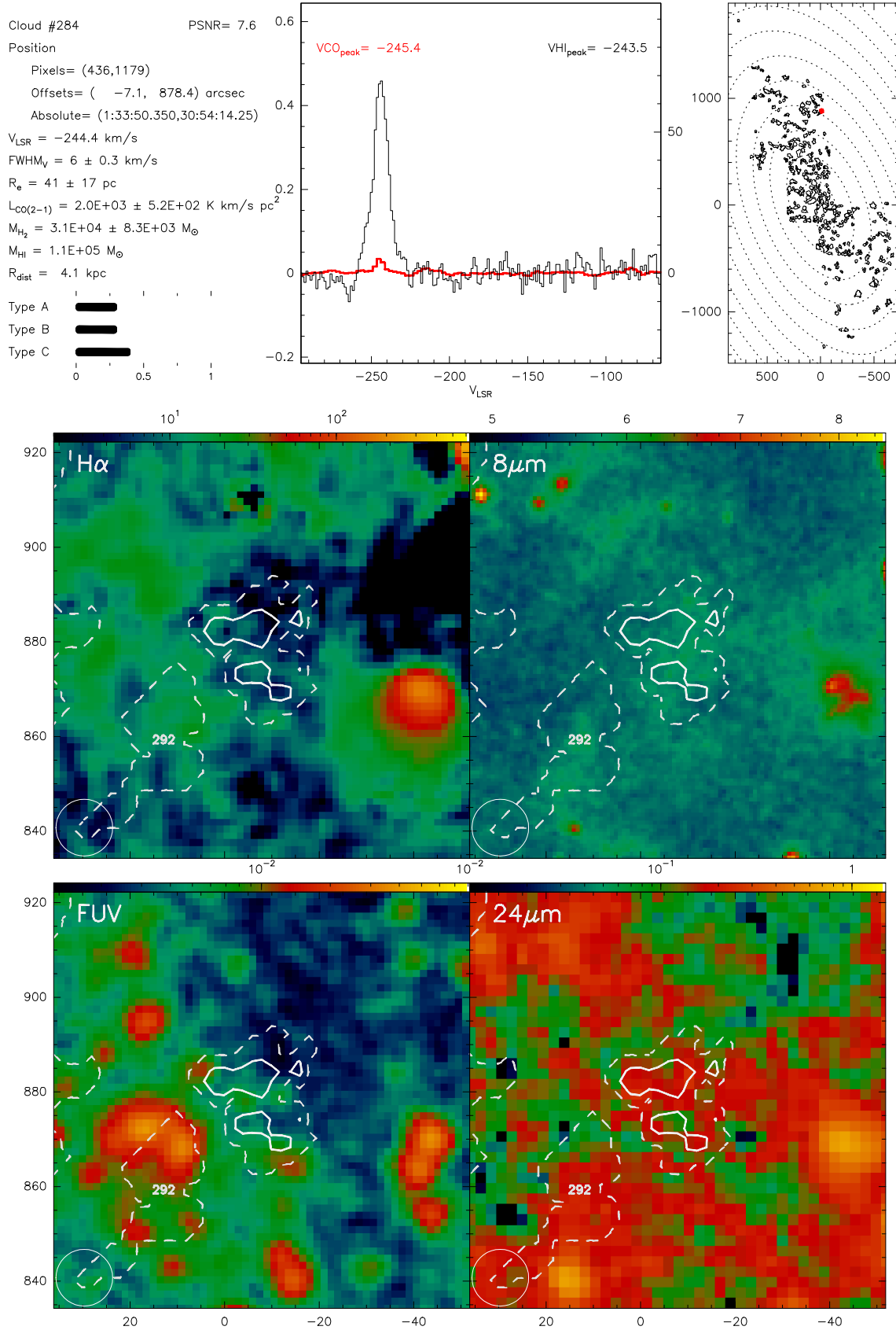
Fig. B.284. Catalogue entry for cloud 284. See description at the beginning of this appendix.
