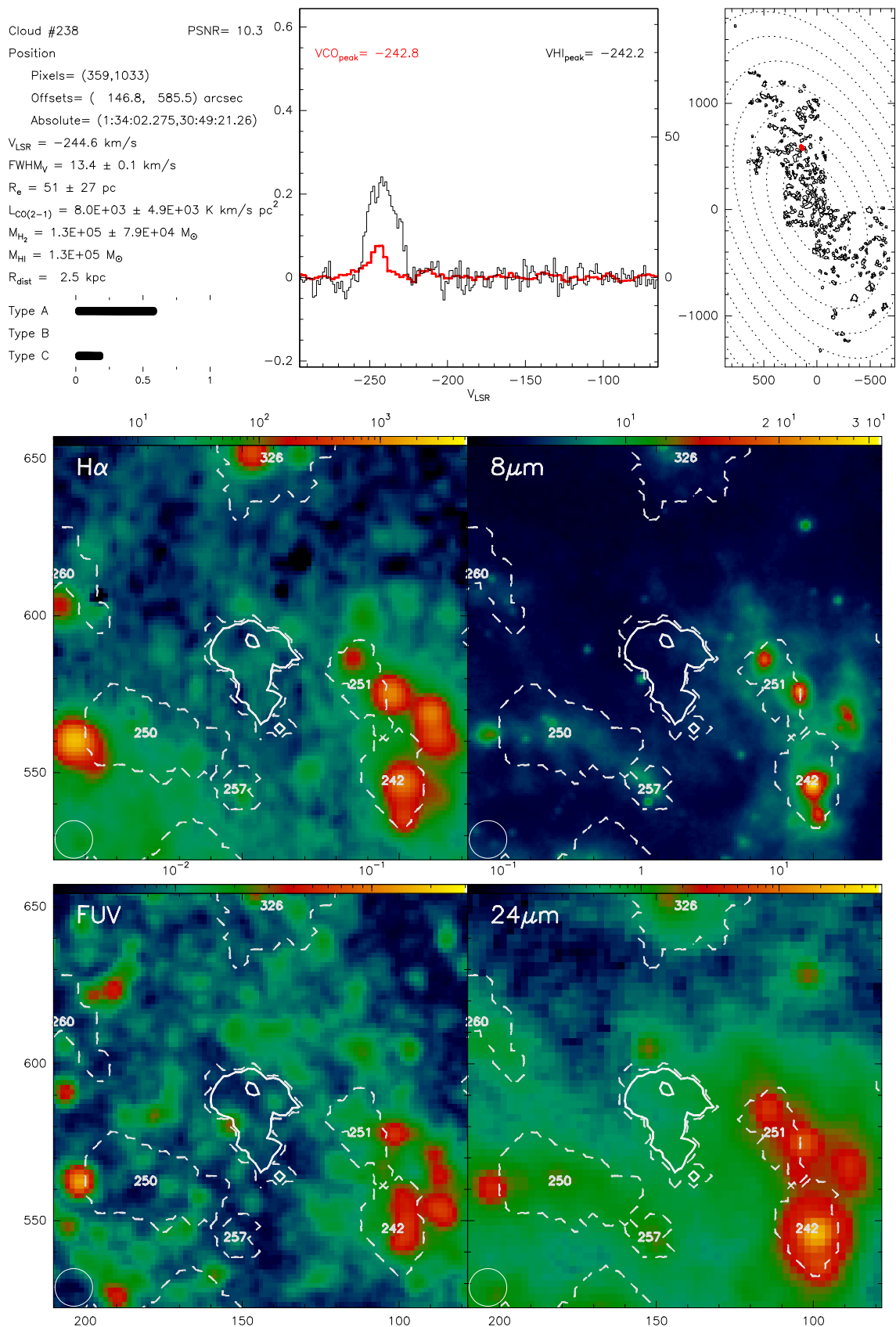
Fig. B.238. Catalogue entry for cloud 238. See description at the beginning of this appendix.
