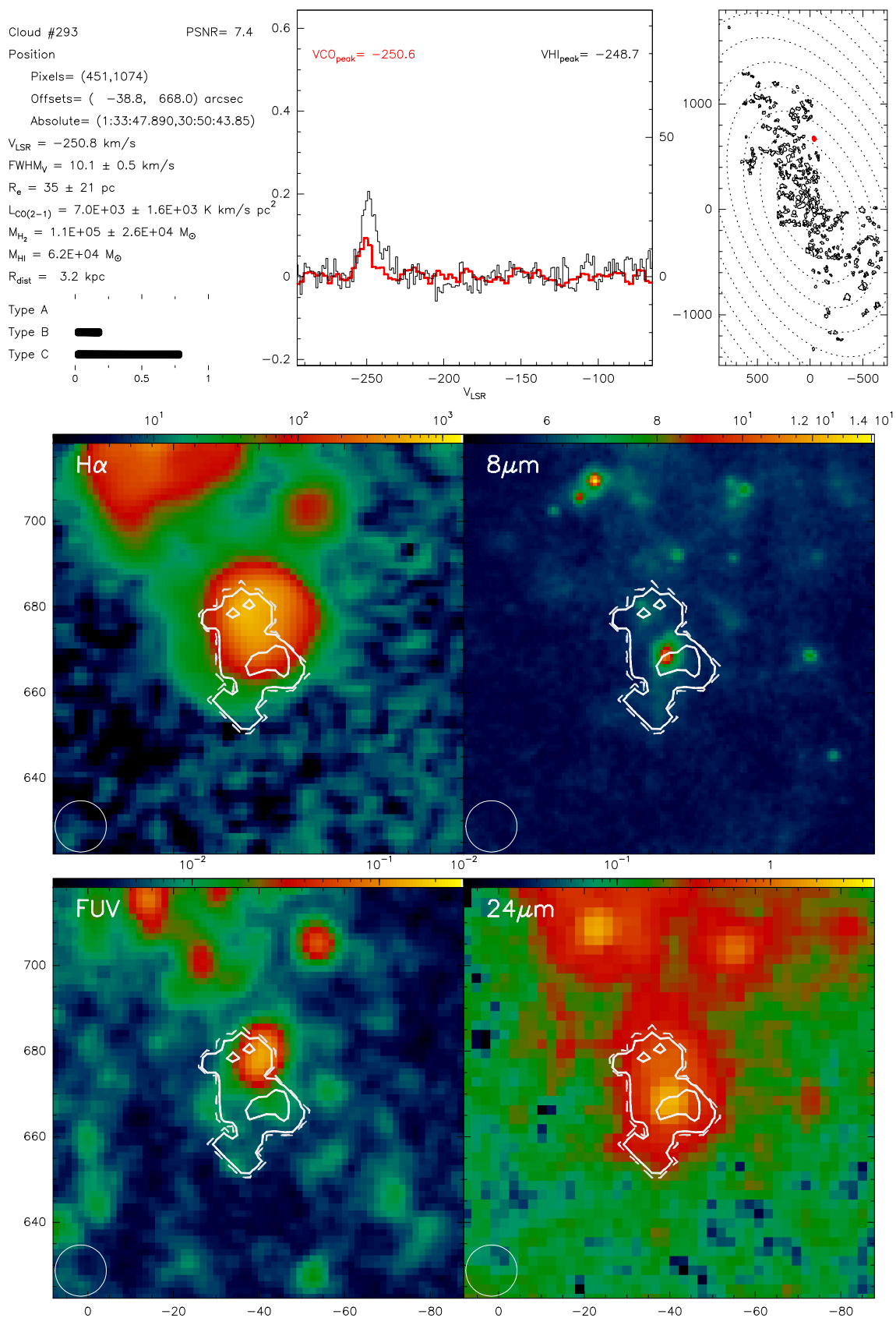
Fig. B.293. Catalogue entry for cloud 293. See description at the beginning of this appendix.
