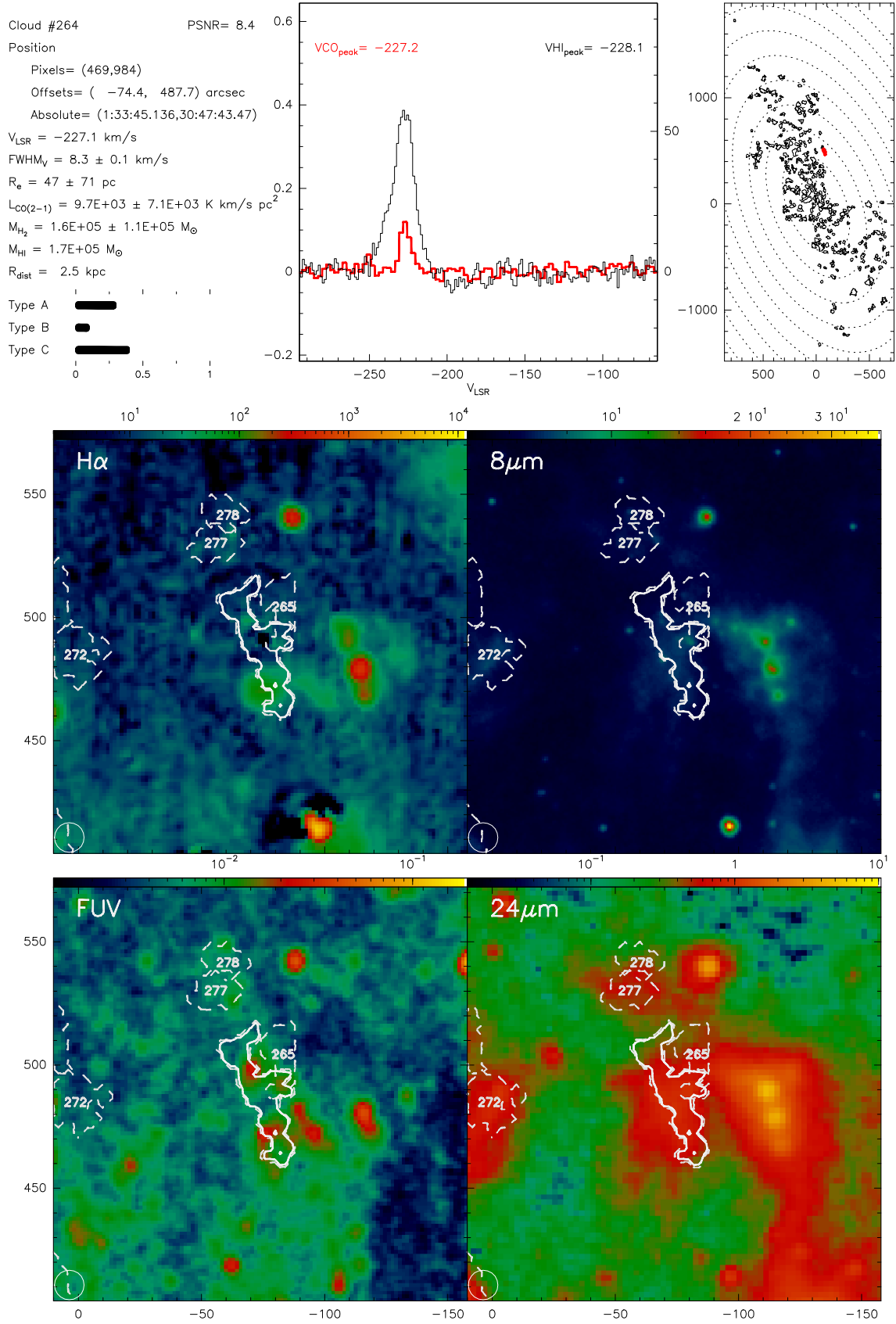
Fig. B.264. Catalogue entry for cloud 264. See description at the beginning of this appendix.
