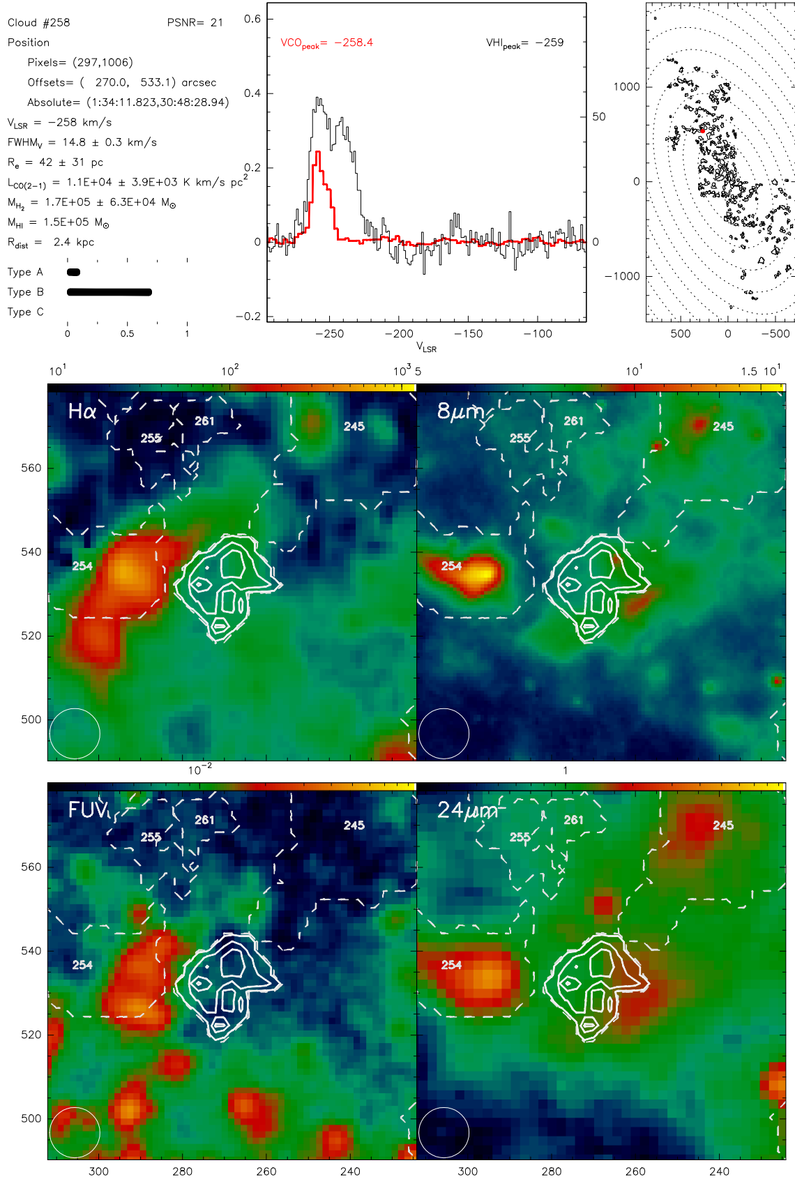
Fig. B.258. Catalogue entry for cloud 258. See description at the beginning of this appendix.
