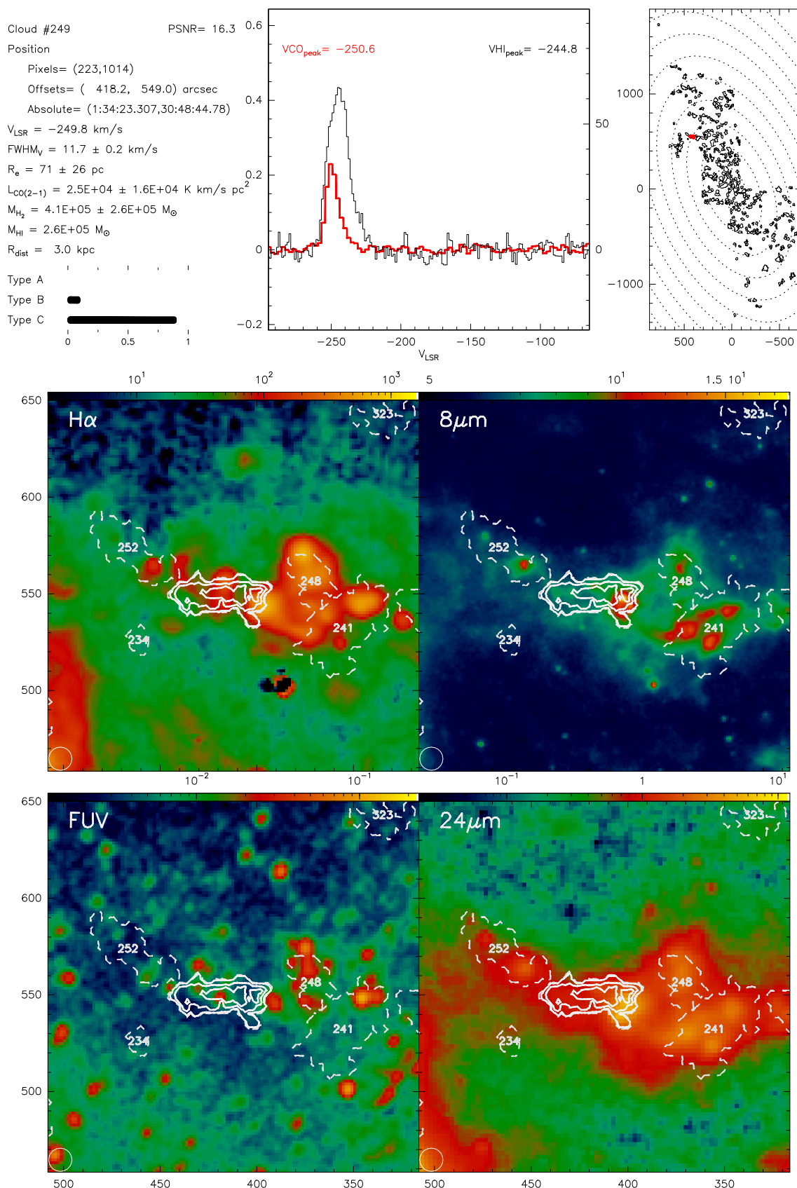
Fig. B.249. Catalogue entry for cloud 249. See description at the beginning of this appendix.
