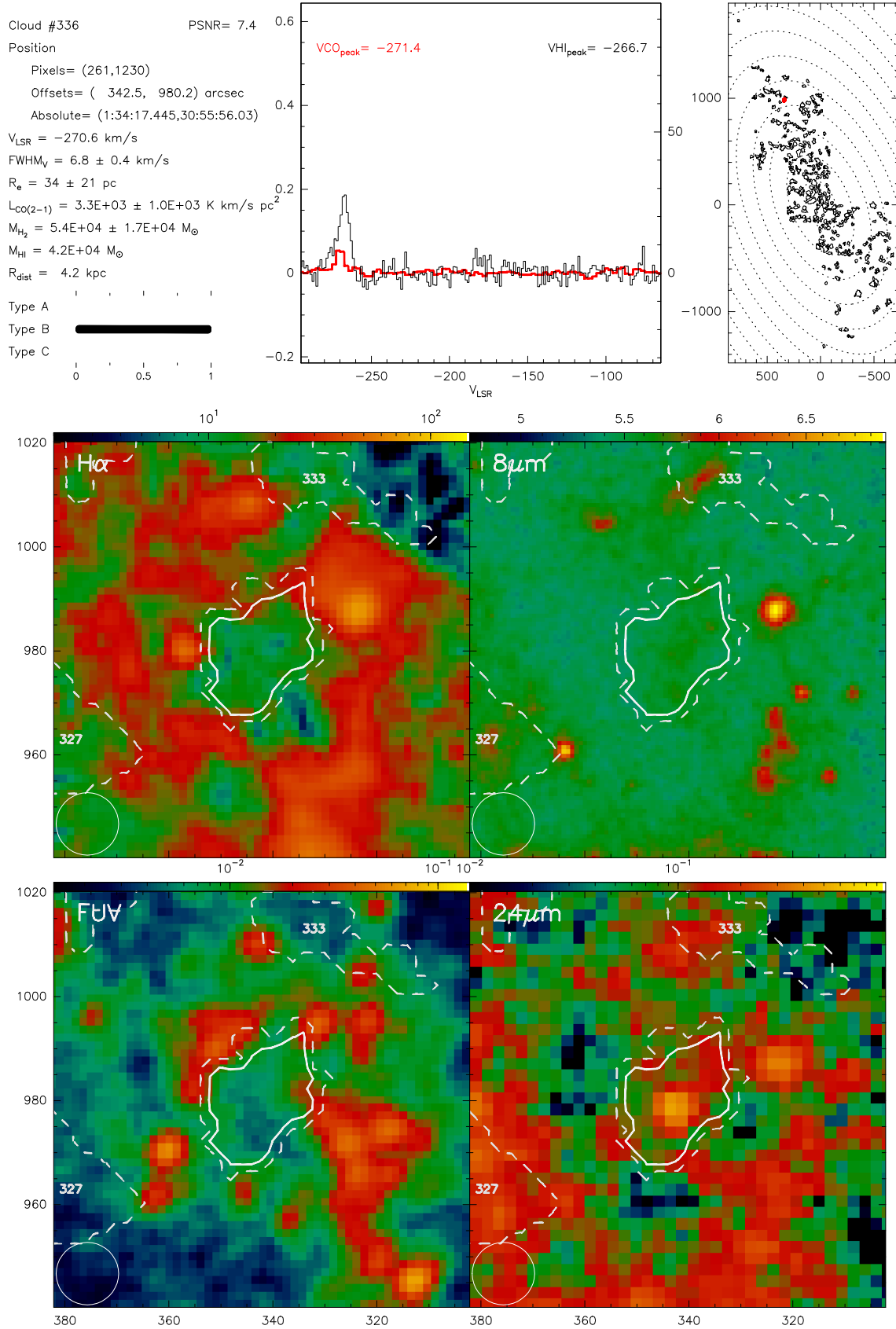
Fig. B.336. Catalogue entry for cloud 336. See description at the beginning of this appendix.
