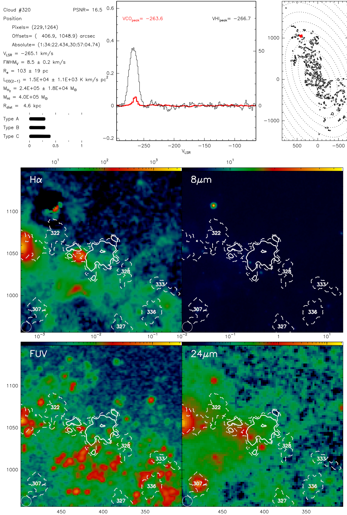
Fig. B.320. Catalogue entry for cloud 320. See description at the beginning of this appendix.
