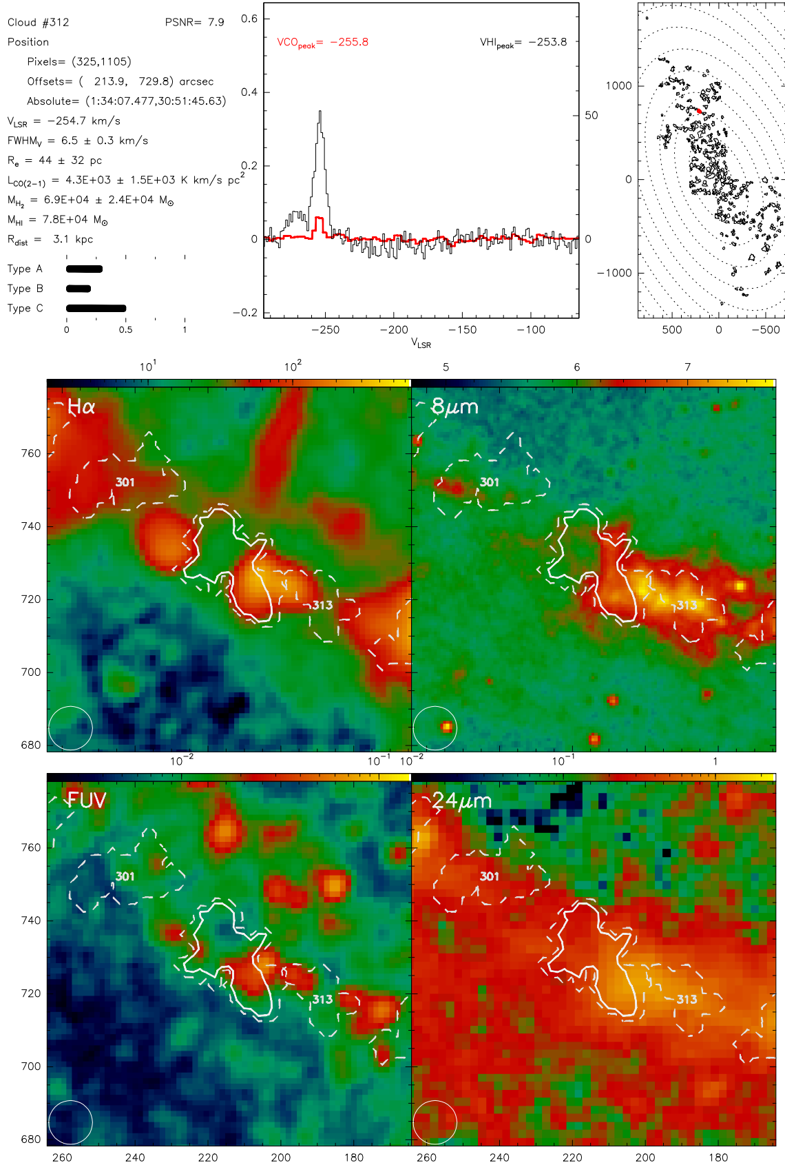
Fig. B.312. Catalogue entry for cloud 312. See description at the beginning of this appendix.
