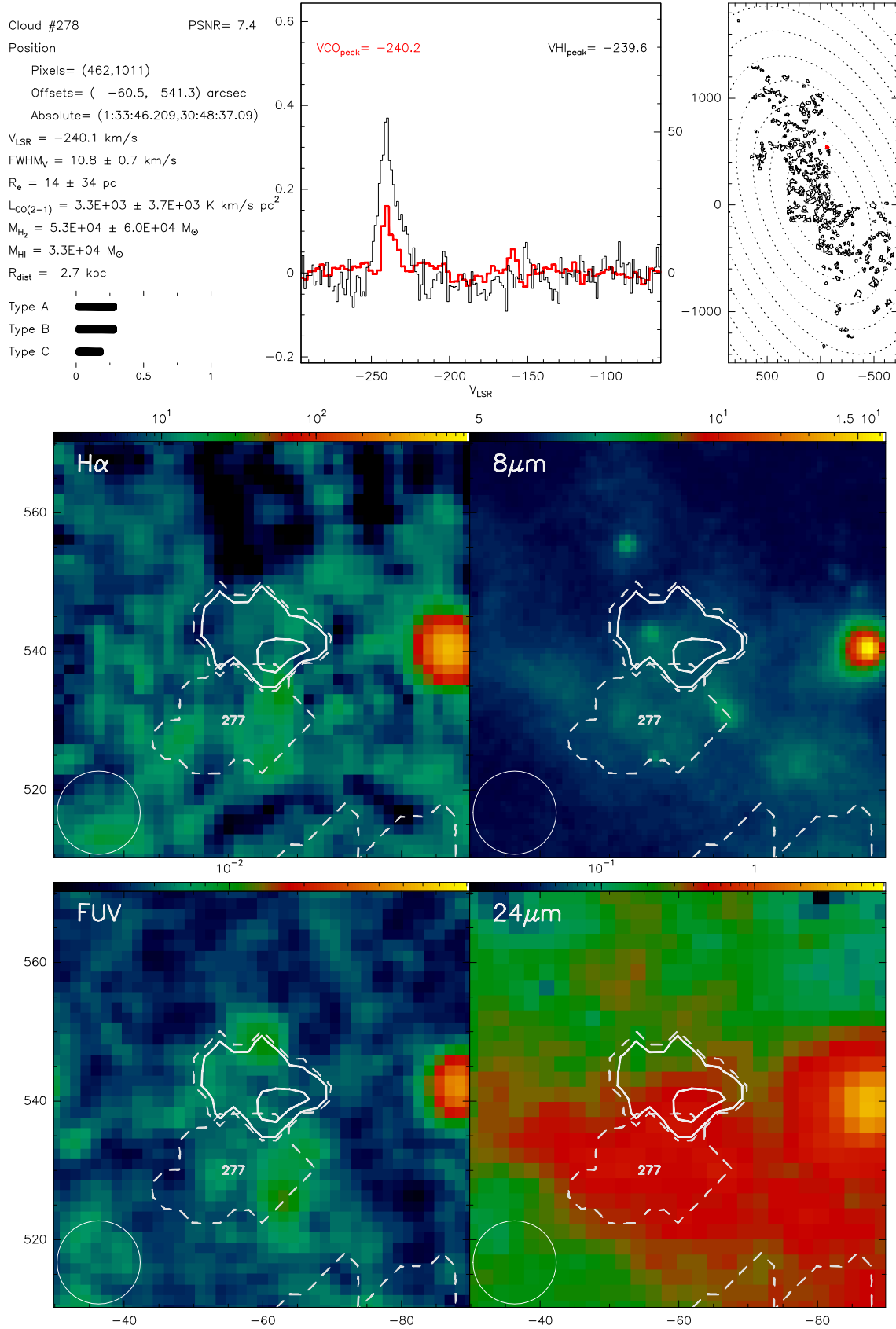
Fig. B.278. Catalogue entry for cloud 278. See description at the beginning of this appendix.
