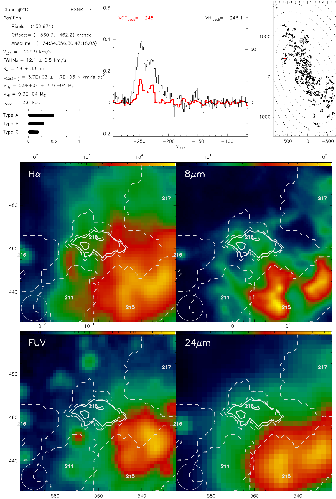
Fig. B.210. Catalogue entry for cloud 210. See description at the beginning of this appendix.
