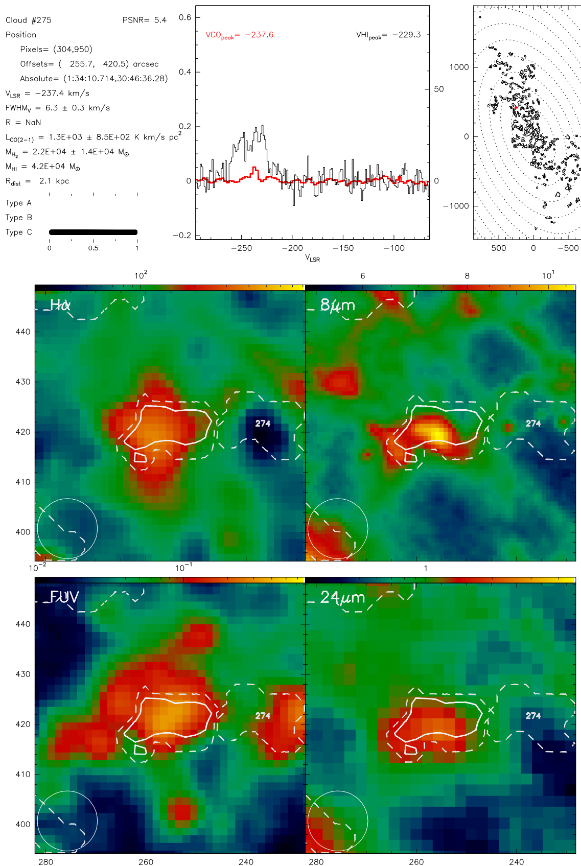
Fig. B.275. Catalogue entry for cloud 275. See description at the beginning of this appendix.
