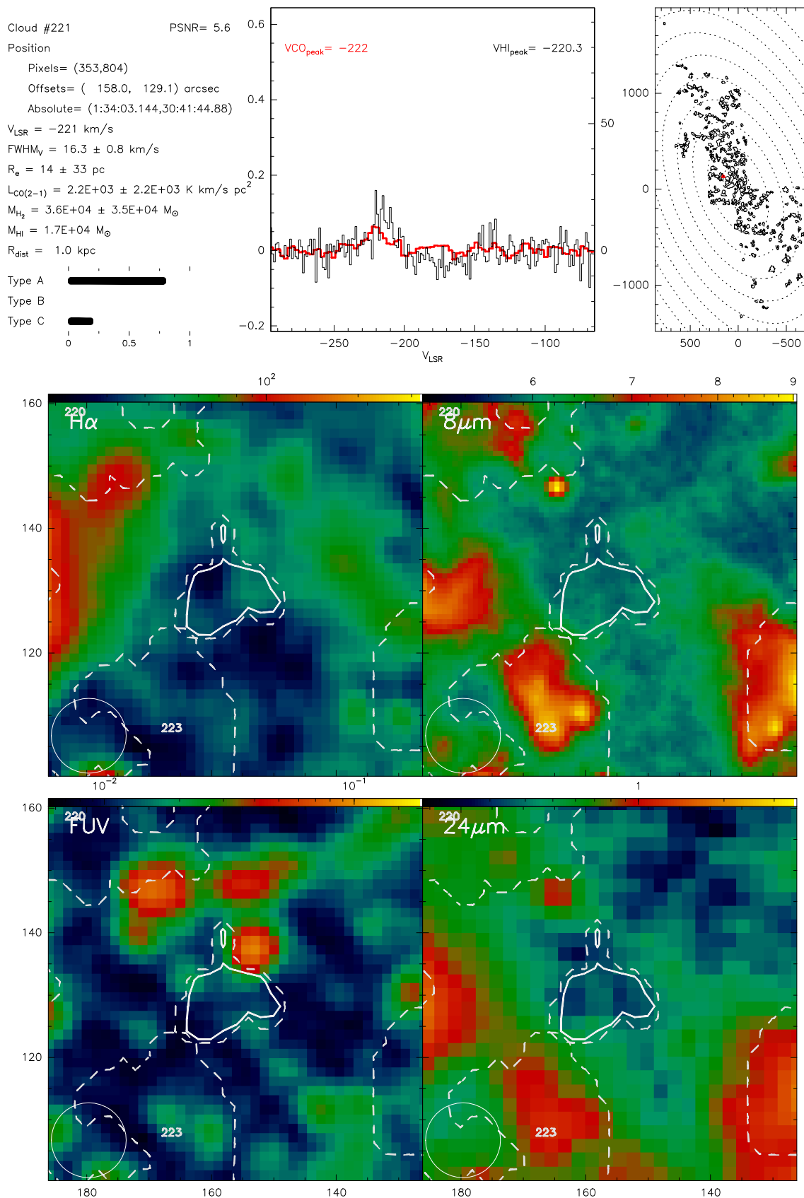
Fig. B.221. Catalogue entry for cloud 221. See description at the beginning of this appendix.
