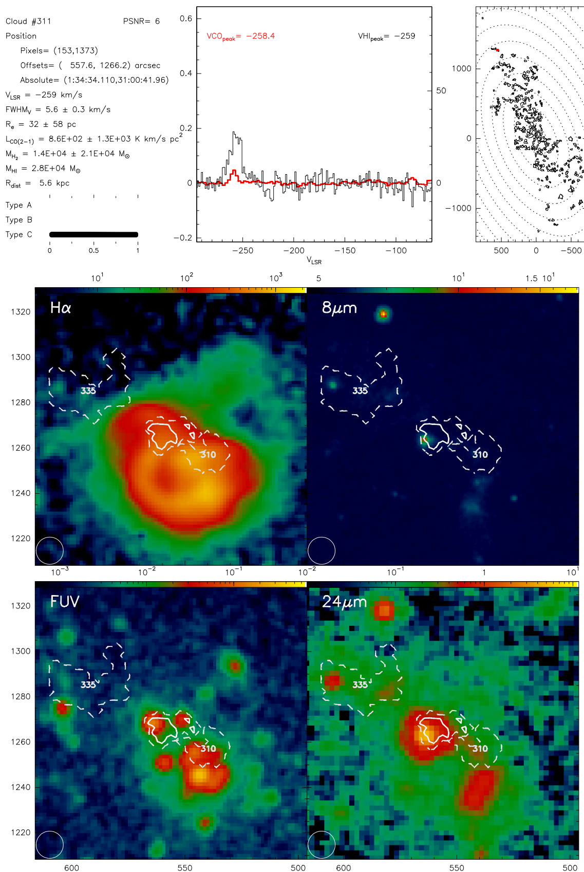
Fig. B.311. Catalogue entry for cloud 311. See description at the beginning of this appendix.
