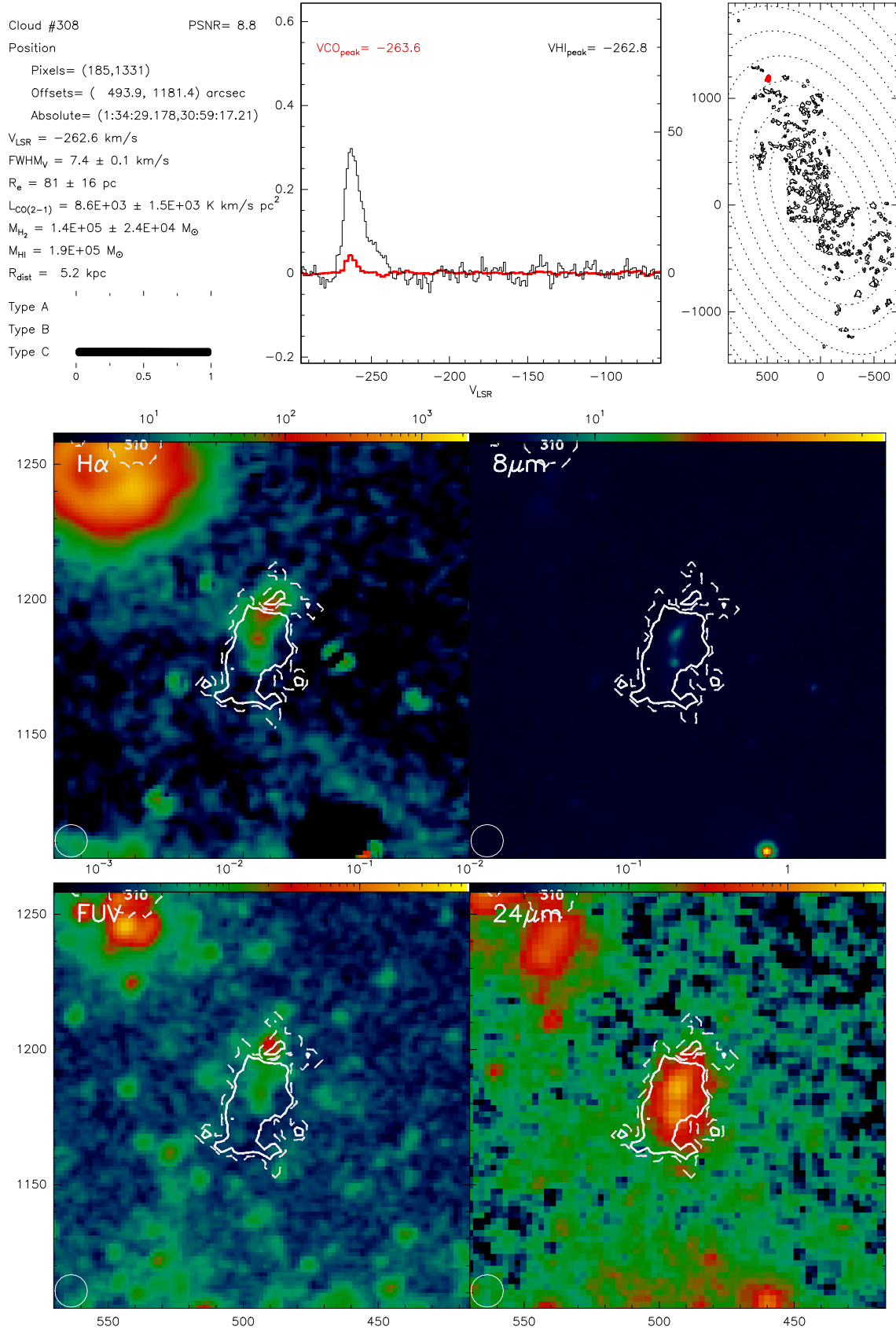
Fig. B.308. Catalogue entry for cloud 308. See description at the beginning of this appendix.
