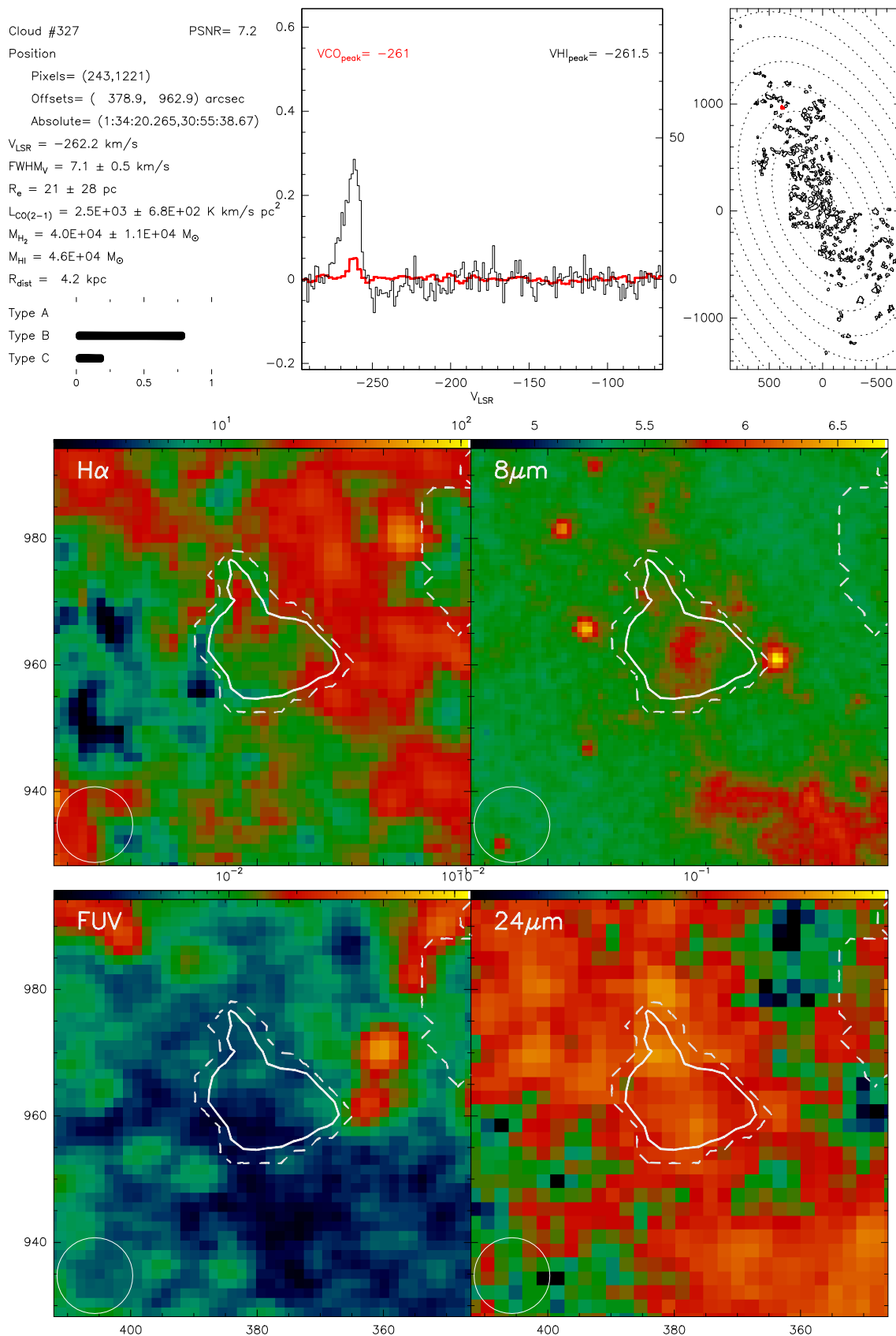
Fig. B.327. Catalogue entry for cloud 327. See description at the beginning of this appendix.
