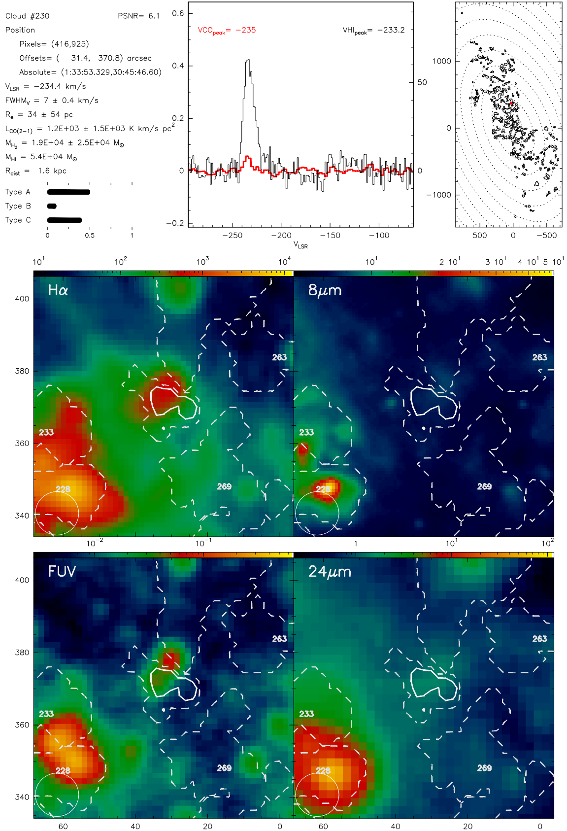
Fig. B.230. Catalogue entry for cloud 230. See description at the beginning of this appendix.
