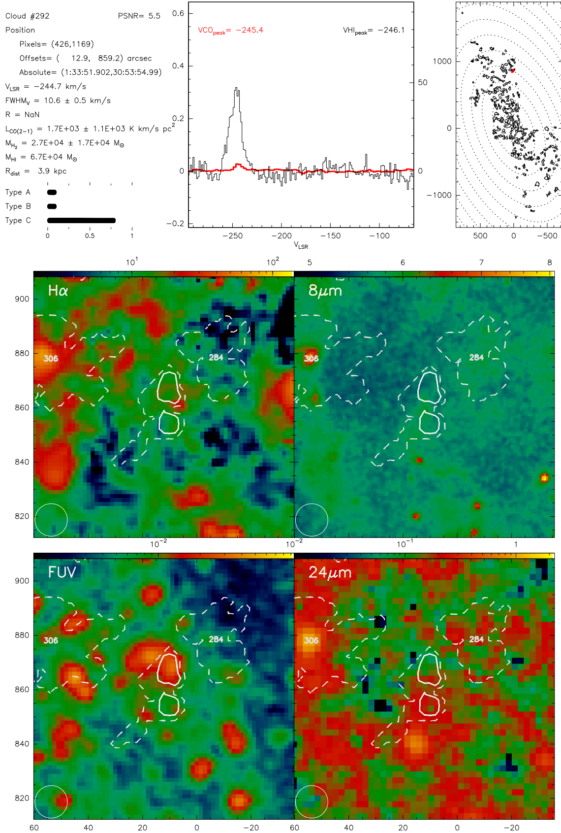
Fig. B.292. Catalogue entry for cloud 292. See description at the beginning of this appendix.
