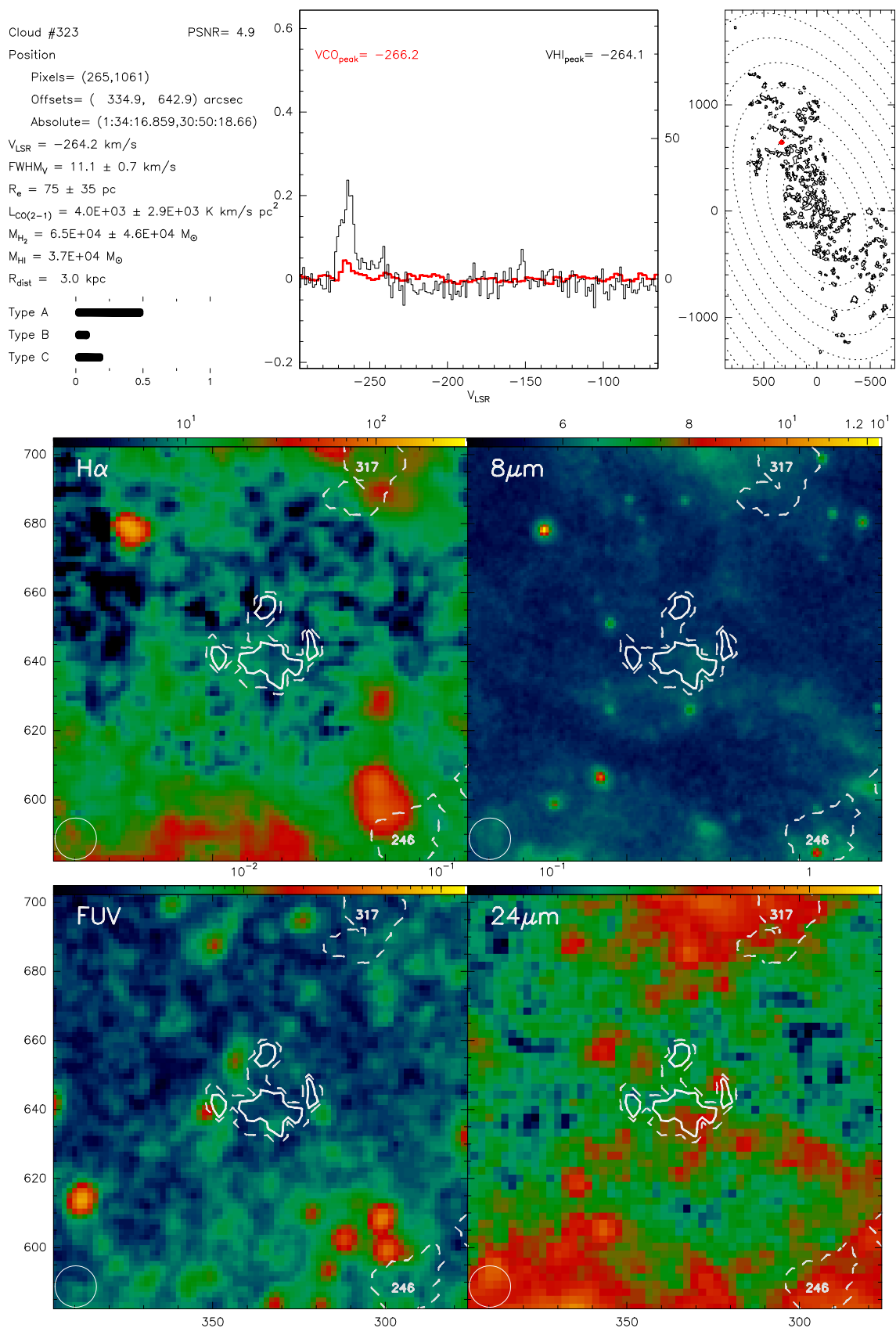
Fig. B.323. Catalogue entry for cloud 323. See description at the beginning of this appendix.
