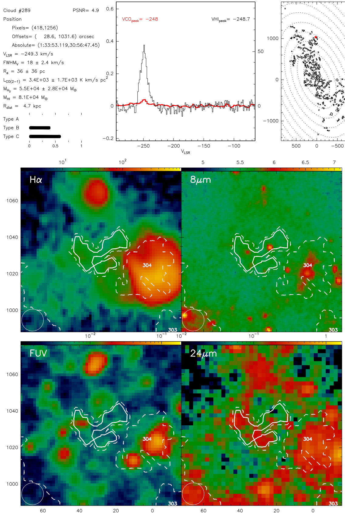
Fig. B.289. Catalogue entry for cloud 289. See description at the beginning of this appendix.
