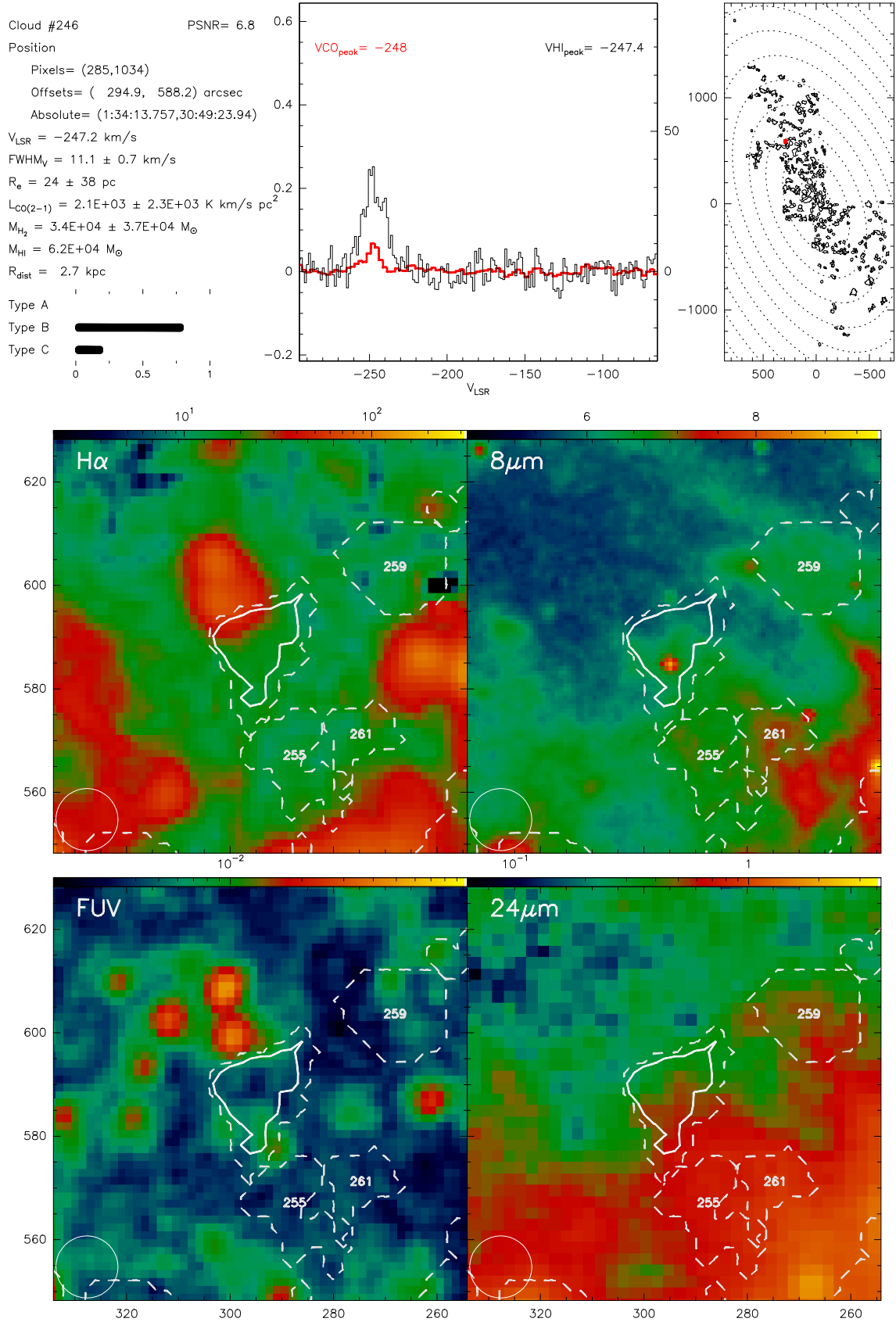
Fig. B.246. Catalogue entry for cloud 246. See description at the beginning of this appendix.
