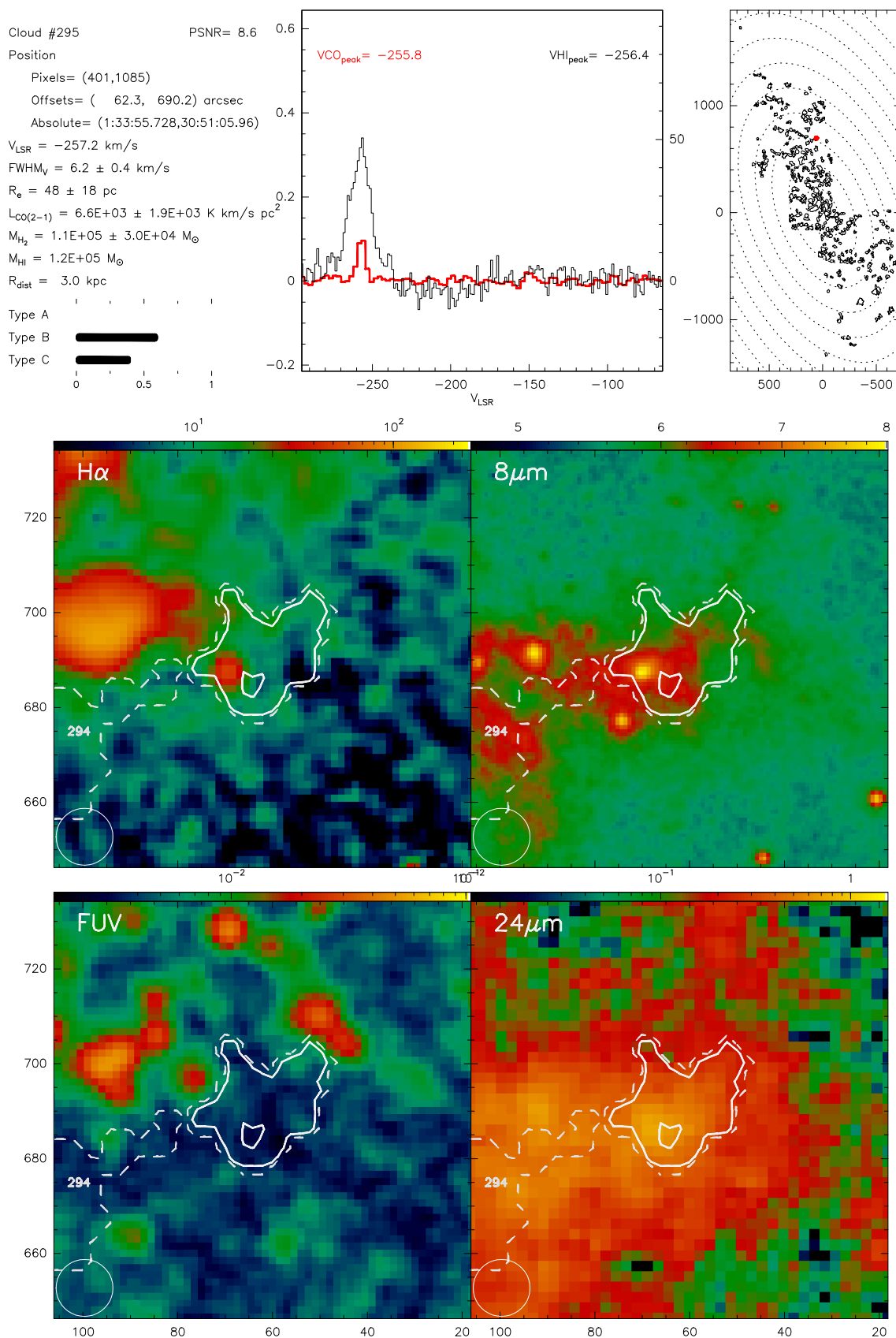
Fig. B.295. Catalogue entry for cloud 295. See description at the beginning of this appendix.
