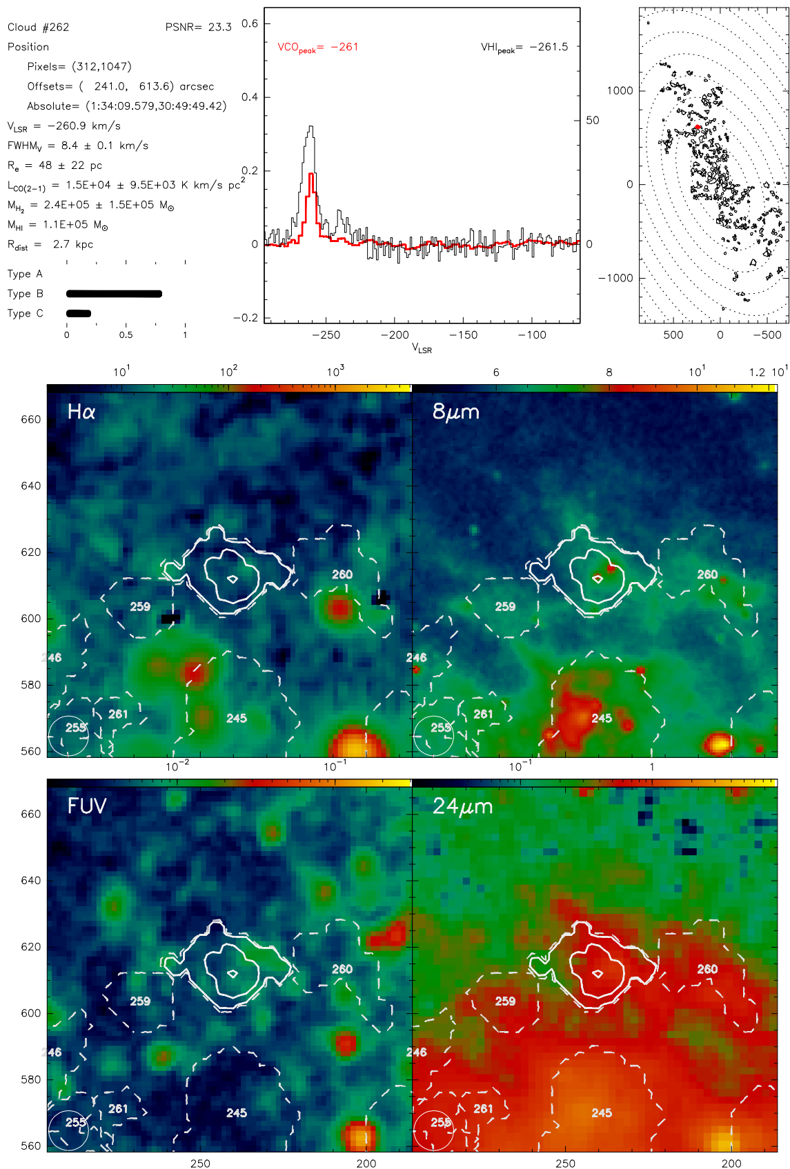
Fig. B.262. Catalogue entry for cloud 262. See description at the beginning of this appendix.
