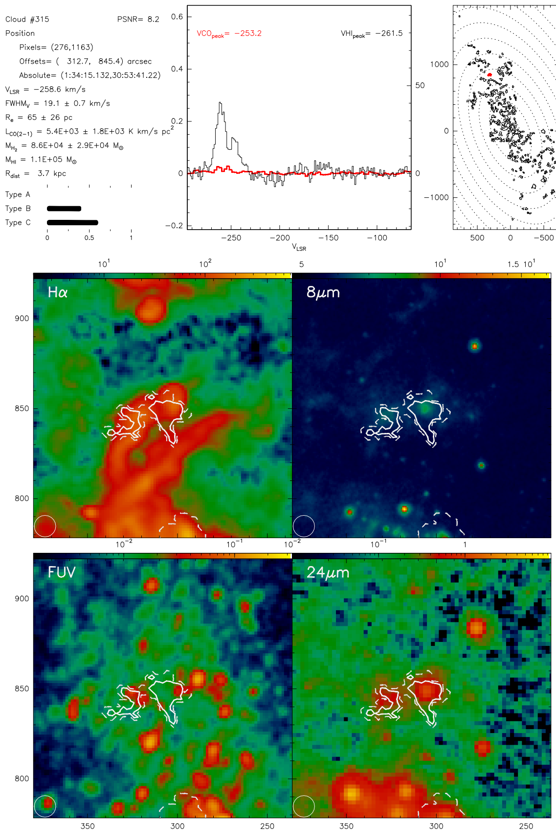
Fig. B.315. Catalogue entry for cloud 315. See description at the beginning of this appendix.
