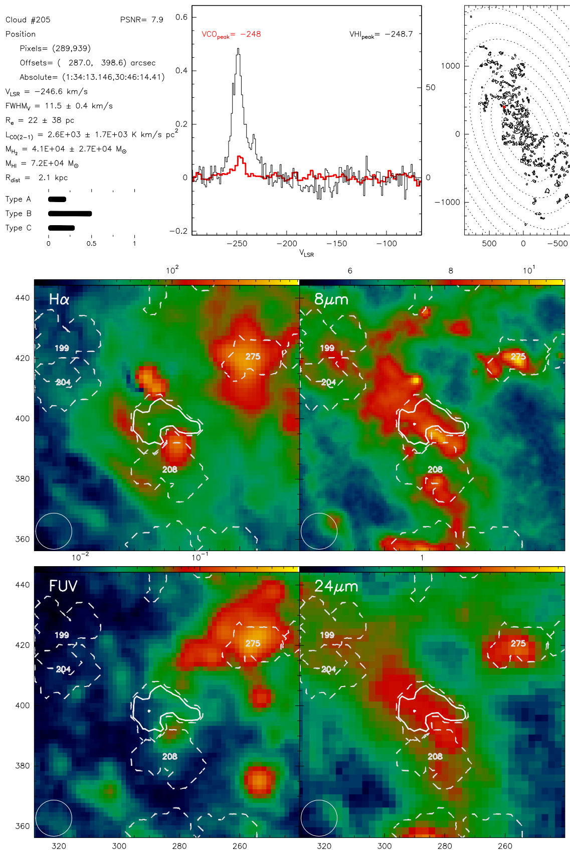
Fig. B.205. Catalogue entry for cloud 205. See description at the beginning of this appendix.
