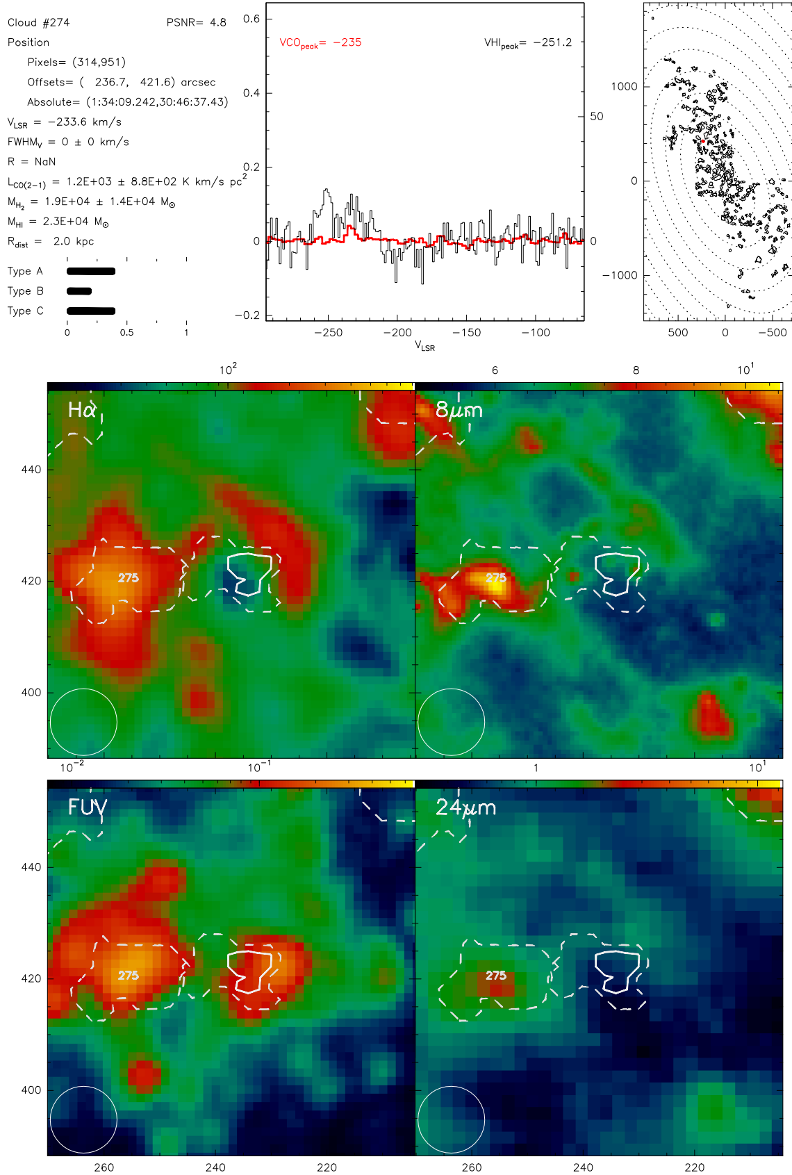
Fig. B.274. Catalogue entry for cloud 274. See description at the beginning of this appendix.
