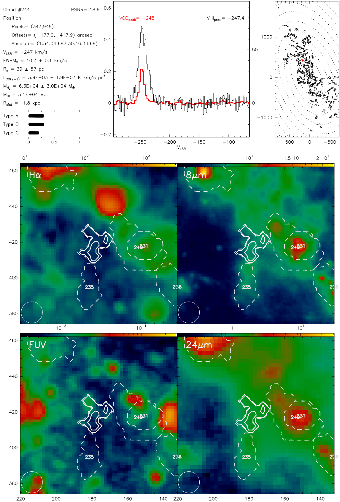
Fig. B.244. Catalogue entry for cloud 244. See description at the beginning of this appendix.
