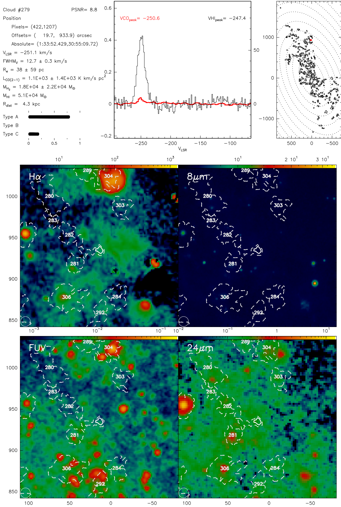
Fig. B.279. Catalogue entry for cloud 279. See description at the beginning of this appendix.
