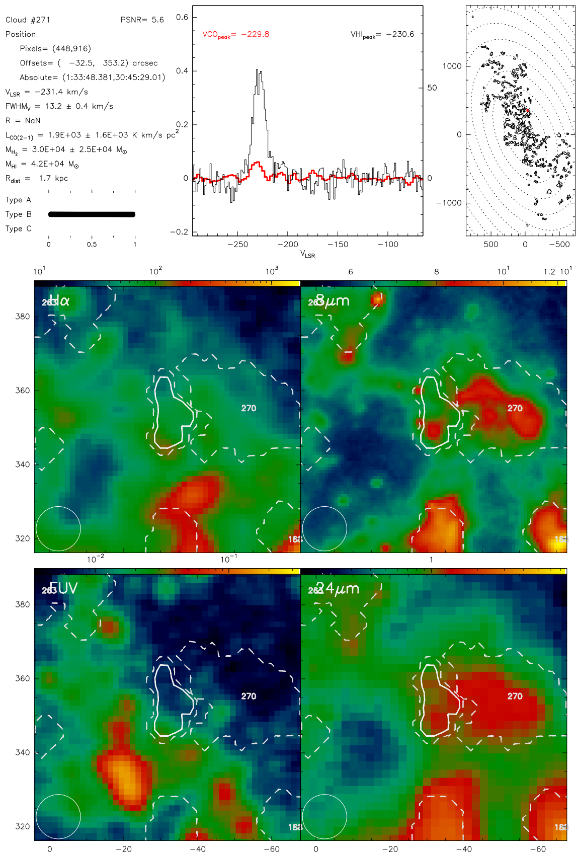
Fig. B.271. Catalogue entry for cloud 271. See description at the beginning of this appendix.
