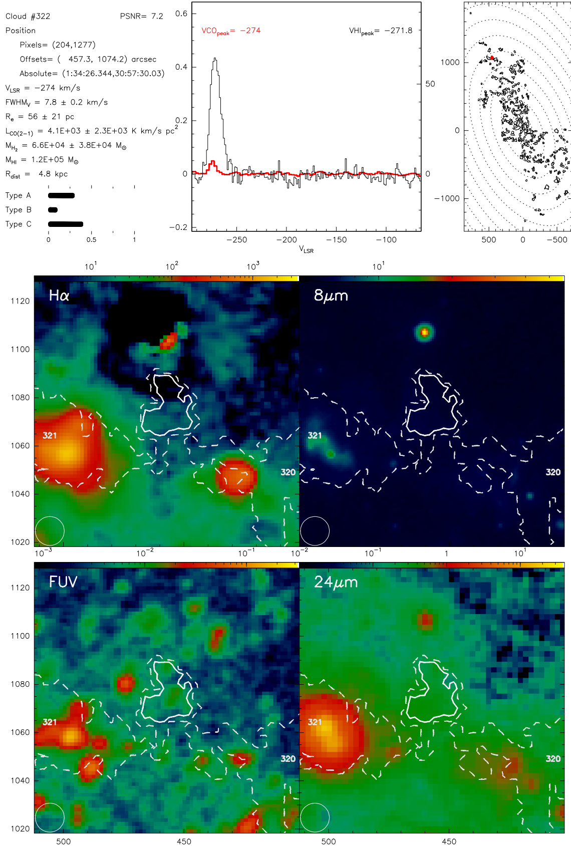
Fig. B.322. Catalogue entry for cloud 322. See description at the beginning of this appendix.
