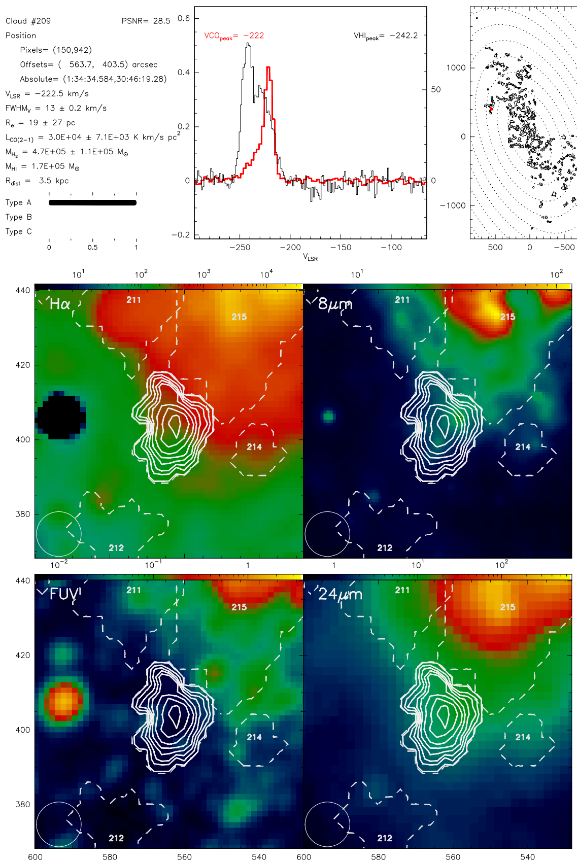
Fig. B.209. Catalogue entry for cloud 209. See description at the beginning of this appendix.
