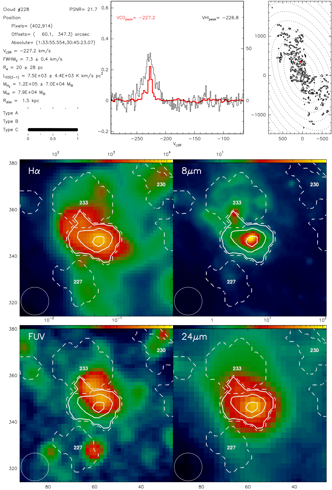
Fig. B.228. Catalogue entry for cloud 228. See description at the beginning of this appendix.
