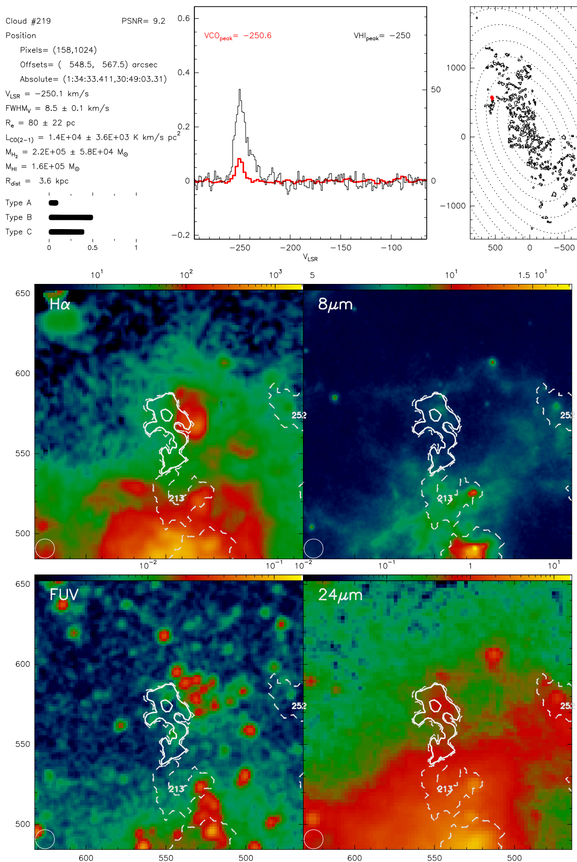
Fig. B.219. Catalogue entry for cloud 219. See description at the beginning of this appendix.
