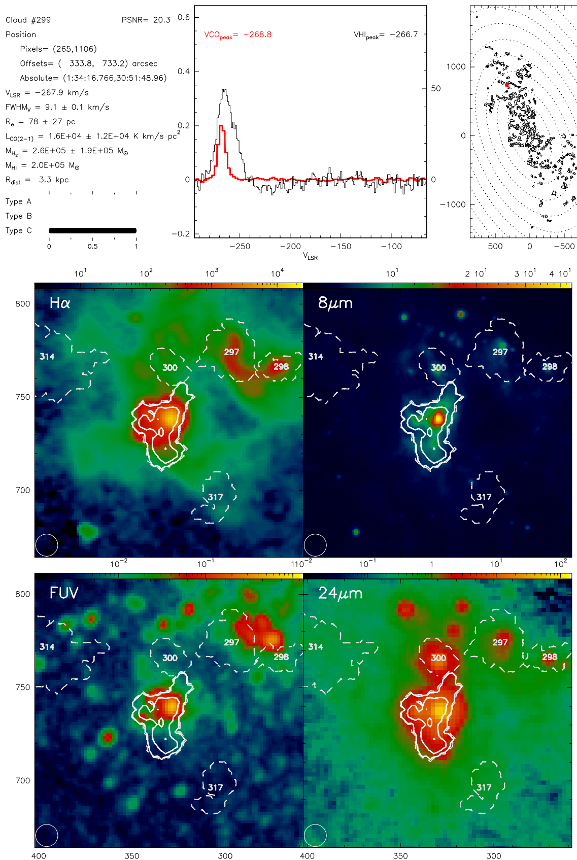
Fig. B.299. Catalogue entry for cloud 299. See description at the beginning of this appendix.
