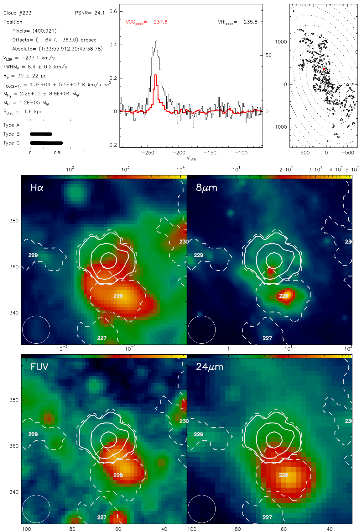
Fig. B.233. Catalogue entry for cloud 233. See description at the beginning of this appendix.
