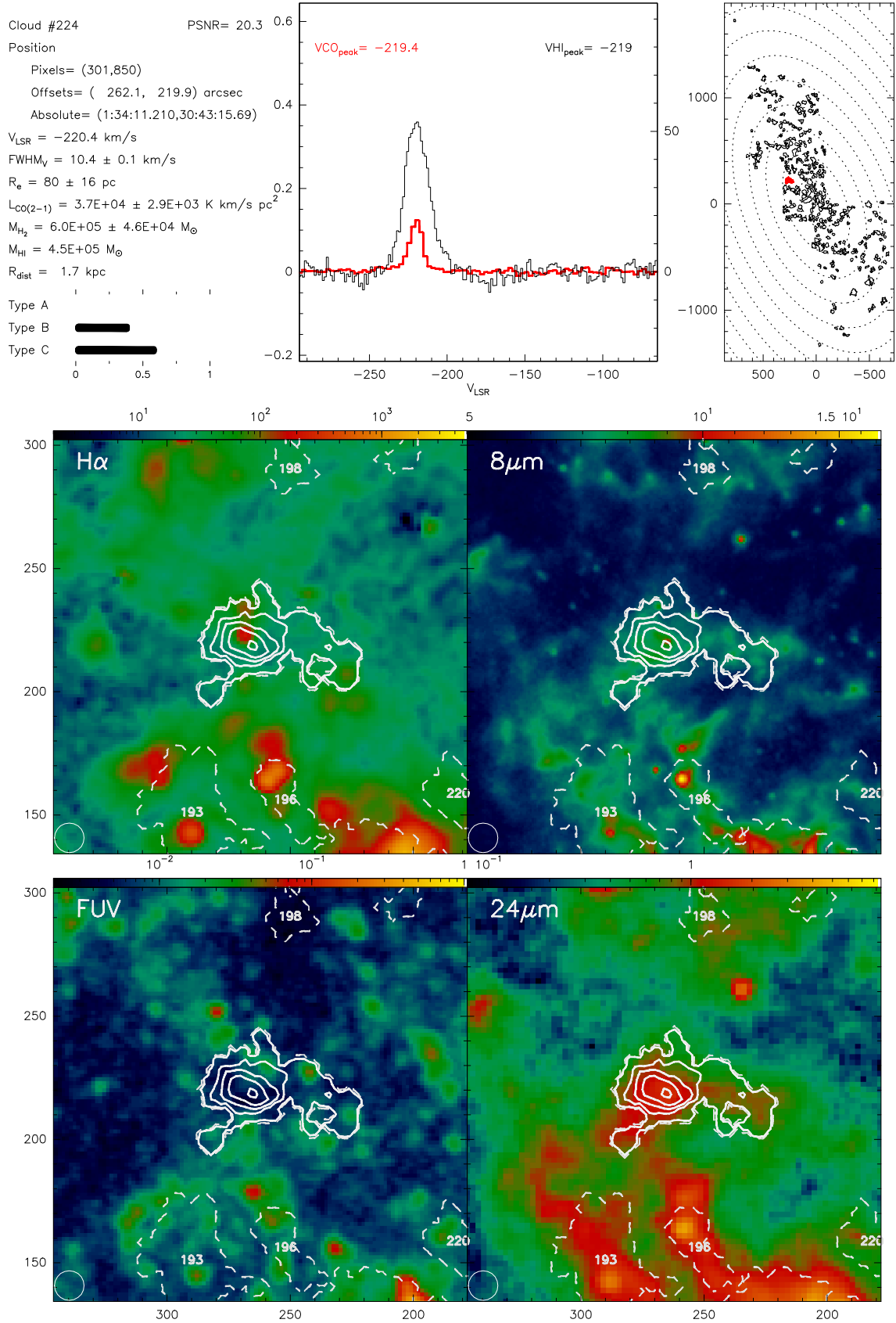
Fig. B.224. Catalogue entry for cloud 224. See description at the beginning of this appendix.
