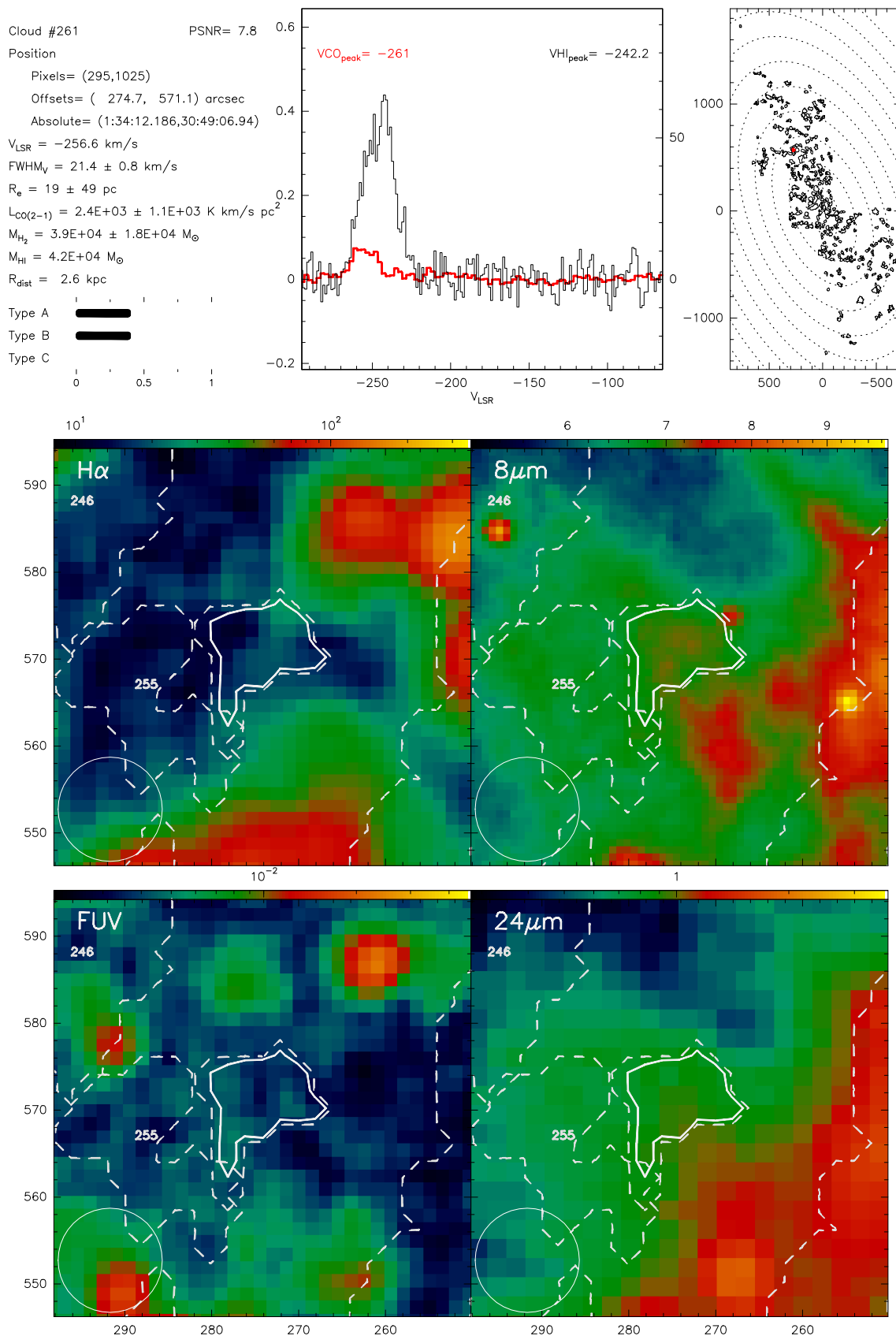
Fig. B.261. Catalogue entry for cloud 261. See description at the beginning of this appendix.
