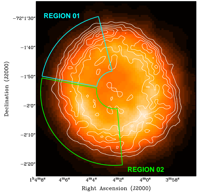
Fig. 1. Contours of the radio image of SNR 0102-72.3 taken at ATCA superimposed on the XMM-Newton EPIC-MOS image (0.2–3.0 keV). For the radio image a combination of data presented by Amy & Ball (1993) and data obtained from additional observations at ATCA is used. The radio contours are 0.1, 0.3, 0.5, 0.7, 0.9, and 1.1 mJy/beam. Regions selected for the spectral analysis of the EPIC-PN data are shown
