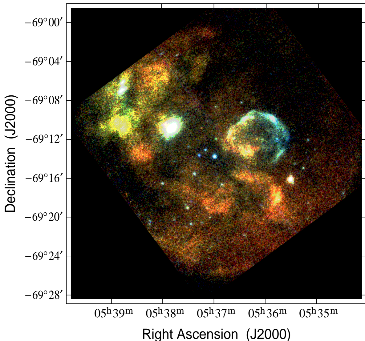
Fig. 5. Final version of the XMM-Newton EPIC pn first light X-ray colour image of the LMC, after applying all the data reductions described in the text
