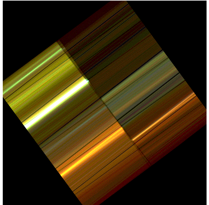
Fig. 3. Out-of-time event image of Fig. 1, constructed by distributing the events recorded in each readout column homogeneously across the column. The intensity of this image was artificially increased with respect to Fig. 1 by a factor of 20 for better visibility of these events
