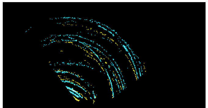
Fig. 4. Single mirror reflections of LMC X-1 in the lower corner of Fig. 1. Pixels affected during the first two observations are marked in yellow, while pixels affected during the last three observations are coded in blue. The correction was done individually for the two sets of observations
