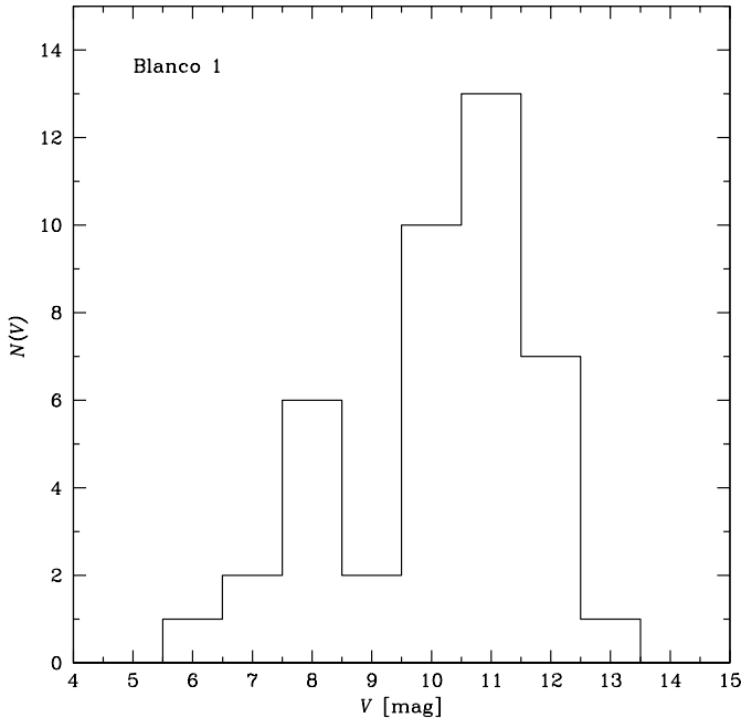
Fig. 8. V_T luminosity function of Blanco 1. Note the dip around V_T = 9 mag
