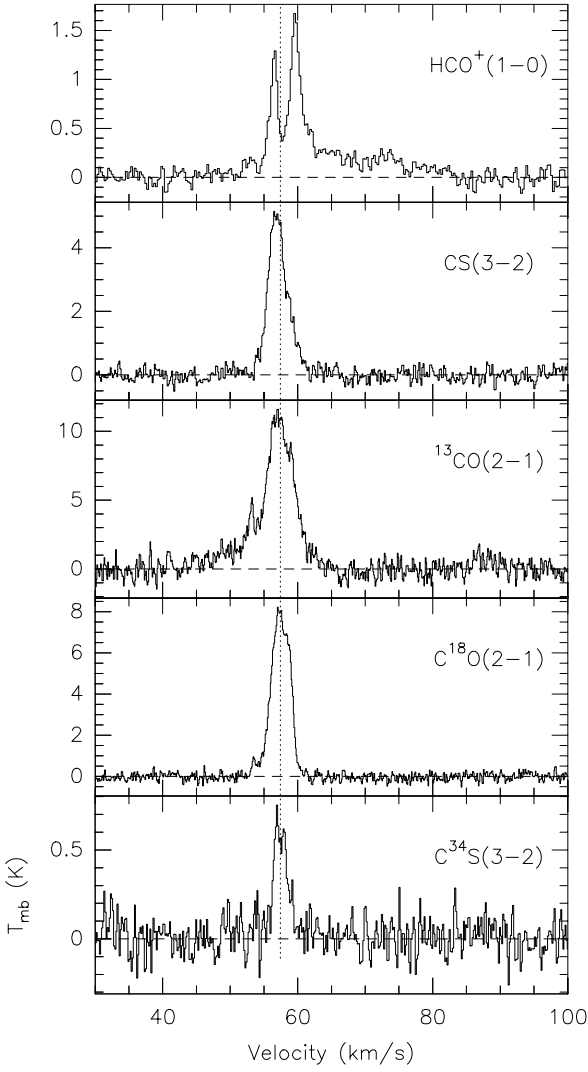
Fig. 1. d) As a), for Mol 75
