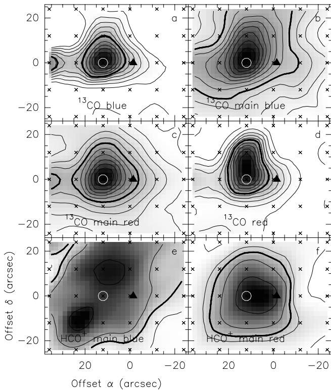
Fig. 13. Mol 59 data. Emission in the ^{13}\text{CO} (top 4 panels) and \text{HCO}^+ (bottom 2 panels) lines, integrated over different velocity intervals: a) 105\text{--}111\text{ km s}^{-1} [lowest contour 0.5, step 1\text{ K km s}^{-1} ]; b) 111\text{--}114.3\text{ km s}^{-1} [ 5.5, 1.5\text{ K km s}^{-1} ]; c) 114.3\text{--}117\text{ km s}^{-1} [ 1.5, 1.5\text{ K km s}^{-1} ]; d) 117\text{--}122\text{ km s}^{-1} [ 0.5, 1\text{ K km s}^{-1} ]; e) 111\text{--}114.3\text{ km s}^{-1} [ 0.5, 0.5\text{ K km s}^{-1} ]; f) 114.3\text{--}117\text{ km s}^{-1} [ 0.5, 0.5\text{ K km s}^{-1} ]. Thick contours in each panel indicate the half-maximum level. The IRAS position is indicated by the triangle, the white circle is the position where longer integrations were made. Small crosses are the observed positions
