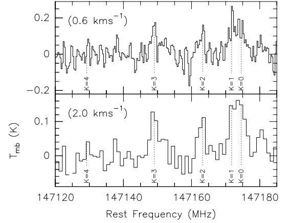
Fig. 4. Spectra of the \text{CH}_3\text{CN}(8-7) rotational transition towards the peak position ( 24'', 0'' ) in Mol 98. The velocity resolution of the spectra is indicated in the panels. The location of the first few K-components are indicated in the spectra
