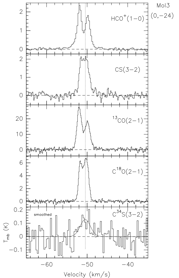
Fig. 1. a) Spectra towards the peak position in the maps for Mol 3. Source name, offset position, and molecules/transitions are indicated. The offset is relative to the maps’ central position, which is the sub-mm peak (Molinari et al. 2000). The main beam brightness temperature ( T_{mb} ) is plotted against V_{lsr} . The vertical dotted line indicates the V_{lsr} of the C^{34}S(3-2) line, obtained from a Gaussian fit; the horizontal dashed lines indicate the T_{mb} = 0 K level in each spectrum
