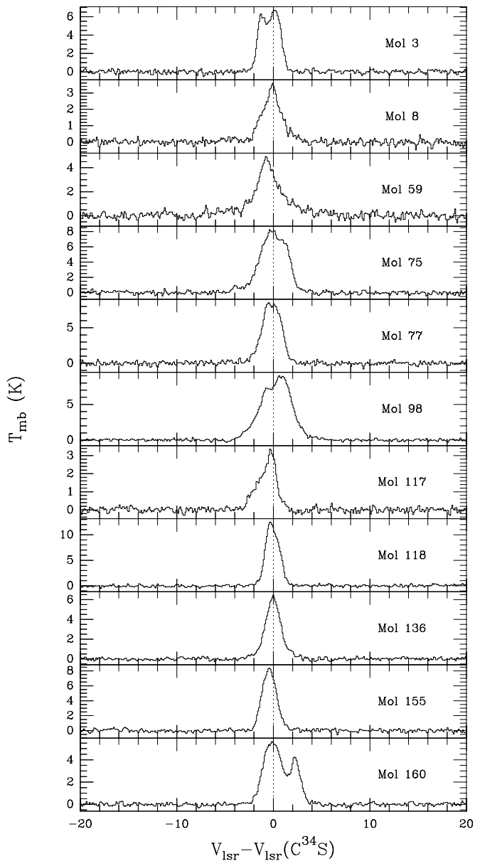
Fig. 6. d) As a) but for the C 18 O(2–1) spectra
