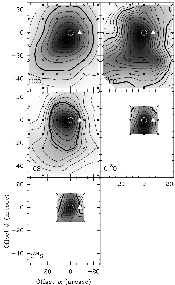
Fig. 5. k) Same as a), for Mol 160. Contour values (low (step) high, in \text{Kkm s}^{-1} ) are: 3(2)18 ( \text{HCO}^+ ); 31(6)110 ( ^{13}\text{CO} ); 0.5(2)22.5 (CS); 5(2)19 ( \text{C}^{18}\text{O} ); 0.3(0.3)3 ( \text{C}^{34}\text{S} )
