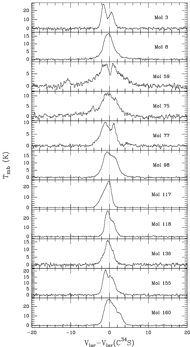
Fig. 6. a) Spectra of the ^{13}\text{CO}(2-1) emission towards the peak position in each source (as indicated in Fig. 1). The velocity is indicated with respect to that of the \text{C}^{34}\text{S}(3-2) line, taken to represent the velocity of the bulk of the high-density gas
