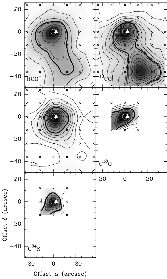
Fig. 5. b) Same as a), for Mol 8. Contour values (low (step) high, in \text{Kkm s}^{-1} ) are: 0.5(1)6.5 ( \text{HCO}^+ ); 4.5(4)60.5 ( ^{13}\text{CO} ); 0.5(1)11 (CS); 1(1)8 ( \text{C}^{18}\text{O} ); 0.4(0.4)2 ( \text{C}^{34}\text{S} )
