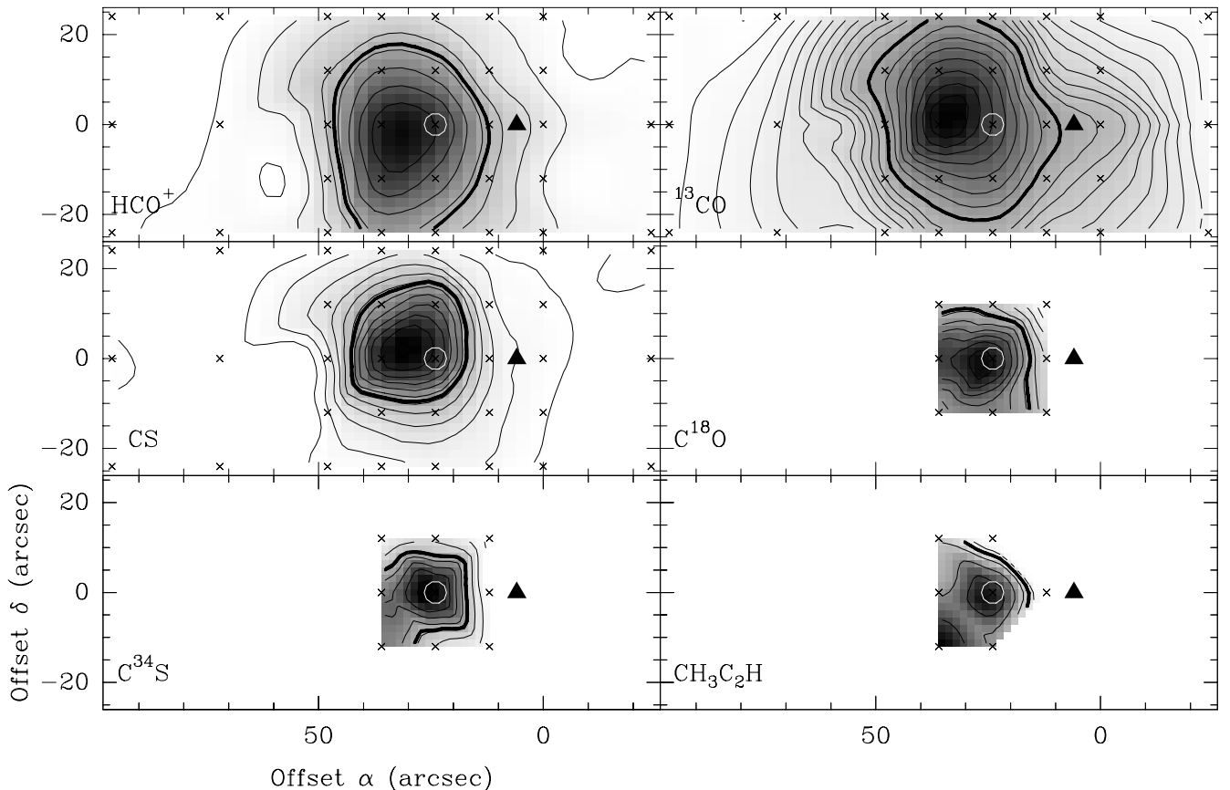
Fig. 5. f) Same as a) , for Mol 98. Added here is a panel showing the distribution of the integrated emission over the K = 0, 1 components of \text{CH}_3\text{C}_2\text{H}(6-5) . Contour values (low (step) high, in \text{K km s}^{-1} ) are: 1(2)17 ( \text{HCO}^+ ); 1(4)41(6)95 ( ^{13}\text{CO} ); 1(2)23 (CS); 3(3)35 ( \text{C}^{18}\text{O} ); 0.5(0.5)4 ( \text{C}^{34}\text{S} ); 1(0.5)3.5 ( \text{CH}_3\text{C}_2\text{H} )
