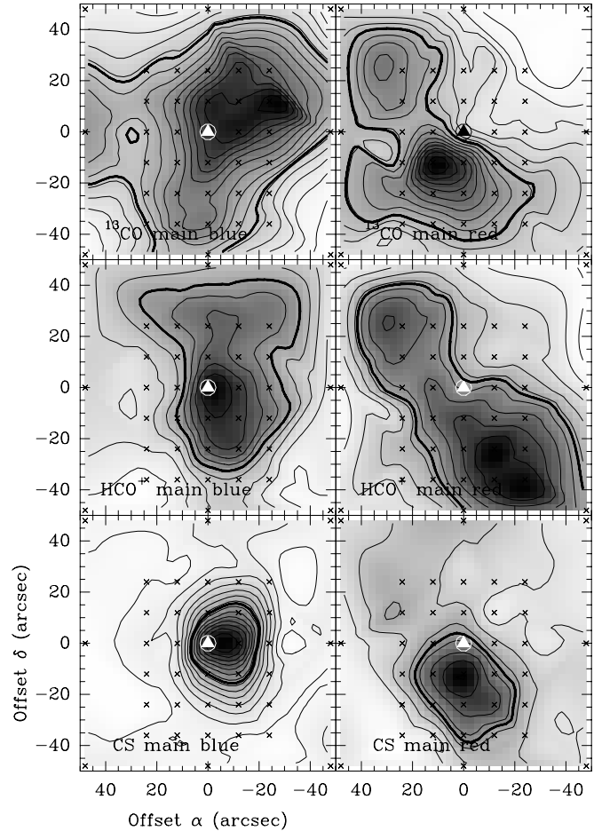
Fig. 14. Mol 75 data. Emission in the ^{13}\text{CO} (top 2 panels), \text{HCO}^+ (middle 2 panels), and CS (bottom 2 panels) lines, integrated over the blue and red parts of the emission (see text). Thick contours in each panel indicate the half-maximum level. The IRAS position is indicated by the triangle, the white circle is the position where longer integrations were made. Small crosses are the observed positions. Contours: ^{13}\text{CO} blue 8(2)37\text{ K km s}^{-1} , red 4(2)36 ; \text{HCO}^+ blue 0.2(0.2)2 , red 0.2(0.8)7.4 ; CS blue 1(1)15 , red 1(1)7
