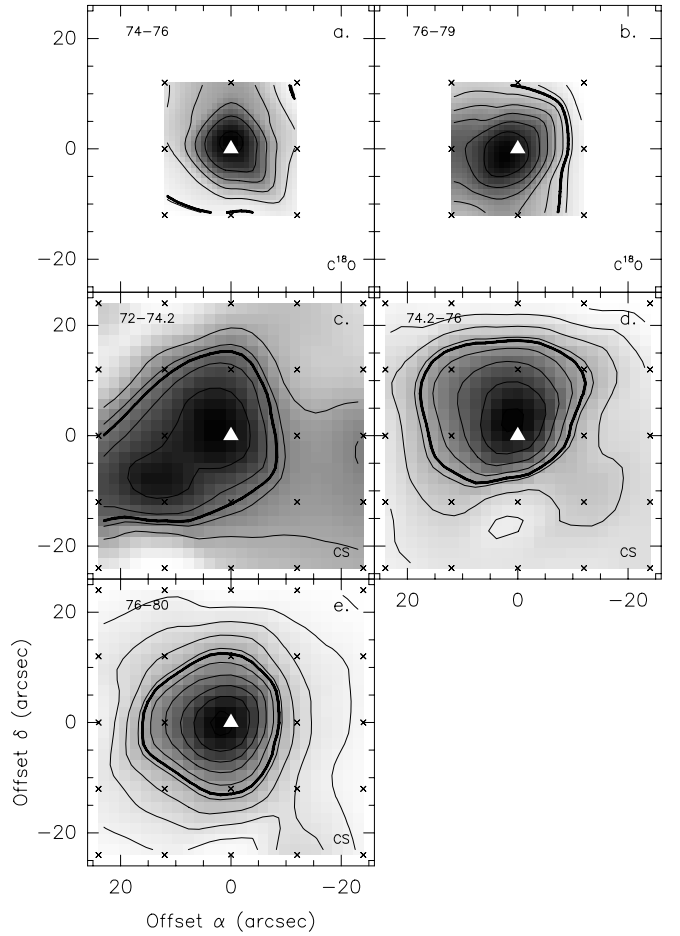
Fig. 16. c) As a) but for \text{C}^{18}\text{O} (panels a, b) and CS (panels c-e)). Contours: 5(1)10 \text{ K km s}^{-1} (panel a); 3(1)11 b); 0.2(0.2)1 c); 0.2(0.4)3.4 d); 0.2(0.4)4 e)
