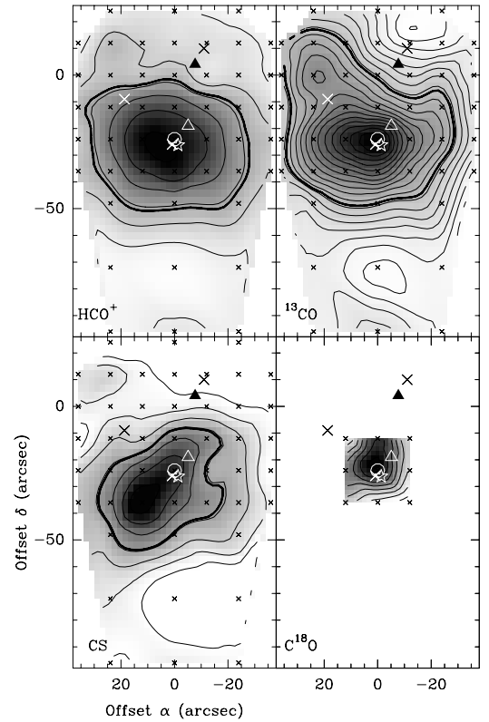
Fig. 5. Maps towards all sources of the integrated emission in the lines of \text{HCO}^+(1-0) , ^{13}\text{CO}(2-1) , \text{CS}(3-2) , and \text{C}^{18}\text{O}(2-1) . Where \text{C}^{34}\text{S}(3-2) was strong enough, a panel with a map of that molecule is shown as well. Thick contours indicate the 50% level in each map. The (0,0) position is the position of the sub-mm peak (Molinari et al. 2000). The small crosses mark the observed positions, the filled triangle indicates the IRAS point source position, and the circle marks the position where we made longer integrations at the frequency of the \text{CH}_3\text{C}_2\text{H}(6-5) and \text{CH}_3\text{CN} lines. a) Data for Mol 3. The open triangle is the peak of the 850 \mu\text{m} emission, while the star indicates the position of the \text{H}_2\text{O} maser (Jenness et al. 1995). The big crosses indicate the positions of the peaks of the radio continuum emission (VLA D-array, 3.6 cm; Molinari et al., in preparation). For details, see Sect. 5. Contour values (low(step)high, in \text{K km s}^{-1} ) are: 0.5(1)6.5 ( \text{HCO}^+ ); 13(3)69 ( ^{13}\text{CO} ); 0.5(1)6.5 (CS); 9(1)17 ( \text{C}^{18}\text{O} )
