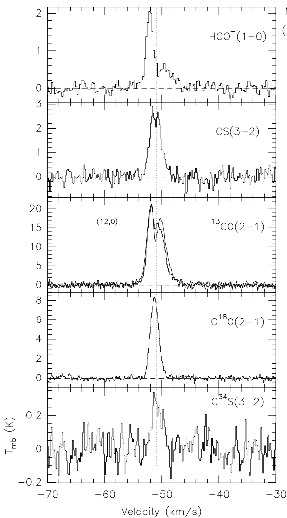
Fig. 1. j) As a) , for Mol 155. The ^{13}\text{CO}(2-1) spectrum at (12'',0'') is also shown (drawn), for comparison
