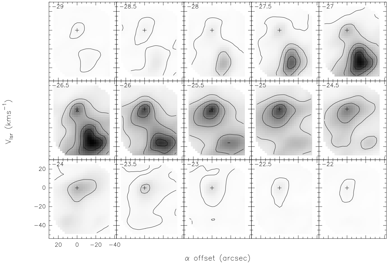
Fig. 11. Mol 8 data. Integrated emission of the ^{13}\text{CO} line, shown in steps of 0.5 \text{ km s}^{-1} . The cross indicates the position of the sub-mm peak ( \approx IRAS source position). Contours 0.5(4)17 \text{ K km s}^{-1} . The \text{HCO}^+ and \text{CS} emission show the same behaviour, and are not shown
