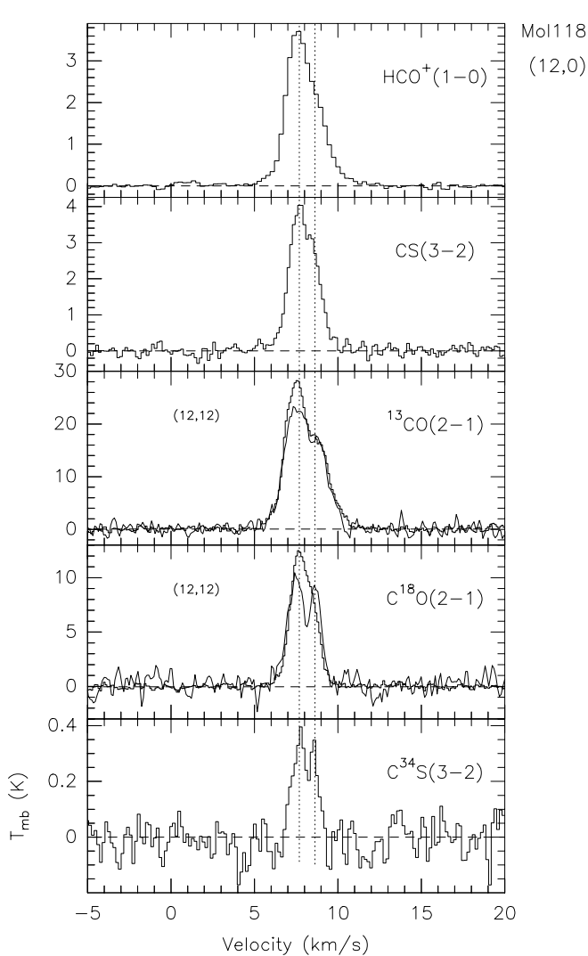
Fig. 1. h) As a) , for Mol 118. The ^{13}\text{CO}(2-1) and \text{C}^{18}\text{O}(2-1) spectra at (12'',12'') are also shown (drawn), for comparison. The dotted line with the red-shifted velocity, with respect to the V_{\text{LSR}} of the \text{C}^{34}\text{S} line, indicates the second component present in these observations (see Sect. 5)
