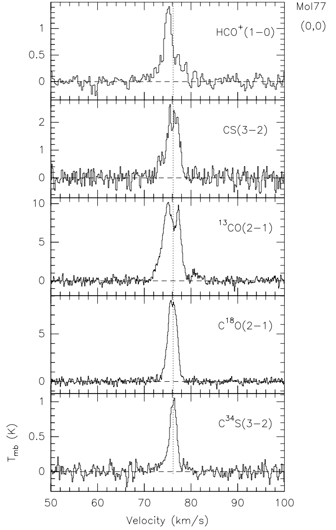
Fig. 1. e) As a), for Mol 77
