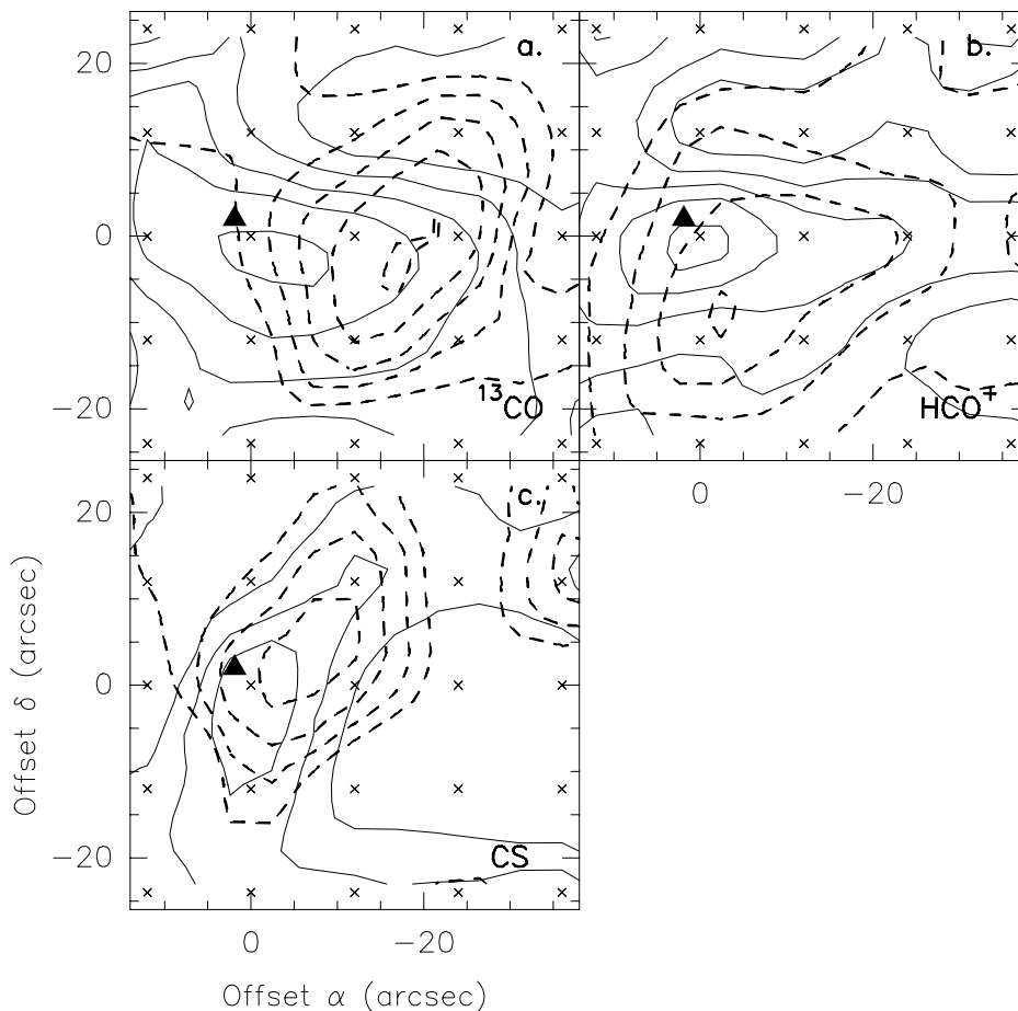
Fig. 20. Mol 136 data. Emission in the wings of the profiles of ^{13}\text{CO} a ), \text{HCO}^+ b ), and CS c ). Drawn and dashed contours refer to blue and red wings, respectively. Integrated velocity interval for the blue emission is -51 to -48 ; for the red emission it's -44.5 to -41 ( -42 for CS). Contour values (low(step)max) are: 1(1)5 \text{K km s}^{-1} a ); 0.2(0.2)1 \text{K km s}^{-1} ( b ), blue), 0.2(0.2)0.8 \text{K km s}^{-1} ( b , red); 0.2(0.3)1.1 \text{K km s}^{-1} ( c ), blue), and 0.2(0.2)1 \text{K km s}^{-1} ( c , red). The triangle indicates the position of the IRAS source
