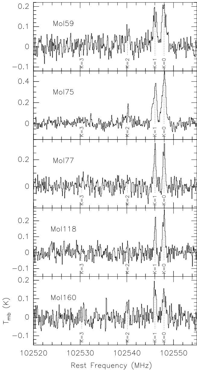
Fig. 3. a) Spectra of the \text{CH}_3\text{C}_2\text{H}(6-5) rotational transition towards the peak position. Only the higher-resolution ( 0.23 \text{ km s}^{-1} ) spectra are shown. The location of the first few K -components are indicated in the spectra
