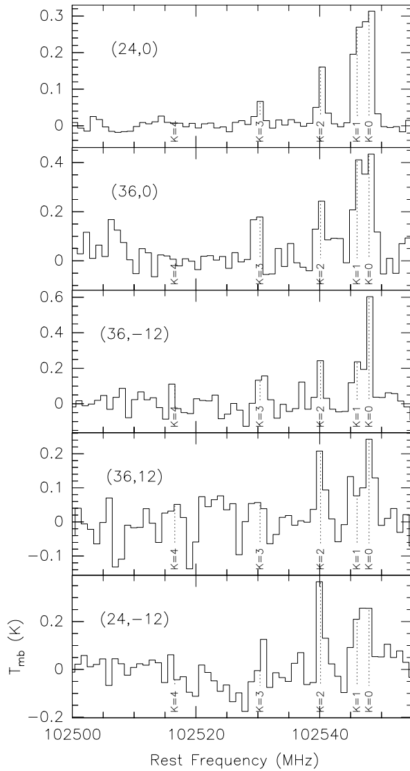
Fig. 3. d) As a), but for various positions towards Mol 98. The velocity resolution of the spectra is 2.92 \text{ km s}^{-1} ; the offset position at which they were taken are indicated in the panels
