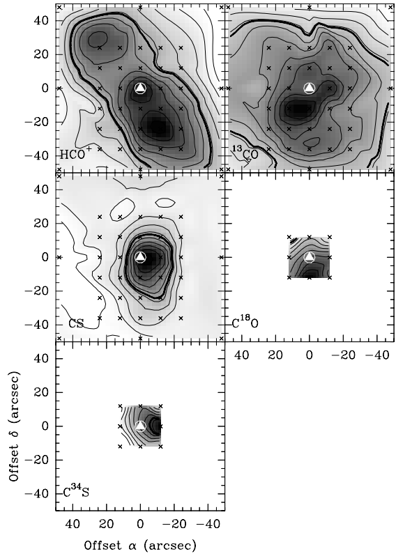
Fig. 5. d) Same as a), for Mol 75. Contour values (low (step) high, in \text{Kkm s}^{-1} ) are: 1(1)10 ( \text{HCO}^+ ); 15(6)81 ( ^{13}\text{CO} ); 1(2)19 (CS); 14(2)34 ( \text{C}^{18}\text{O} ); 0.3(0.3)2.7 ( \text{C}^{34}\text{S} )
