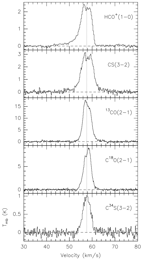
Fig. 1. f) As a), for Mol 98
