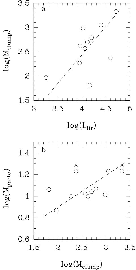
Fig. 25. a) Relation between clump mass (data from Table 8) and luminosity (data from Table 2). The least-squares (bisector) fit is shown as the dashed line, which has a slope of 1.17 \pm 0.22 ; b) Mass of the embedded protostellar object, as function of clump mass. The dashed line is the least-squares (bisector) fit to the data, and has a slope of 0.30 \pm 0.07
