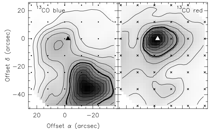
Fig. 12. Mol 8 data. Emission under the ^{13}\text{CO} lines, integrated over the blue and red components (separated by Gaussian fits). Contour values are 2(4)45 \text{ K km s}^{-1} (blue) and 2(4)38 \text{ K km s}^{-1} (red), respectively. The thick contours indicate the FWHM level. The triangle represents the IRAS position
