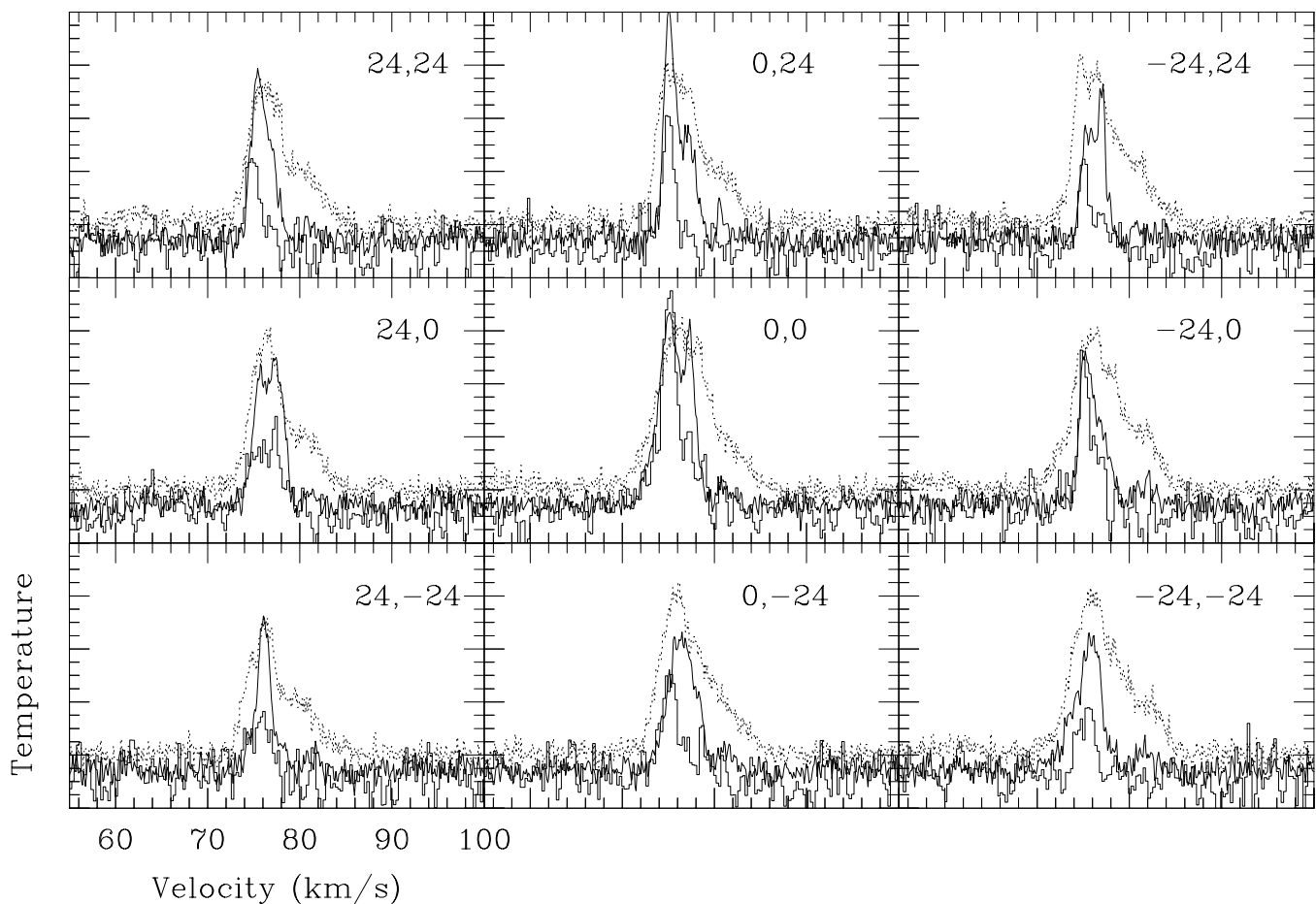
Fig. 15. Mol 77 data. Comparison of line profiles of ^{12}\text{CO} (dashed), ^{13}\text{CO} (drawn), and \text{HCO}^+ (histogram), in the central part of the cloud. The vertical scale is temperature, but scaled such as to make all lines clearly visible. The NRAO 12-m ^{12}\text{CO} spectra were actually taken on a 29'' grid, rather than 24'' . The beam of the ^{12}\text{CO} observations ( \sim 29'' ) is comparable to that of the IRAM 30-m \text{HCO}^+ ( \sim 27'' ); the ^{13}\text{CO} observations were made with a \sim 11'' beam. These plots suggest that the dip/shoulder in the IRAM spectra is probably due to the superposition in velocity of 2 components
