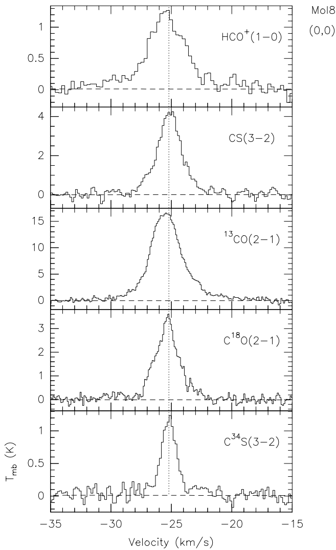
Fig. 1. b) As a), for Mol 8
