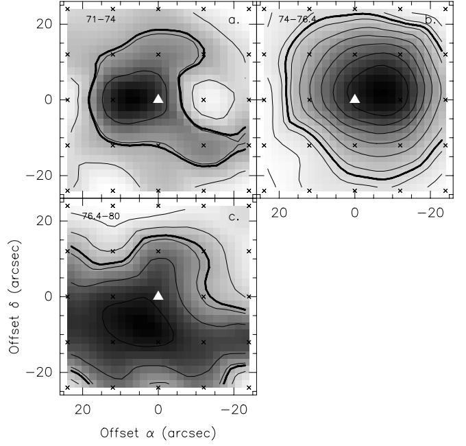
Fig. 16. b) As a) but for \text{HCO}^+ . Contours: 0.2(0.2)0.8 \text{ K km s}^{-1} (panel a); 0.8(0.2)2.6 b); 0.2(0.2)1.2 c)
