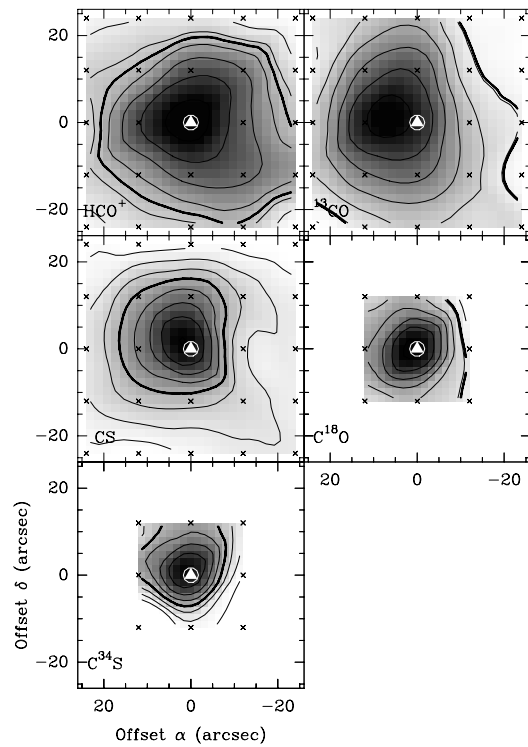
Fig. 5. e) Same as a), for Mol 77. Contour values (low (step) high, in \text{Kkm s}^{-1} ) are: 1(0.5)4 ( \text{HCO}^+ ); 18(4)42 ( ^{13}\text{CO} ); 1(1)8 (CS); 7(2)21 ( \text{C}^{18}\text{O} ); 0.3(0.3)2.4 ( \text{C}^{34}\text{S} )
