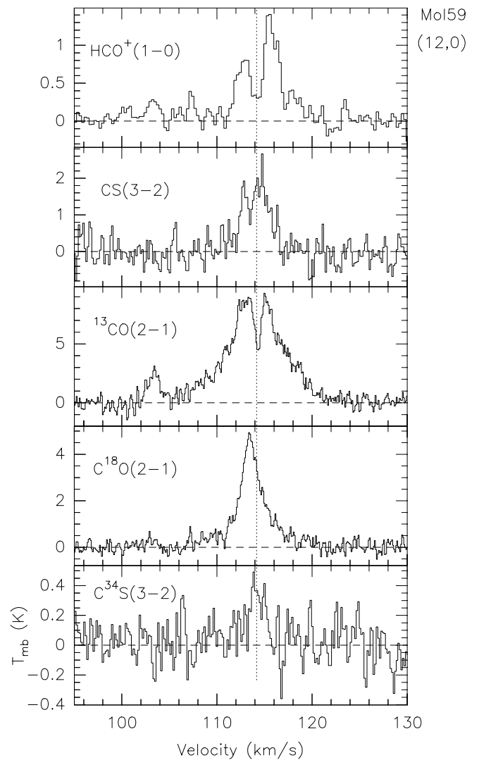
Fig. 1. c) As a), for Mol 59
