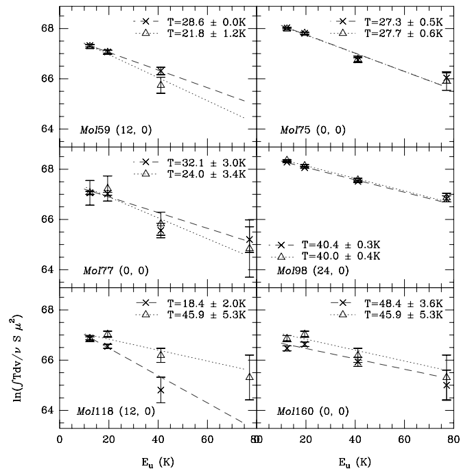
Fig. 8. Boltzmann plots, constructed from the CH_3C_2H(6-5) observations. The results from the high- (0.23 km s^{-1} ) and low-resolution (2.92 km s^{-1} ) spectra are shown as crosses and triangles, respectively. The dashed and dotted lines are weighted least-squares fits through the data points. The sources are identified in the panels, where also the derived T_{kin} is given. Full results are presented in Table 7
