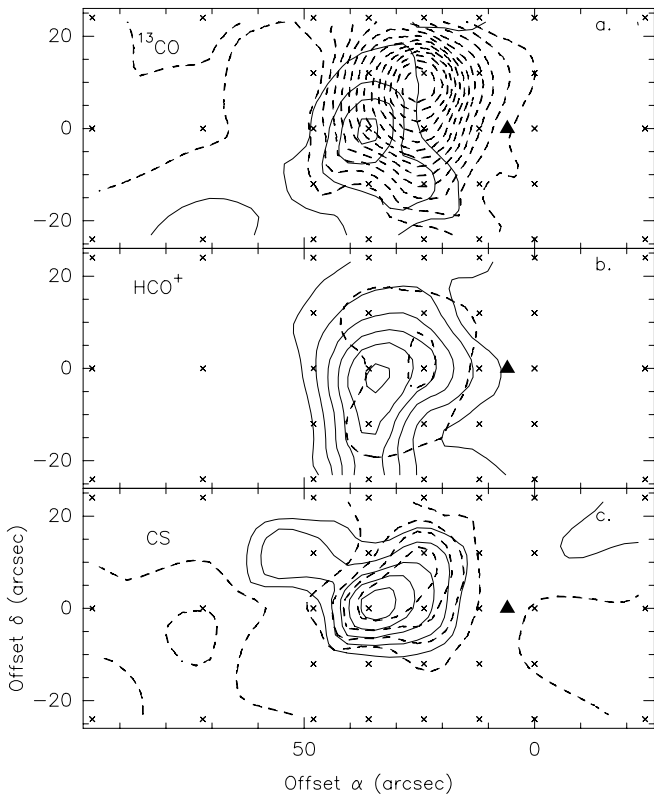
Fig. 17. Mol 98 data. Emission in the wings of the profiles of ^{13}\text{CO} a ), \text{HCO}^+ b ), and CS c ). Drawn and dashed contours refer to blue and red wings, respectively. Integrated velocity interval and contour values (blue, red: range, low(step)max) are: 52–54: 1(1)4, 60–65: 1(1)14 \text{K km s}^{-1} a ); 45–54: 0.5(0.5)3, 60–64: 0.5(0.5)1 \text{K km s}^{-1} b ); 48–54: 0.5(0.5)2.5, 61–65: 0.5(0.5)2.5 \text{K km s}^{-1} c )
