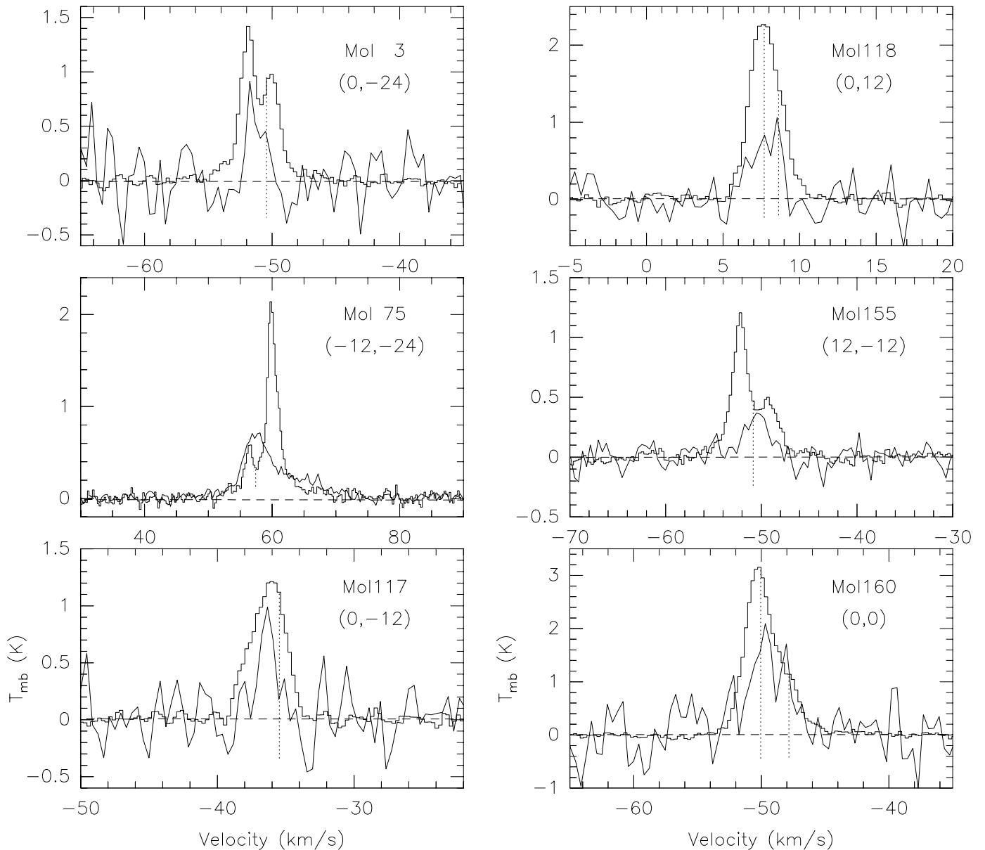
Fig. 2. a) Comparison of the IRAM \text{HCO}^+(1-0) [histogram] spectra with the KOSMA \text{HCO}^+(4-3) [drawn] spectra, at the indicated positions, for Mol 3, 75, and 117. The dotted vertical lines indicate the V_{1sr} of the \text{C}^{34}\text{S}(3-2) emission (from Gaussian fits); the dashed horizontal lines indicate the 0 K level. The IRAM spectra were convolved to a 70'' beam; the KOSMA spectra were smoothed to a resolution of 0.4 \text{ km s}^{-1} , and multiplied by 7 (Mol 3), and 5 (Mol 117) to make comparison easier
