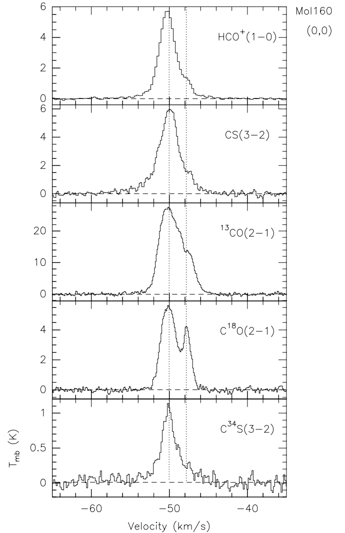
Fig. 1. k) As a) , for Mol 160. The dotted line with the redshifted velocity, with respect to the V_{\text{lsr}} of the \text{C}^{34}\text{S} line, indicates the second component present in these observations (see Sect. 5)
