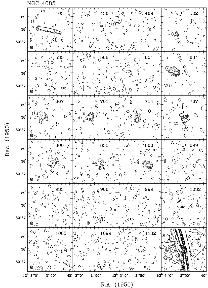
Channel maps at a resolution of 12'' \times 15'' \times 20 km s -1 . Contour levels at -3, -1.5 (dashed), 1.5, 3, 4.5, ... \times \sigma .
