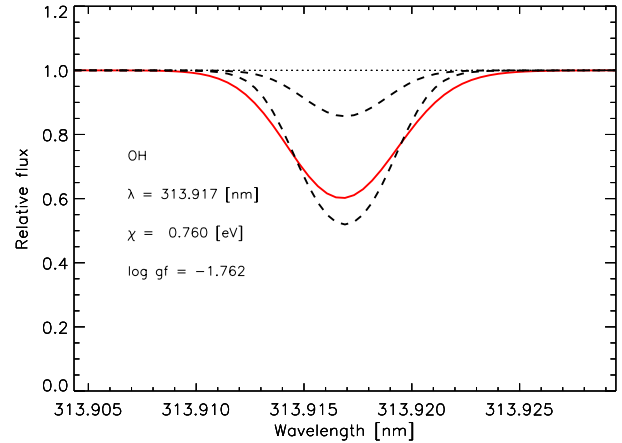
Fig. 2. The predicted profile for the OH 313.9 nm line using the 3D hydrodynamical model atmosphere for T_{\text{eff}} = 5800 K, \log g = 4.44 [cgs], [\text{Fe}/\text{H}] = -3.0 with an adopted O abundance of \log \epsilon_{\text{O}} = 6.4 (solid line). In comparison the corresponding 1D profile with the same abundance is much weaker (upper dashed line). Only with \log \epsilon_{\text{O}} = 7.05 (lower dashed line) is the 1D profile comparable in strength to the 3D profile. In no cases have extra broadening in the form of rotation or macro-turbulence been applied.
