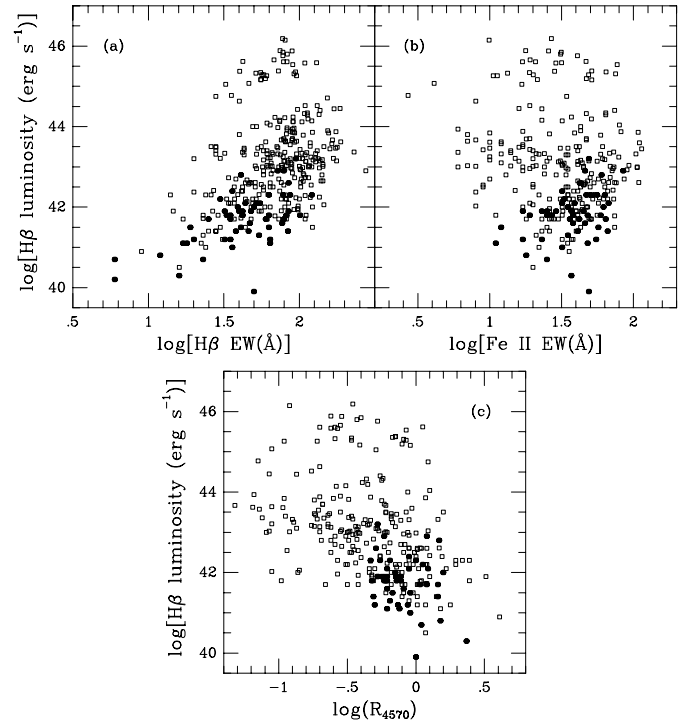
Fig. 10. Plots of the broad H \beta luminosity: in a ) vs. the EW of the broad H \beta component; the two parameters are highly correlated ( r = 0.43 ) for low luminosity objects ( L(\text{H}\beta) < 10^{42.5} erg s ^{-1} ); but the H \beta EW s saturate at \sim 100 Å for larger luminosity objects; in b ), vs. the Fe II EW ; it is a scatter diagram ( r = 0.20 ); in c ) vs. R_{4570} . The anticorrelation observed ( r = 0.42 ) is clearly due to the weakness of H \beta in the low luminosity objects rather than to the strength of R_{4570} . Several samples of Seyfert 1s have been used; our own is shown as filled circles; others (see text) are shown as open squares.
