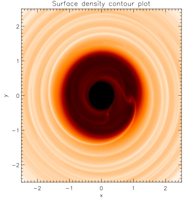
Fig. 2. Surface density plot for inner regions of the disc at a time corresponding to 300 orbits. Darker areas on the plot correspond to regions of lower surface density. The disc cavity is clearly visible, as are the density waves outside the cavity. Inside the cavity are the wakes of the two planets.
