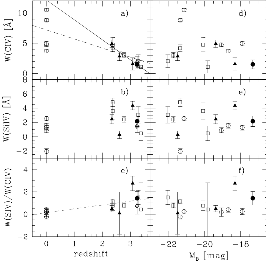
Fig. 9. Measured C IV 1550 and Si IV 1400 rest frame equivalent widths as well as their ratio Si IV/C IV versus redshift (a)–(c) and absolute B -magnitude (d)–(f)). The absolute magnitudes are determined with H_0 = 50 \text{ km s}^{-1}/\text{Mpc} and q_0 = 0.5 . For the k -correction we used values provided by Möller et al. (2001). Evolutionary corrections are not applied. Filled triangles: 1E0657-56 galaxies; filled circle: core; asterisk: arc of 1E0657-56; open squares: FDF galaxies; open hexagons: nearby starburst galaxies. Solid line: weighted \chi^2 fit for high- z objects only (i.e., without local ones); dashed line: weighted \chi^2 fit for all shown galaxies (both high- z and local).
