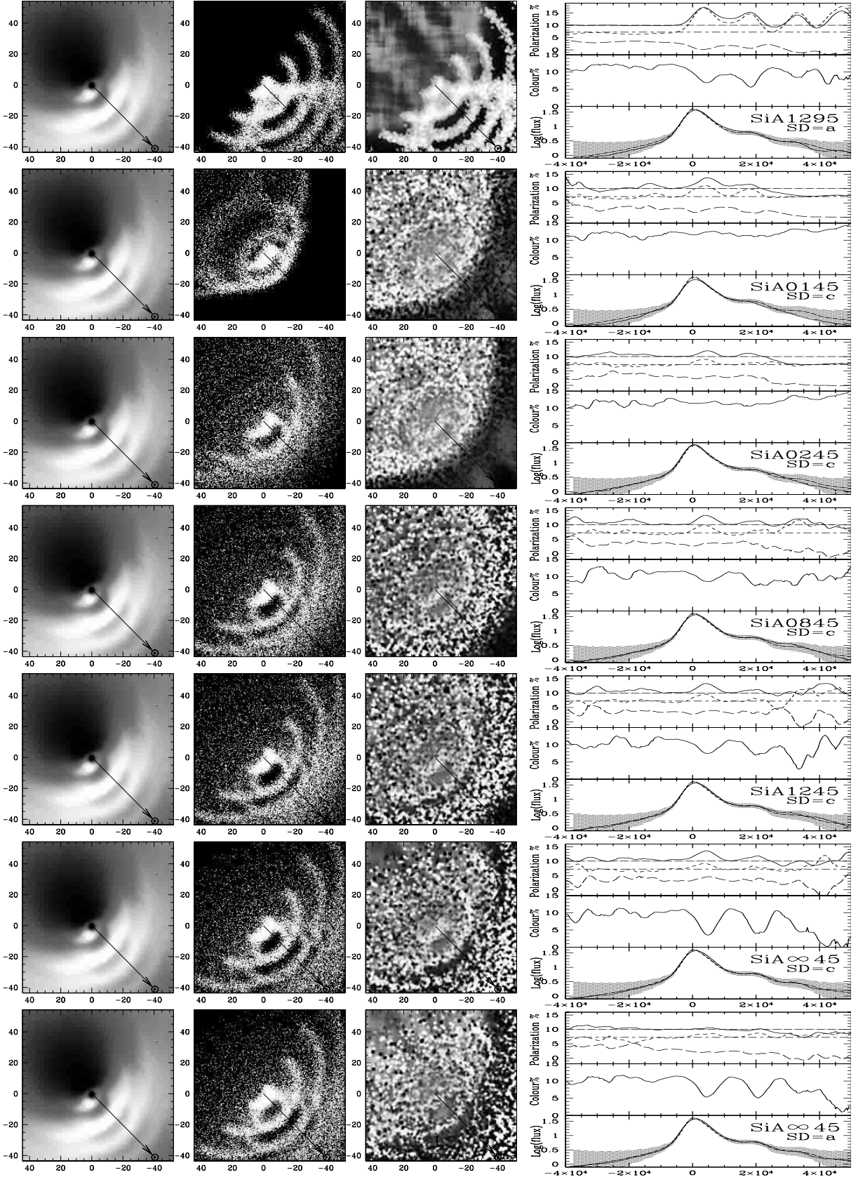
Fig. 5. Column 1: observed processed image from VBO \times (projected cometocentric distance) -1 . North is top and East is left. The sets of shells expanding from the nucleus in the direction of N-W, S-W and S-E are from the sources at -5^\circ , 65^\circ and +5^\circ respectively. Columns 2 and 3: simulated intensity (shell) and polarization (shell + coma) maps. Column 4: intensity scans of the shells superposed on the coma (lower panel), colour in % (middle panel), P_r (solid line in top panel), P_b (short dashed line in top panel) and P_r - P_b (long dashed line in top panel).
