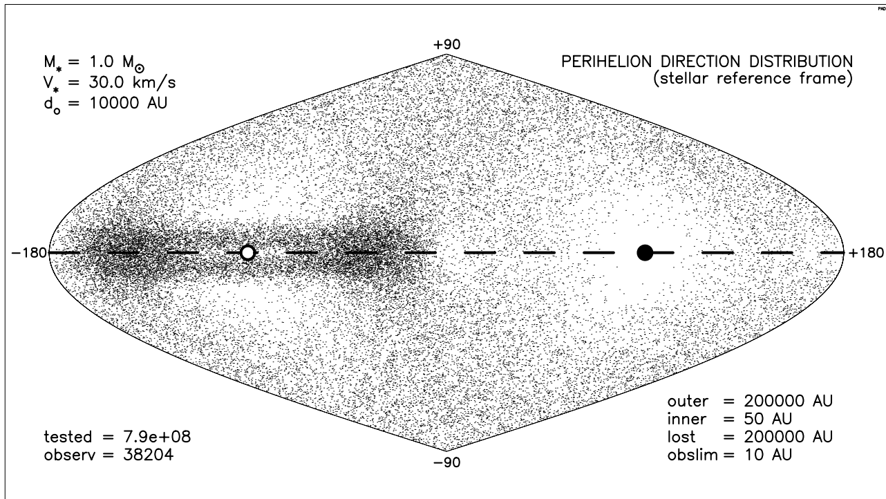
Fig. 2. Perihelion points direction distribution for the observable subsample of comets, presented in the equal-area projection of the celestial sphere. The dashed line is the stellar path projection with an empty circle at star perihelion and full circle at its anti-perihelion.
