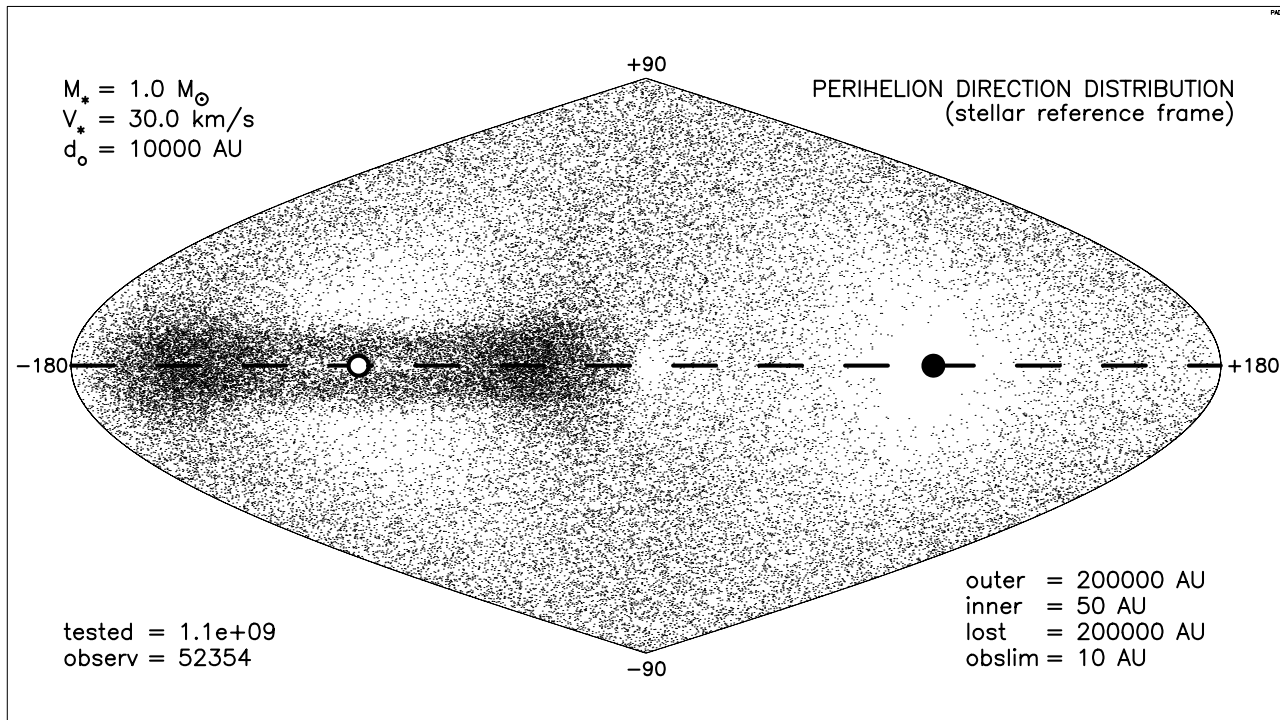
Fig. 5. The same as in Fig. 3 but obtained with the exact numerical integration of separate three body (Sun – star – comet) problems constituting the simulation.
