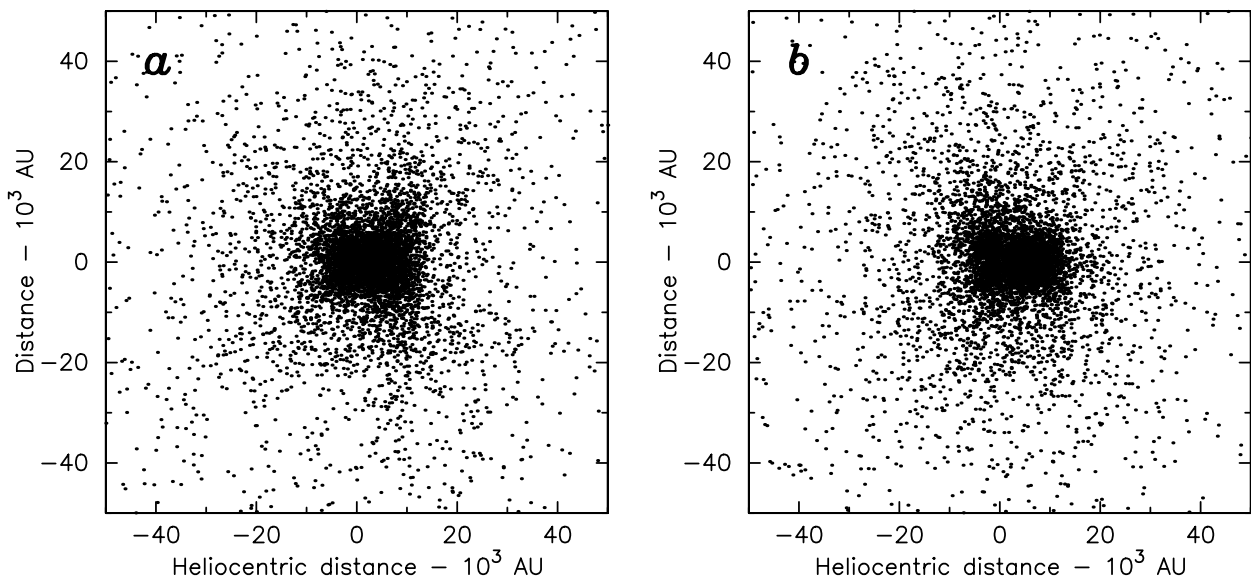
Fig. 4. The same as in Fig. 1 but for IB = 10 AU. Note that this is a rather peculiar and hardly acceptable value of the parameter IB (see text for explanation).
