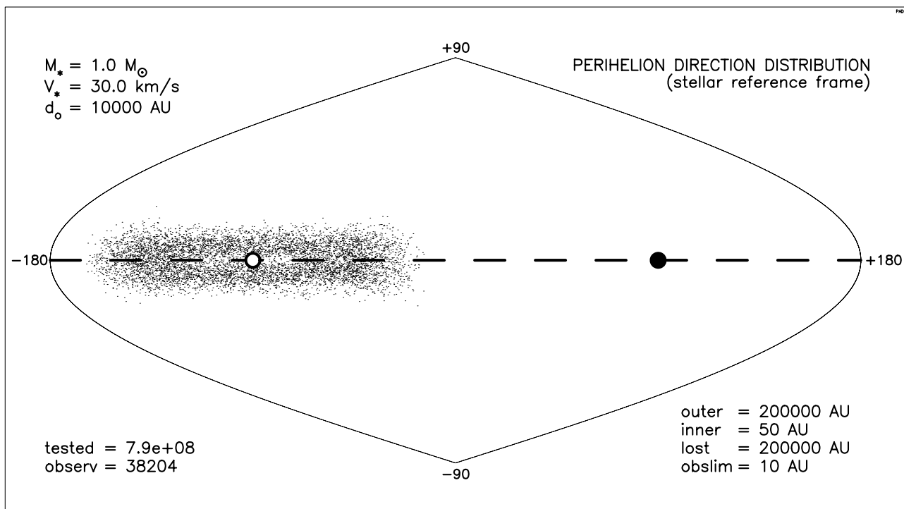
Fig. 3. Same as in Fig. 2, but limited to comets, which arrive at perihelion no later than 500 000 years after the stellar passage.
