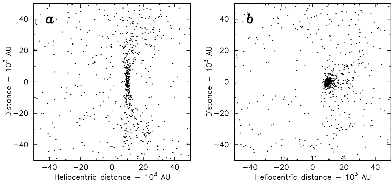
Fig. 1. The positions of comets perturbed to q < 10 AU, obtained from our simulation for IB = 50 AU and recorded at the moment of the minimum Sun-star distance.
