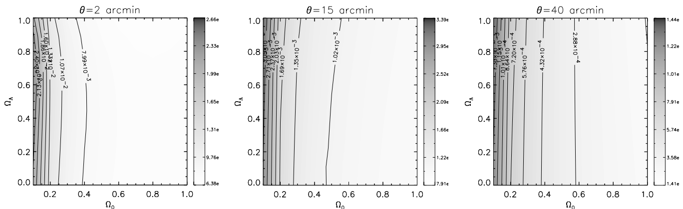
Fig. 2. The dependence of w_{\kappa\delta} on \Omega_0 and \Omega_\Lambda is shown for two different angular scales ( \theta = 2' , 15' and 40' ). Here we have used a cluster normalised cosmology, with \Gamma = \Omega_0 h and \bar{b} = 1 . On scales greater than one arcminute, the \Omega_\Lambda -dependence is so weak that this parameter can safely be eliminated.
