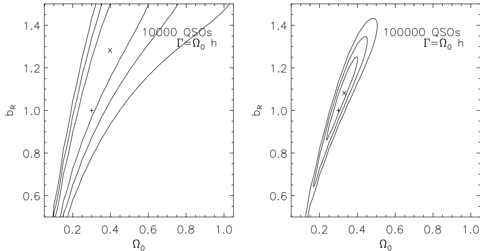
Fig. 5. Expected constraints on the parameters \Omega_0 and \bar{b} for cluster normalised universes. The input parameters used to create the simulated observation are (\Omega_0, \Omega_\Lambda, \sigma_8, \Gamma) = (0.3, 0.7, 1.0, 0.21) , and the bias was set to unity. The panels show the 1-, 2- and 3- \sigma confidence levels for quasar sample sizes of 10^4 , 10^5 , using the relation \Gamma = \Omega_0 h . The symbol “+” shows the location of the input model, and the symbol “x” shows the minimum of the \chi^2 .
