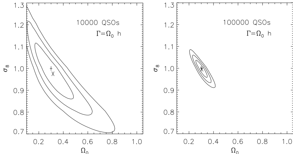
Fig. 6. Expected constraints on cosmological parameters. The contours show the 68%, 90%, and 95% confidence levels. The two panels show results for quasar sample sizes of 10^4 , 10^5 . The parameters of the input model are (\Omega_0, \Omega_\Lambda, \sigma_8, \Gamma) = (0.3, 0.7, 1.0, 0.21) , and \bar{b}_R = 1 .
