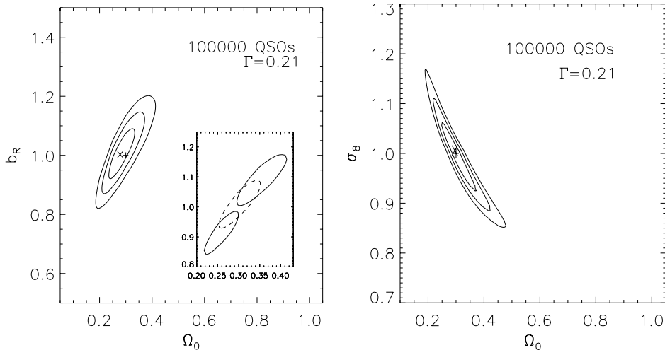
Fig. 7. Expected constraints on cosmological parameters. The contours show the 68%, 90%, and 95% confidence levels, for a quasar sample size of 10^5 , considering the fixed value \Gamma = 0.21 . The parameters of the input model are (\Omega_0, \Omega_\Lambda, \sigma_8, \Gamma) = (0.3, 0.7, 1.0, 0.21) , and \bar{b}_R = 1 . The frame in the left panel shows how the 1- \sigma contour moves by considering \Gamma = 0.21 , but having \Gamma_{\text{true}} = 0.19 or 0.23 .
