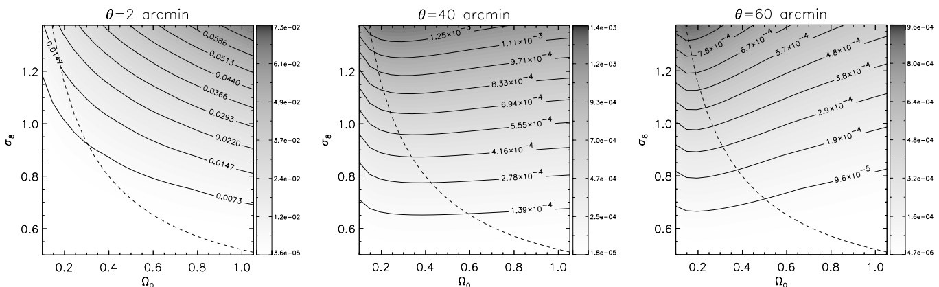
Fig. 3. The dependence of w_{\kappa\delta} on \Omega_0 and \sigma_8 is shown for three different angular scales ( \theta = 2' , 40' and 60' from left to right) and assuming \Gamma = \Omega_0 h . We kept h = 0.72 and \bar{b} = 1 fixed for the plot. As the dependence on \sigma_8 and \Omega_0 changes with angular scale, the degeneracy between these two parameters can be broken. At \sim 40' , the correlation function is almost insensitive to \Omega_0 . The dashed line shows the cluster normalisation from Eke et al. (1996).
