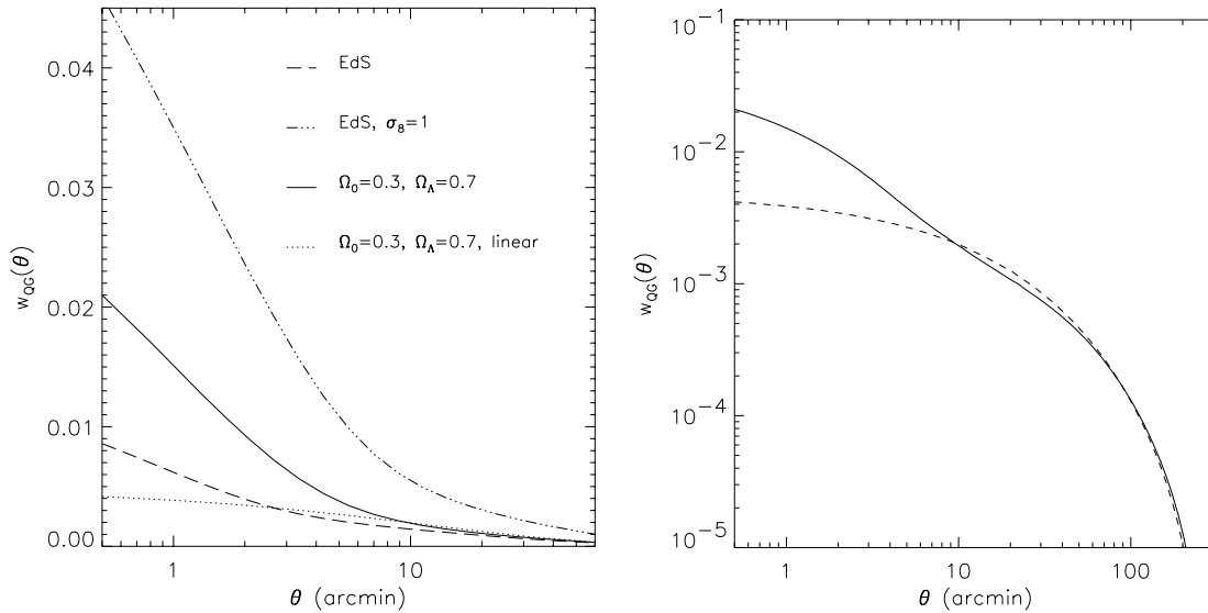
Fig. 1. Left panel: the QSO-galaxy cross-correlation function w_{\text{QG}}(\theta) is plotted for different cluster normalised cosmologies. A low-density flat universe with \Omega_0 = 0.3 , \Omega_\Lambda = 0.7 is plotted in solid line; an Einstein-de Sitter universe is plotted in dashed line, and in dashed-dotted line for a universe normalised with \sigma_8 = 1 . Both curves were computed using the non-linearly evolving matter power spectrum. For comparison, the dotted line shows how the correlation function if we consider linear growth of the power spectrum for a \Omega_0 = 0.3 , \Omega_\Lambda = 0.7 cosmology. Here we have assumed \alpha = 2 , a bias factor of \bar{b} = 1 and a shape parameter of \Gamma = 0.21 . The right panel shows how the correlation function drops at large scales before reaching negative values in a low-density flat universe.
