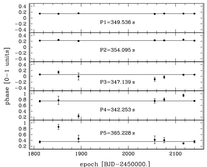
Fig. 5. Phases of all the detected pulsation modes determined from each single run during the period September 2000–August 2001. The phases are normalized to 1 (i.e. 1 corresponds to 2\pi ) and are referred to BJD 24511800.0. The error bars are the formal errors obtained from the sinusoidal fits. Note that even in the worst cases of very low amplitude (P4 and P5), the phases of at least five out of seven independent observations are in agreement within the errors.
