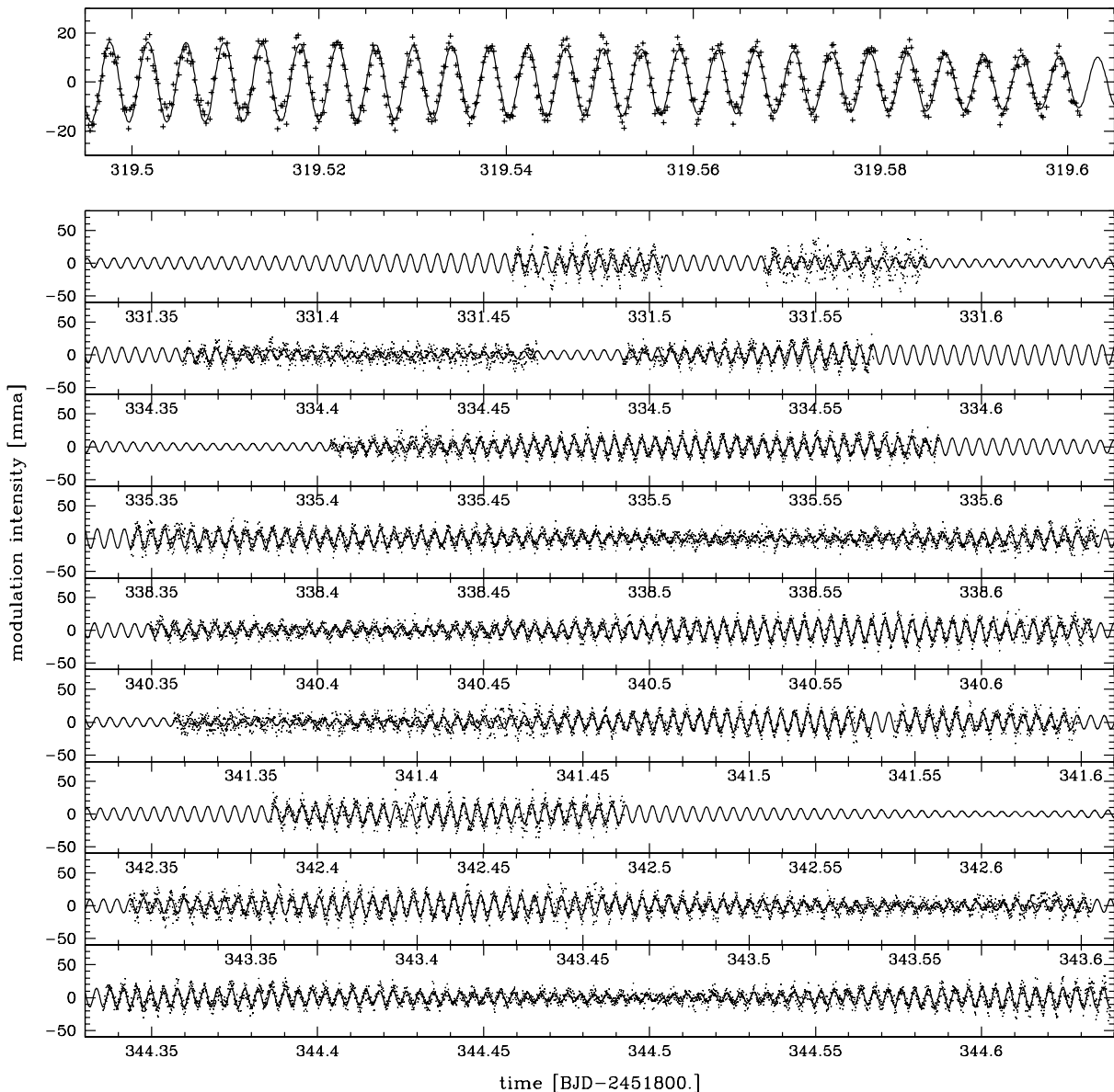
Fig. 2. Light curve of HS 2201 obtained during the run of August 2001 at Loiano. Each panel is 7.44 hours long. The continuous line represents a synthetic light curve obtained with the best fit parameters from the lower section of Table 2. The upper panel shows the quality of the fit compared with the longest (2.6 hours) high-quality observation performed at the NOT in July 2001.
