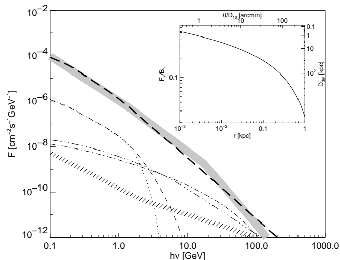
Fig. 8. Toy model for the gamma ray signature produced in a microquasar CR halo via pion decay (including \pi^0 decay and bremsstrahlung from secondary electrons and positrons). Curves were calculated assuming a source active for over \tau \gtrsim 15 \times 10^6 yrs with an average power of L_{\text{kin}} = 3 \times 10^{38} ergs s^{-1} , at a distance of 10 kpc, and for an ISM particle density of 1 \text{ cm}^{-3} , assuming CRs are lost once they have reached the edge of the Galactic disk at about 1 kpc distance from the source. Labels according to Fig. 5. Dotted line : Gamma ray signature from narrow component of the microquasar halo; dashed line : from thermalized component; dash-dotted line : from “powerlaw type component” in the case of efficient scattering; dash-triple-dotted line : from “powerlaw type component” in the case of inefficient scattering. Thick grey line : EGRET diffuse gamma ray background at the position of GRS 1915+105 (Hunter et al. 1997), assuming the same solid angle as subtended by the source. Thick long dashed line : background gamma emission over the same solid angle modeled assuming the proton CR spectrum measured near earth and an average ISM density of 1 \text{ cm}^{-3} . Hatched line : GLAST sensitivity. Models were computed using the GALPROP routines by Moskalenko & Strong (1998). Insert : Angular dependence of the source contribution to the gamma ray flux F_v , relative to the background flux B_v at a photon energy of 1 GeV (see Eq. (8)). The right Y-axis shows the source distance at which the GLAST sensitivity is reached for the value of F_v/B_v shown in the curve, the top X-axis shows the angle \theta = r/D in units of arcmin/ D_{10} where D_{10} is the source distance in units of 10 kpc.
