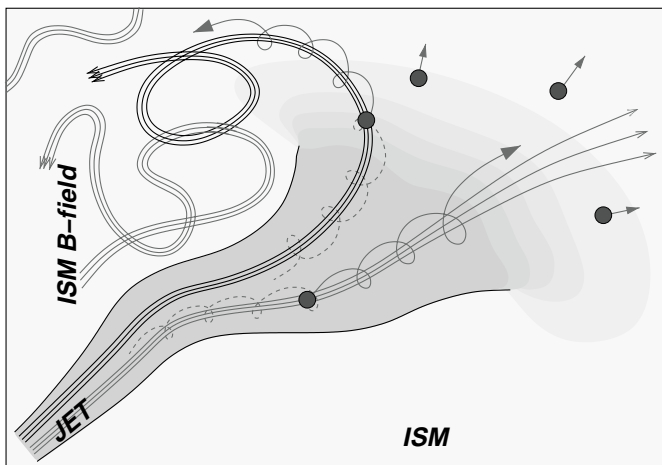
Fig. 4. Cartoon of particle injection by a jet without a strong shock at its interface with the ISM (e.g., if the magnetic structure of the jet is connected with the ISM and the jet is sub-Alfvénic). Dots represent CRs transported by the jet and released into the ISM at the bulk speed of the jet, grey arrows represent magnetic flux tubes. The right flux tube representation depicts the case where adiabatic losses are important, the left shows a case where the field flux tube is smoothly fused with the stochastic interstellar field and adiabatic losses might not be dominant in particle transport.
