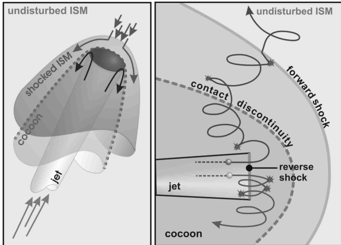
Fig. 2. Cartoon of the standard picture of the interface between jet and ISM ( left panel ), as envisaged to apply in FR II radio galaxies. The injection of relativistic particles can occur either in the reverse or forward shock. Right panel : cartoon of particle trajectories for particles crossing the shock only once (upper solid line) and particles participating in diffusive shock acceleration (lower solid line), particle scattering indicated as stars.
