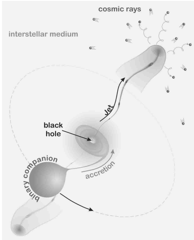
Fig. 1. Cartoon of the proposed model of CR production in microquasars: The interface between the relativistic jet and the ISM is a natural site for the production and release of relativistic particles.
