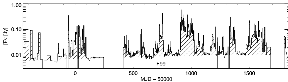
Fig. 6. Plot of the 2.25 GHz GBI monitoring data ( http://www.gb.nrao.edu/fgdocs/gbi/gbint.html ) for GRS 1915+105 over the time span from June 1994 to August 2000. Shown as a hatched area is the flux considered above the baseline flux, i.e., the flux considered to originate from flares, which we integrated to arrive at the estimate for the average kinetic power carried by the jet. The flare analyzed by Fender et al. (1999a) is indicated by the mark “F99”. The large gaps are due to gaps in the monitoring campaign and were not included in the procedure.
