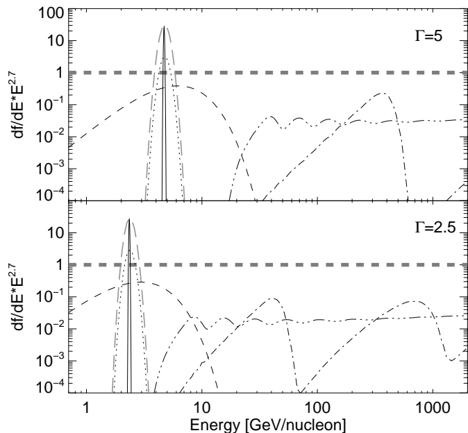
Fig. 7. Toy model of the microquasar contribution to the CR spectrum, for a single microquasar situated in a low mass X-ray binary, active for \tau \gtrsim 1.5 \times 10^7 yrs on the level of 3 \times 10^{38} ergs s^{-1} (similar to GRS 1915+105), and at a distance of 1 kpc. For simplicity, we assumed the source was operating with uniform bulk Lorentz factor \Gamma_{\text{jet}} = 5 (top) and \Gamma_{\text{jet}} = 2.5 (bottom). The curves are normalized relative to the measured differential Galactic CR background spectrum (thick grey dashed line). Shown are the same curves as in Fig. 5: narrow feature for upstream temperature of T \sim 7 \times 10^{10} K (dotted line) and for T \sim 7 \times 10^8 K (solid line), Maxwellian with kT \sim \Gamma_{\text{jet}} m_p c^2/3 (dashed line), multiply scattered component for efficient pitch angle scattering (dash-dotted line) and for inefficient pitch angle scattering (dash-triple-dotted line), and the relative contribution of heavy elements for metallicity 10 times the solar value (long-dashed grey curve), as seen in GRO J1655-40 and V4641 Sgr. Each spectral component has been steepened by E^{-1/2} to account for the energy dependence of the diffusion coefficient.
