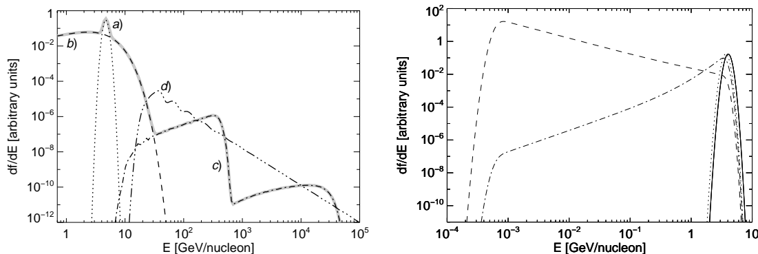
Fig. 5. Left panel: sketch of the predicted contribution from a microquasar to the Galactic CR spectrum for \Gamma_{\text{jet}} = 5 . a) Dotted line: narrow component, corresponding to cold ( T \sim 7 \times 10^{10} K) upstream particles simply isotropized upon crossing the working surface (Lorentz transformed energy distribution), arbitrary normalization; b) dashed line: Maxwell-Boltzmann component from particles thermalized in the shock (normalized to contain the same power as component a ); c) dash-dotted line: powerlaw-like component (escape probability 99%, normalized to contain 10% of component a ) for the case of strong scattering. Note the similarity to Comptonization of low energy seed photons by a relativistic medium with low optical depth (i.e., high escape probability); d) dash-triple-dotted line: powerlaw spectrum for weak scattering case (Achterberg et al. 2001) for the same normalization as component c ). Note the difference in the position of the first peak between c ) and d ), \sim \Gamma_{\text{jet}}^2 vs. \sim \Gamma_{\text{jet}}^3 . Right panel: estimate of the effects of adiabatic losses on the particle distribution for different ratios of the adiabatic losses time \tau_{\text{ad}} of the particles to the escape time \tau_{\text{esc}} , compared to the injected particle distribution (solid) line for a pressure differential between shock and ISM of p_{\text{shock}}/p_{\text{ISM}} = 3 \times 10^8 (see Appendix B): strong adiabatic losses ( \tau_{\text{ad}}/\tau_{\text{esc}} = 10^{-3} , dashed line), intermediated losses ( \tau_{\text{ad}} = \tau_{\text{esc}} , dash-dotted line), and weak adiabatic losses ( \tau_{\text{ad}}/\tau_{\text{esc}} = 10^3 , dotted line).
