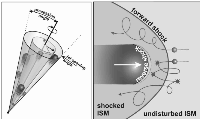
Fig. 3. Left : cartoon of a jet composed of discrete ejections with precession. In such a non-stationary picture, each ejection is slowed by its interaction with the ISM (which might be disturbed by previous ejections). This interaction will likely happen in the form of a forward shock (into the ISM). ISM particles will leave the shock with energies of order \Gamma_{\text{jet}} m_p c^2 (here, \Gamma_{\text{jet}} is the Lorentz factor of the individual ejection, which decreases with time). Right : cartoon of particles crossing a relativistic forward shock, likely the appropriate scenario for a cold ejection running into the ISM. Same nomenclature as in Fig. 2.
