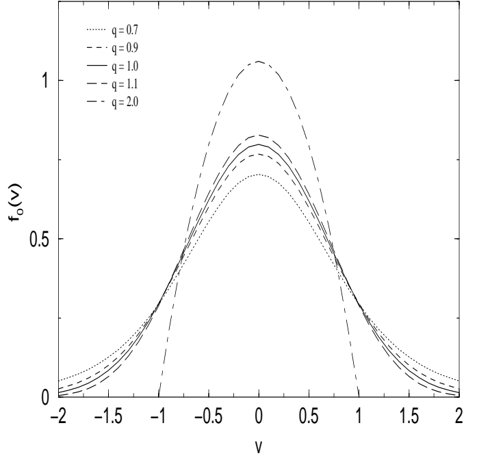
Fig. 1. Nonextensive velocity distribution function f_0(v) for typical values of the q parameter. Power law distributions with q > 1 exhibits a thermal cutoff on the maximum value allowed for the velocity of the particles. This cutoff is absent for \frac{1}{3} < q \leq 1 , and the distribution is unnormalizable for q < \frac{1}{3} .
