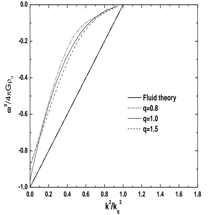
Fig. 3. Unstable branches of the dispersion relations as a function of the critical wavenumbers k_q . Notice that the magnitude of k_q is related to the critical Jeans wavenumber by Eq. (15). As in Fig. 2, the straight solid line stands to the case of an infinite homogeneous fluid.
