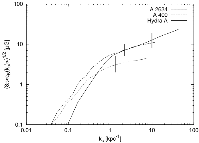
Fig. 4. Magnetic field strength B dependent on the upper k -cutoff in the integration of Eq. (17). The equivalent beamsizes k_{\text{beam}} are represented as vertical lines.
