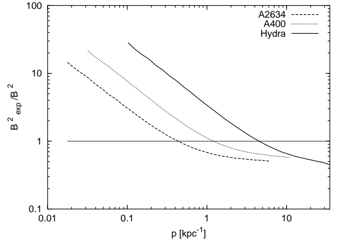
Fig. 8. Comparison between the expected magnetic field strength B to the measured one B_{\text{exp}} for the particular p -scales for the three clusters.
