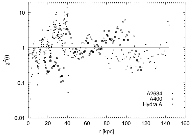
Fig. 5. Testing the window function by calculating the \chi^2(x_\perp) distribution for all three cluster.
