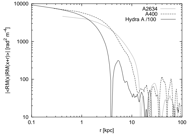
Fig. 1. RM autocorrelation function |C_{RM}(r_{\perp})| of Abell 400, Abell 2634 and Hydra A obtained using Eq. (5). Note that the correlation function for Hydra A was divided by 100 for representing purposes.
