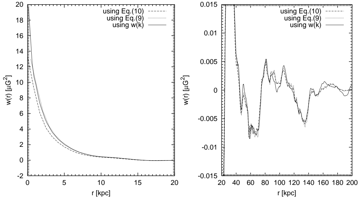
Fig. 2. The magnetic autocorrelation function w(r) for Abell 2634 calculated using Eqs. (9), (10) and (21). One can clearly see that the value of w(r = 0) can deviate by a factor of two but for larger r all methods yield almost the same results.
