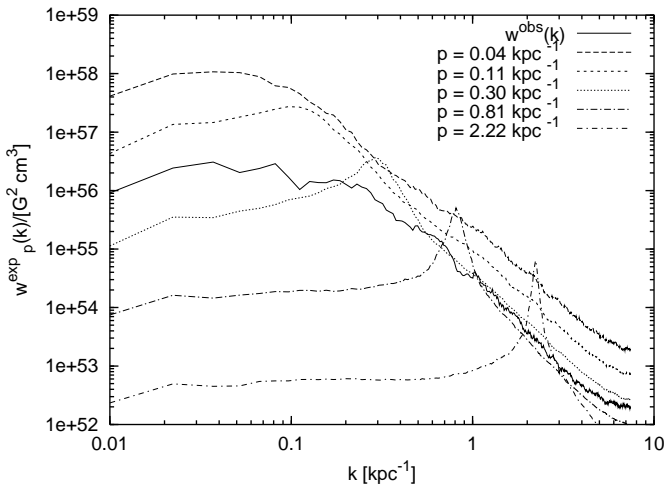
Fig. 7. Responses at various scales p to the window function of Abell 2634 assuming a B = 5 \mu\text{G} in comparison to the observed magnetic autocorrelation function \hat{w}(k) .
