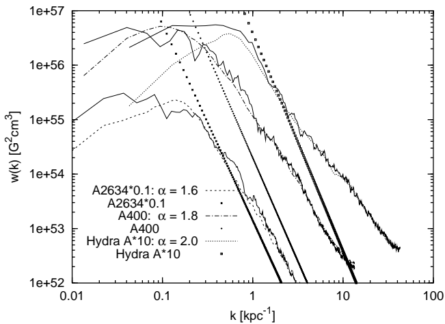
Fig. 9. Closely p -spaced response functions were integrated by employing Eq. (27) and the resulting \hat{w}^{\text{exp}}(k) are exhibited in comparison to the observed power spectrum \hat{w}^{\text{obs}}(k) shown as solid lines. The spectral index \alpha used for Abell 2634 is 1.6, for Abell 400 is 1.8 and for Hydra A is 2.0. The straight lines represent the power law assuming the spectral index determined from the response analysis. Note that the data for Abell 2634 are multiplied by 0.1 and the data for Hydra by 10 for representing purposes.
