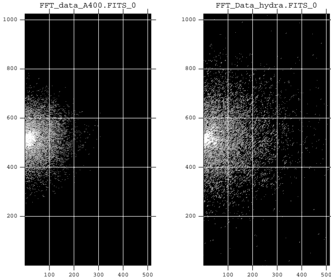
Fig. 6. The power |\langle \hat{R}M(k) \rangle|^2 of the Fourier transformed RM map of Abell 400 on the left side and Hydra A on the right side. The image for Abell 2634 looks similar. Only half of the Fourier plane is exhibited the other half is point symmetric to the one shown.
