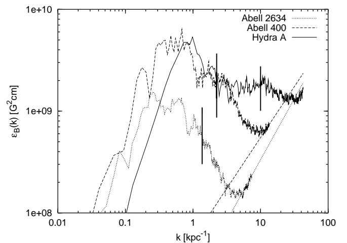
Fig. 3. Magnetic energy spectrum \varepsilon_B^{\text{obs}}(k) derived for Abell 400, Abell 2634 and Hydra A. The Fourier transformed beamsizes ( k_{\text{beam}} = \pi/l_{\text{beam}} ) are represented by the thick vertical lines. The other straight lines describe the slope (dashed line represents \varepsilon_B \propto k and the dotted represents \varepsilon_B \propto k^{1.2} ) of the increase in the energy density for the largest k .
