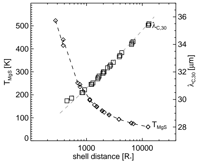
Fig. 6. MgS temperature and the centroid position of the “30” \mu\text{m} feature as a function of distance to the star. The diamonds show the MgS temperature at the inner edges of the detached dust shell. The squares represent the centroid position of the “30” \mu\text{m} emission feature versus the typical distance of the shell, which is defined as the inner radius plus one quarter of the shell thickness. The grey dashed line shows a simple analytic representation of the relation between the distance and the centroid position (see Eq. (2)).
