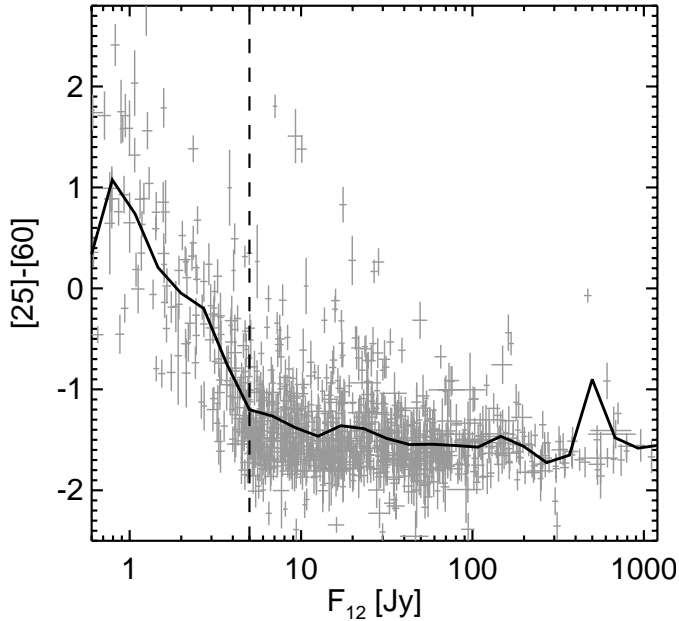
Fig. 4. IRAS colour-magnitude diagram of galactic carbon stars. The thick black line shows the mean of the [25]–[60] colour as a function of 12 \mu\text{m} flux for the carbon stars (shown in grey). The sources with the largest 60 \mu\text{m} excess are all very faint at 12 \mu\text{m} (to the left of the dashed line). The photometry of these sources is probably affected by cirrus contamination or confusion due to the poor angular resolution of IRAS.
