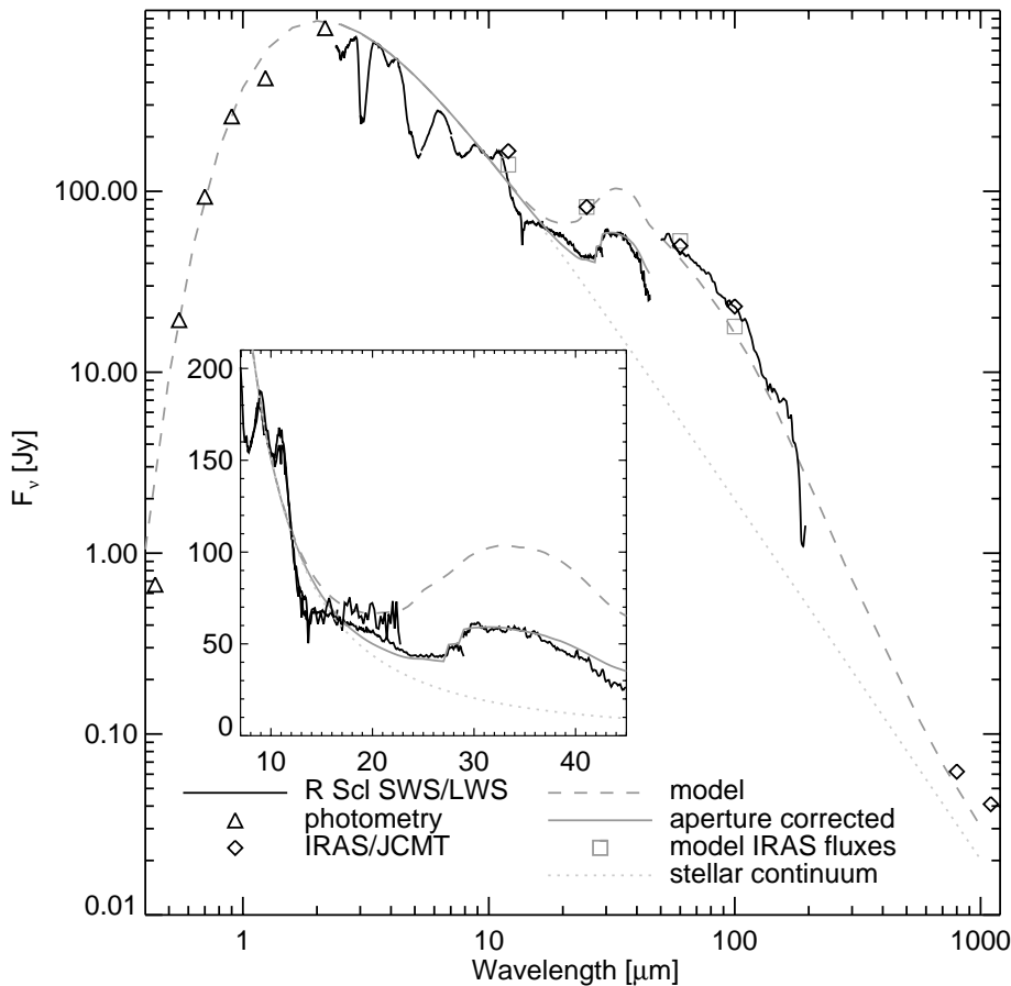
Fig. 7. The detached-shell model compared to the observations of R Scl in black. The optical photometry is shown in triangles (Johnson et al. 1966). Between 2 and 45 \mu\text{m} we show the SWS spectrum (Hony et al. 2002); between 45 and 200 \mu\text{m} we show the LWS spectrum. The diamonds represent the IRAS measurements and the submillimetre points from Bagnulo et al. (1998). The dashed gray line is the model SED, taking identical parameters for the dust shell as derived for the CO shell by Schöier & Olofsson (2001). The full gray line shows the model spectrum after correction for the limited size of the apertures of the SWS spectrograph. The dotted line represents the photospheric continuum. We also show the synthetic IRAS fluxes as derived from the model SED. The 25 and 60 \mu\text{m} IRAS fluxes are in excellent agreement. The predicted flux level at longer wavelengths is slightly too low. The model explains the observations very well. In the inset, we show the fit to the “30” \mu\text{m} feature on a linear scale. We also show the IRAS/LRS spectrum, which starts to deviate from the SWS spectrum at the wavelength, where the model predicts a difference, due to the different beam-size of IRAS and SWS.
