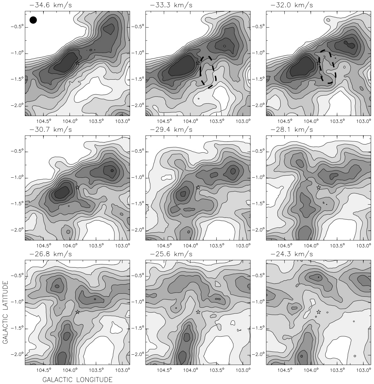
Fig. 3. WR 154 Effelsberg grey-scale images showing the HI distribution in the velocity range -34.6 to -24.3 km s ^{-1} . The half beam width (HPBW \sim 9' ) is shown in the upper left corner of the first image. The stellar position is indicated by a star symbol. The central velocity of every map is specified in the upper left corner. Contour levels are at -10 to 30 K in steps of 5 K.
