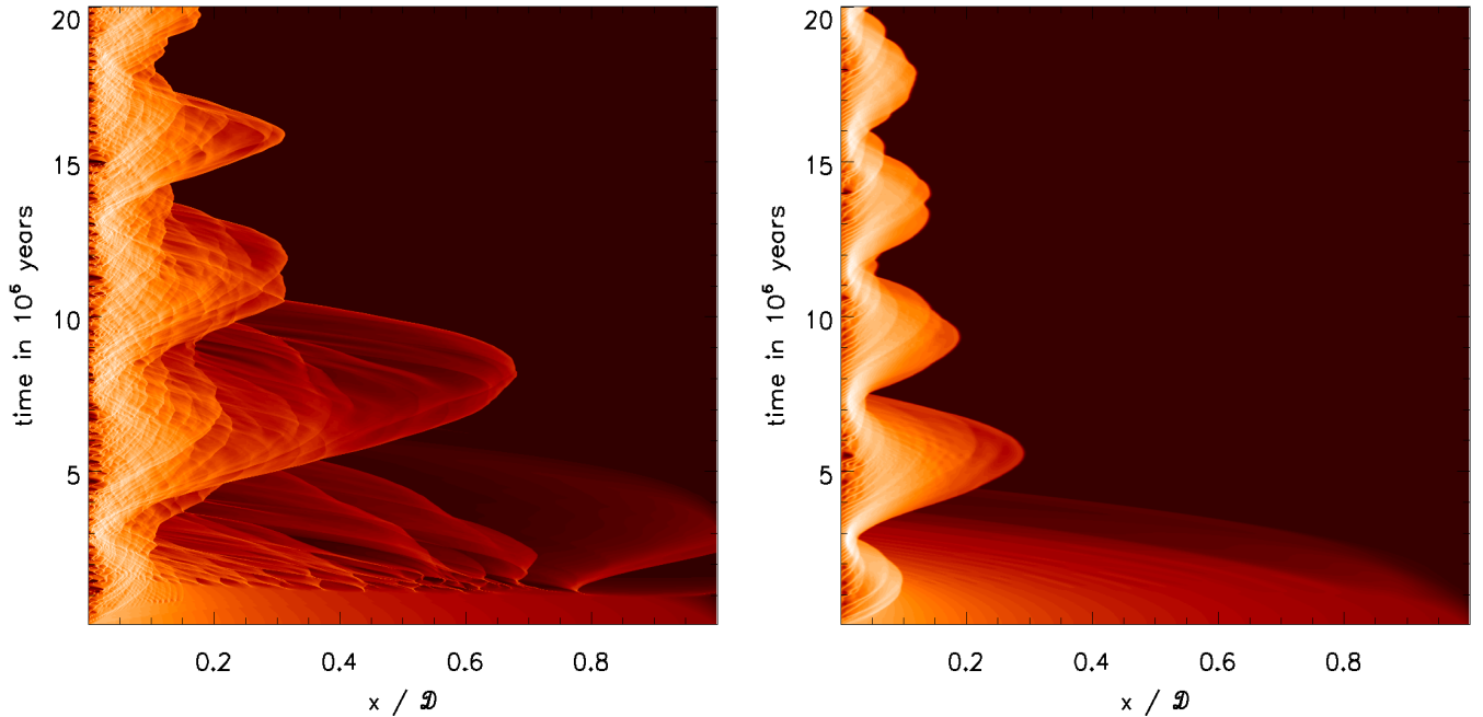
Fig. 8. Good enough spatial resolution is crucial to observe the structuring and supporting effect of the injected Alfvén-wave. Shown is the same simulation, R20.20.5.4.10, once, a ), with our usual spatial resolution of 5000 cells and once, b ), with a reduced resolution of only 1000 cells. Logarithmic particle density is shown as a function of space ( x -axis, in units of 6 pc) and time ( y -axis, in units of 10^6 years). A similar loss of structuring and support we observe if the order of the integration scheme is reduced.
