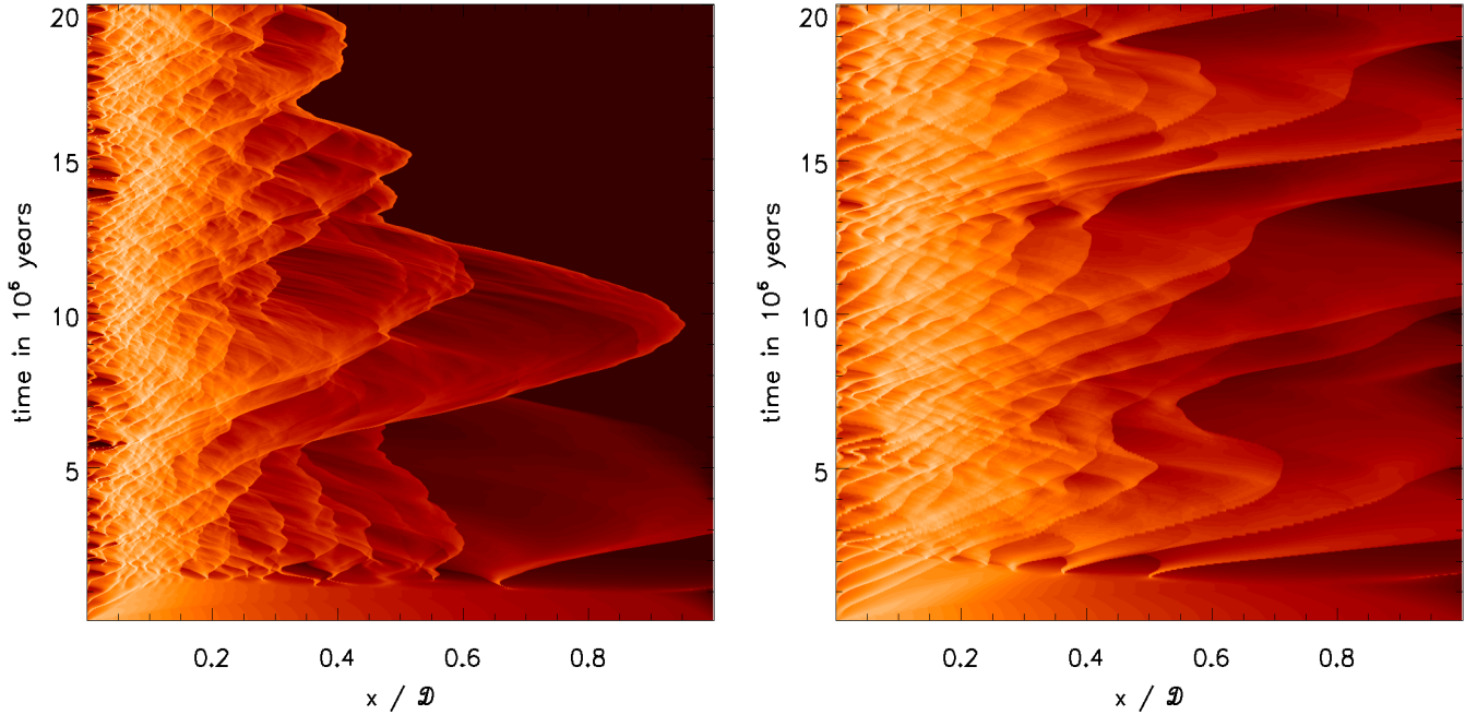
Fig. 4. Smaller voids (black, N = 10^{-1} \text{ cm}^{-3} ) separating the high density sheets (white, N = 10^4 \text{ cm}^{-3} ) are obtained for smaller \lambda_{A0} and / or higher temperatures T . a) Run R20.20.12.4.10 has the same temperature T as run R20.20.25.4.10 in Fig. 3, but only half the value of \lambda_{A0} . b) Run R20.20.25.4.40 has the same \lambda_{A0} as run R20.20.25.4.10 in Fig. 3 but a four times higher temperature T . Shown is the logarithmic particle density as a function of space ( x -axis, in units of 6 pc) and time ( y -axis, in units of 10^6 years).
