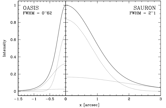
Fig. 3. Effective PSF for the OASIS ( left ) and SAURON ( right ) merged datacubes of NGC 3377. As described in the text, the OASIS PSF is highly non-Gaussian and is properly described by a sum of three Gaussians ( dotted lines ); the spatial resolution is estimated to be 0''.62 FWHM . The SAURON PSF is described by a double Gaussian of 2''.1 FWHM .
