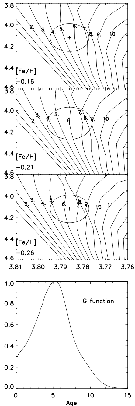
Fig. 13. Top: three slices of the three-dimensional HR “cube” showing the observed point (central panel) and three cuts through the 1- \sigma error ellipsoid. The probability distribution function (G-function, bottom) is computed from all points on the isochrones, not just those on or inside the error ellipsoid.
