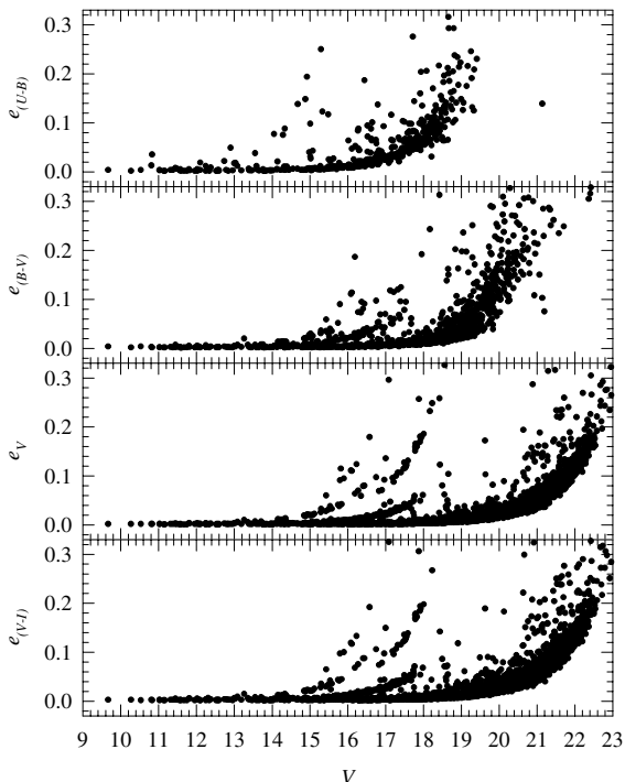
Fig. 2. DAOPHOT errors in the colour indexes and V magnitude as a function of V .
