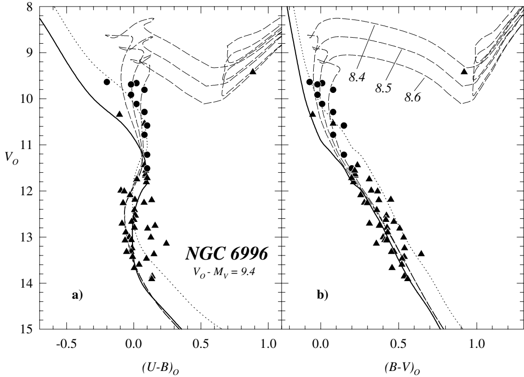
Fig. 12. V_0 vs. (B - V)_0 diagram of the likely and probable member stars in the region of NGC 6996. Symbols as in Fig. 7a. Solid and dotted lines are the Schmidt-Kaler (1982) ZAMS shifted by the adopted distance modulus V_0 - M_V = 9.4 and the 0.75 envelope limit for binaries. Dashed curves are the isochrones from Girardi et al. (2000). Numbers give the \log (age).
