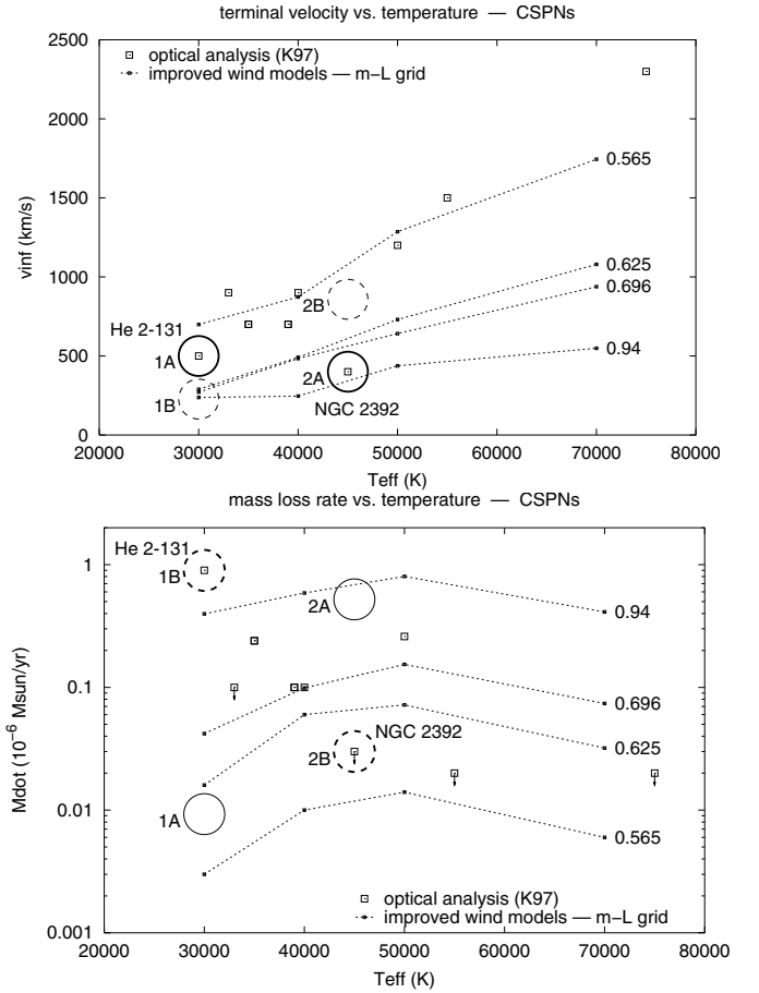
Fig. 2. Terminal velocities ( upper panel ) and mass-loss rates ( lower panel ) calculated for a grid of stars following post-AGB evolutionary tracks (dashed lines, masses in M_{\odot} labelled on the right) compared to observed values derived by Kudritzki et al. (1997) (squares). Note that the observed terminal velocities and mass-loss rates indicate different masses for the same objects (circles) – for a discussion see text.
