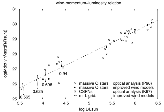
Fig. 1. The wind-momentum–luminosity relation for massive O stars and CSPNs. P96 designates the analysis based on H\alpha profiles by Puls et al. (1996), K97 that of CSPNs by Kudritzki et al. (1997). Also plotted are the calculated wind momenta for a sample of massive O stars and for a grid of stars following post-AGB evolutionary tracks (masses given in M_{\odot} ).
