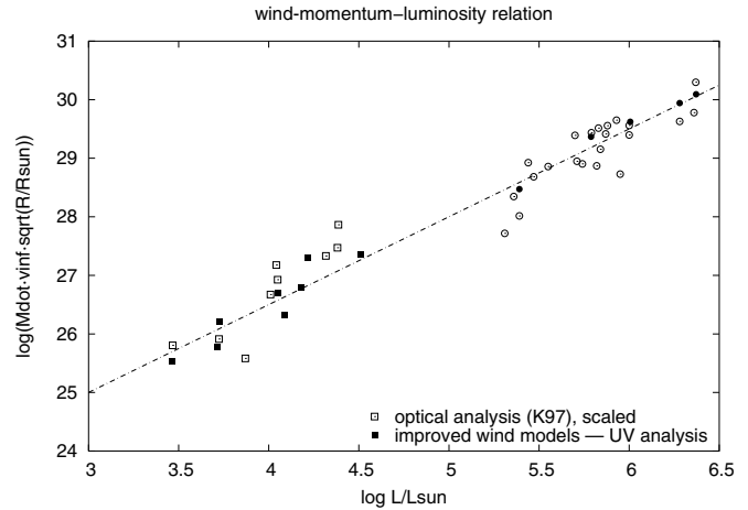
Fig. 6. The wind-momentum–luminosity relation for CSPNs (lower left) based on our values determined from the UV spectra (filled squares). The open squares are the values from Kudritzki et al. (1997) scaled to our determined radii, thus eliminating the need for an a-priori assumption for the radii, as was done by Kudritzki et al. (see text). Compared to Fig. 1 the result is striking: now there is good agreement between the optical and UV mass loss rate determinations.
