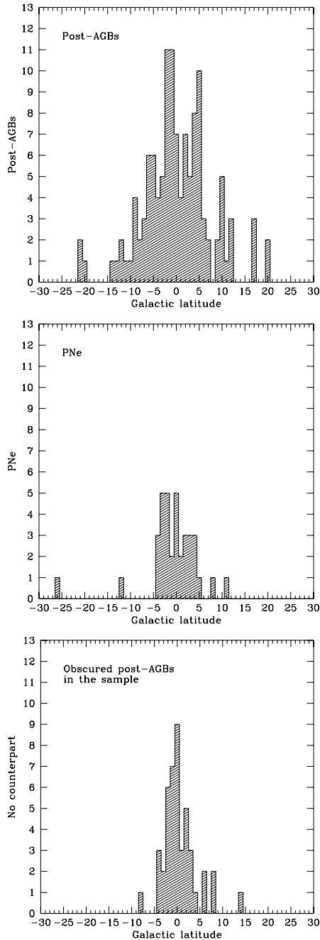
Fig. 1. Galactic latitude distribution of optically bright post-AGB stars, PNe, and obscured post-AGB stars identified in the sample.
