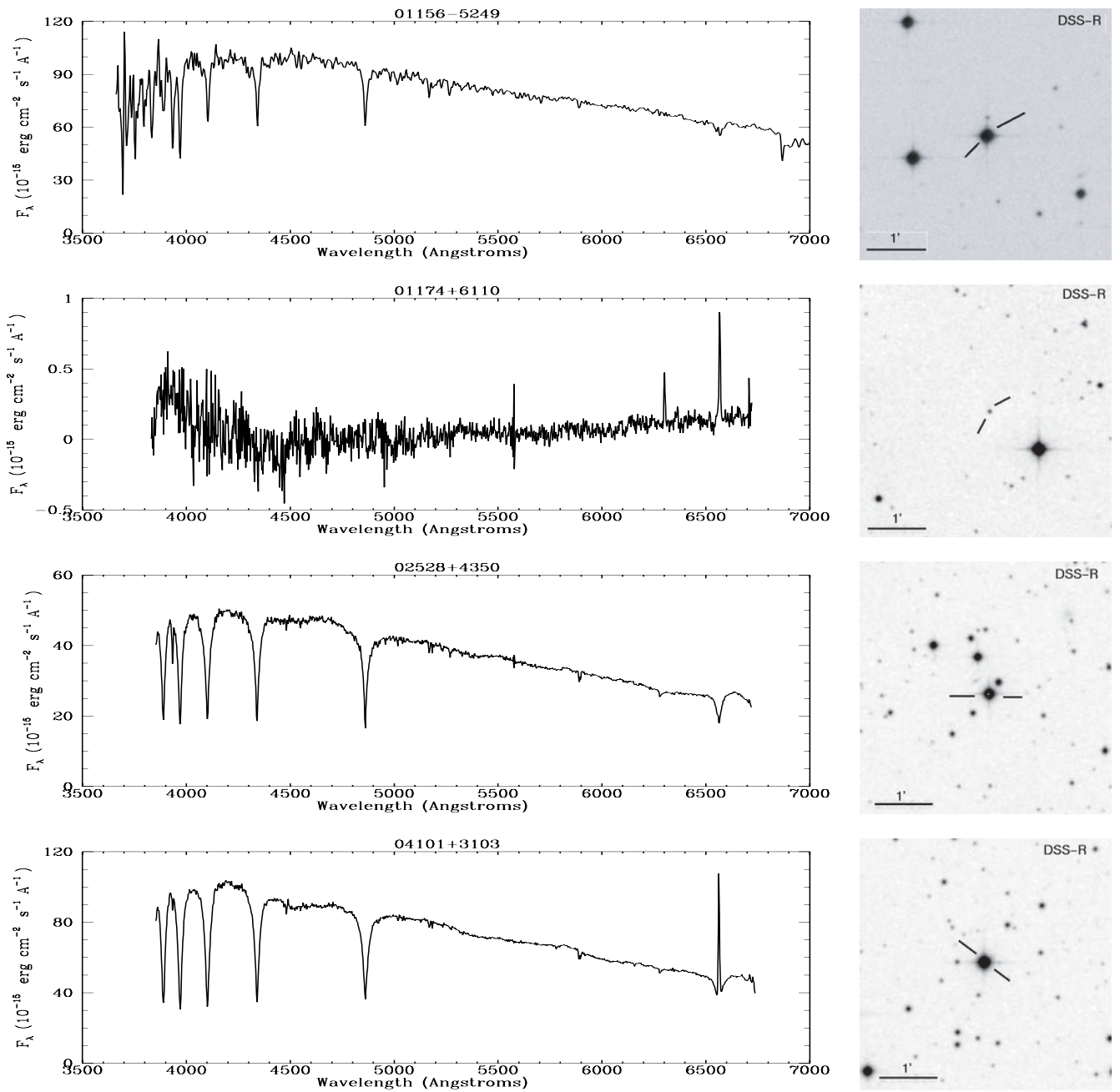
Fig. D.1. Spectra of the objects classified as young stars in the sample together with their corresponding identification charts.
