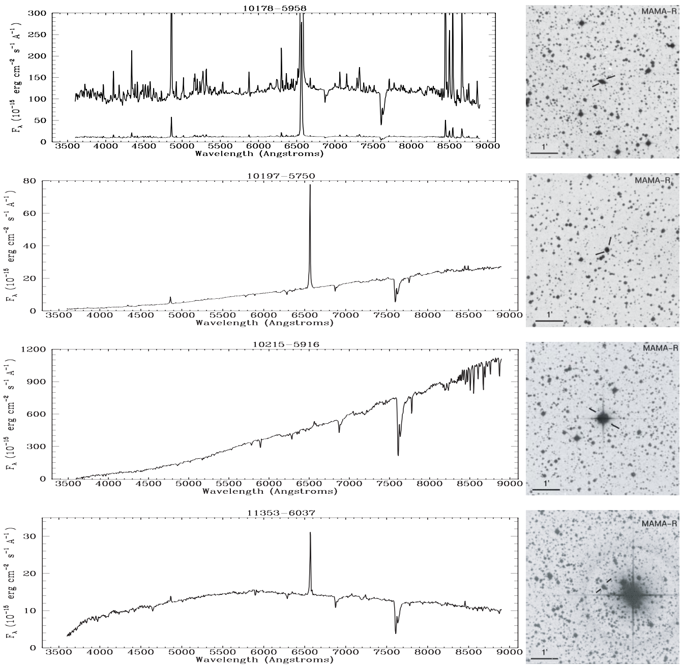
Fig. B.1. Spectra of the transition objects together with their corresponding identification charts.
