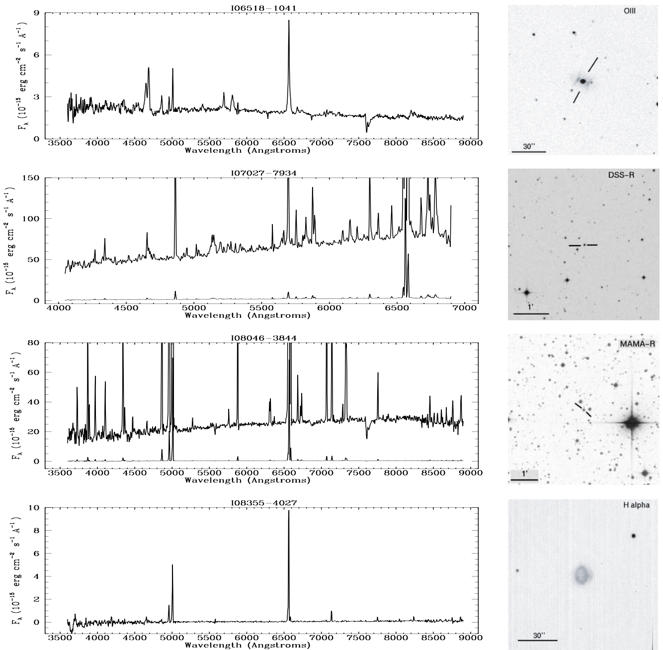
Fig. C.1. Spectra of the PNe in the sample together with their corresponding identification charts.
