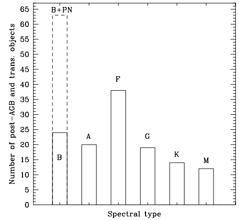
Fig. 2. Relative distribution of spectral types for the post-AGB stars in our sample.
