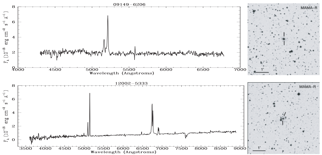
Fig. E.1. Spectra of the sources classified as galaxies in the sample together with their corresponding identification charts.
