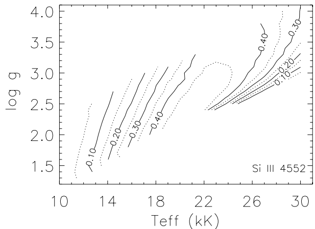
Fig. 3. As Fig. 2, but for Si III 4552. At temperatures around 23 000 K, Si III 4552 reaches a maximum in equivalent line width. The isocontours show that from this maximum, theoretical line profiles can behave similarly towards lower and higher temperatures, causing a dichotomy in the determination of the effective temperature, when we lack Si II or Si IV.
