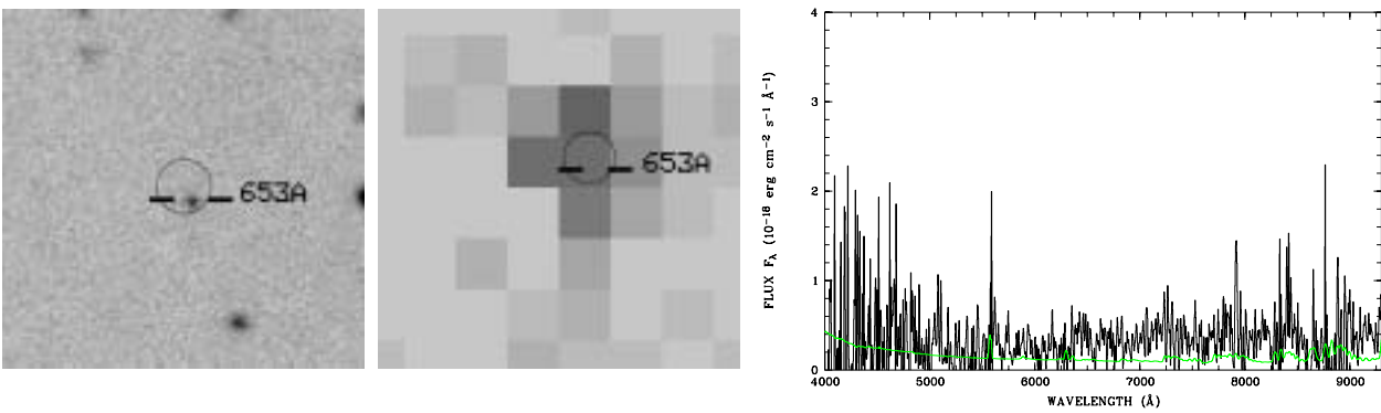
object 653A, no redshift, spectrum too noisy
