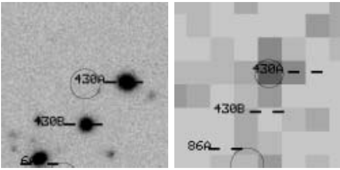
object 430B, z = 0.391
