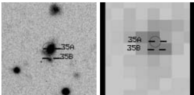
object 35A, z = 0.391
