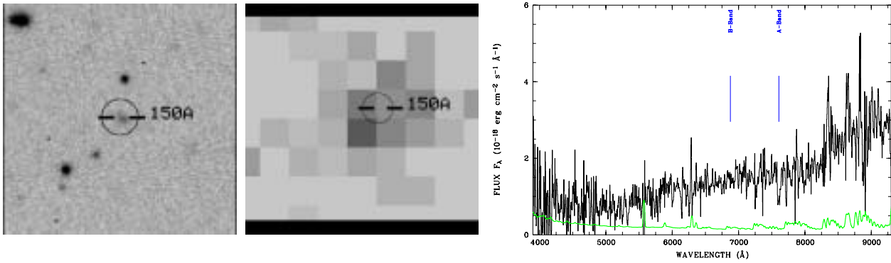
object 150A, no redshift, spectrum too noisy
