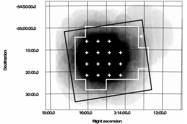
Fig. 1. Averaged mos1 and mos2 exposure map (0.5–2.0 keV) of the 4 \times 4 pointing pattern (small white crosses). The exposure time in the central region reaches 78 ks. The black rectangle shows the area covered by the WFI R -band images. The white polygon marks the area covered by the SOFI K -band images (see Sect. 2.2).
