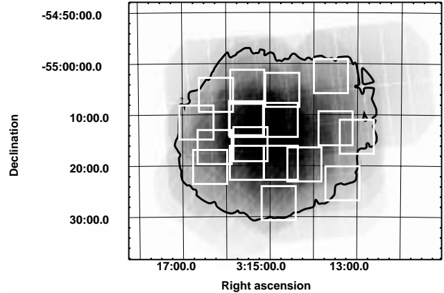
Fig. 2. PN exposure map (0.5–2.0 keV) of the 4 \times 4 pointing pattern. The exposure time in the central region reaches 35.5 ks. The area inside the black contour marks the “core sample” region where the pn-detector exposure time exceeds six ks. White rectangles show the position of the spectroscopic masks for the optical follow-up observations (see Sect. 2.4).
