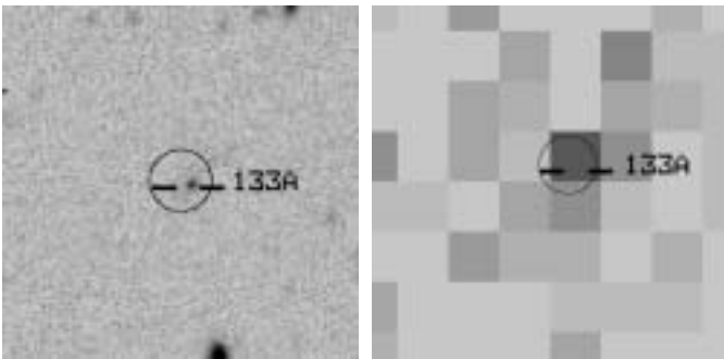
object 133A, z = 2.321
