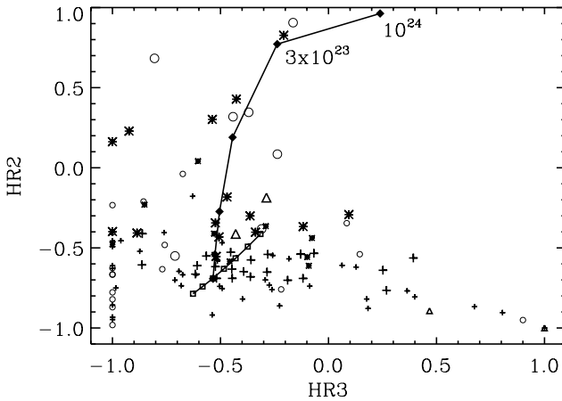
Fig. 14. X-ray diagnostic diagram based on hardness ratios. HR2 is calculated by using the 0.5–2.0 keV and 2.0–4.5 keV band, HR3 2.0–4.5 keV and 4.5–7.5 keV. Only X-ray sources that have \sigma_{HR2} < 0.3 are plotted. Labels: crosses – 63 type I AGN, asterisks – 24 type II AGN, triangles – 4 galaxies, and open circles – 24 unidentified X-ray sources with ML > 10 . Large symbols represent objects with \sigma_{HR3} < 0.3 , small symbols \sigma_{HR3} \geq 0.3 . The solid line with box symbols (at HR2 \sim HR3 \sim -0.5 ) represents an unabsorbed power-law X-ray spectrum (corrected for galactic absorption) with different photon index \Gamma = 2.4-1.2 in steps of 0.2 (squares). Different hydrogen column densities ( N_H/\text{cm}^{-2} = 10^{20}, 10^{22}, 3 \times 10^{22}, 10^{23}, 3 \times 10^{23}, 10^{24} ; see Sect. 4.4) are plotted as a solid line with diamonds for \Gamma = 2 and z = 1 .
