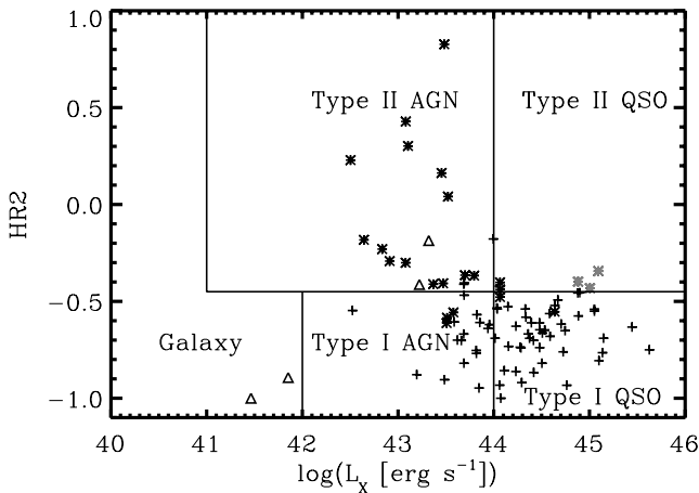
Fig. 17. Observed X-ray luminosity (0.2–10 keV) vs. hardness ratio. HR2 is calculated by using 0.5–2.0 keV & 2.0–4.5 keV bands. Only X-ray sources that have \sigma_{HR2} < 0.3 are plotted. Labels: crosses – 63 type I AGN, asterisks – 24 type II AGN (grey marked have z \geq 2.0 ), and triangles – 4 galaxies. The diagram separation into different regions is based on Szokoly et al. (2004) with an adjusted threshold in the HR2 -value.
