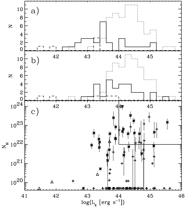
Fig. 19. a) Histogram of the absorbed (observed) X-ray luminosity (0.2–10 keV) for the core sample. Dotted line – 70 type I AGN, solid line – 30 type II AGN, and dashed line – 5 galaxies. b) Histogram of the X-ray luminosity (0.2–10 keV) corrected for intrinsic absorption (core sample). Same notation as in a) . c) Corrected X-ray luminosity (0.2–10 keV) vs. hydrogen column density (core sample). Crosses – type I AGN, asterisks – type II AGN, and triangles – galaxies. The upper right corner is suggested as being defined as the “type II QSO region” by Mainieri et al. (2002). Objects with N_{\text{H}} = 0 are set to N_{\text{H}} = 5 \times 10^{19} \text{ cm}^{-2} .
