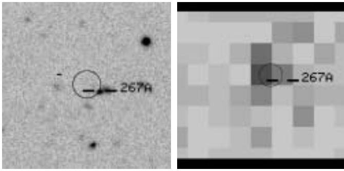
object 267A, z = 1.495
