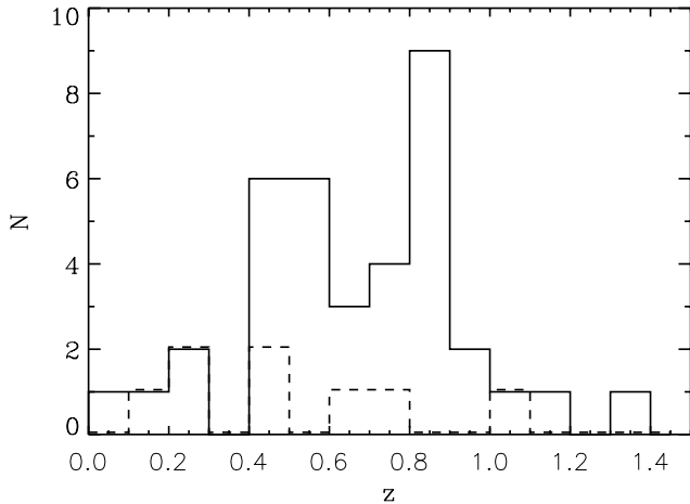
Fig. 22. Redshift distribution of the additional objects. Labels: solid line – 37 NELGs, and dotted line – 8 optically normal galaxies.
