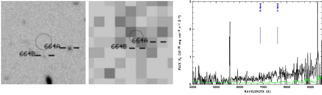
object 664A, no redshift, spectrum too noisy
