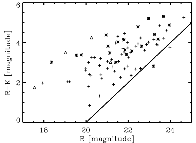
Fig. 21. Colour magnitude diagram of spectroscopically classified X-ray sources. Labels: crosses – 56 type I AGN, asterisks – 20 type II AGN, and triangles – 4 galaxies. Only objects with detections in both R and K are included. The absence of blue, faint objects (below the solid line) is due only to the K -magnitude limit.
