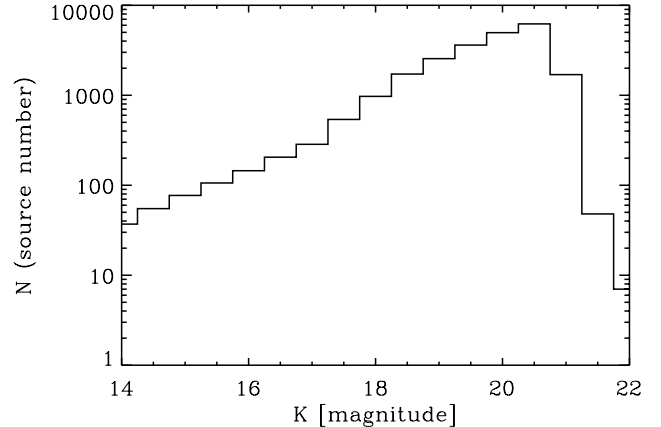
Fig. 6. Histogram of the K-band magnitudes in the NTT-SOFI images. Completeness in detecting objects is lost for K > 20.5 .
