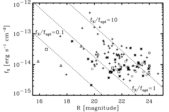
Fig. 20. Observed X-ray flux (0.2–10 keV) vs. R -band magnitude. Dashed lines indicate the f_{\text{X}}/f_{\text{opt}} values 0.1, 1.0, and 10. Labels: crosses – 63 type I AGN, asterisks – 25 type II AGN, triangles – 5 galaxies, rectangles – 3 stars, and circles – 21 spectroscopically unidentified sources ( R -band lower limits are plotted as circles at R = 24 ). Note that for a few objects of the core sample no WFI R -magnitudes were available and therefore these are not plotted here.
