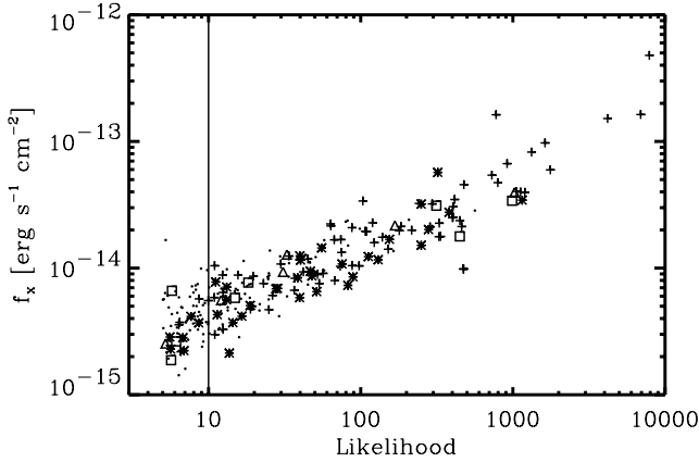
Fig. 13. Likelihood vs. 0.2–10 keV X-ray-flux of the 252 central X-ray sources (pn-detector exposure time \geq 6 ks). Crosses mark type I AGN, asterisks type II AGN, triangle galaxies, and rectangles stars. Dots indicate X-ray sources with no spectroscopic classification. The vertical line indicates ML = 10 .
