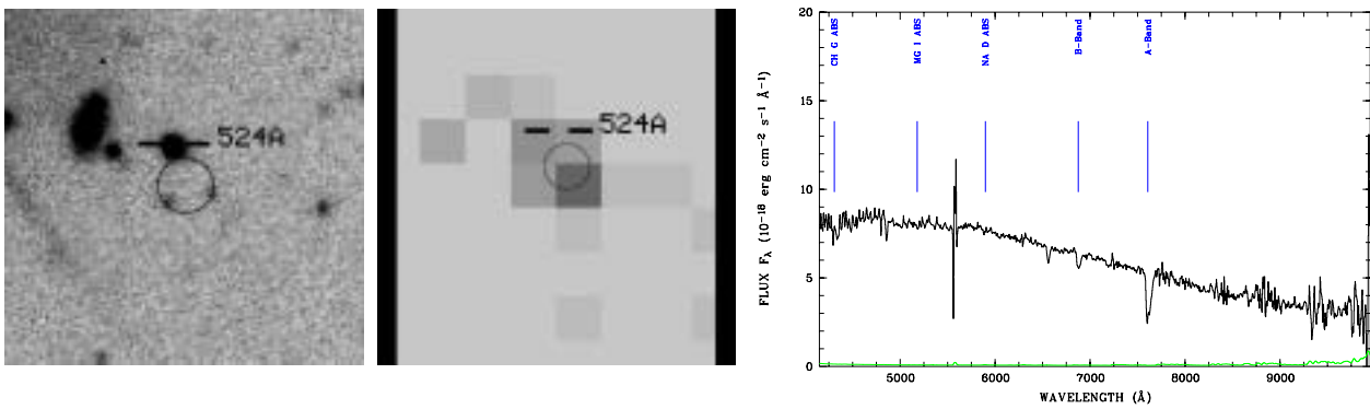
object 524A, z = 0.000
