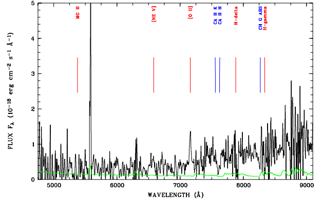
Fig. 7. Optical atmospheric absorption corrected, wavelength and flux calibrated spectrum for X-ray source 480. The black spectrum marks the object's spectrum. The green line (see the online colour version of the manuscript) shows the error spectrum. Possible emission and absorption features in the spectrum are labelled. The spectral feature at 5580 \text{\AA} is spurious due to incomplete subtraction of a night sky line.
