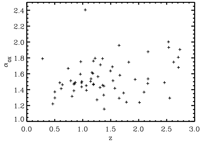
Fig. 23. UV to X-ray spectral index \alpha_{OX} vs. redshift for type I AGN in the core sample.
