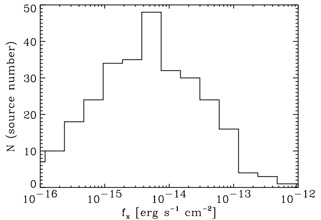
Fig. 3. 0.2–10 keV X-ray flux histogram of the 328 XMM-Newton detected X-ray sources in the Marano Field. Up to an X-ray flux of f_{\text{X}} \sim 5 \times 10^{-15} \text{ erg cm}^{-2} \text{ s}^{-1} (turnover flux) we detect more and more sources. Below that X-ray flux the detection rate decreases dramatically.
