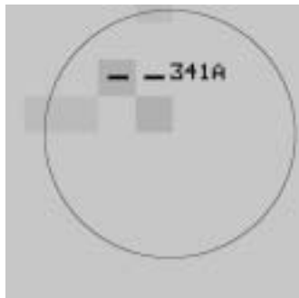
object 341A, z = 2.784
