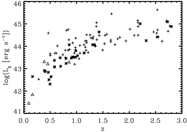
Fig. 16. Observed X-ray luminosity (0.2–10 keV) vs. redshift. Labels: crosses – 70 type I AGN, asterisks – 30 type II AGN, and triangles – 5 galaxies.
