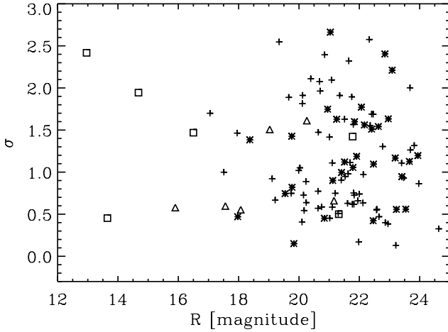
Fig. 11. WFI R -band magnitude vs. difference in X-ray and optical position scaled to a 1\sigma_X position error with a systematic X-ray position error of 0.7 arcsec. Crosses mark type I AGN, asterisks type II AGN, triangle galaxies, and rectangles stars.
