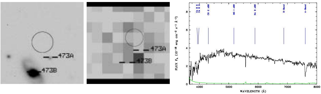
object 473A, z = 0.000
