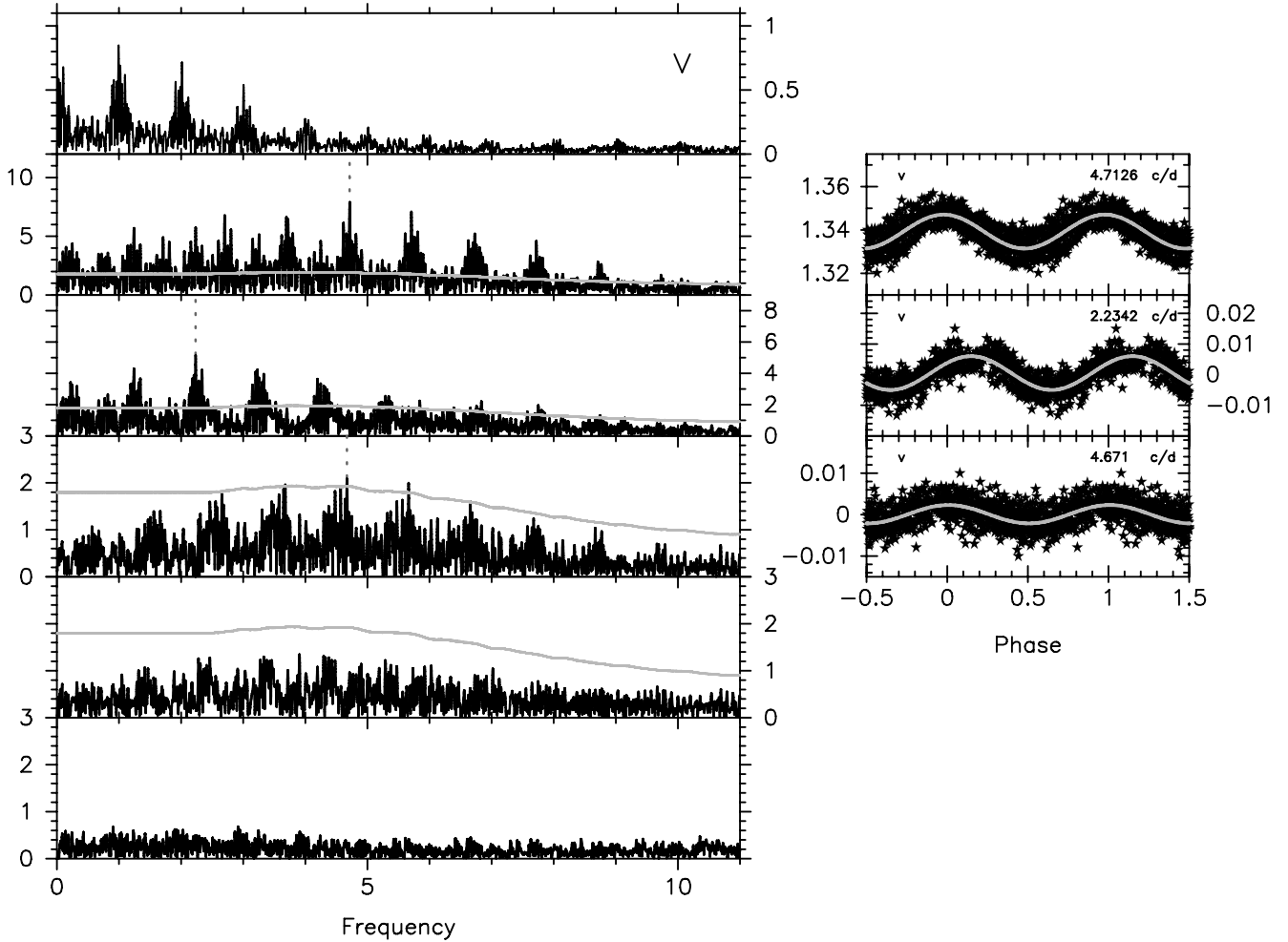
Fig. 2. Left panel: Window function ( top ) and SCARGLE periodograms of V2104 Cyg at different stages of the frequency search in the Strömgren v filter. The amplitudes are expressed in mmag. The detected frequencies \nu_1 = 4.7126 \pm 0.0004 \text{ d}^{-1} , \nu_2 = 2.2342 \pm 0.0005 \text{ d}^{-1} and \nu_3 = 4.671 \pm 0.001 \text{ d}^{-1} are indicated by dashed vertical lines. The last but one bottom periodogram shows the final residuals after prewhitening with \nu_1 , \nu_2 and \nu_3 . The light grey horizontal lines represent the ( S/N > 3.6 )-level. In the bottom periodogram we present the variability of the comparison stars, illustrating that they are constant at the level of a few 0.1 mmag. Right panel: Phase diagrams of the 3 detected frequencies in the v filter. Black stars correspond to observations and the grey full lines represent the least-squares fit. The amplitudes are expressed in mag.
