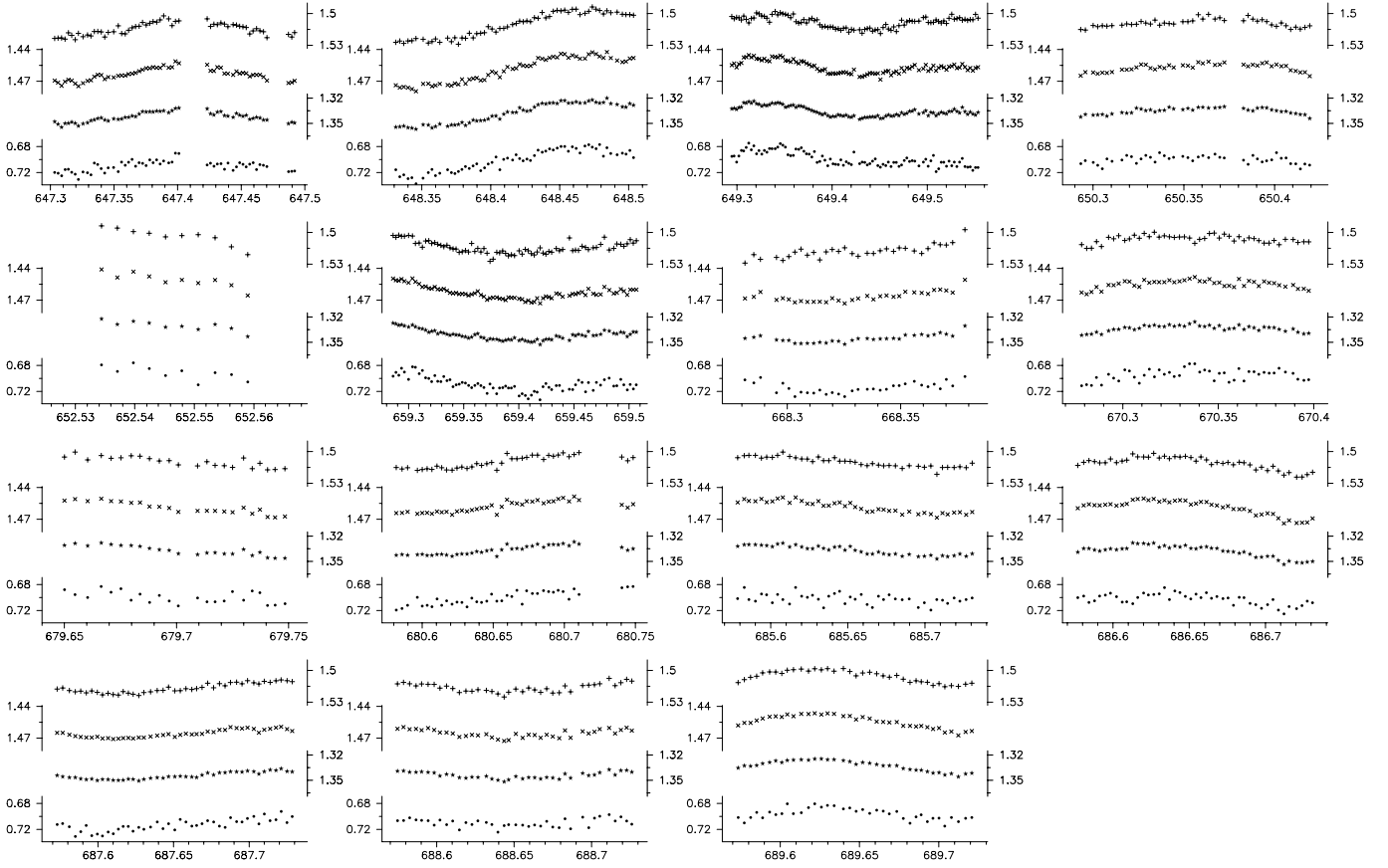
Fig. 1. Light curves of V2104 Cyg obtained at SNO and SPMO in October–November 2005. The u (dots), v (stars), b (crosses) and y (+) magnitude differences are plotted in time (HJD-2453000). Note the difference in scale between the u and vby data: tickmarks in the u filter and vby filters correspond to 0.04 mag and 0.03 mag respectively.
