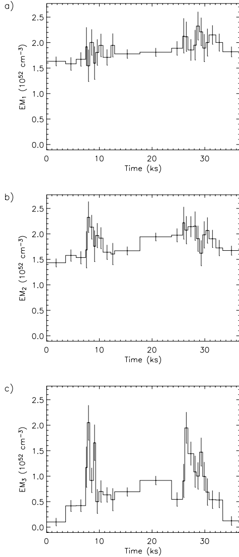
Fig. 10. Time-evolution obtained for the emission measure of the three thermal components. Note that the time-resolution is the same as that shown in Fig. 5.
