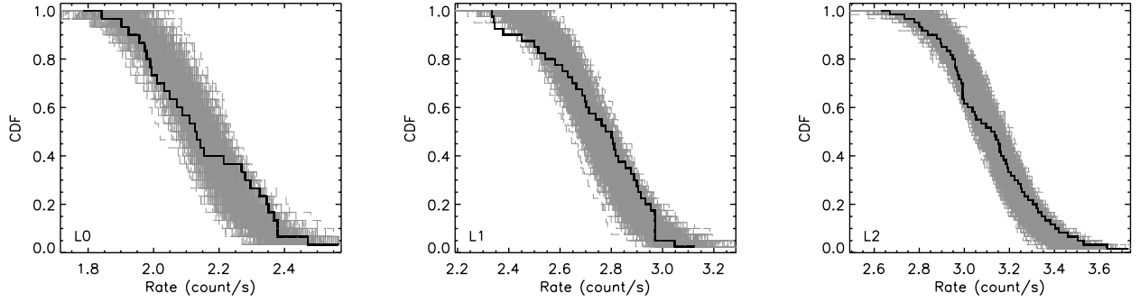
Fig. 2. Cumulative distribution function of the count-rates observed in the regions L0, L1 and L2 (solid black line) compared to those simulated by supposing a constant source with count-rate equal to the mean value ( R_m[\text{Li}] ) in the given region (dashed area).
