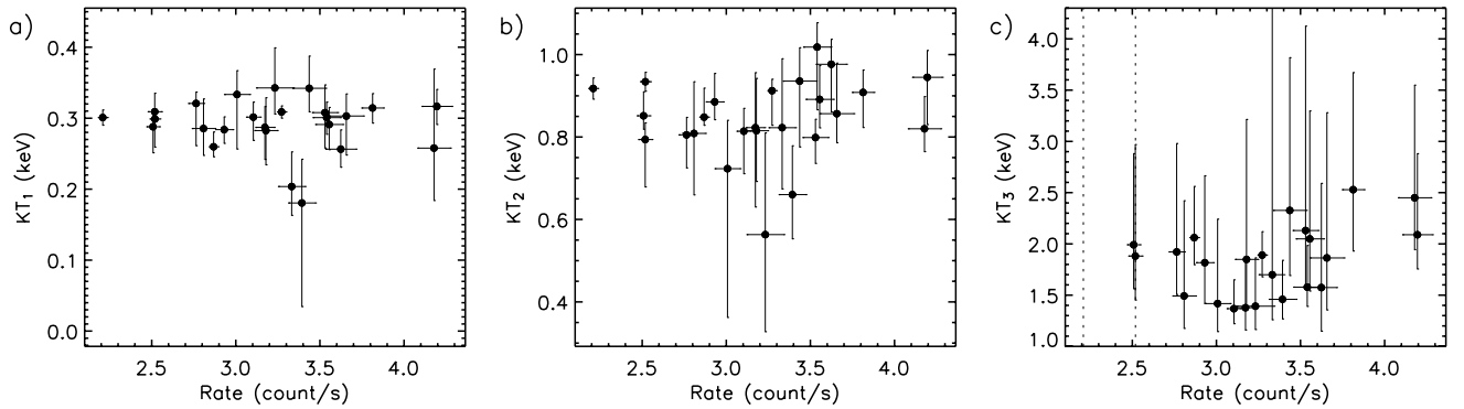
Fig. 8. Coronal temperatures (obtained with the 3- T model) vs. count-rate. In the KT_3 panel, a dashed line marks the time-segments for which this temperature could not be constrained (see text). Note that no significant changes in the temperature values are observed even at flare maxima (points with the highest count-rates).
