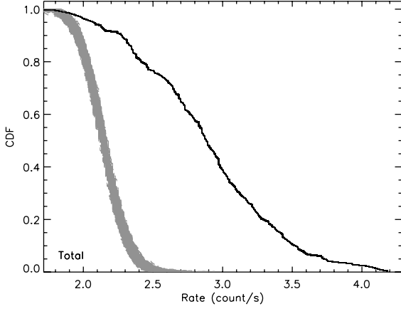
Fig. 4. Cumulative distribution function of the count-rates detected in the whole observation of CC Eri (solid black line) compared to those simulated by supposing a constant source with count-rate equal to the quiescent value (dashed area).
