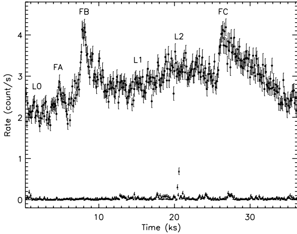
Fig. 1. Source (upper region) and background (lower region) light curves of CC Eri as observed with the EPIC-PN detector for the energy band 0.5–10.0 keV and a temporal binning of 100 s. The labels FA, FB and FC refer to the detected flares while L0, L1 and L2 designate different emission levels where no clear flare activity was observed.
