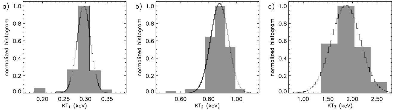
Fig. 9. Distribution of the three temperatures that characterize the corona of CC Eri during the XMM-Newton observation. The corresponding Gaussian fits are also plotted.
