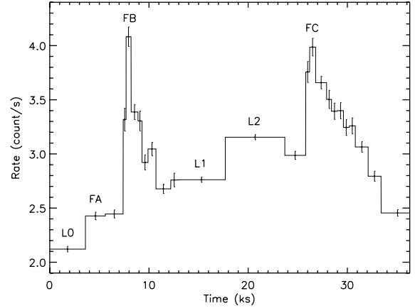
Fig. 5. Rebinned light curve of CC Eri for the energy band 0.5–10.0 keV.
