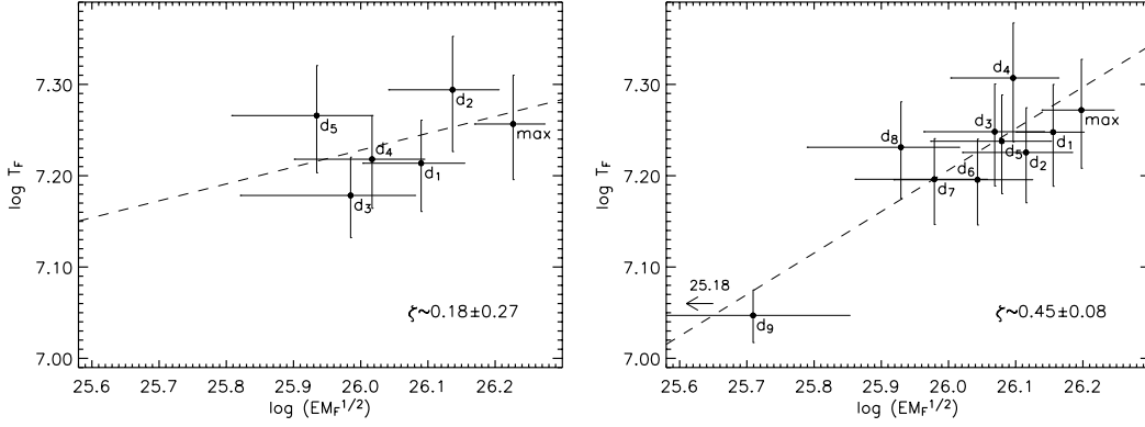
Fig. 12. Density-temperature ( \log n_F - \log T_F ) diagram of the variable component (see text) for the decay phase of flares FB (left panel) and FC (right panel). EM_F^{1/2} has been used as a proxy for the density. Numbers indicate the time-evolution of the values. The point at the flare maximum (max) is also plotted. For each flare, the dashed line shows the best linear fit to the decay data. The derived slopes ( \zeta ) are also given.
