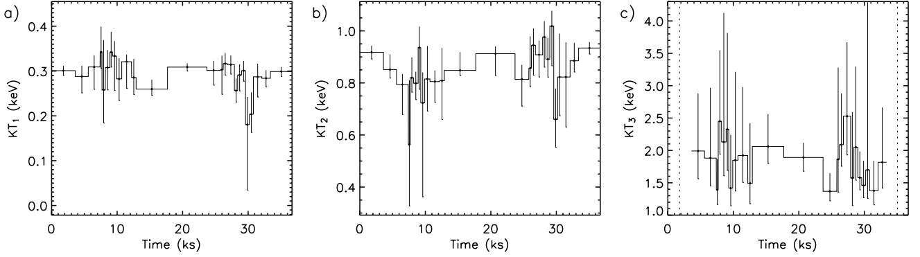
Fig. 7. Time-evolution of the coronal temperatures obtained with the 3- T model. In the KT_3 panel, a dashed line marks the time-segments for which this temperature could not be constrained (see text). Note that the time-resolution is the same as that shown in Fig. 5.
