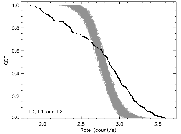
Fig. 3. Cumulative distribution function of the observed count-rates obtained for L0, L1 and L2 altogether (solid black line) compared to those simulated by supposing a constant source with count-rate equal to the mean value of these three regions (dashed area).
