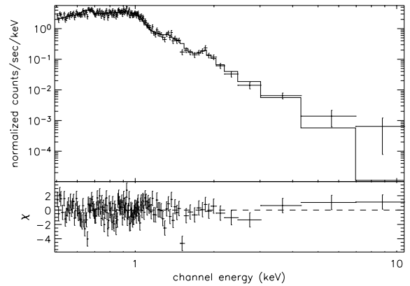
Fig. 6. X-ray spectrum of the quiescent state of CC Eri (L0). The best fit (2- T APEC model) is also shown with a solid line.
