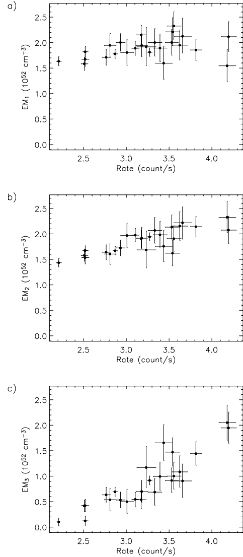
Fig. 11. Emission measure of the three thermal components vs. count-rate.
