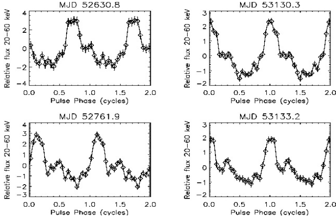
Fig. 9. ISGRI (20–60 keV) mean pulse profiles of SAX J2103.5+4545 generated by combining profiles from individual INTEGRAL ScWs.
