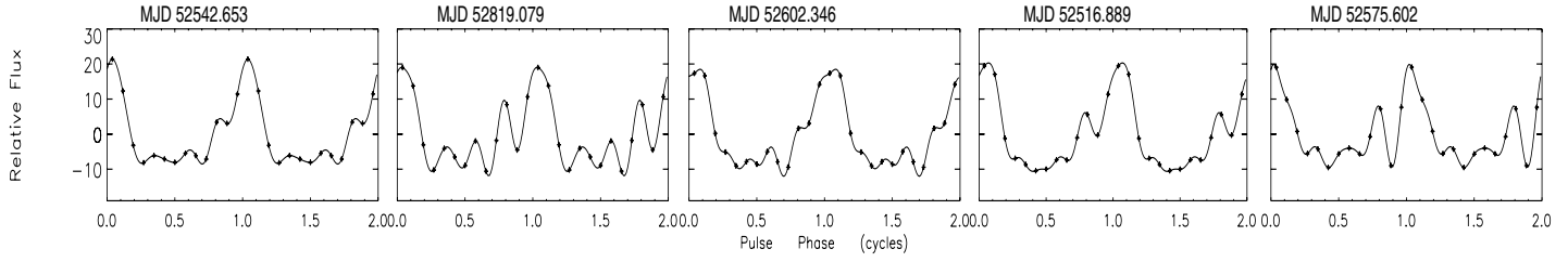
Fig. 3. RXTE PCA 2–60 keV pulse profiles at the same luminosity state ( L \approx 2 \pm 0.6 \times 10^{36} \text{ erg s}^{-1} ; see Fig. 4 bottom).
