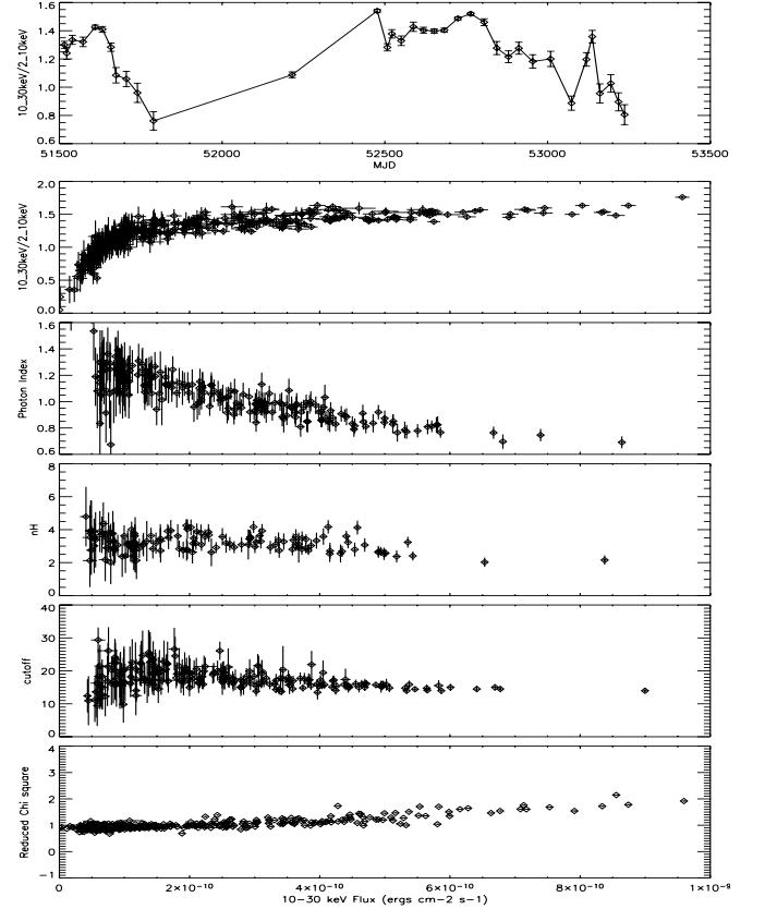
Fig. 11. Top. Long-term hardness ratios history. From middle to bottom: HR-intensity diagram and spectral parameters evolution vs. intensity.
