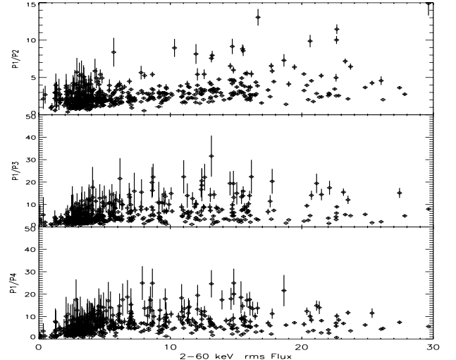
Fig. 6. From top to bottom, the ratio of the main to the second, the third and the fourth peak plotted vs. luminosity (2–60 keV rms flux). We have rejected few observations with large uncertainties for clarity.
