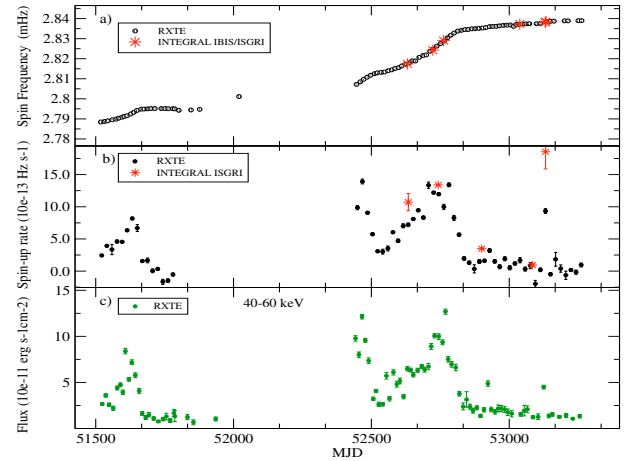
Fig. 12. Top: long-term frequency history. Middle: averaged spin-up rates history. Bottom: 40–60 keV RXTE HEXTE averaged fluxes. A spin-up rate and X-ray flux correlation was found, confirming that an accretion disk during periastron passage is present.
