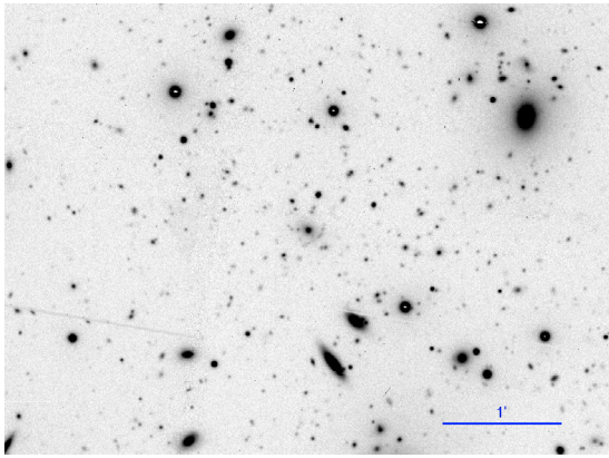
Fig. 4. Combined R -band image of the galaxy associated with the radio source SUMSS J033057-522811 in the centre of the NE X-ray peak. The total exposure time is 360 s. Note the arc to the Southwest of the galaxy. The scale of 1' is indicated on the image.
