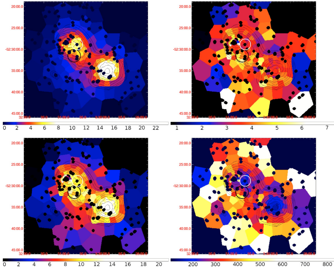
Fig. 5. Top left: the projected emission measure per arcminute, in units of 10^{64} \text{ cm}^{-3} \text{ arcmin}^{-2} , integrated along the line of sight, after the emission of the background cluster was subtracted. Top right: temperature map derived from spectral fitting in units of keV. Bottom left: map of the pressure derived from the best fit temperature and emission measure, assuming a length scale along our line of sight of 1 Mpc. The units are 10^{-12} \text{ dyne cm}^{-2} . Bottom right: map of the entropy derived from the best fit temperature and emission measure, assuming a length scale along our line of sight of 1 Mpc. The units are \text{keV cm}^2 . The white and black circles indicate the high surface brightness low entropy region and the region at the centre of the galaxy distribution, respectively. These we use for subsequent spectral analysis. The X-ray isophotes from the wavelet decomposed image are overlotted.
