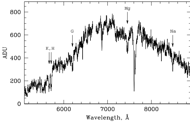
Fig. 3. Spectrum of the galaxy associated with the radio source SUMSS J033057-522811 in the centre of the NE X-ray peak. On the y -axis we plot arbitrary count units (ADU). Lines, used for redshift determination, are shown with arrows.
