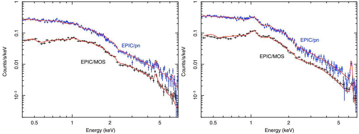
Fig. 2. The spectrum of the NE ( left panel ) and SW ( right panel ) X-ray peak extracted from circular region with a radius of 1.5' . The continuous line represents the best fit model. The EPIC/pn and the coadded EPIC/MOS spectra are indicated. The position of the Fe K line in the spectrum from the NE peak shows that the emitting cluster is at a redshift of z = 0.44 .
