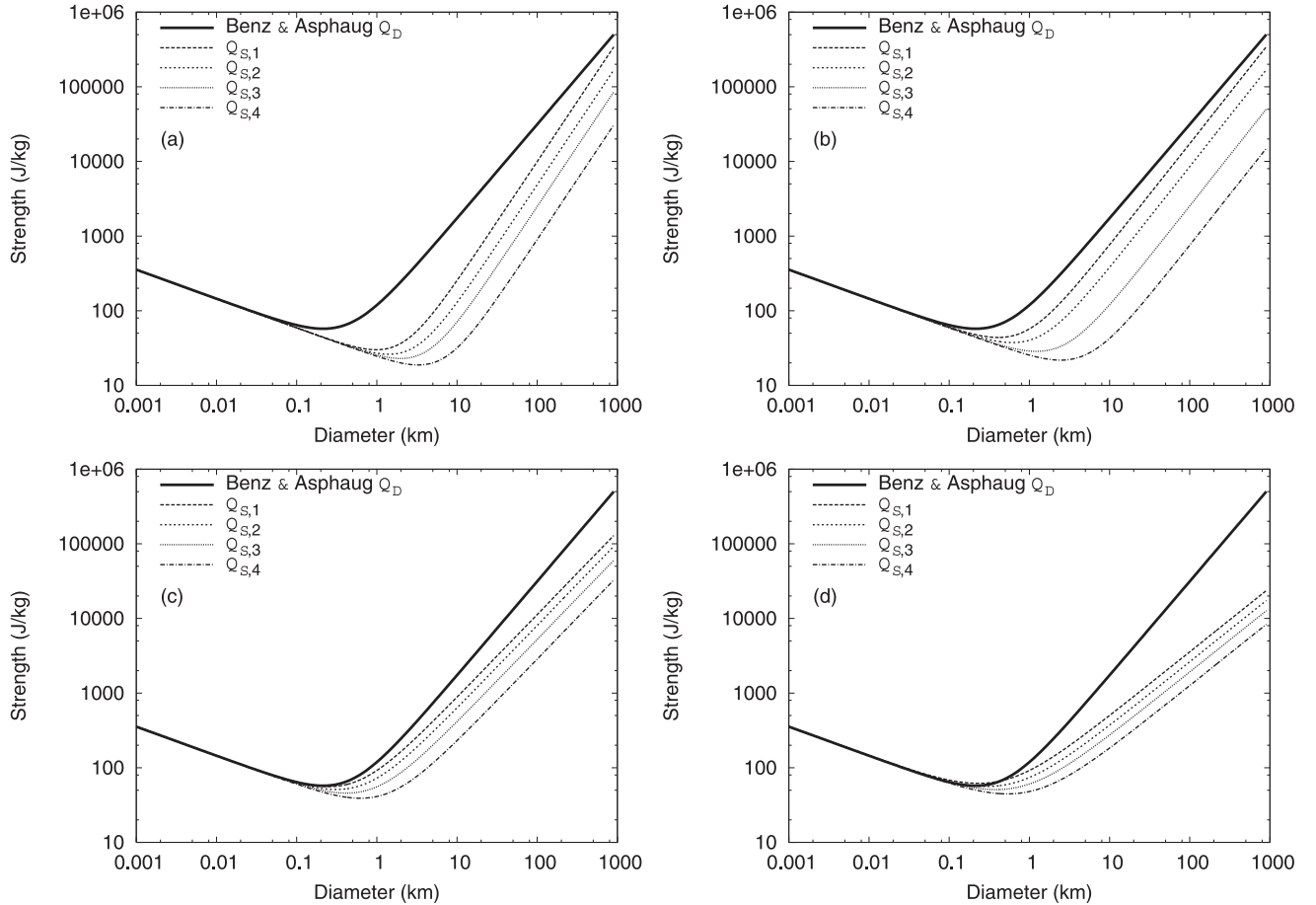
Fig. 3. Asteroid strength. The dashed lines represent the Q_S laws used in our simulations. From a ) to d ), the Q_S curves show decreasing slopes in the “gravity-scaled regime” covering all the possibilities from small to large gaps between Q_S and the Q_D law from Benz & Asphaug (1999) for icy bodies at 3 \text{ km s}^{-1} , which is plotted as a solid line.
