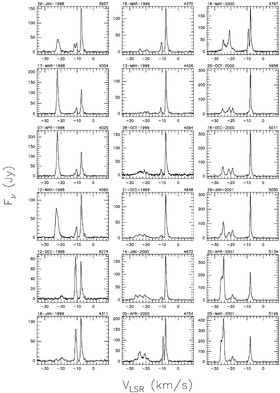
Fig. A.30. a continued.
