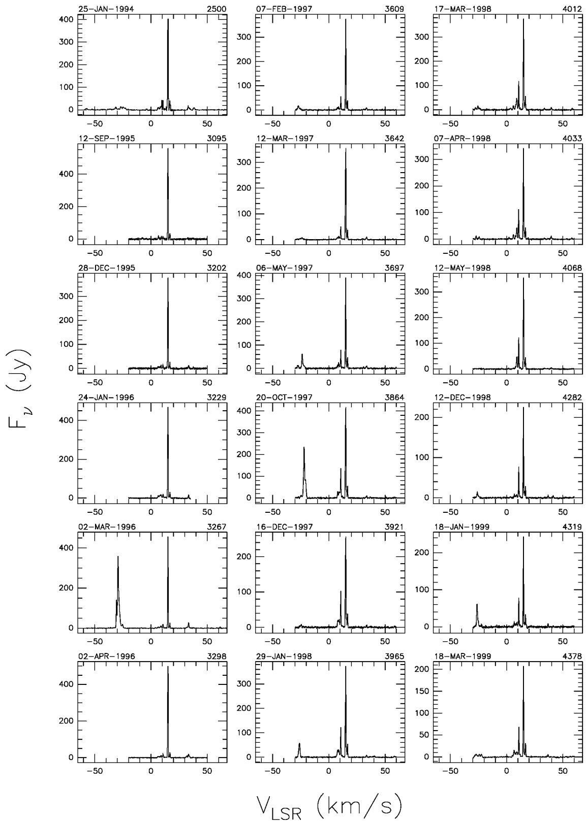
Fig. A.28. a continued.
