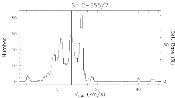
Fig. A.17. f Rate-of-occurrence plot for source Sh 2-255/7. The scale to the right refers to the dotted histogram, the scale to the left to the solid line histogram. The vertical solid line marks the velocity of the associated thermal molecular gas.
