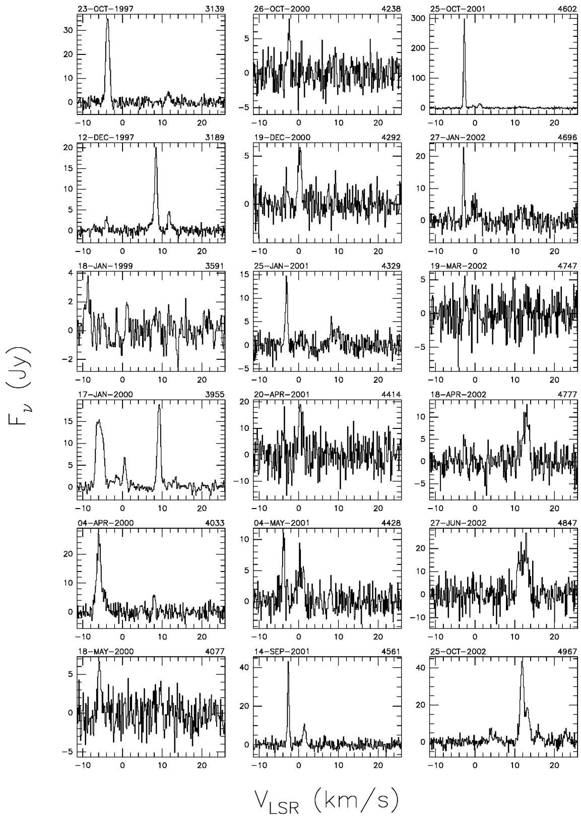
Fig. A.12. a continued.
