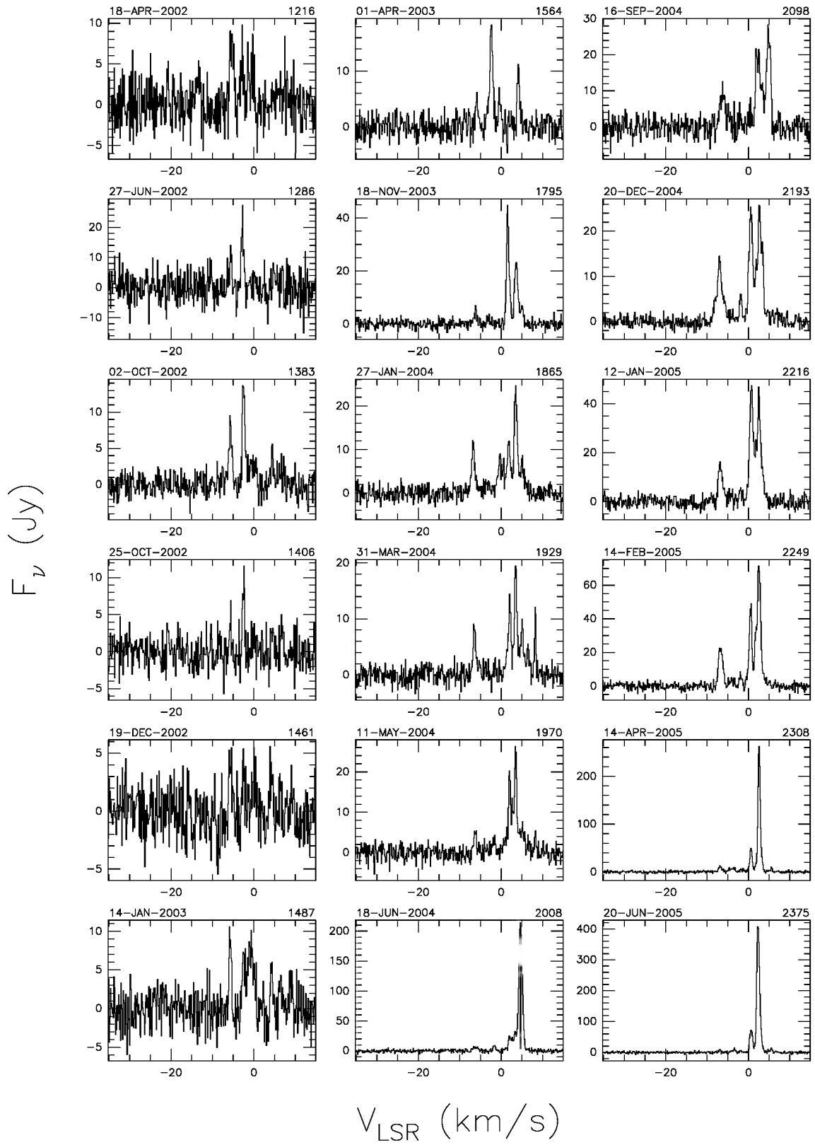
Fig. A.15. a continued.
