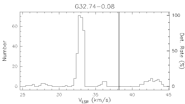
Fig. A.22. f Rate-of-occurrence plot for source G32.74-0.08. The scale to the right refers to the dotted histogram, the scale to the left to the solid line histogram. The vertical solid line marks the velocity of the associated thermal molecular gas.
