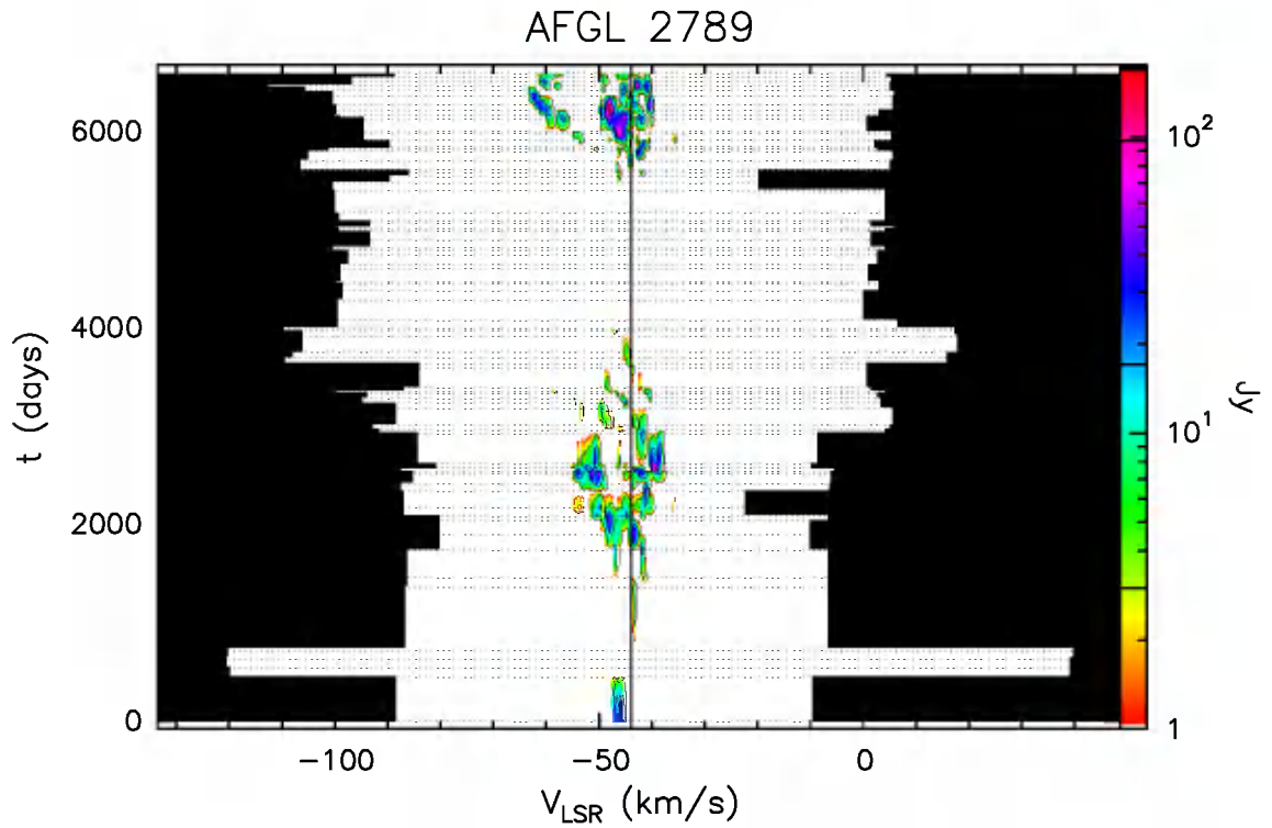
Fig. A.33. b Velocity–time–flux density full plot for source AFGL 2789. The vertical solid line indicates the velocity of the associated thermal molecular gas. The flux density scale is shown by the bar on the right. In this bar the three lines give the flux density of the drawn contours.
