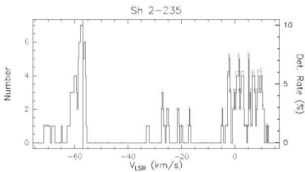
Fig. A.10. f Rate-of-occurrence plot for source Sh 2-235. The scale to the right refers to the dotted histogram, the scale to the left to the solid line histogram. The vertical solid line marks the velocity of the associated thermal molecular gas.
