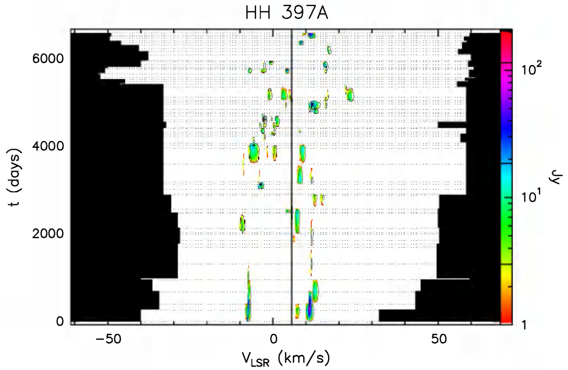
Fig. A.12. b Velocity–time–flux density full plot for source HH 397A. The vertical solid line indicates the velocity of the associated thermal molecular gas. The flux density scale is shown by the bar on the right. In this bar the three lines give the flux density of the drawn contours.
