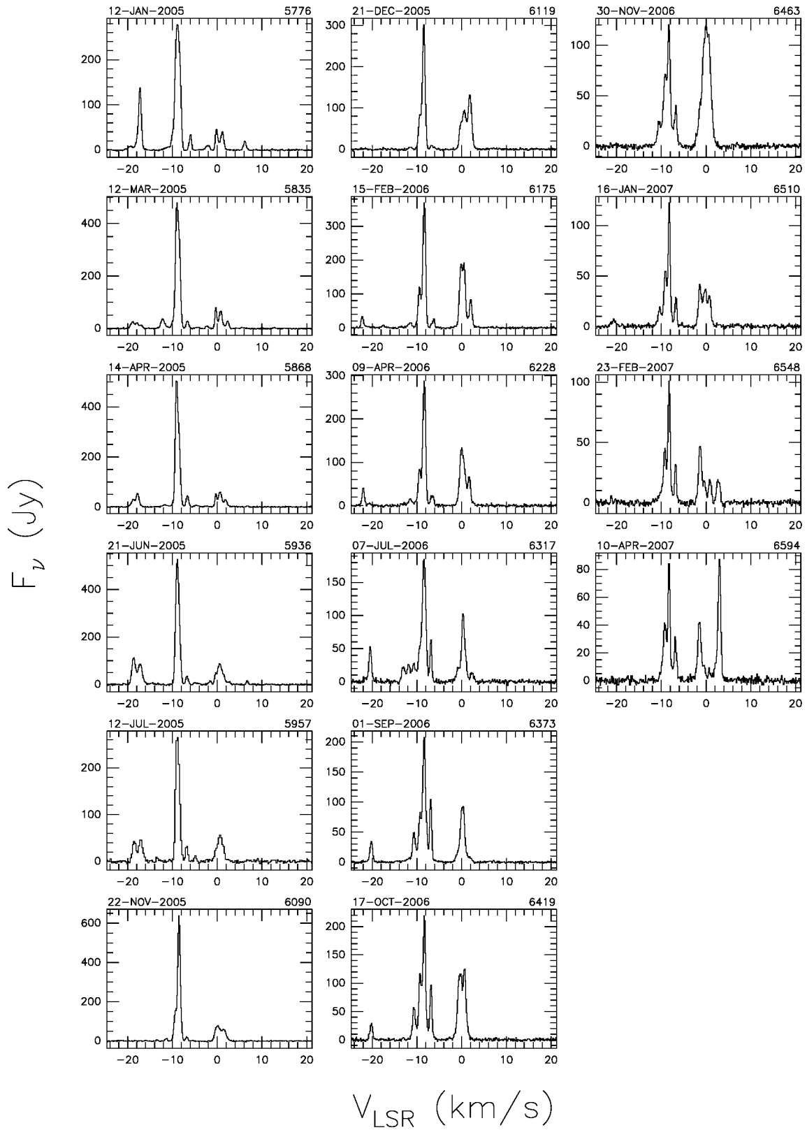
Fig. A.34. a continued.
