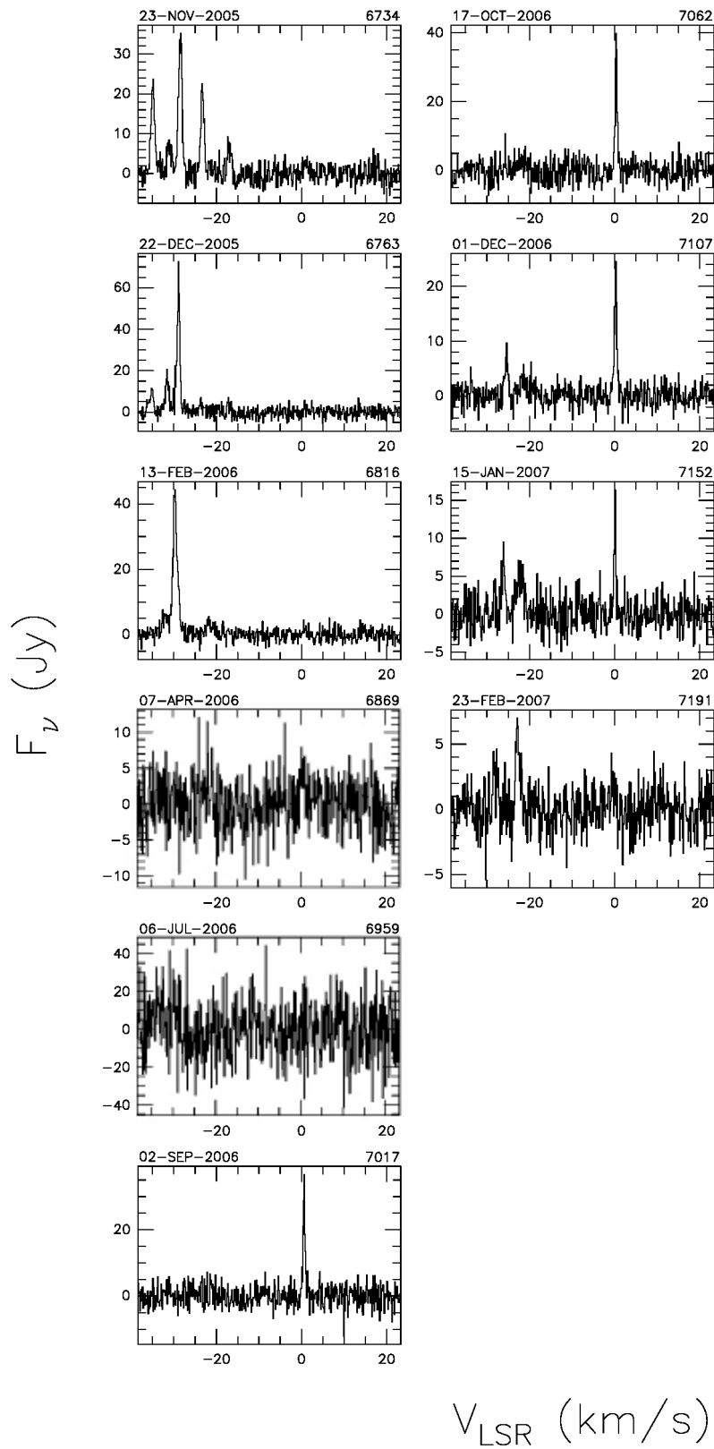
Fig. A.16. a continued.
