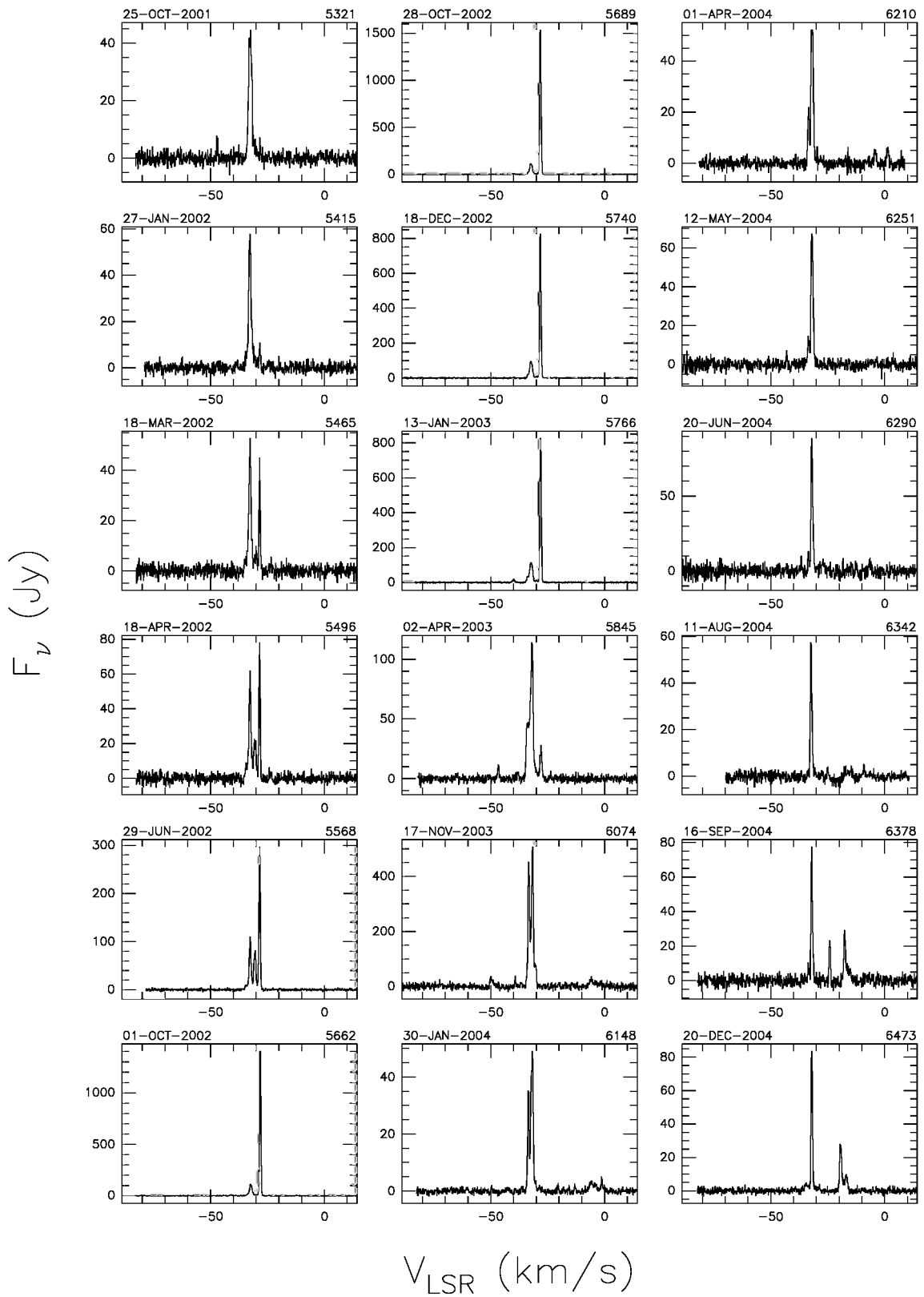
Fig. A.1. a continued.
