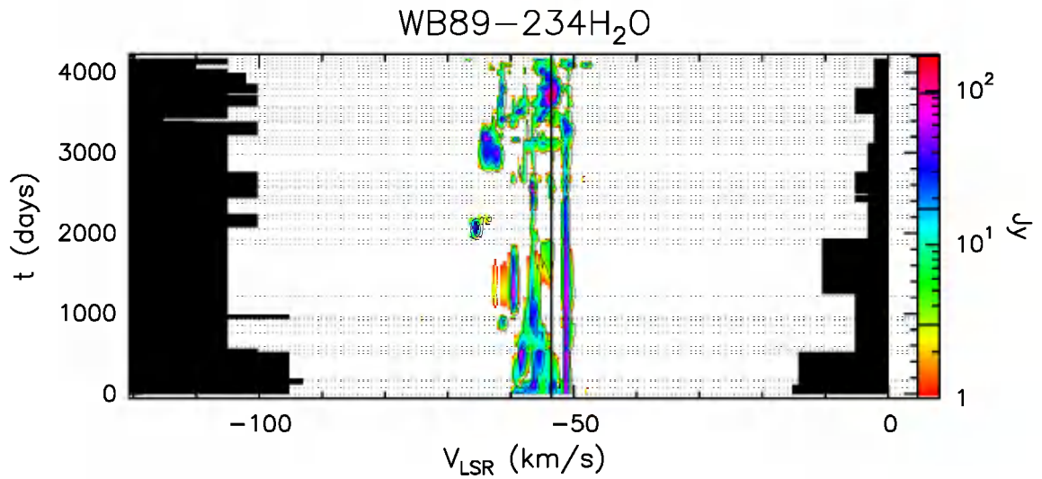
Fig. A.40. b Velocity–time–flux density full plot for source WB89-234H 2 O. The vertical solid line indicates the velocity of the associated thermal molecular gas. The flux density scale is shown by the bar on the right. In this bar the three lines give the flux density of the drawn contours.
