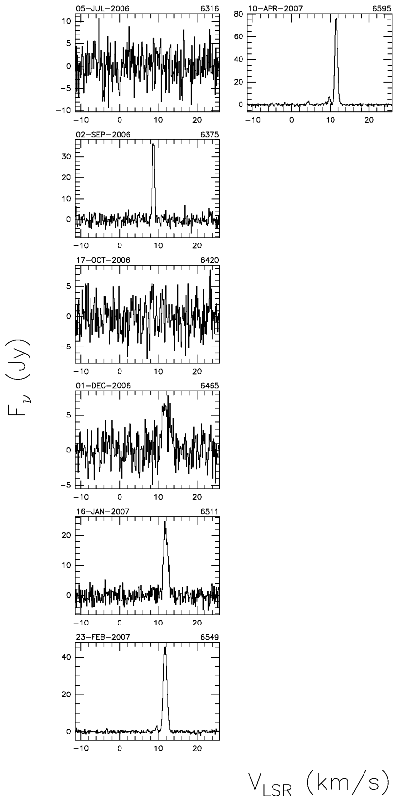
Fig. A.12. a continued.
