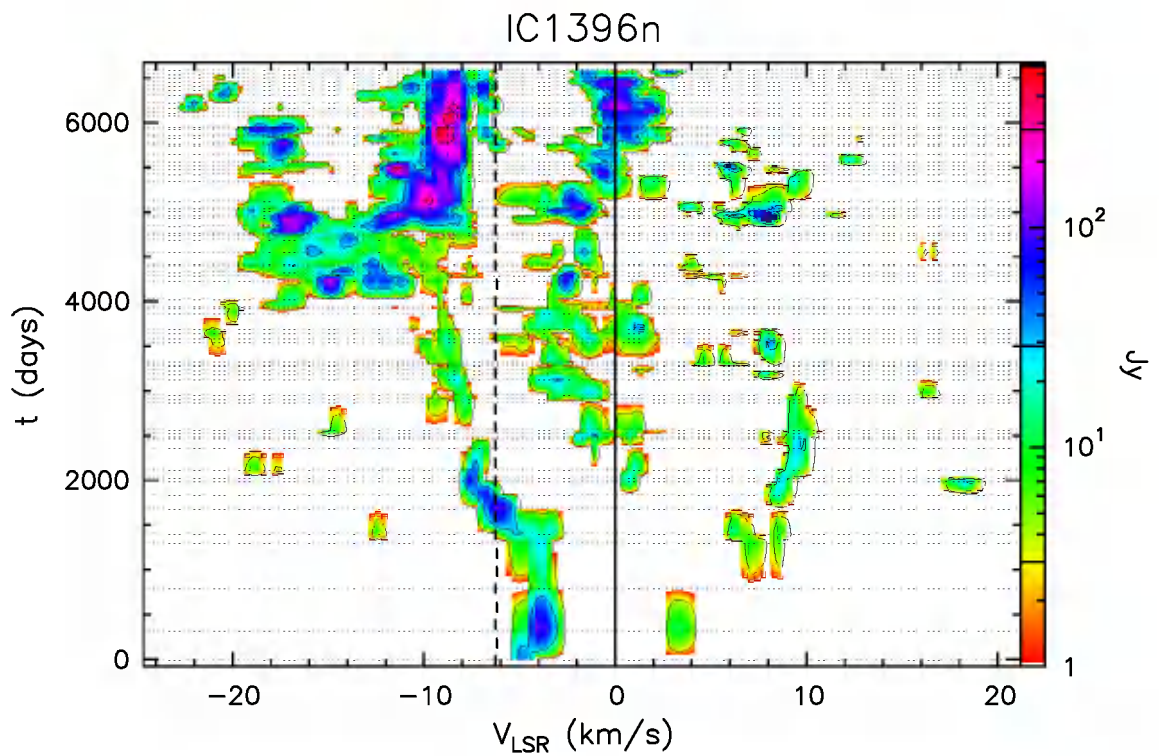
Fig. A.34. c Same as previous figure, but “zoomed” to velocity range over which emission has been detected.
