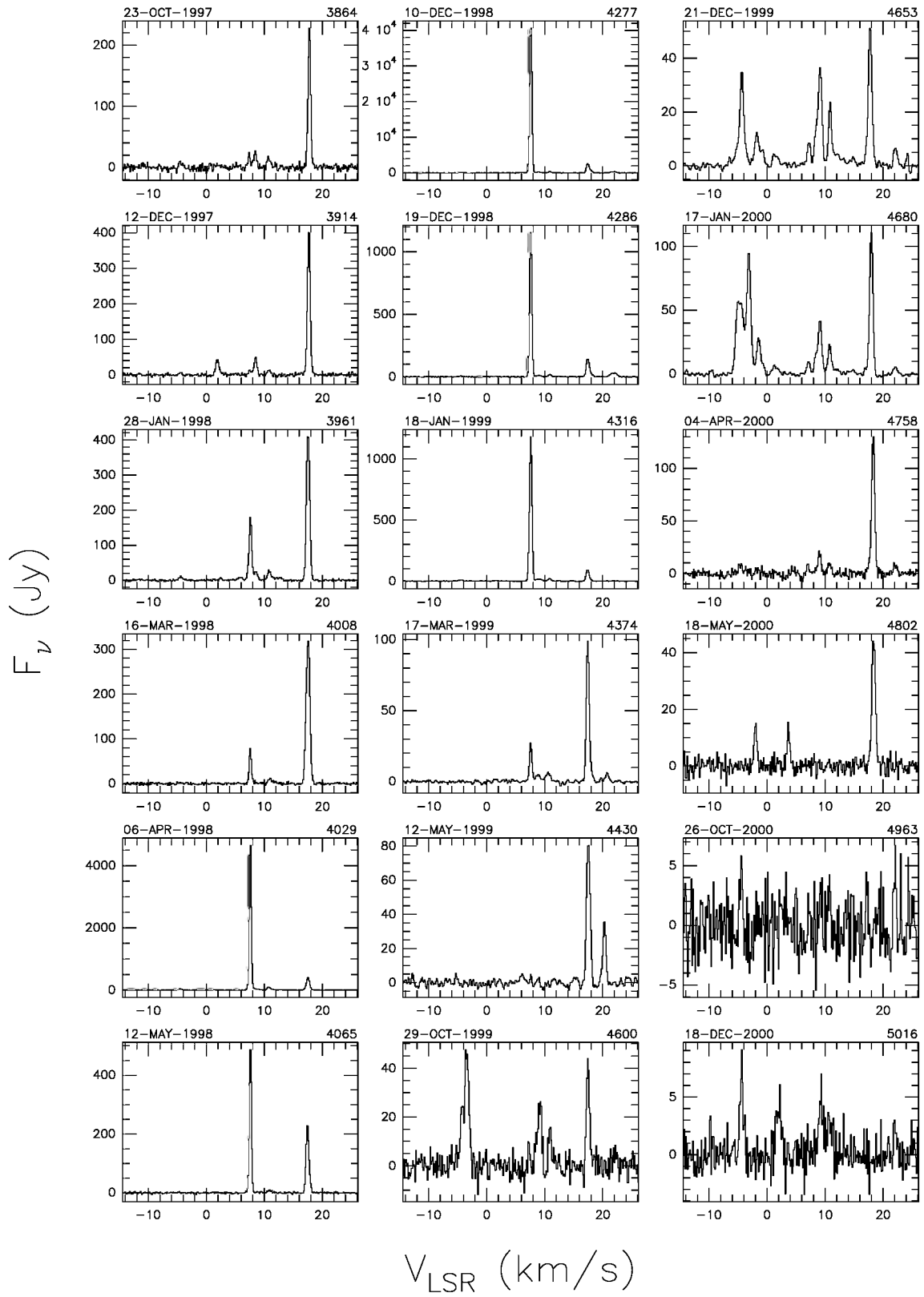
Fig. A.7. a continued.
