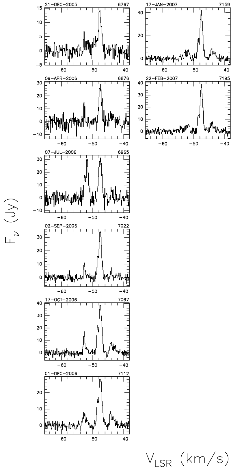
Fig. A.42. a continued.
