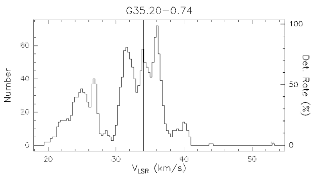
Fig. A.24. f Rate-of-occurrence plot for source G35.20-0.74. The scale to the right refers to the dotted histogram, the scale to the left to the solid line histogram. The vertical solid line marks the velocity of the associated thermal molecular gas.
