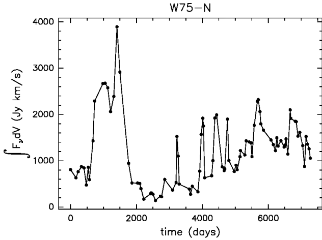
Fig. 7. The integral of the flux density over the observed velocity range as a function of time for the source W75-N.
