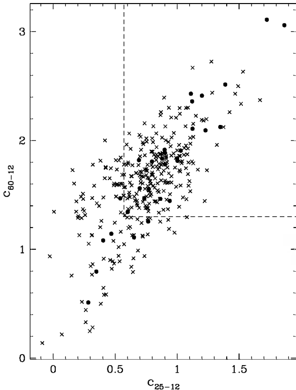
Fig. 1. Colour-colour ( C_{a-b} = \log(F_a/F_b) , F_a = IRAS flux in band a \mu\text{m} ) diagram of the IRAS counterparts of the sources listed in Table 1 (●), compared to that of a larger sample of H 2 O masers of SFR type (a merger of Comoretto et al. 1990; Brand et al. 1994; and Valdetarro et al. 2001) (×). The dashed box defines the location of Ultracompact HII regions (Wood & Churchwell 1989).
