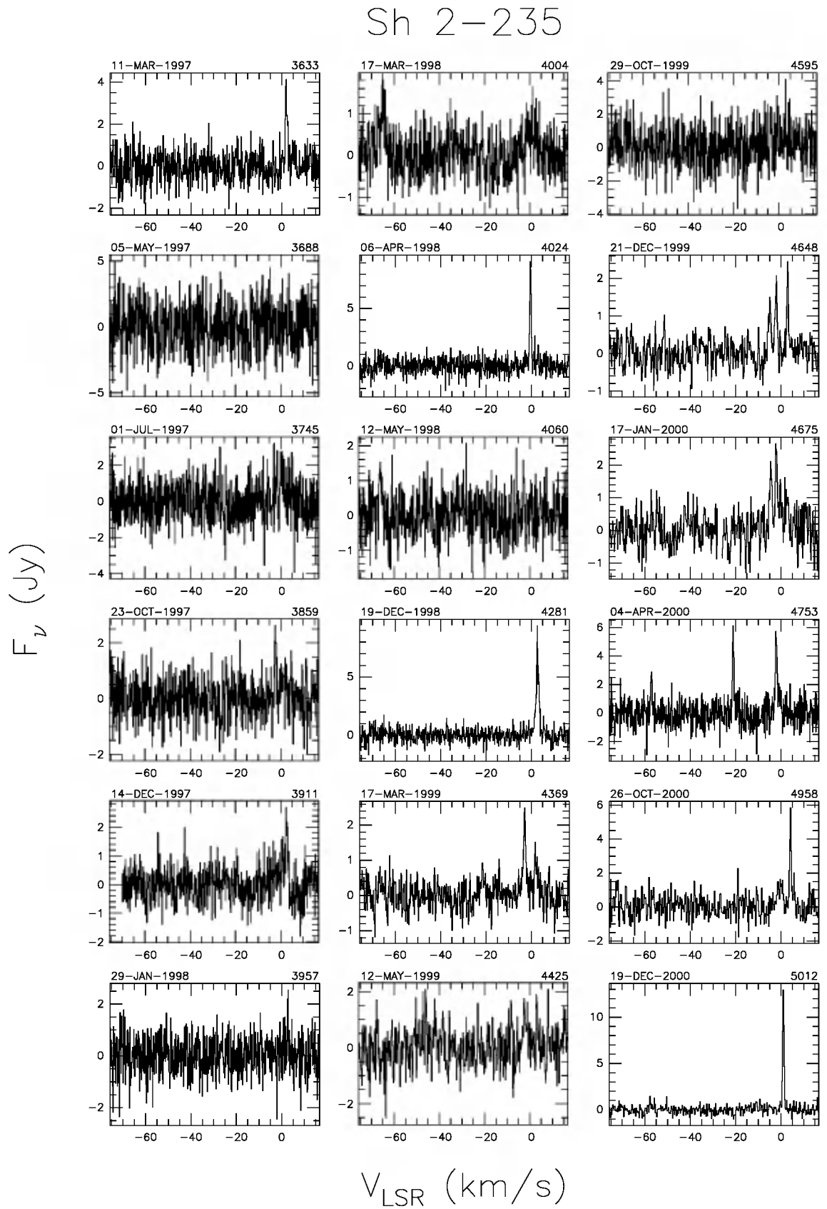
Fig. A.10. a continued.
