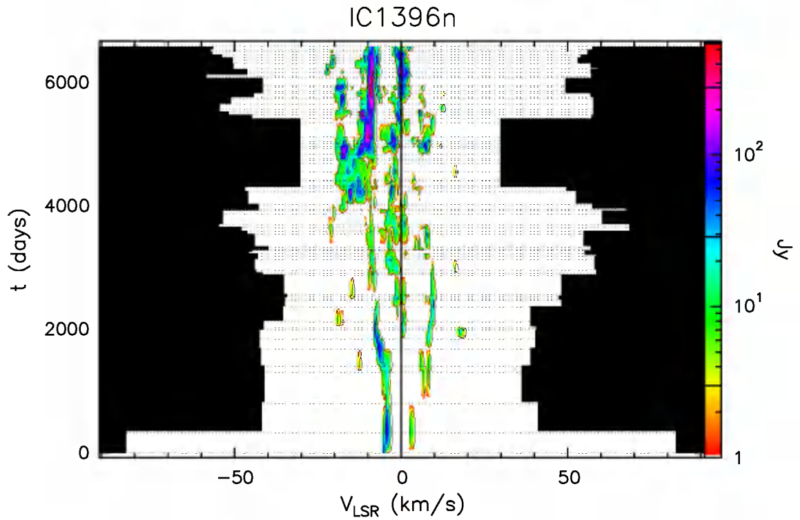
Fig. A.34. b Velocity–time–flux density full plot for source IC1396n. The vertical solid line indicates the velocity of the associated thermal molecular gas. The flux density scale is shown by the bar on the right. In this bar the three lines give the flux density of the drawn contours.
