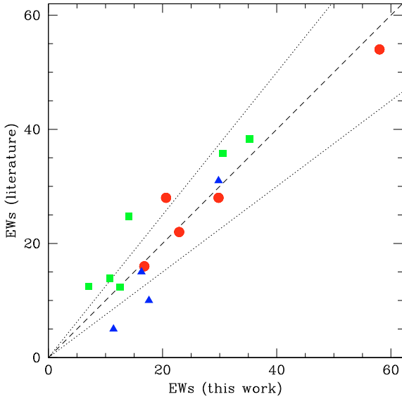
Fig. 1. Comparison between our measured EWs and values in the literature. Circles: Aller & Jugaku (1958), but excluding uncertain values, triangles: Gies & Lambert (1992), squares: Kilian & Nissen (1989). The 1:1 relationship is shown as a dashed line, while the two dotted lines indicate a discrepancy reaching 25%.
