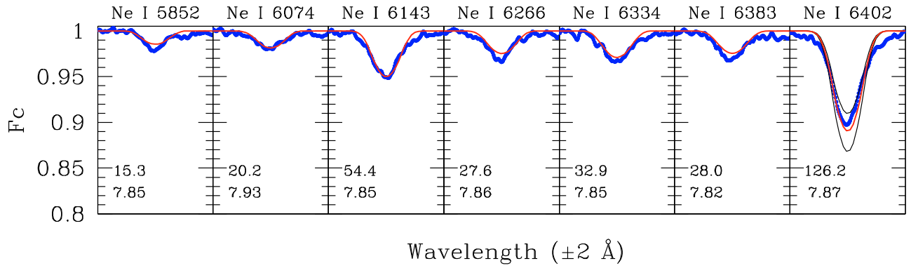
Fig. A.1. Comparison for \iota CMA between the observed (blue dots) and the synthetic profiles (red line) computed for the abundance given by the corresponding spectral line (value given in every panel, along with the measured EW ; see Table B.1). The synthetic spectra were convolved with a rotational broadening function with v \sin i = 32 \text{ km s}^{-1} (Morel et al. 2008). The effect of varying the abundance by \pm 0.1 dex is shown for Ne I \lambda 6402 . The spectral range in each panel is 4 \text{ \AA} .
