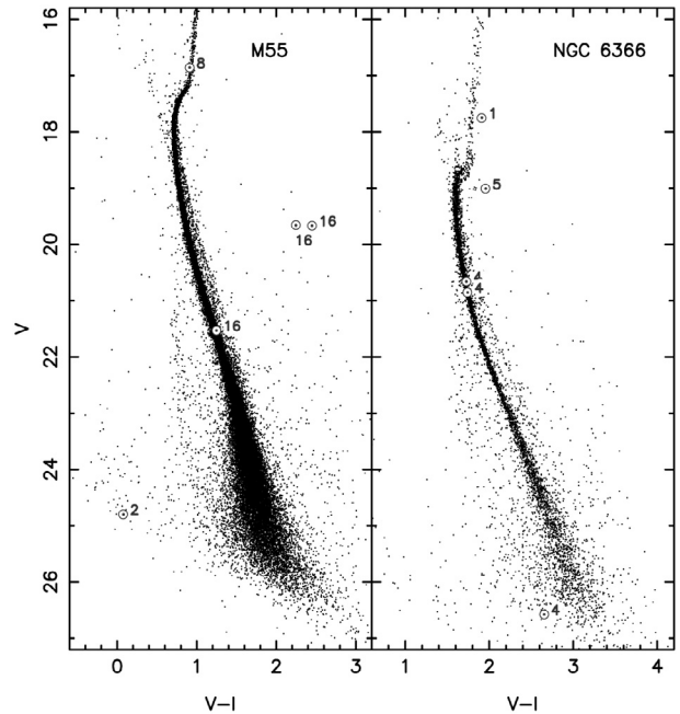
Fig. 5. Optical color–magnitude diagrams for M 55 and NGC 6366 constructed from the Anderson et al. (2008) photometry. Candidate optical counterparts to the Chandra X-ray sources are indicated and numbered.
