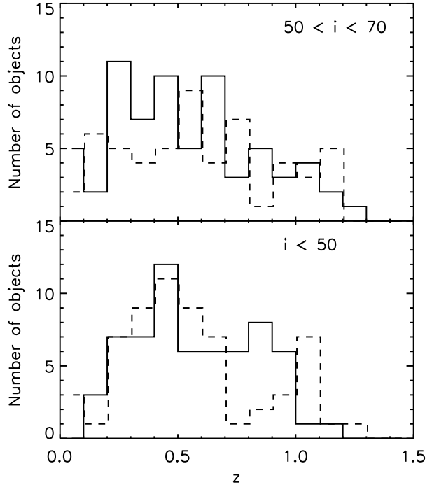
Fig. 1. Distribution of redshifts for the high-inclination and low-inclination samples. Solid line: spectroscopic redshifts. Dashed line: photometric redshifts.
