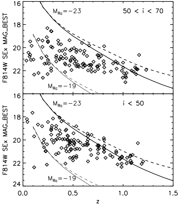
Fig. 2. Distribution of F814W apparent magnitude (SETRACTOR MAG_BEST magnitudes) vs. redshift for the high-inclination and low-inclination samples. Thick solid and dashed lines: apparent magnitude of Sa and Sd galaxy models (from GISSEL03 library, Bruzual & Charlot 2003; Chabrier 2003 IMF, solar metallicity and exponential SFR with \tau = 3 and 30 Gyr), respectively, for an R -band absolute magnitude equal to -23 . Thin lines: the same but for M_R = -19 .
