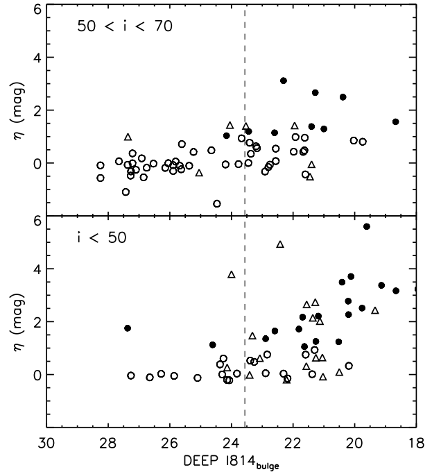
Fig. 5. Central prominence index \eta vs. DEEP GIM2D apparent bulge F814W magnitude for the high-inclination and low-inclination samples. Filled circles: galaxies with \eta > 1 (prominent bulges). Open circles: galaxies with \eta < 1 . Triangles: galaxies morphologically classified as mergers.
