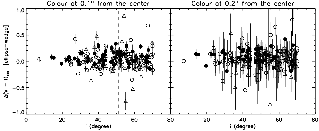
Fig. 9. Differences between colours calculated by ellipse method and the colours by wedge method at different distances from the centre ( left : 0.1'', right : 0.2'') vs. the galaxy inclination. Filled circles: colours of galaxies with \eta > 1 , prominent bulges. Open circles: colours of galaxies with \eta < 1 . Triangles: galaxies morphologically classified as mergers. The vertical dashed line separates the low- and high-inclination samples.
