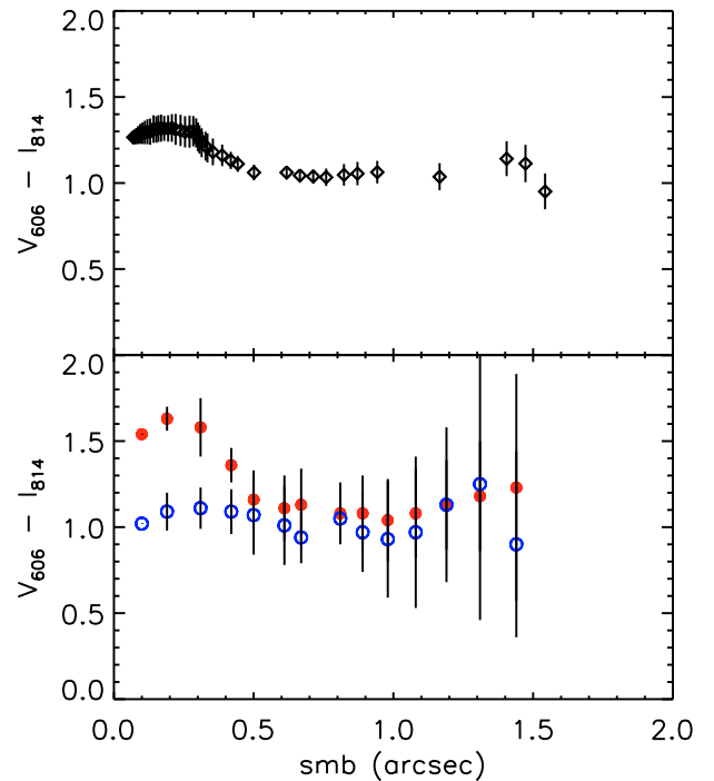
Fig. 8. a) Surface brightness map and colour map for an inclined galaxy. The map side is 6'' . Darker areas correspond to brighter and redder regions, respectively. b) Observed ( F606W - F814W ) colour profile derived from an elliptically-averaged surface brightness profile. c) Colour profiles derived along 40^\circ wedge-shaped apertures opening on both semi-minor axes; filled circles: side reddened by dust in the disk; open circles: profile that diminishes dust reddening effect since its light is not seen through the disk.
