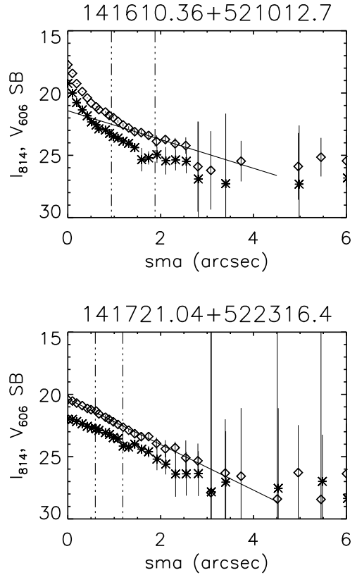
Fig. 7. Observed surface brightness averaged profiles derived from 15^\circ wedge-shaped apertures over both semi-major axes. Diamonds: F814W band. Asterisks: F606W band. Both galaxies belong to the high-inclination sample. The solid line is the exponential law fit over the outer regions of the profiles. Vertical dashed lines: 1 and 2 times the scale length of the exponential law, respectively; range in which disk colours were measured. The upper galaxy has \eta > 1 , while the lower one has \eta < 1 .
