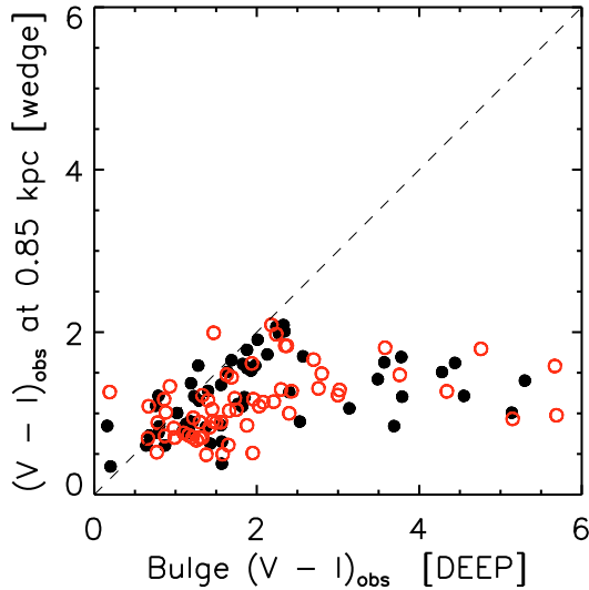
Fig. 10. Observed (F606W - F814W) wedge colour measured at 0.85 kpc vs. integrated bulge colour from DEEP bulge-disk decomposition, for the 123 galaxies in our sample for which the DEEP database lists a bulge colour. Filled circles: galaxies from the low-inclination sample. Open circles: galaxies from the high-inclination sample.
