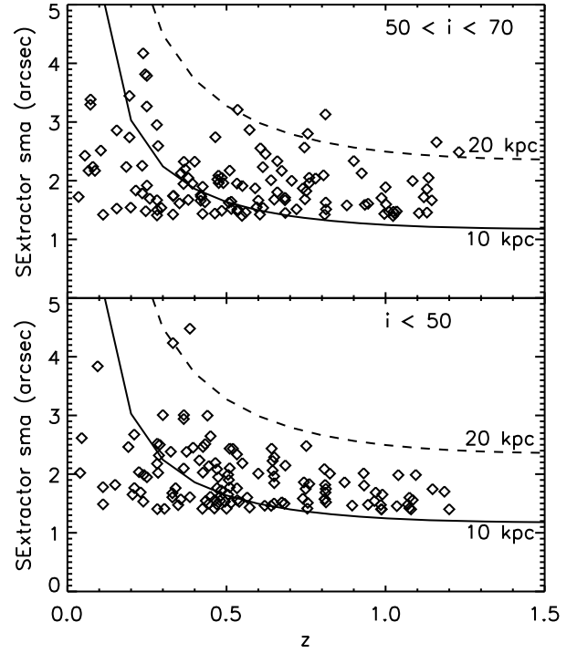
Fig. 3. Distribution of F814W semi-major axis in arcsec (from SETRACTOR A_IMAGE size parameter) vs. redshift for the high-inclination and low-inclination samples. Solid line: apparent size in arcsec for galaxies with a semi-major axis equal to 10 kpc. Dashed lines: the same for a semi-major axis equal to 20 kpc.
