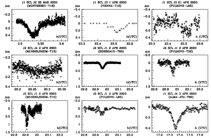
Fig. 34. Light curves for the observations of the mutual events of the Galilean satellites in 2002–2003.
