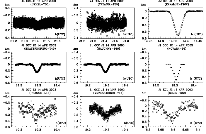
Fig. 36. Light curves for the observations of the mutual events of the Galilean satellites in 2002–2003.
