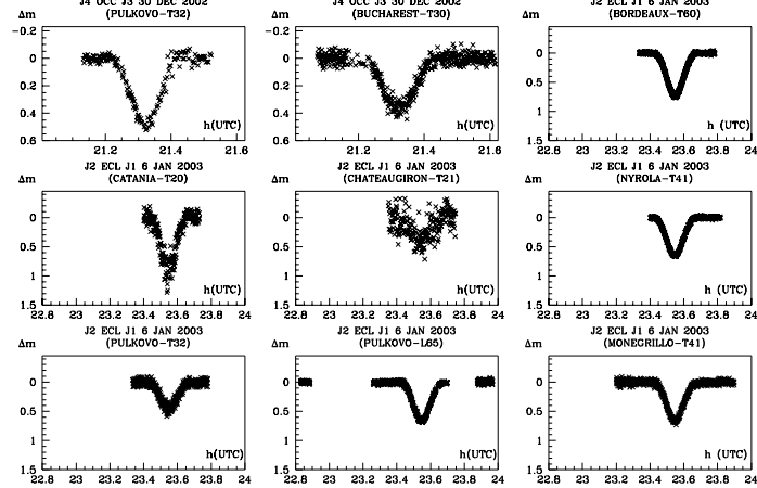
Fig. 6. Light curves for the observations of the mutual events of the Galilean satellites in 2002–2003.
