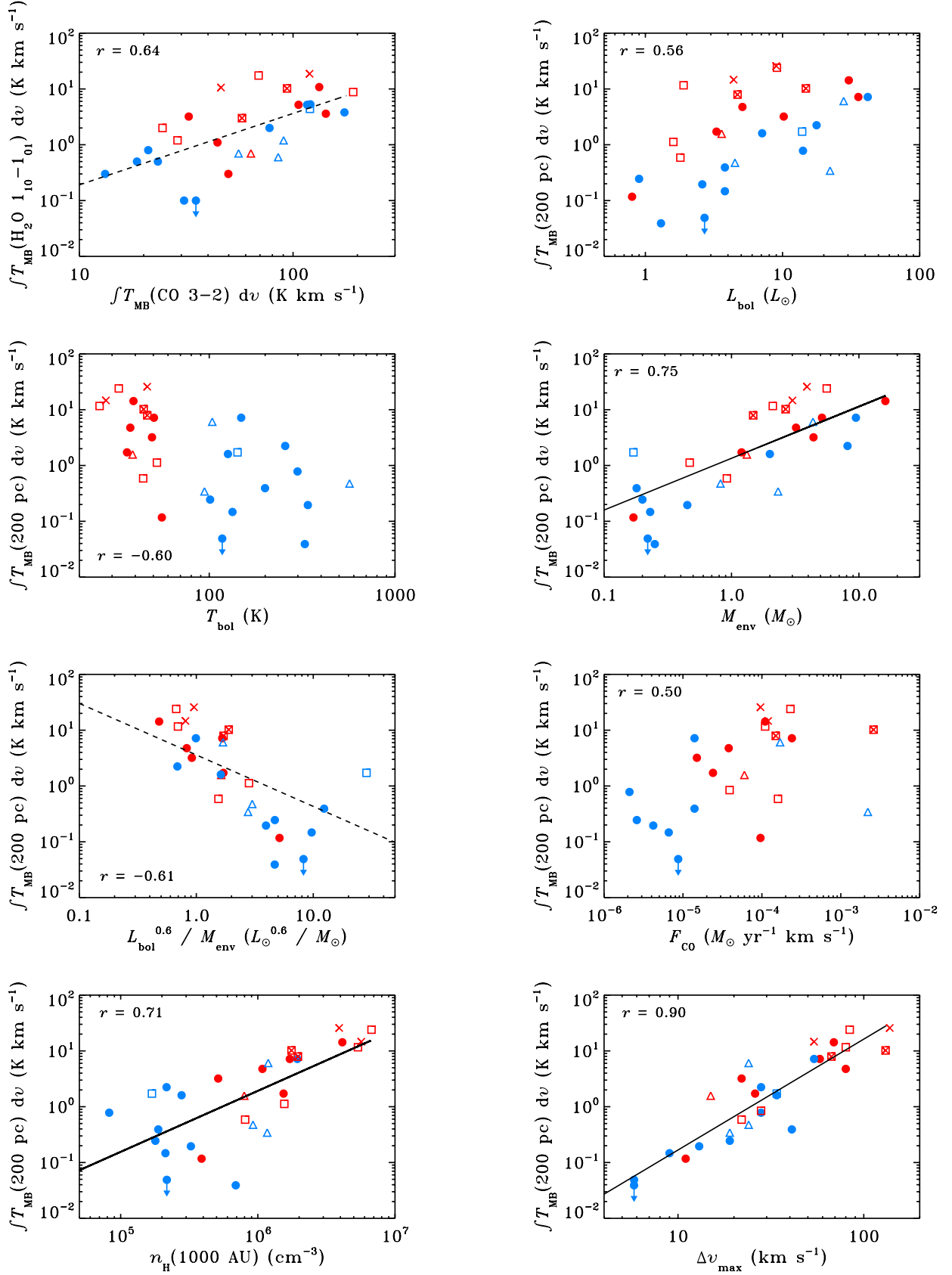
Fig. 6. Correlation plots showing the integrated \text{H}_2\text{O} 1_{10}\text{--}1_{01} 557 GHz line intensity scaled to a distance of 200 pc as a function of various envelope parameters; the \text{H}_2\text{O} intensity is not scaled when comparing to CO 3–2 emission. Class 0 sources are marked in red, Class I sources in blue; sources with bullet emission are marked with crosses, inverse P-Cygni profiles with squares and regular P-Cygni profiles with triangles; the upper limit for TMC1A is marked with an arrow. Strong correlations ( |r| > 0.7 ) are marked with full lines, tentative correlations ( 0.6 < |r| < 0.7 ) with dashed lines. The parameters are (from left to right, top to bottom): CO 3–2 emission, L_{\text{bol}} , T_{\text{bol}} , M_{\text{env}} , the evolutionary parameter L_{\text{bol}}^{0.6}/M_{\text{env}} , F_{\text{CO}} , n(1000 \text{ AU}) and \Delta v_{\text{max}} .
