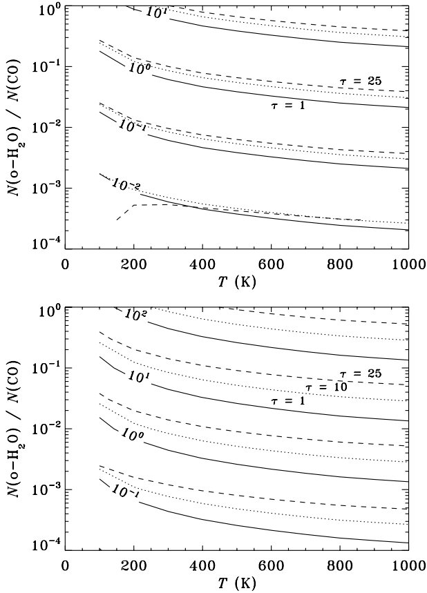
Fig. 13. \text{H}_2\text{O}/\text{CO} column density ratio as a function of kinetic gas temperature for three \text{H}_2\text{O} optical depths, \tau = 1, 10 and 25 ( \text{CO} is assumed to be optically thin in all cases). Contours are for intensity ratios of \text{H}_2\text{O } 1_{10}-1_{01}/\text{CO } 3-2 . The top panel shows the ratio for a density of n_{\text{H}} = 10^5 \text{ cm}^{-3} while the bottom panel is for a density of 10^6 \text{ cm}^{-3} .
