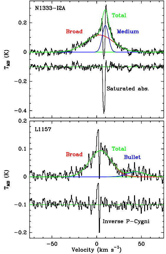
Fig. 3. Gaussian decomposition of the H 2 O 1 10 –1 01 spectra towards the two sources NGC 1333-IRAS2A and L1157. The individual Gaussian components are shown overlaid on the spectra and the residual is plotted below. The saturated absorption and inverse P-Cygni profile are not fitted by Gaussians.
