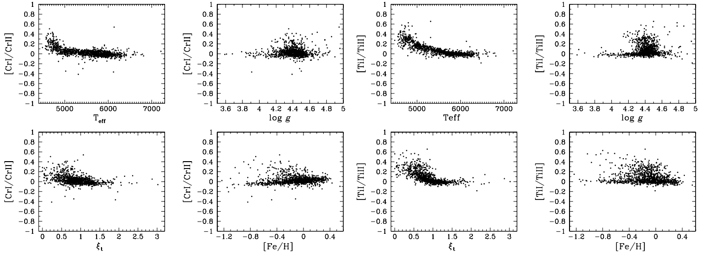
Fig. 3. [CrI/CrII] and [TiI/TiII] as a function of atmospheric parameters.
