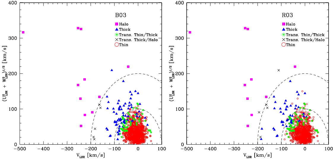
Fig. 6. Toomre diagram for the entire sample. The left and right panels show the separation of the stellar groups according to the B03 and R03 criteria, respectively. The symbols are explained in the figure.
