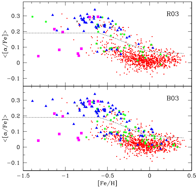
Fig. 7. Abundance ratios [\alpha/Fe] vs. [Fe/H] for the total sample. The blue triangles refer to the thick disk, red circles to the thin disk. The green asterisks and the black crosses refer to the transition stars between thin-thick and thick-halo, respectively. Magenta squares represent the stars belonging to the halo. The black dashed curve separates the stars with high- and low- \alpha content.
