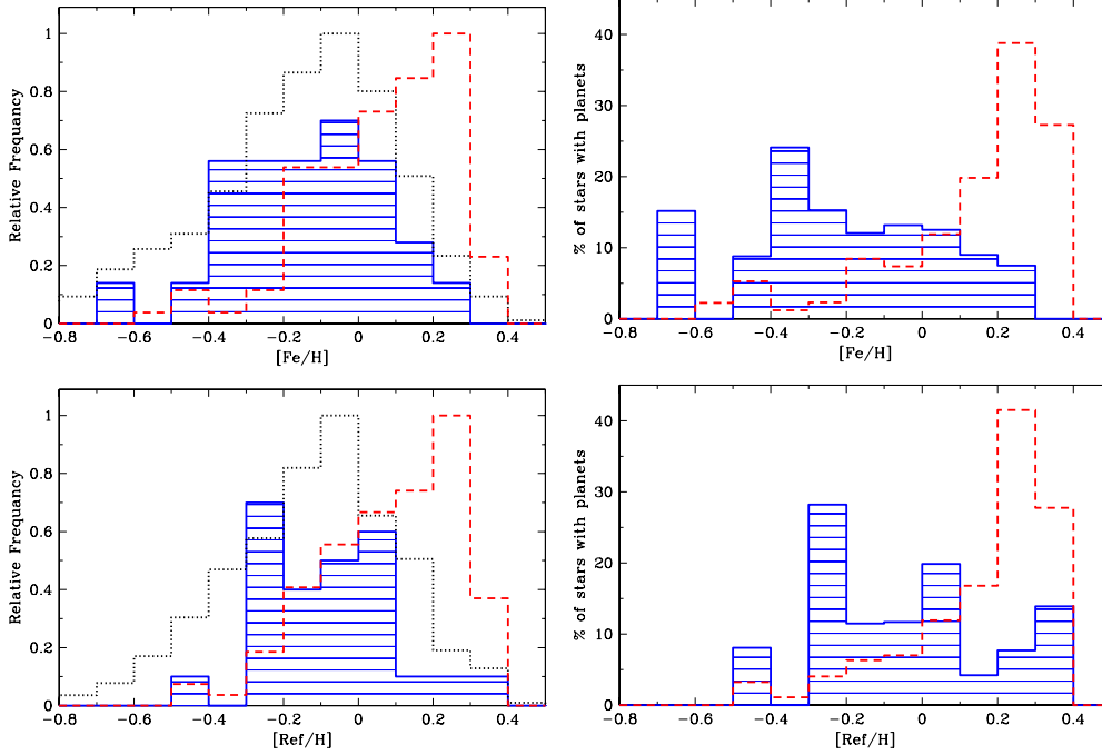
Fig. 11. Left – [\text{Fe}/\text{H}] and [\text{Ref}/\text{H}] distribution of the sample stars. The distribution lines for Jovian, Neptunian/super-Earth host and non-host stars are the same as in Fig. 9. The Neptunian and super-Earth distribution was set smaller for clarity. Right – Percentage of stars with giant (red dashed) and exclusively Neptunian and super-Earth (shaded blue) planets as a function of [\text{Fe}/\text{H}] and [\text{Ref}/\text{H}] . The Neptunian and super-Earth distribution was multiplied by 5 for better visibility.
