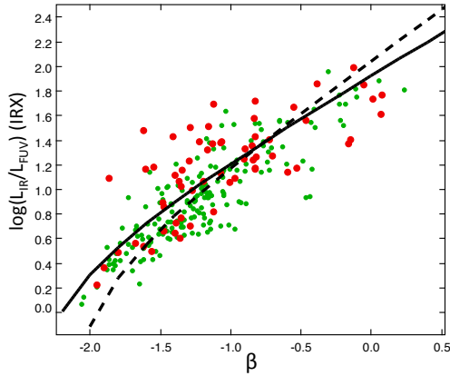
Fig. 16. The observed slope \beta is plotted versus \log(L_{\text{IR}}/L_{\text{FUV}}) = \text{IRX} . The symbols are the same as in Fig. 3. The solid line is the relation found in this work, while the dashed line is that of Overzier et al. (2011).
