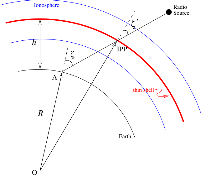
Fig. 1. Schematic representation of an astronomical signal piercing the ionosphere. The solid blue curves delineate the ionosphere. The thick red curve is the ionospheric thin shell approximation, and the thin black curve delineates the surface of the Earth.
